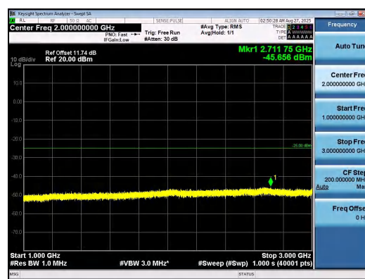
Band7-5MHz-QPSK-21100-1RB#24-1000~3000- PASS
