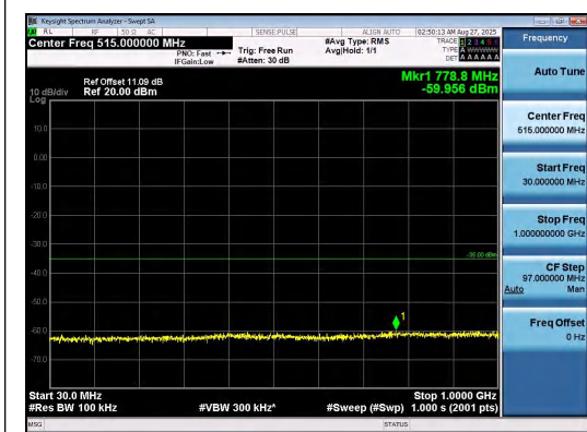
Band7-5MHz-QPSK-21100-1RB#24-30~1000-PA SS
