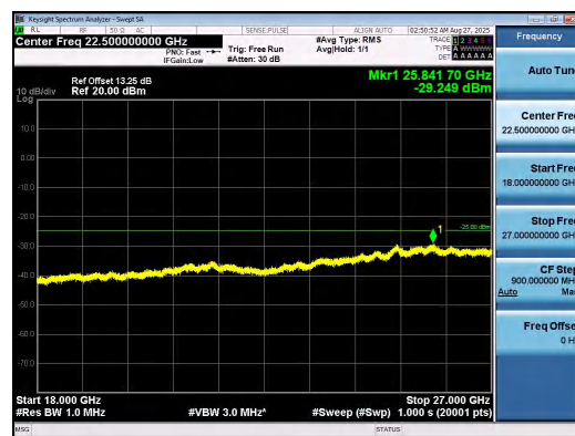
Band7-5MHz-QPSK-21100-1RB#24-18000~270 00-PASS
