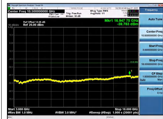
Band7-5MHz-QPSK-21100-1RB#24-3000~1800 0-PASS
