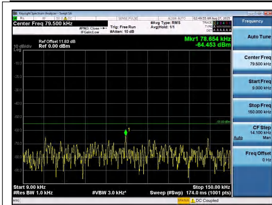
Band7-5MHz-QPSK-21100-1RB#24-0.009~0.15- PASS
