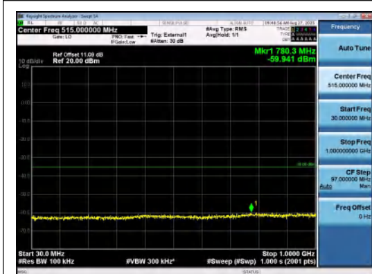
Band41(2535-2655)-5MHz-QPSK-40640-1RB#0- 30~1000-PASS
