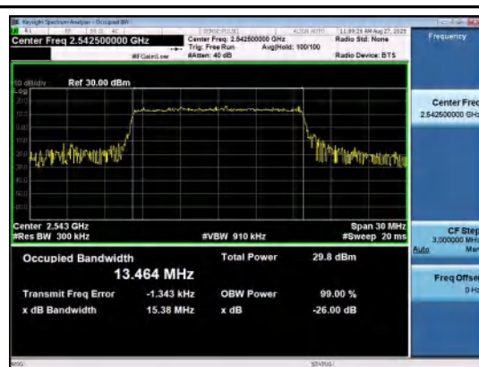
Band41(2535-2655)-15MHz-16QAM-40115-75RB# 0-PASS
