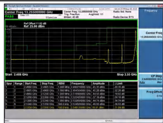
Band41(2535-2655)-15MHz-QPSK-40115-1RB#74 -PASS
