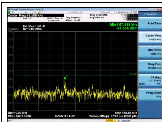
Band41(2535-2655)-10MHz-16QAM-40090-1RB #49-0.009~0.15-PASS
