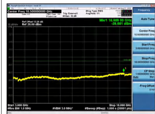
Band41(2535-2655)-5MHz-QPSK-40640-1RB#0- 3000~18000-PASS
