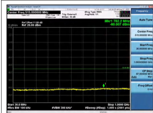
Band41(2535-2655)-10MHz-16QAM-40090-1RB #49-30~1000-PASS
