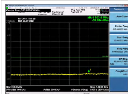
Band41(2535-2655)-5MHz-QPSK-41215-1RB#2 4-30~1000-PASS
