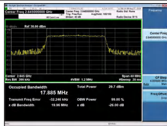
Band41(2535-2655)-20MHz-16QAM-41140-100RB #0-PASS
