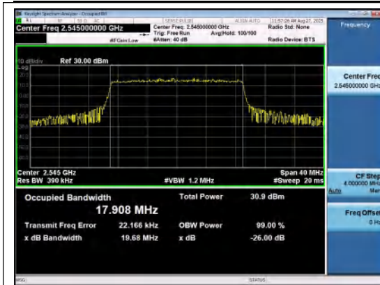
Band41(2535-2655)-20MHz-QPSK-40140-100RB #0-PASS
