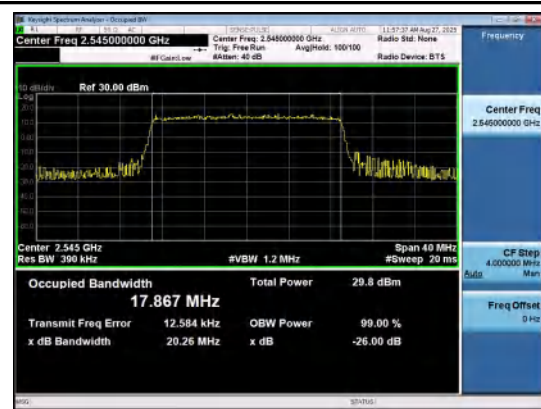
Band41(2535-2655)-20MHz-16QAM-40140-100RB #0-PASS
