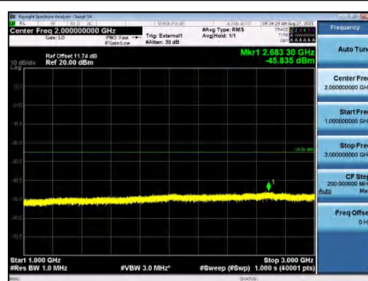
Band41(2535-2655)-5MHz-16QAM-40065-1RB# 0-1000~3000-PASS
