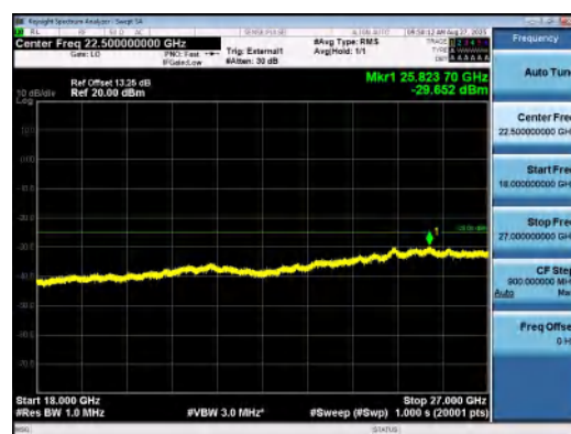
Band41(2535-2655)-5MHz-QPSK-40640-1RB#0- 18000~27000-PASS
