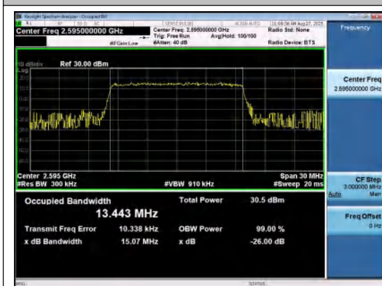
Band41(2535-2655)-15MHz-QPSK-40640-75RB# 0-PASS
