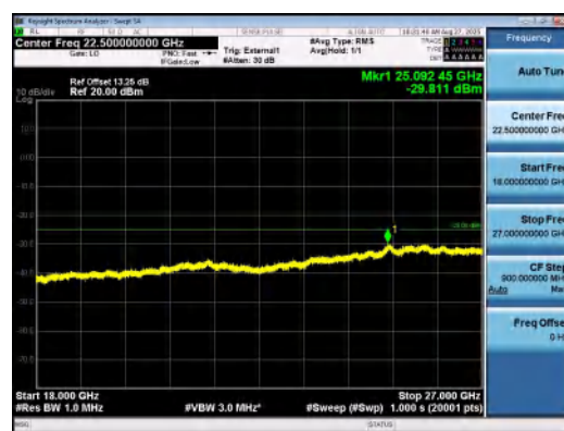
Band41(2535-2655)-10MHz-16QAM-40090-1RB #49-18000~27000-PASS
