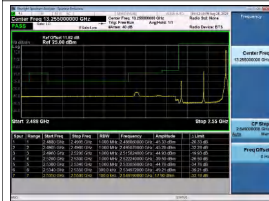
Band41(2535-2655)-15MHz-16QAM-40115-1RB# 74-PASS
