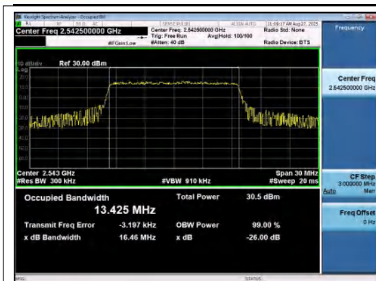
Band41(2535-2655)-15MHz-QPSK-40115-75RB# 0-PASS
