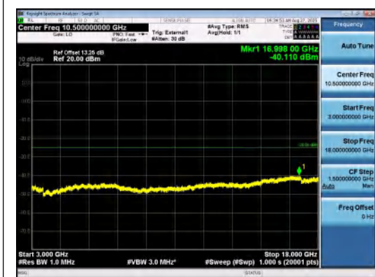
Band41(2535-2655)-5MHz-16QAM-40065-1RB# 0-3000~18000-PASS
