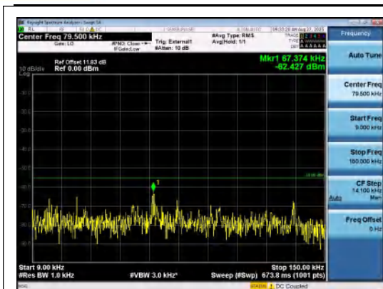
Band41(2535-2655)-5MHz-16QAM-40065-1RB# 0-0.009~0.15-PASS
