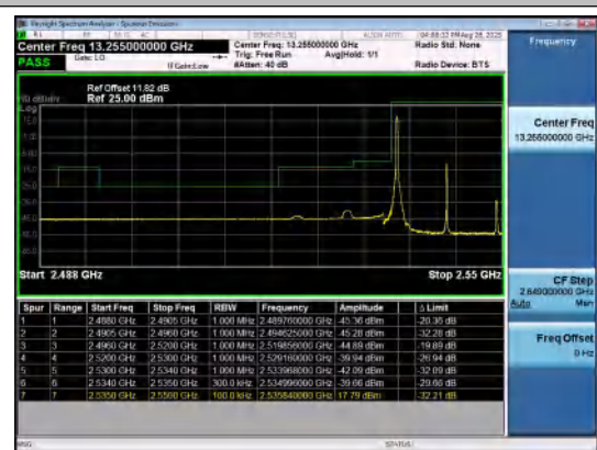
Band41(2535-2655)-15MHz-16QAM-40115-1RB#0 -PASS
