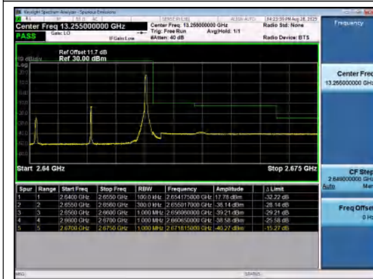
Band41(2535-2655)-15MHz-16QAM-41165-1RB# 74-PASS
