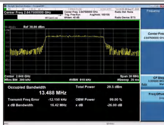
Band41(2535-2655)-15MHz-16QAM-41165-75RB# 0-PASS
