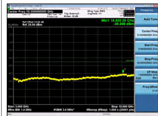
Band41(2535-2655)-10MHz-16QAM-40090-1RB #49-3000~18000-PASS
