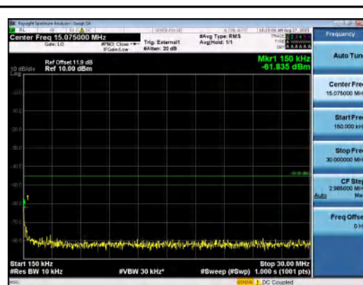
Band41(2535-2655)-5MHz-QPSK-41215-1RB#2 4-0.15~30-PASS
