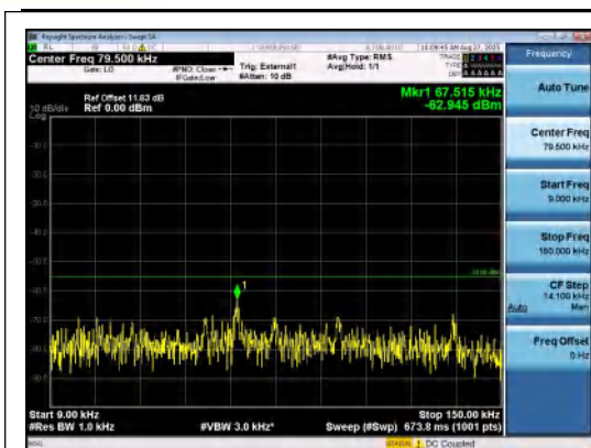
Band41(2535-2655)-5MHz-QPSK-41215-1RB#2 4-0.009~0.15-PASS
