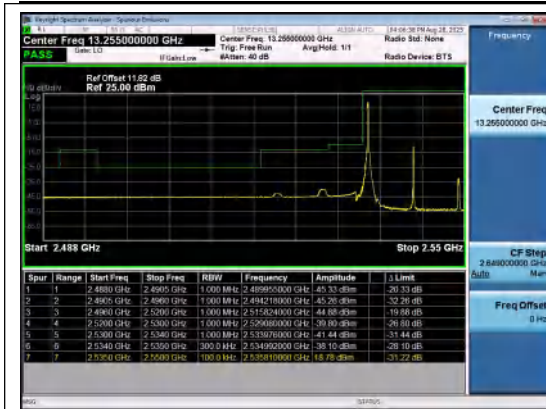
Band41(2535-2655)-15MHz-QPSK-40115-1RB#0 -PASS
