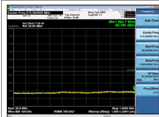
Band41(2535-2655)-5MHz-16QAM-40065-1RB# 0-30~1000-PASS
