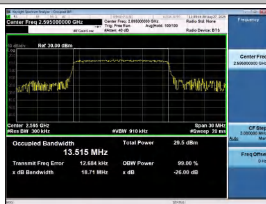
Band41(2535-2655)-15MHz-16QAM-40640-75RB# 0-PASS
