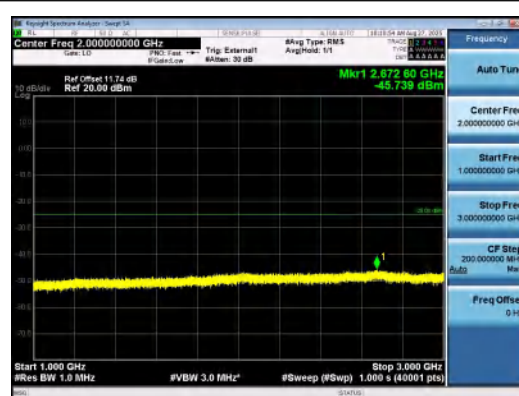
Band41(2535-2655)-5MHz-QPSK-41215-1RB#2 4-1000~3000-PASS
