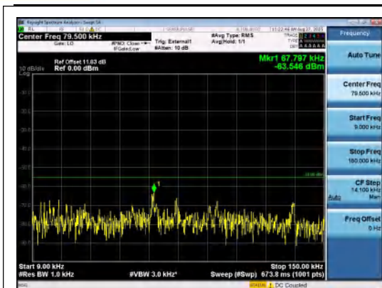
Band41(2535-2655)-15MHz-16QAM-40115-75R B#0-0.009~0.15-PASS
