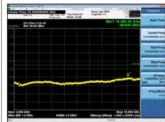
Band41(2535-2655)-15MHz-16QAM-40115-75R B#0-3000~18000-PASS
