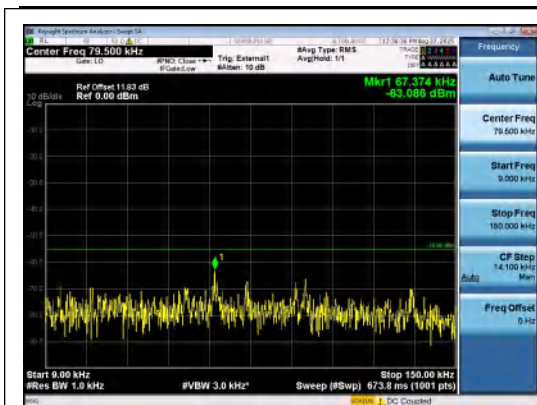
Band41(2535-2655)-20MHz-16QAM-41140-1RB #99-0.009~0.15-PASS
