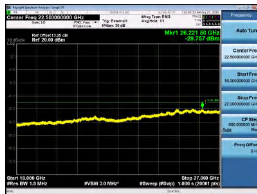
Band41(2535-2655)-15MHz-16QAM-41165-1RB #74-18000~27000-PASS
