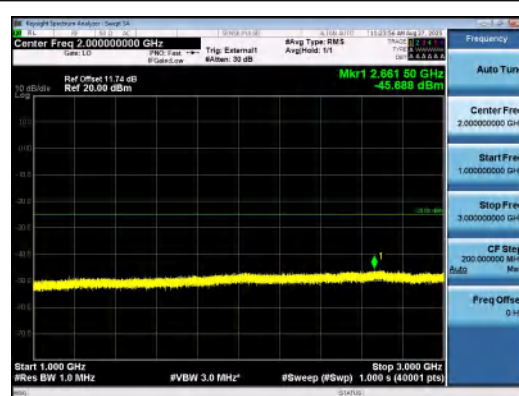
Band41(2535-2655)-15MHz-16QAM-40115-75R B#0-1000~3000-PASS
