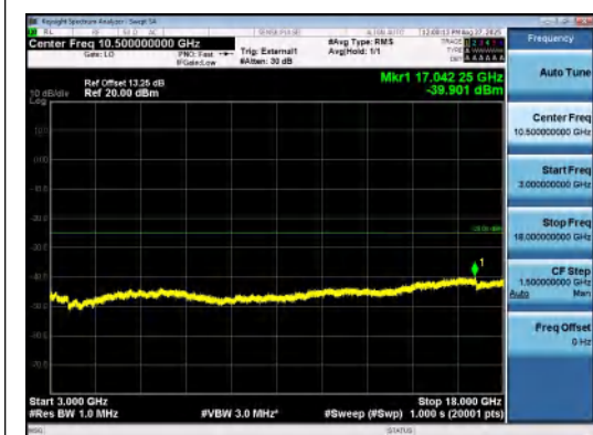
Band41(2535-2655)-20MHz-QPSK-40140-1RB# 0-3000~18000-PASS
