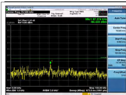
Band41(2535-2655)-20MHz-QPSK-40140-1RB# 0-0.009~0.15-PASS
