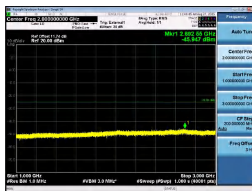
Band41(2535-2655)-15MHz-16QAM-41165-1RB #74-1000~3000-PASS
