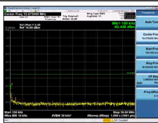
Band41(2535-2655)-15MHz-16QAM-41165-1RB #74-0.15~30-PASS
