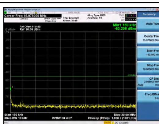
Band41(2535-2655)-15MHz-16QAM-40115-75R B#0-0.15~30-PASS
