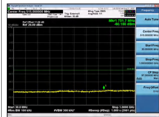
Band41(2535-2655)-10MHz-16QAM-40090-50R B#0-30~1000-PASS
