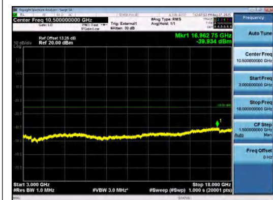
Band41(2535-2655)-20MHz-16QAM-40140-1RB #99-3000~18000-PASS
