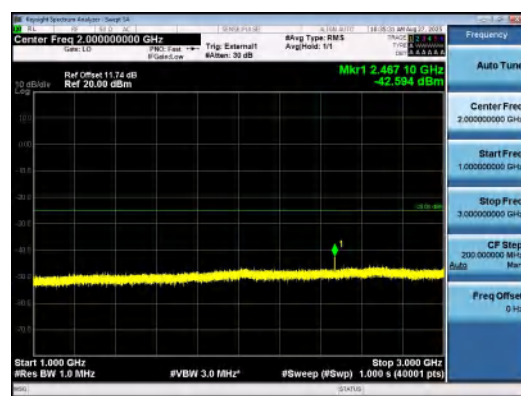
Band41(2535-2655)-10MHz-16QAM-40090-50R B#0-1000~3000-PASS
