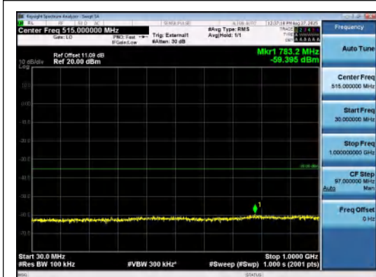
Band41(2535-2655)-20MHz-16QAM-41140-1RB #99-30~1000-PASS
