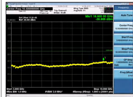
Band41(2535-2655)-15MHz-16QAM-41165-1RB #74-3000~18000-PASS
