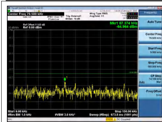
Band41(2535-2655)-10MHz-16QAM-40090-50R B#0-0.009~0.15-PASS
