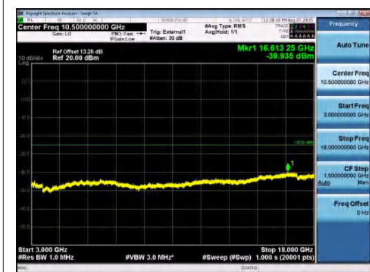
Band41(2535-2655)-20MHz-16QAM-41140-1RB #99-3000~18000-PASS
