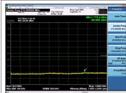
Band41(2535-2655)-20MHz-16QAM-40140-1RB #99-30~1000-PASS
