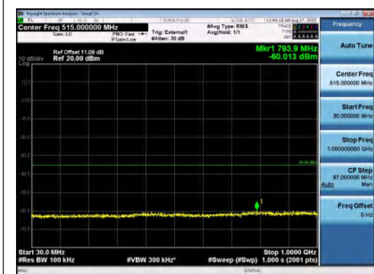
Band41(2535-2655)-15MHz-16QAM-41165-1RB #74-30~1000-PASS
