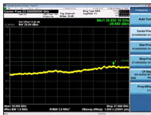
Band41(2535-2655)-20MHz-16QAM-40140-1RB #99-18000~27000-PASS
