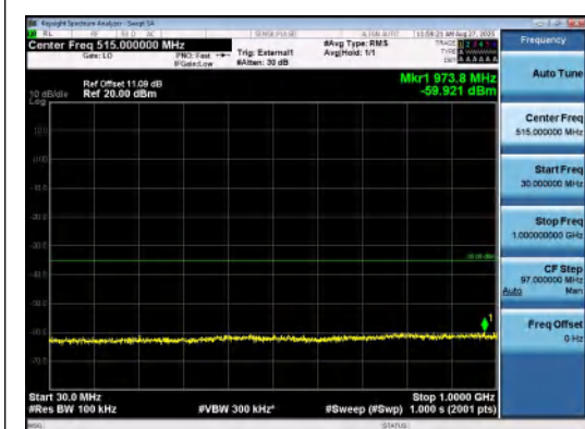
Band41(2535-2655)-20MHz-QPSK-40140-1RB# 0-30~1000-PASS
