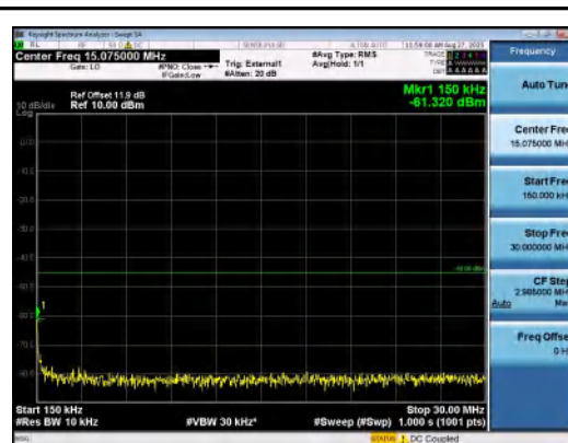
Band41(2535-2655)-20MHz-QPSK-40140-1RB# 0-0.15~30-PASS
