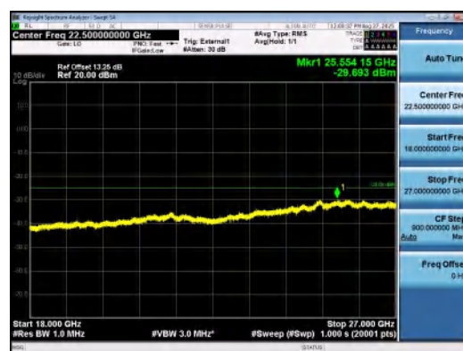
Band41(2535-2655)-20MHz-QPSK-40140-1RB# 0-18000~27000-PASS
