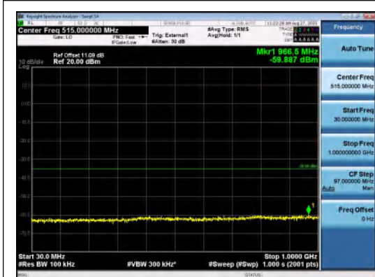
Band41(2535-2655)-15MHz-16QAM-40115-75R B#0-30~1000-PASS
