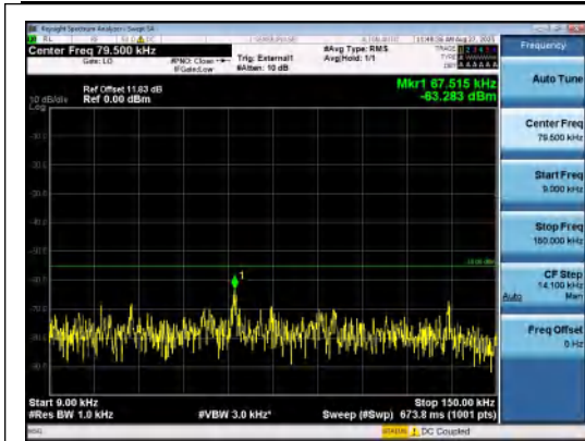
Band41(2535-2655)-15MHz-16QAM-41165-1RB #74-0.009~0.15-PASS
