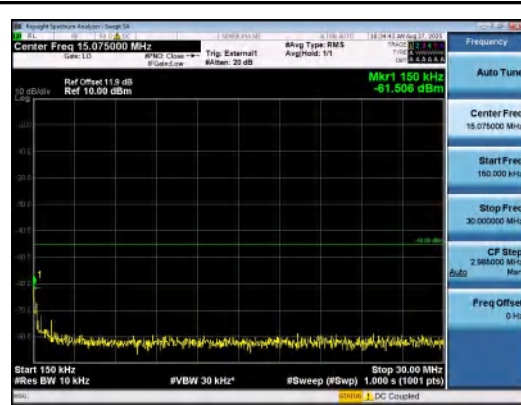
Band41(2535-2655)-10MHz-16QAM-40090-50R B#0-0.15~30-PASS
