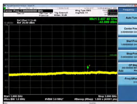
Band41(2535-2655)-20MHz-QPSK-40140-1RB# 0-1000~3000-PASS
