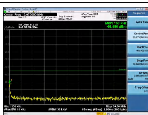
Band41(2535-2655)-20MHz-16QAM-41140-1RB #99-0.15~30-PASS
