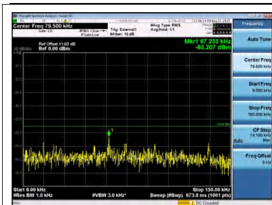
Band41(2535-2655)-20MHz-16QAM-40140-1RB #99-0.009~0.15-PASS
