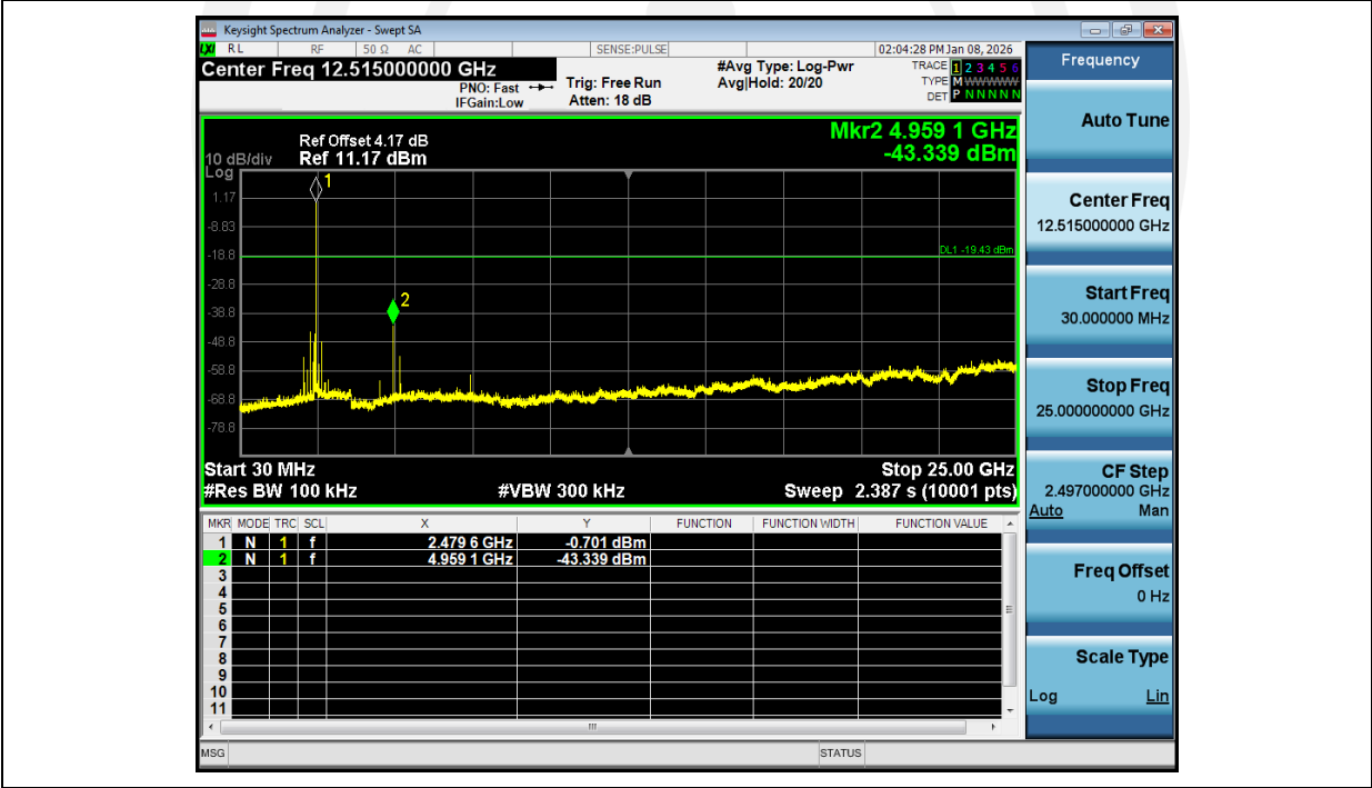
2_Spurious_Emissions_NVNT_ANT1_1-DH1_2480_00
