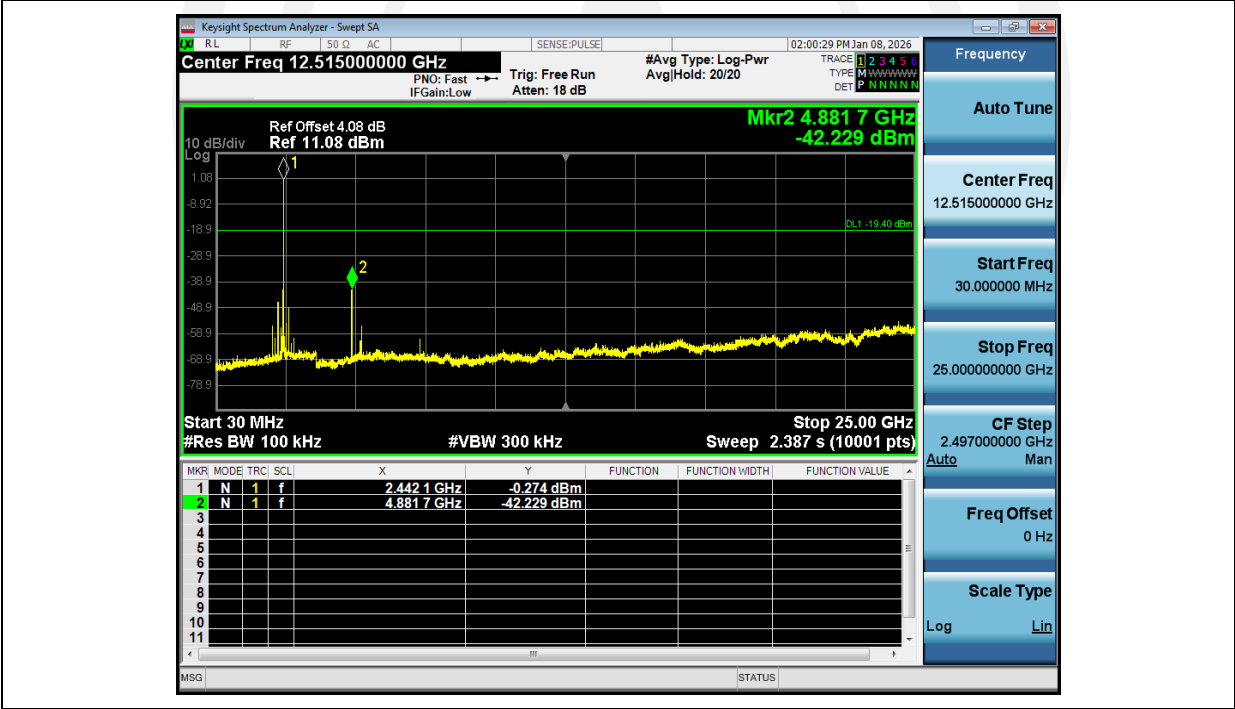
2_Spurious_Emissions_NVNT_ANT1_1-DH1_2441_00
