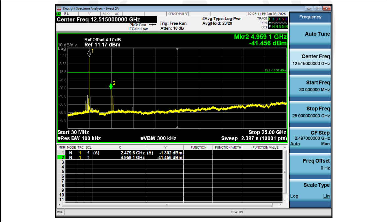
2_Spurious_Emissions_NVNT_ANT1_2-DH1_2480_00
