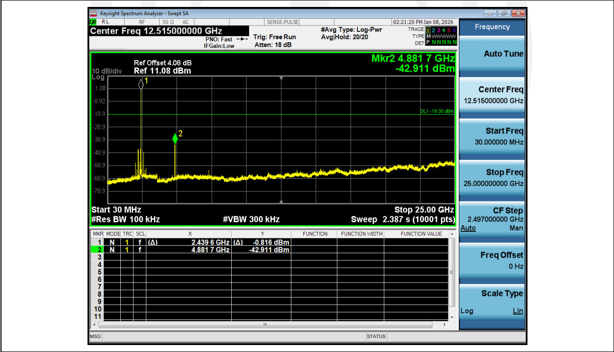
2_Spurious_Emissions_NVNT_ANT1_2-DH1_2441_00
