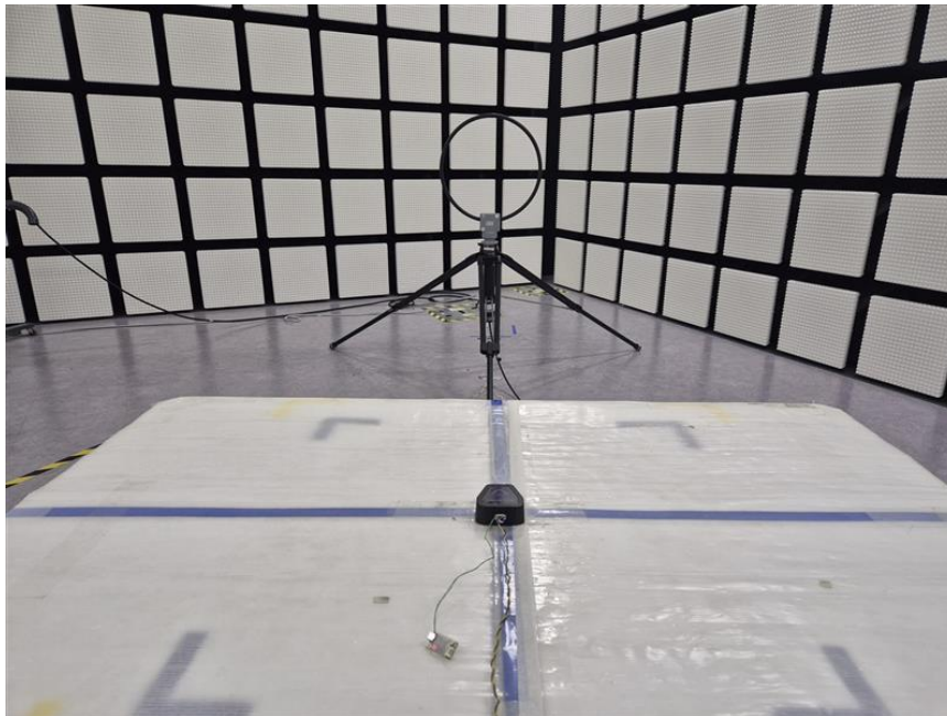
BELOW 30 MHz REAR TEST PHOTO
