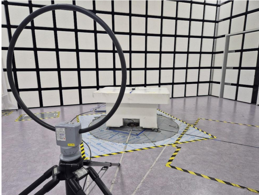
BELOW 30 MHz FRONT TEST PHOTO
