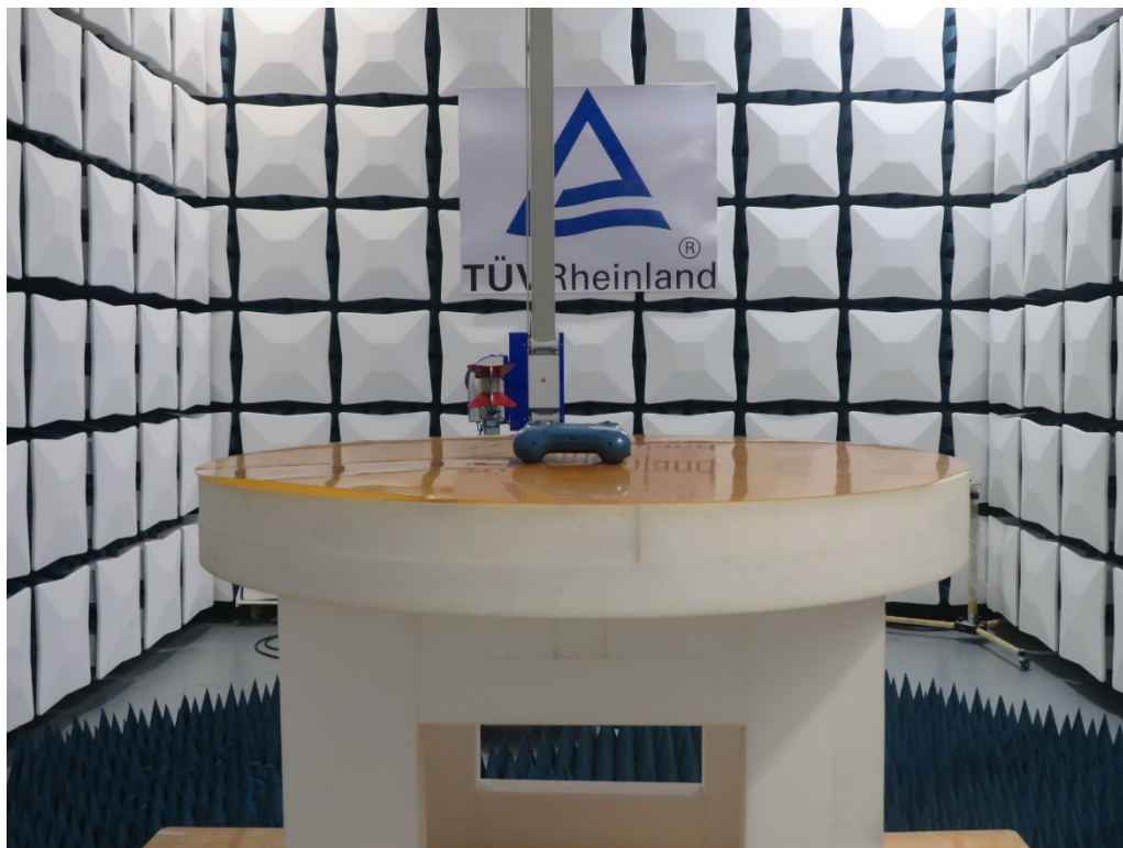
Photograph 2: Set-up photo for Radiated Emission, Above 1GHz
