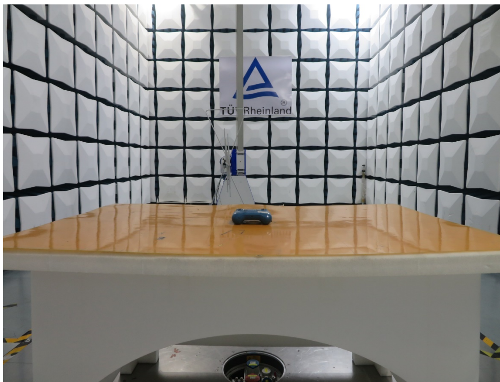
Photograph 1: Set-up photo for Radiated Emission, Below 1GHz
