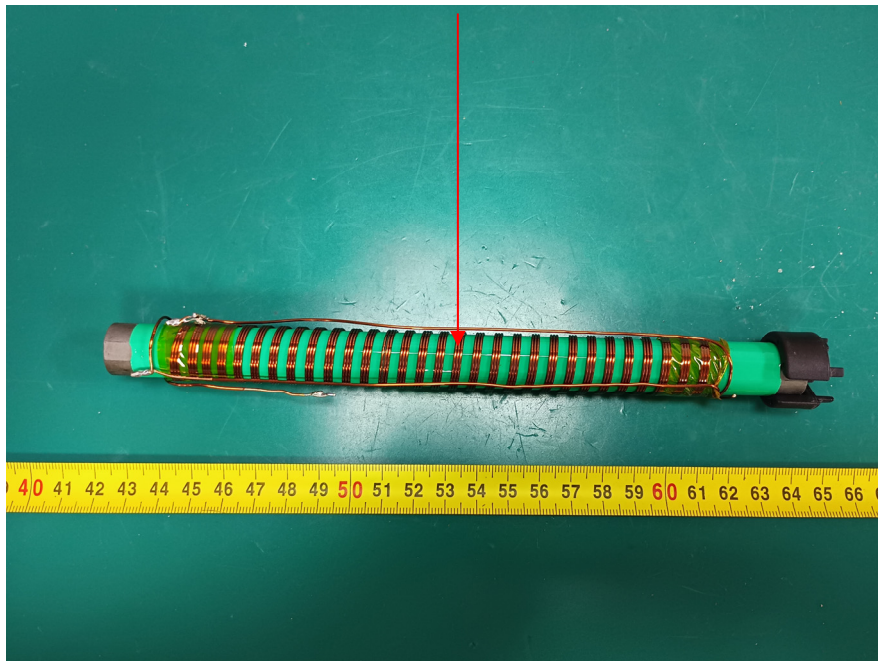
9.925-41.375kHz wound coil
