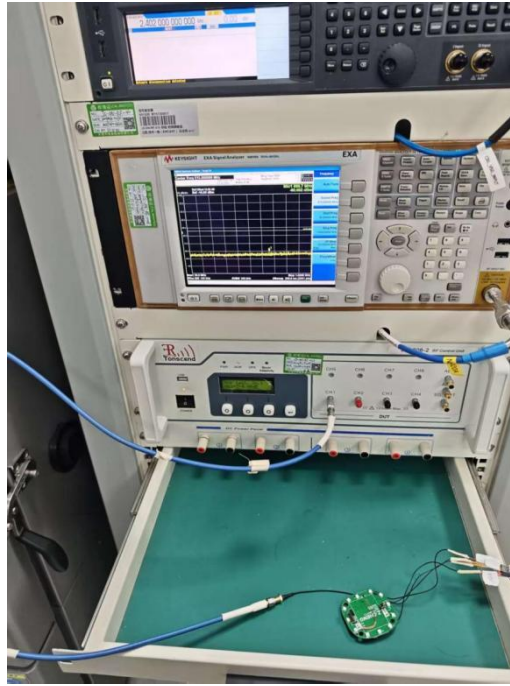
Conducted Emission View
