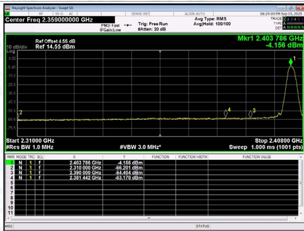
Restrict Band NVNT BLE 2Mbps 2404MHz Ant1 Average
