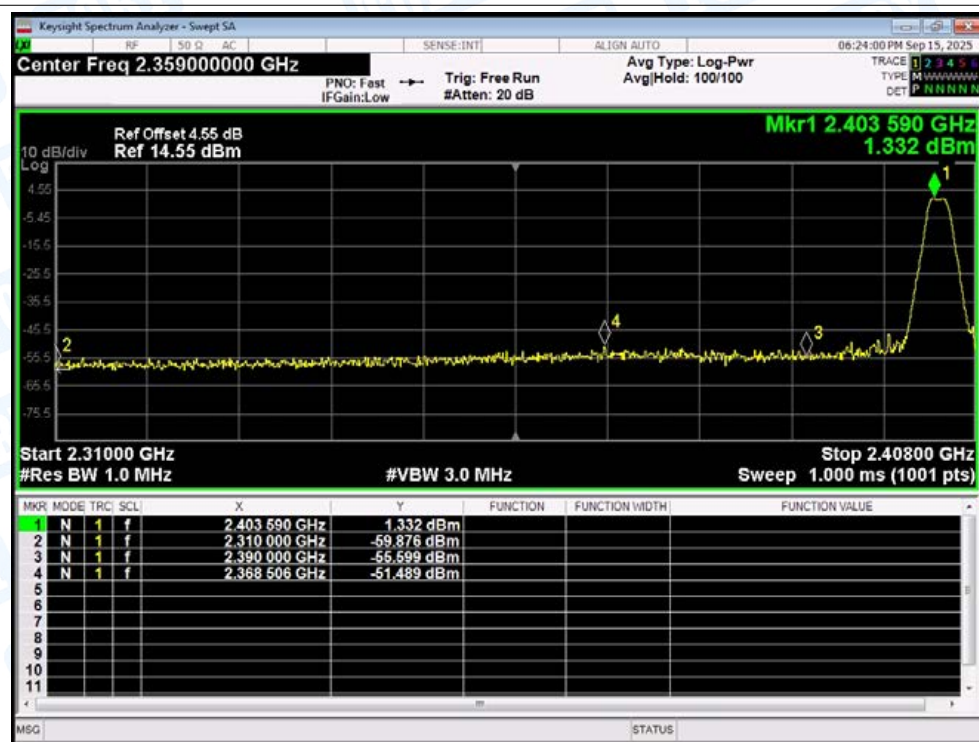
Restrict Band NVNT BLE 2Mbps 2404MHz Ant1 Average
