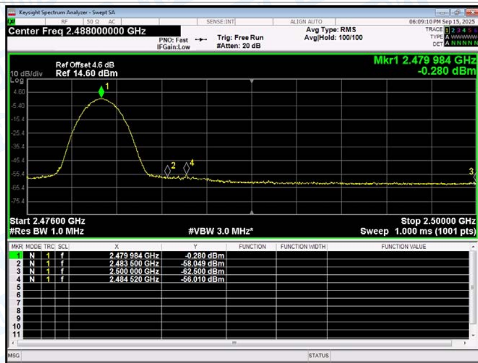
Restrict Band NVNT BLE 1Mbps 2480MHz Ant1 Average
