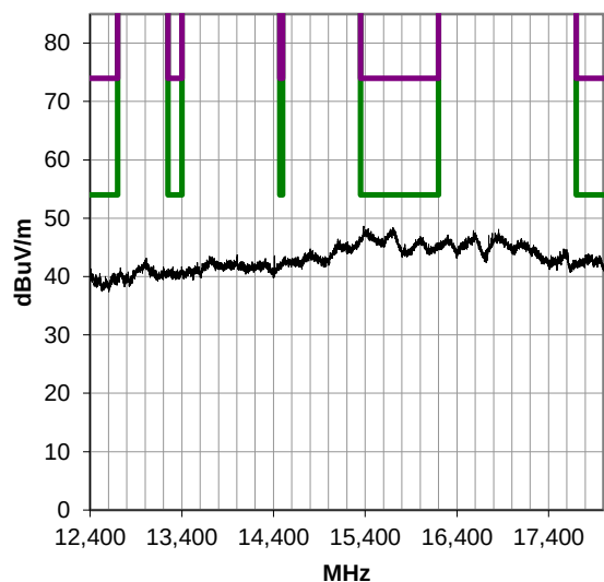
12400-18000 MHz, Run 23
