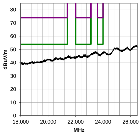
18000-26500 MHz, Run 58
