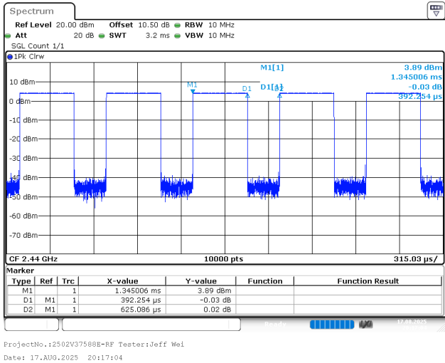
BLE_1M_Middle_Channel
