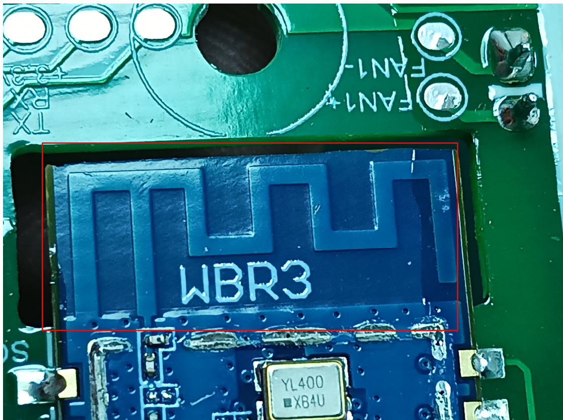
wifi/BT antenna
