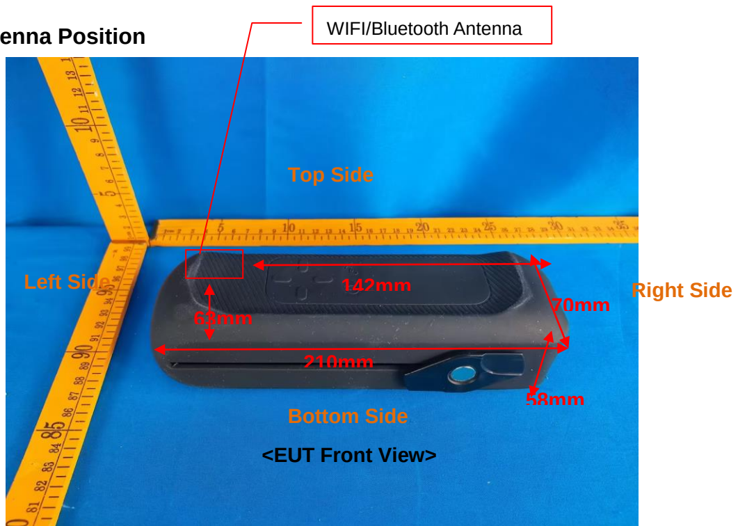
Fig 7.2Block Diagram for EUT Antenna Position
