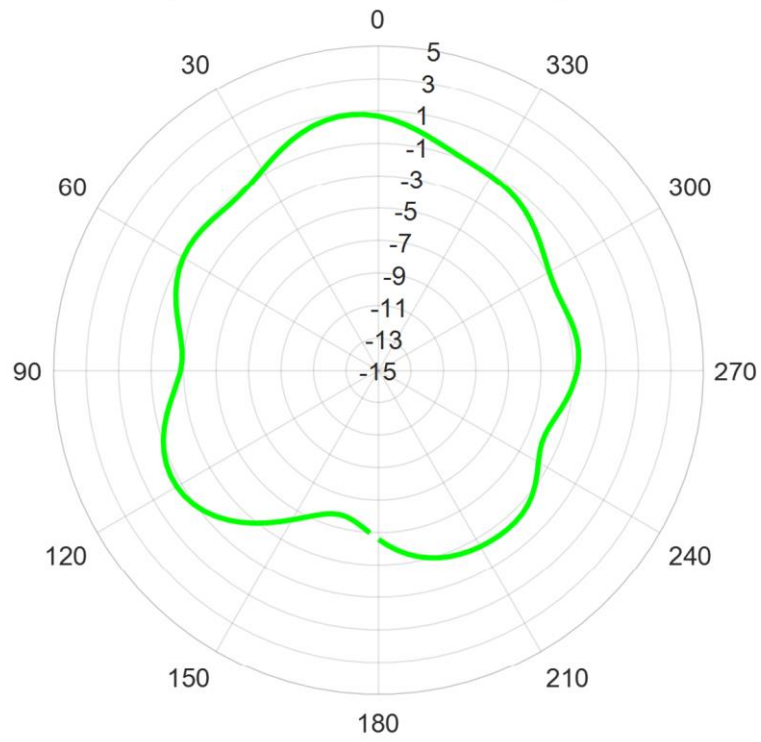
Freq = 2400 MHz Theta = 90 deg Gain
