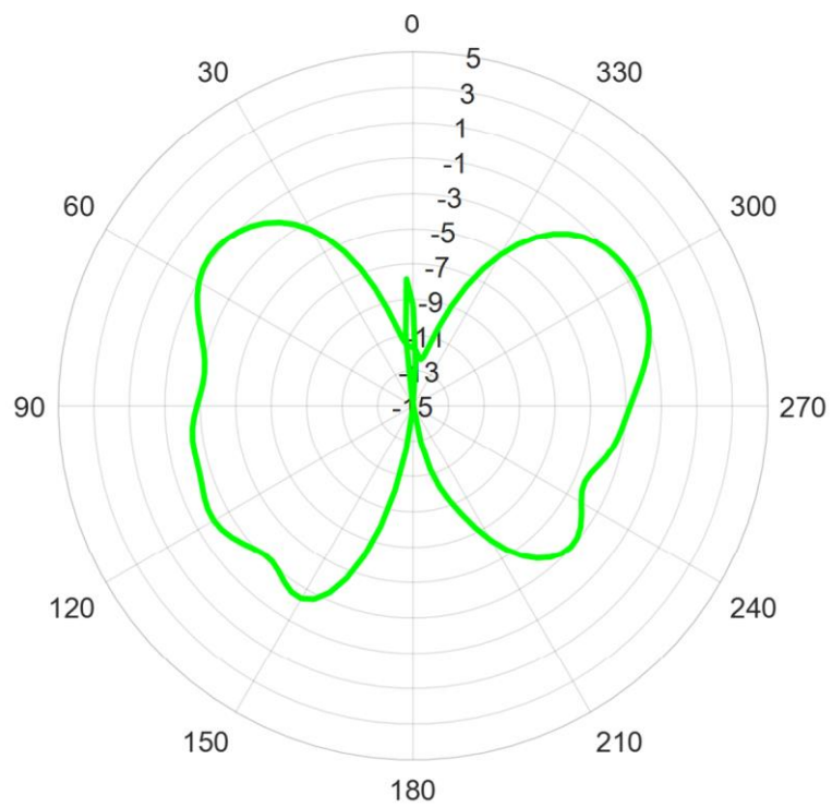
Freq = 2400 MHz Phi = 90 deg Gain
