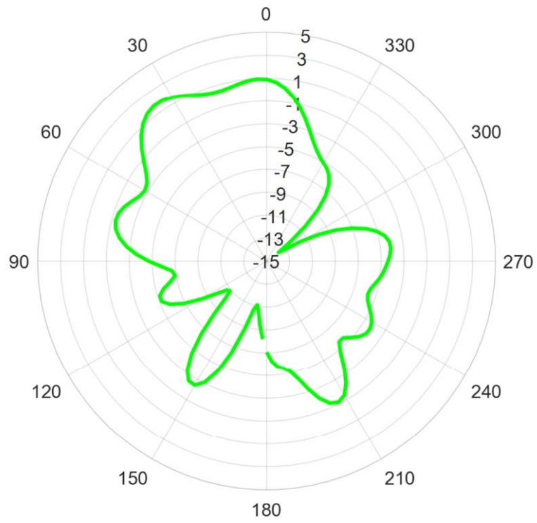
Freq = 5800 MHz Theta = 90 deg Gain
