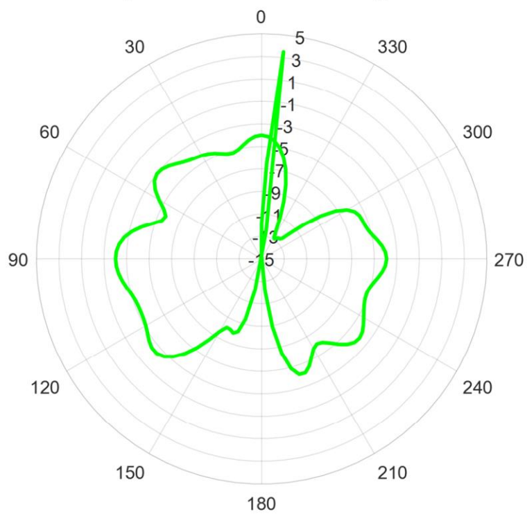
Freq = 5800 MHz Phi = 90 deg Gain
