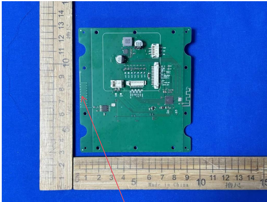
Remote control receiver antenna
