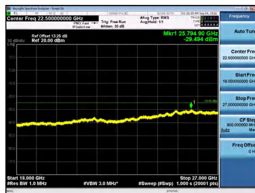
Band7-15MHz-QPSK-21100-1RB#0-18000~27000-PAS
