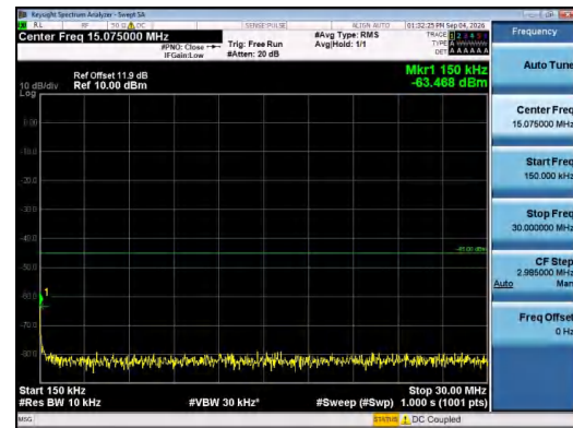
Band7-15MHz-QPSK-21375-1RB#74-0.15~30-PASS
