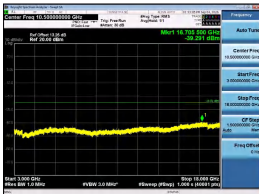
Band7-15MHz-QPSK-21375-1RB#74-3000~18000-PA SS
