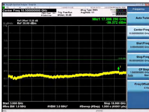
Band7-10MHz-16QAM-21100-1RB#0-3000~18000-PA
