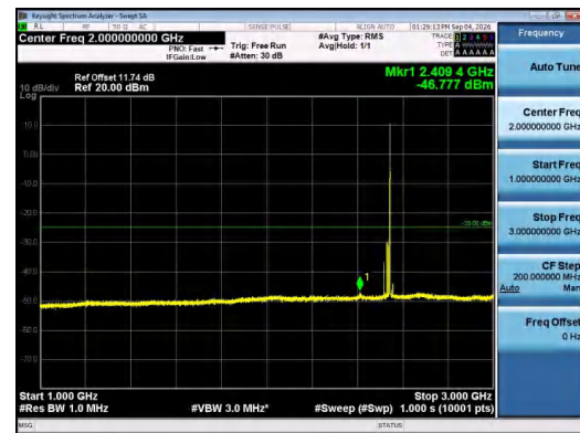
Band7-15MHz-16QAM-21100-1RB#74-1000~3000-PASS S
