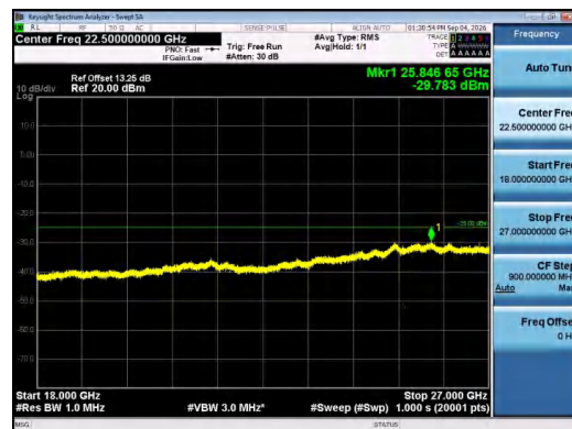
Band7-15MHz-QPSK-21375-1RB#0-18000~27000-PAS
