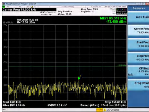
Band7-20MHz-16QAM-21350-1RB#99-0.009~0.15-PA SS
