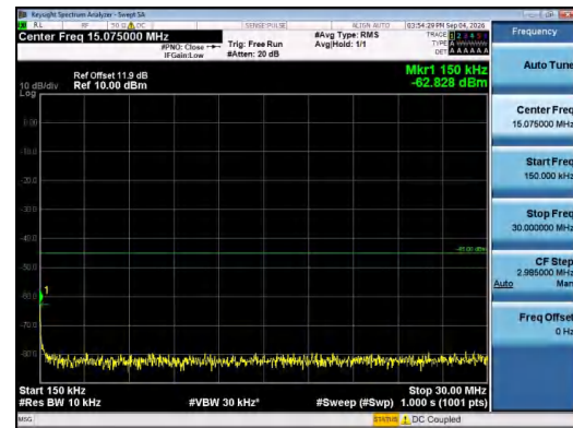
Band7-20MHz-16QAM-21100-1RB#99-0.15~30-PASS
