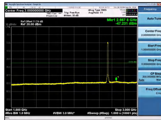
Band7-15MHz-QPSK-21100-75RB#0-1000~3000-PASS
