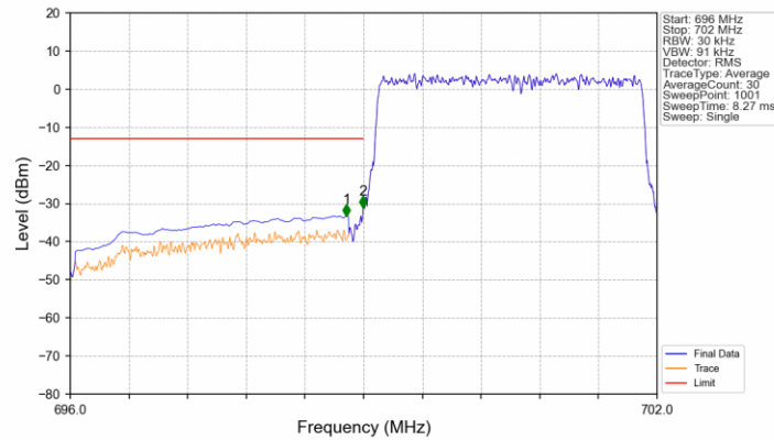
Band12_3MHz_16QAM_LCH_700.5MHz_RB_15_0_NTNV
