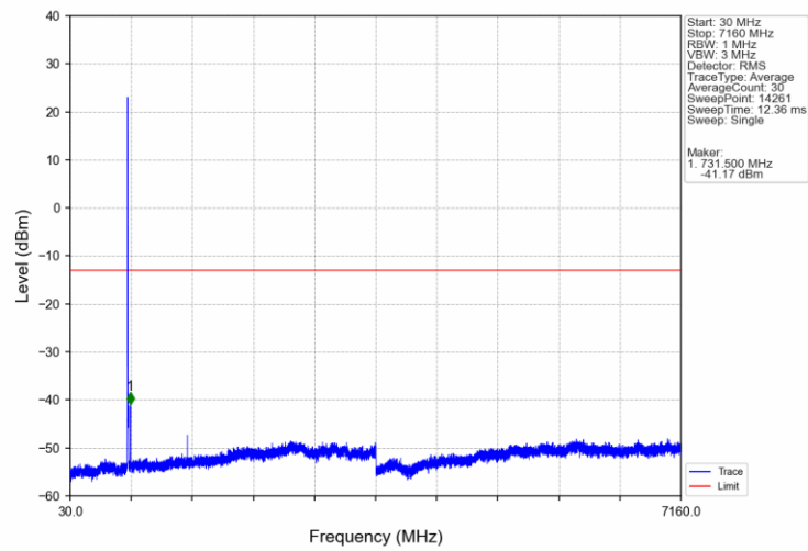
Band12_5MHz_QPSK_LCH_701.5MHz_RB_25_0_NTNV
