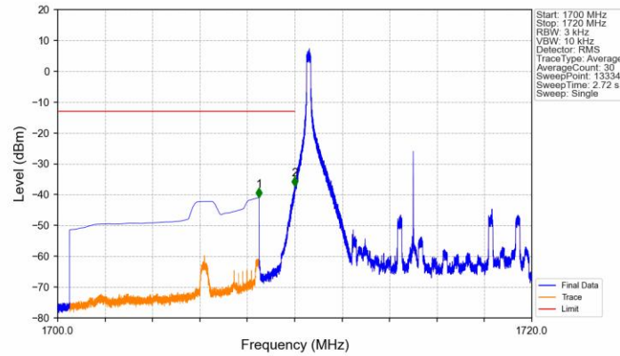
Band4_10MHz_QPSK_LCH_1715MHz_RB_1_0_NTNV
