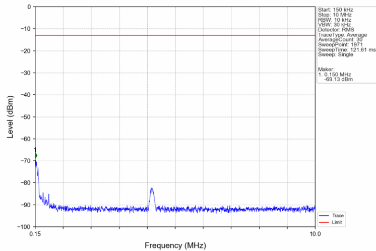
Band4_5MHz_16QAM_LCH_1712.5MHz_RB_1_0_NTNV
