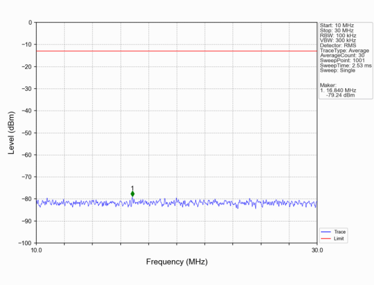
Band66 1.4MHz 16QAM LCH 1710.7MHz RB 1 0 NTN
