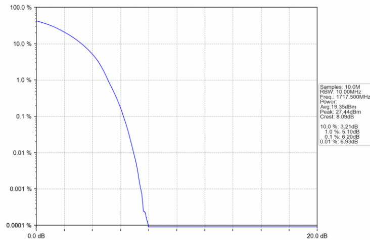
Band66 15MHz 16QAM LCH 1717.5MHz RB 75 0 NTNV
