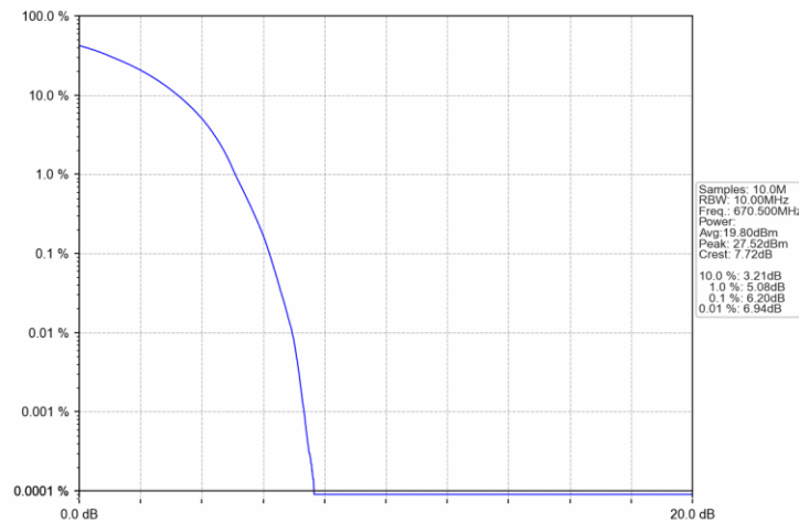
Band71 15MHz 16QAM LCH 670.5MHz RB 75 0 NTNV
