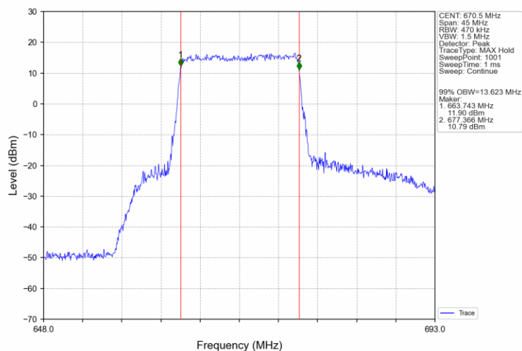
Band71 15MHz 16QAM LCH 670.5MHz RB 75 0 NTNV
