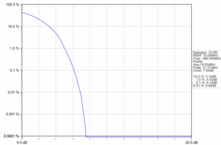
Band71 15MHz 16QAM HCH 690.5MHz RB 75 0 NTNV
