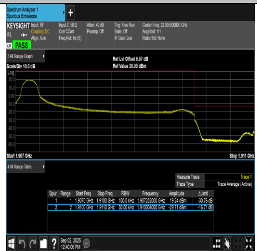
Band2-3MHz-16QAM-19185-1RB#0-PASS
