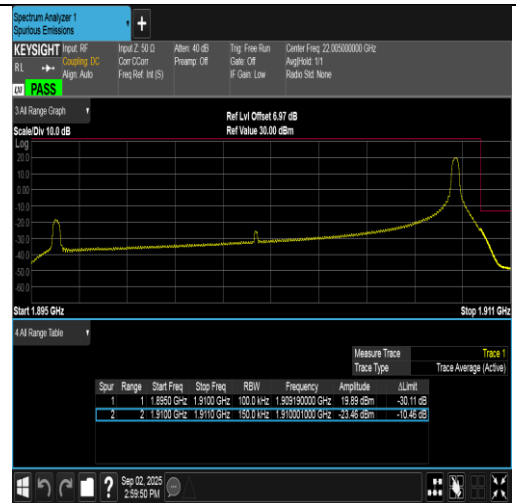
Band2-15MHz-QPSK-19125-1RB#74-PASS
