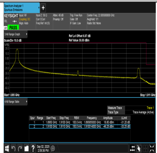
Band2-15MHz-16QAM-19125-1RB#0-PASS
