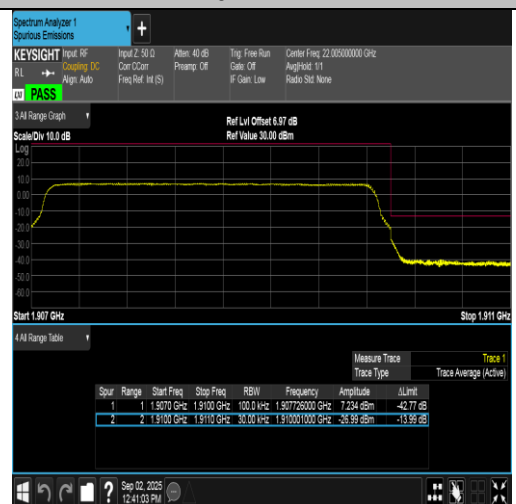
Band2-3MHz-16QAM-19185-15RB#0-PASS
