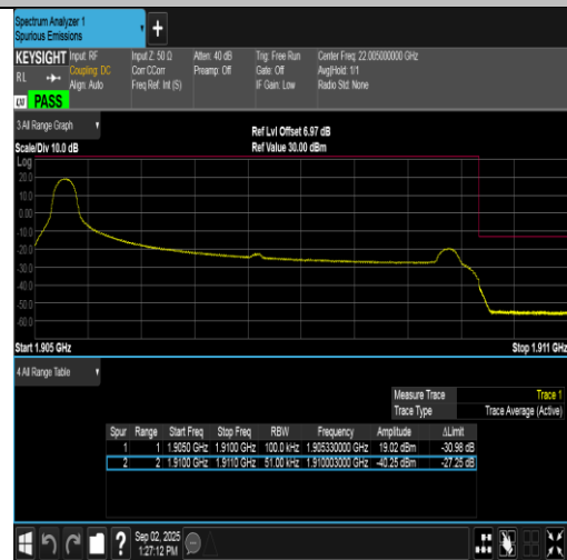
Band2-5MHz-16QAM-19175-1RB#0-PASS
