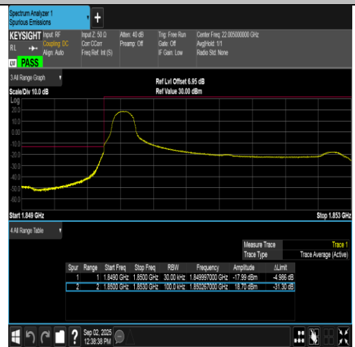
Band2-3MHz-16QAM-18615-1RB#0-PASS
