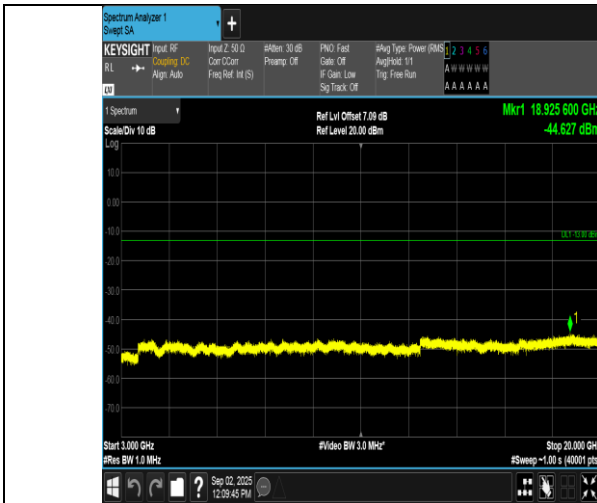
Band2-1.4MHz-16QAM-19193-1RB#5-3000~20000-PASS
