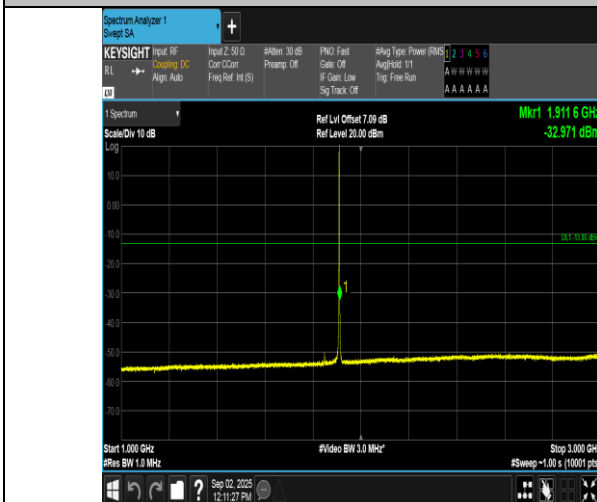
Band2-1.4MHz-16QAM-19193-6RB#0-1000~3000-PASS
