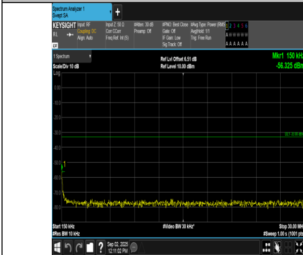
Band2-1.4MHz-16QAM-19193-6RB#0-0.15~30-PASS
