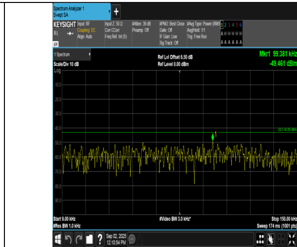
Band2-1.4MHz-16QAM-19193-6RB#0-0.009~0.15-PASS
