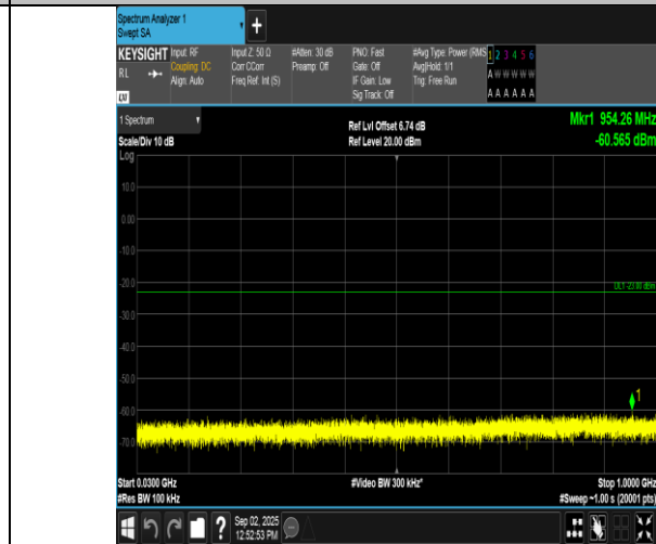
Band2-3MHz-16QAM-18900-15RB#0-30~1000-PASS
