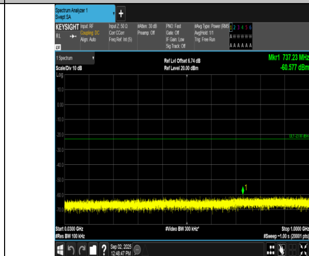
Band2-3MHz-16QAM-18900-1RB#0-30~1000-PASS
