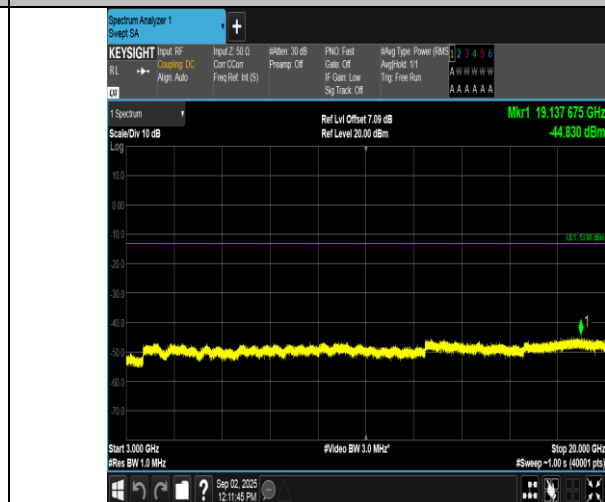
Band2-1.4MHz-16QAM-19193-6RB#0-3000~20000-PASS
