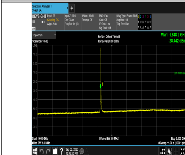
Band2-3MHz-16QAM-18615-15RB#0-1000~3000-PASS
