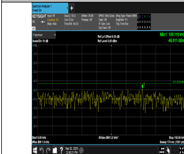
Band2-3MHz-QPSK-18615-15RB#0-0.009~0.15-PASS
