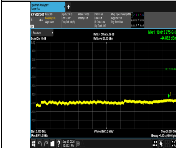
Band2-3MHz-QPSK-18900-15RB#0-3000~20000-PASS
