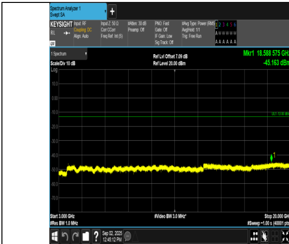
Band2-3MHz-16QAM-18615-1RB#14-3000~20000-PASS
