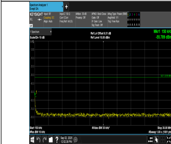
Band2-3MHz-16QAM-18900-15RB#0-0.15~30-PASS
