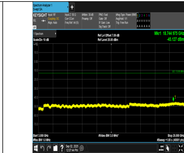
Band2-1.4MHz-16QAM-19193-1RB#0-3000~20000-PASS
