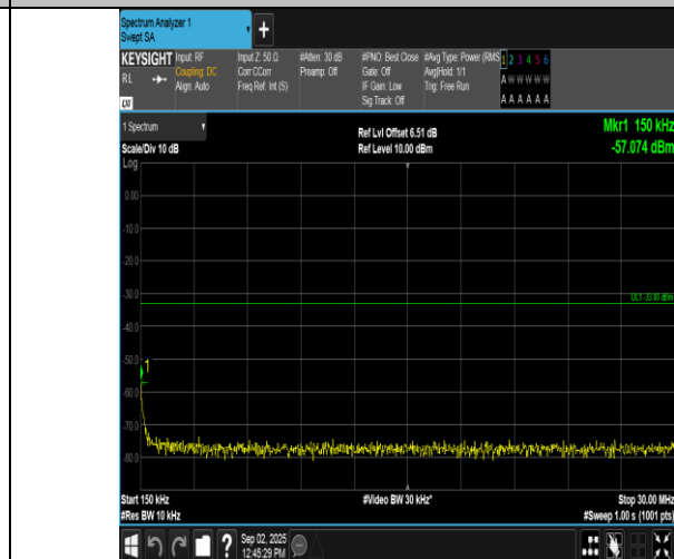
Band2-3MHz-QPSK-18615-15RB#0-0.15~30-PASS
