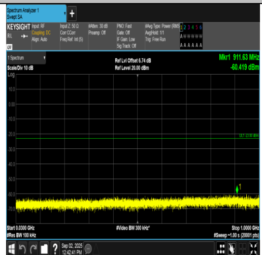
Band2-3MHz-16QAM-18615-1RB#0-30~1000-PASS
