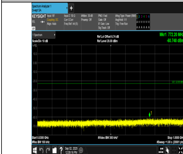
Band2-1.4MHz-16QAM-19193-1RB#5-30~1000-PASS
