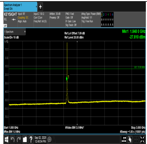
Band2-3MHz-QPSK-18615-15RB#0-1000~3000-PASS
