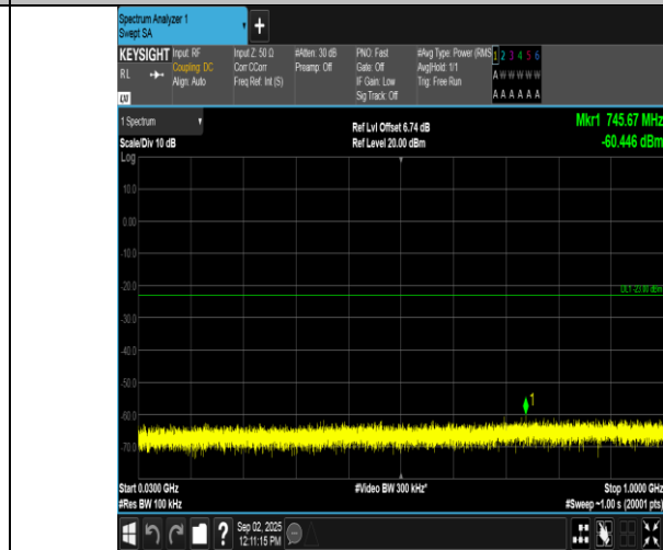
Band2-1.4MHz-16QAM-19193-6RB#0-30~1000-PASS
