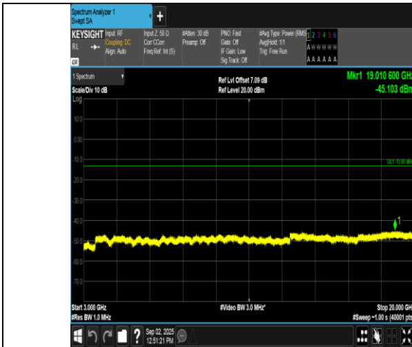
Band2-3MHz-16QAM-18900-1RB#14-3000~20000-PASS
