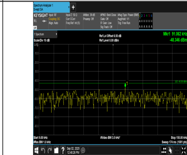
Band2-3MHz-16QAM-18900-1RB#0-0.009~0.15-PASS
