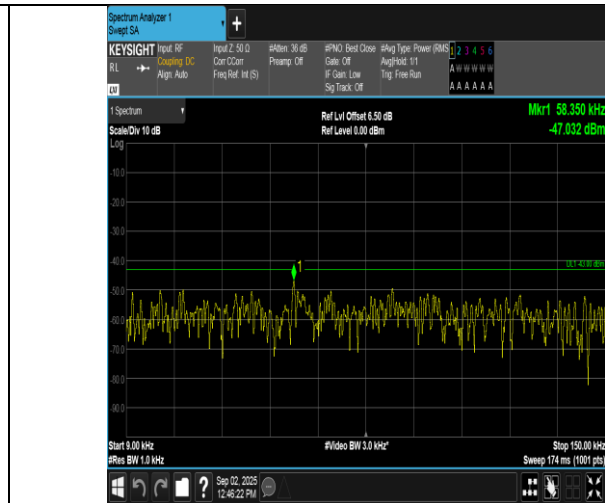
Band2-3MHz-16QAM-18615-15RB#0-0.009~0.15-PASS
