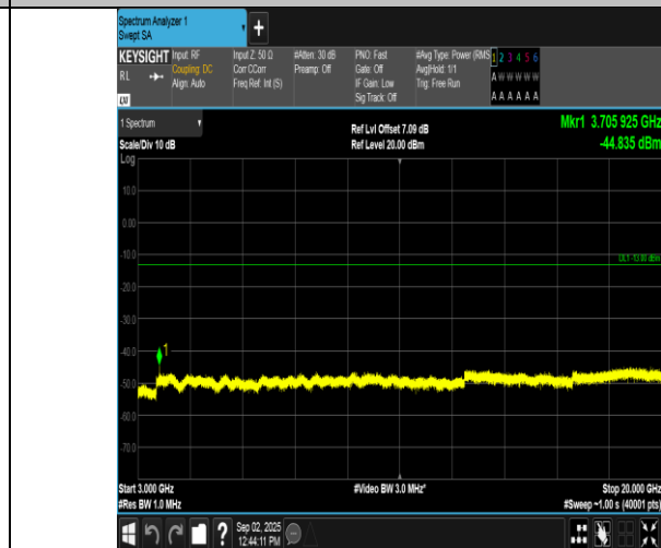
Band2-3MHz-QPSK-18615-1RB#14-3000~20000-PASS
