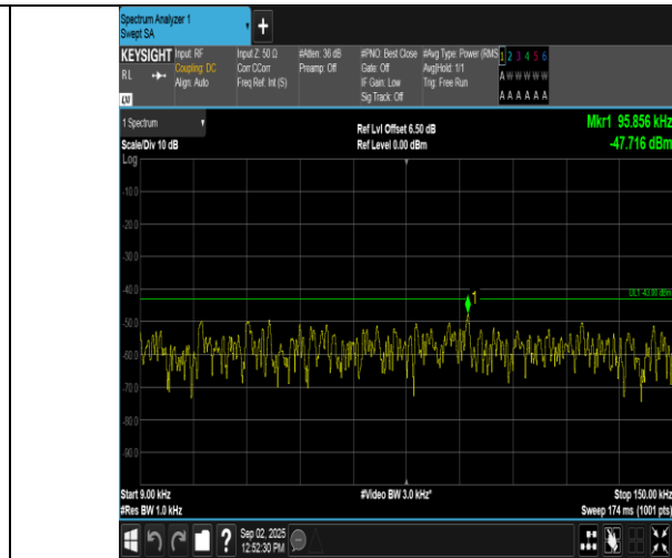
Band2-3MHz-16QAM-18900-15RB#0-0.009~0.15-PASS
