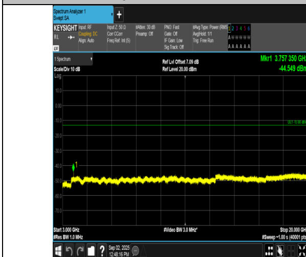
Band2-3MHz-QPSK-18900-1RB#0-3000~20000-PASS
