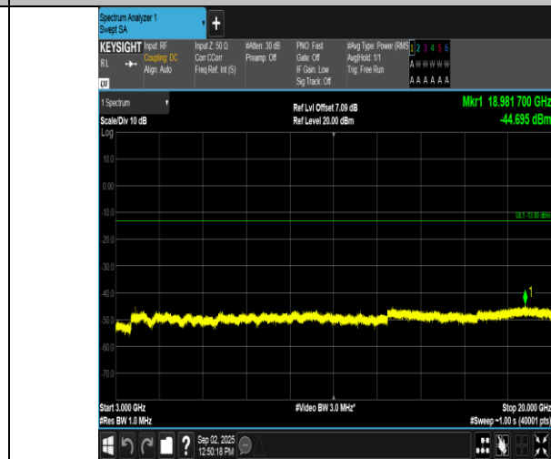
Band2-3MHz-QPSK-18900-1RB#14-3000~20000-PASS
