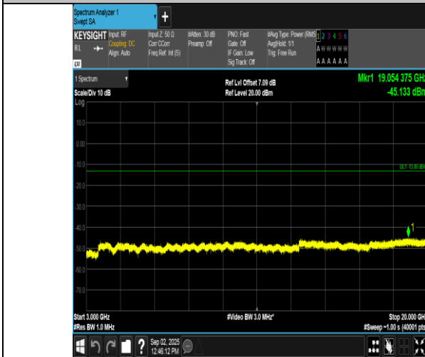
Band2-3MHz-QPSK-18615-15RB#0-3000~20000-PASS
