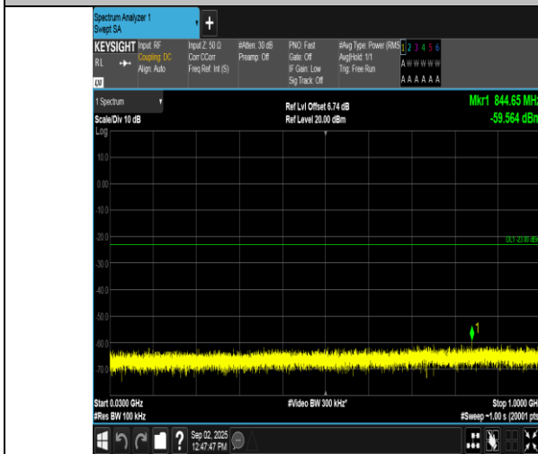
Band2-3MHz-QPSK-18900-1RB#0-30~1000-PASS
