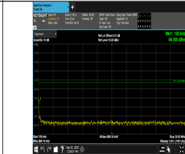
Band2-1.4MHz-16QAM-19193-1RB#5-0.15~30-PASS
