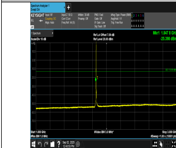
Band2-3MHz-QPSK-18615-1RB#14-1000~3000-PASS
