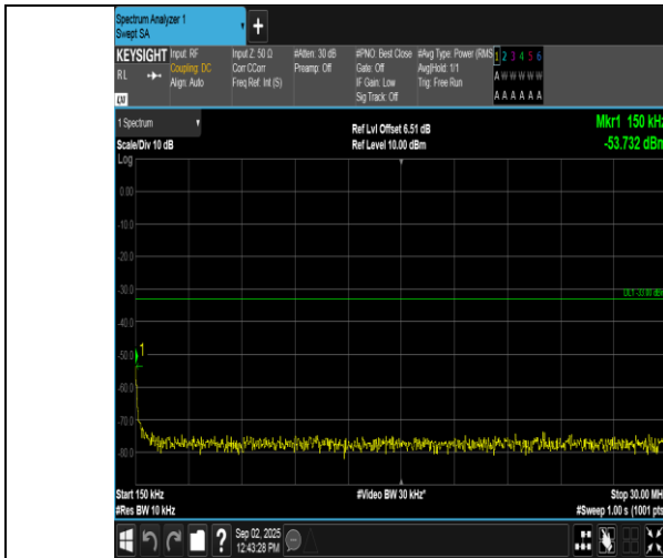
Band2-3MHz-QPSK-18615-1RB#14-0.15~30-PASS
