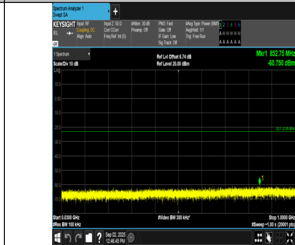
Band2-3MHz-16QAM-18615-15RB#0-30~1000-PASS
