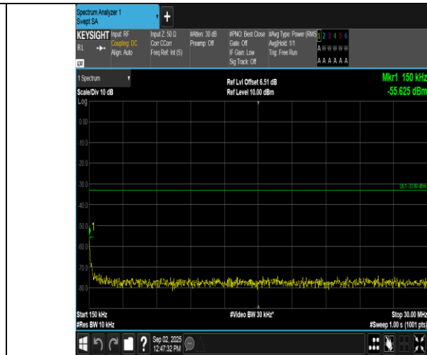
Band2-3MHz-QPSK-18900-1RB#0-0.15~30-PASS
