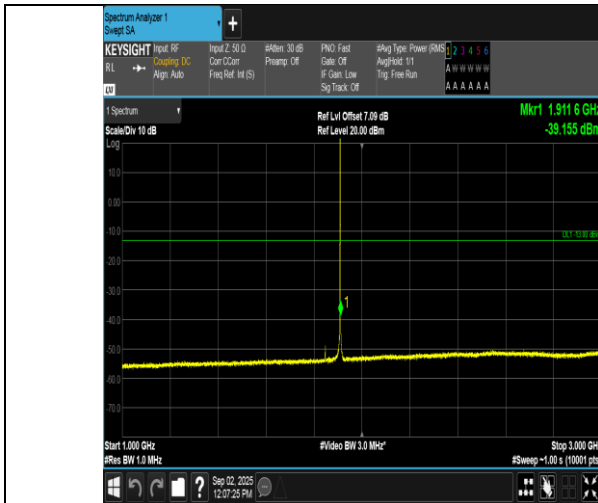
Band2-1.4MHz-16QAM-19193-1RB#0-1000~3000-PASS
