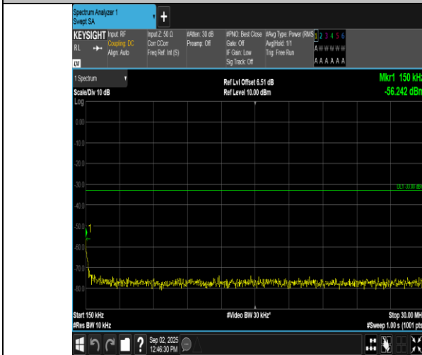
Band2-3MHz-16QAM-18615-15RB#0-0.15~30-PASS
