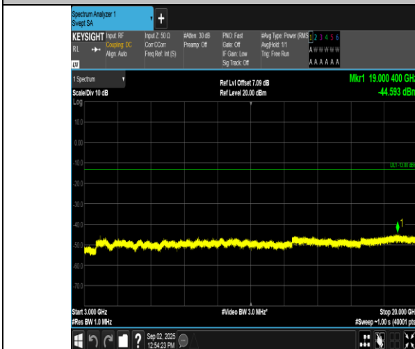
Band2-3MHz-QPSK-19185-1RB#0-3000~20000-PASS
