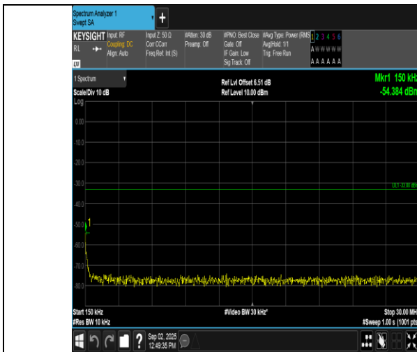
Band2-3MHz-QPSK-18900-1RB#14-0.15~30-PASS
