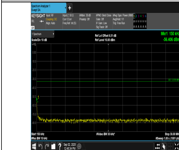
Band2-3MHz-16QAM-18900-1RB#0-0.15~30-PASS
