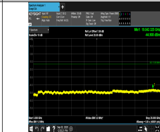
Band2-3MHz-16QAM-18900-15RB#0-3000~20000-PASS
