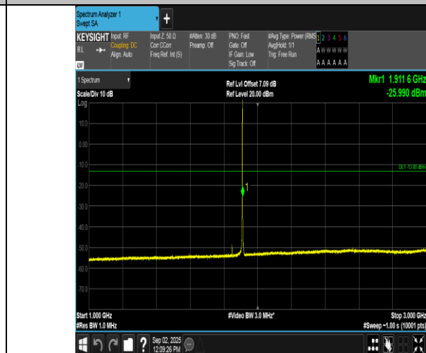
Band2-1.4MHz-16QAM-19193-1RB#5-1000~3000-PASS
