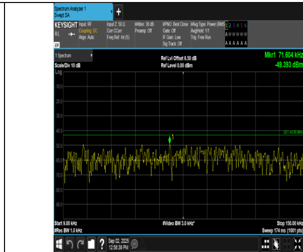
Band2-3MHz-16QAM-19185-15RB#0-0.009~0.15-PASS
