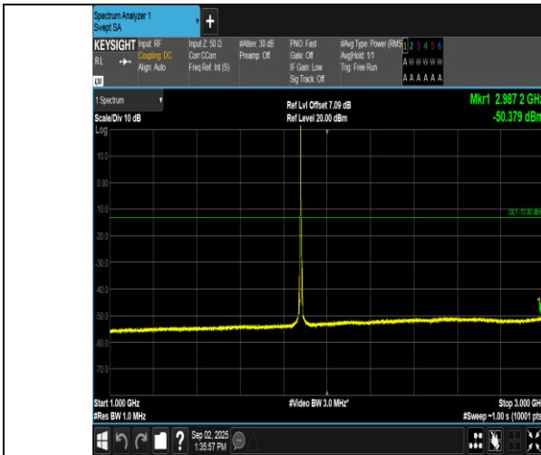
Band2-5MHz-16QAM-18900-1RB#0-1000~3000-PASS
