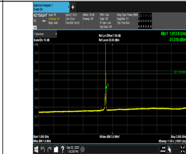
Band2-5MHz-QPSK-19175-1RB#0-1000~3000-PASS
