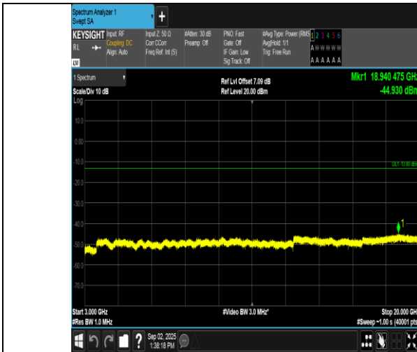
Band2-5MHz-16QAM-18900-1RB#24-3000~20000-PASS
