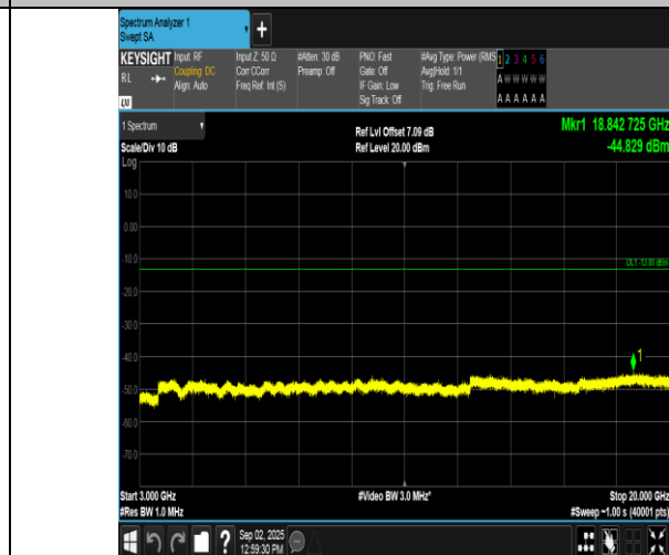
Band2-3MHz-16QAM-19185-15RB#0-3000~20000-PASS
