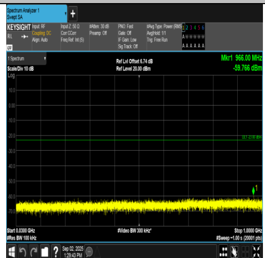
Band2-5MHz-16QAM-18625-1RB#0-30~1000-PASS
