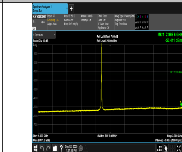
Band2-5MHz-16QAM-18900-1RB#24-1000~3000-PASS
