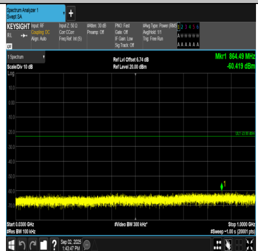
Band2-5MHz-16QAM-19175-1RB#0-30~1000-PASS
