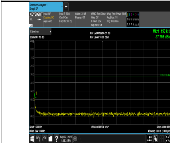
Band2-5MHz-16QAM-18900-25RB#0-0.15~30-PASS
