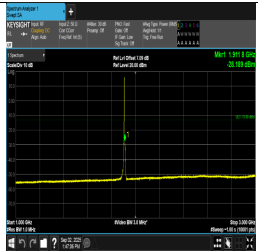
Band2-5MHz-QPSK-19175-25RB#0-1000~3000-PASS
