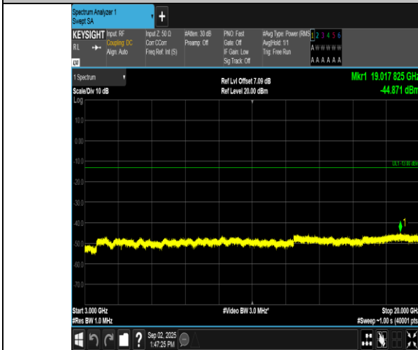
Band2-5MHz-QPSK-19175-25RB#0-3000~20000-PASS
