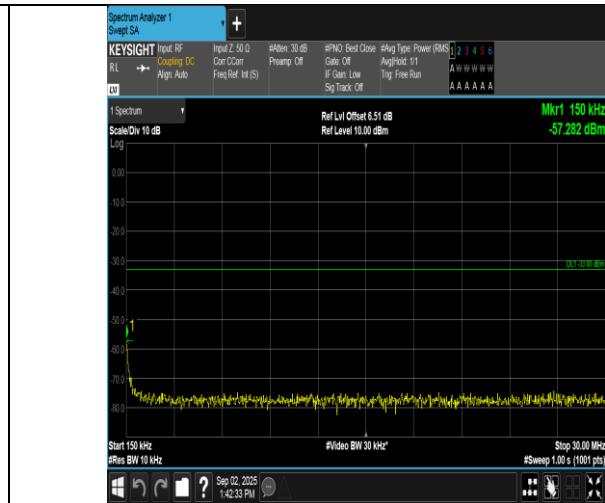
Band2-5MHz-QPSK-19175-1RB#0-0.15~30-PASS
