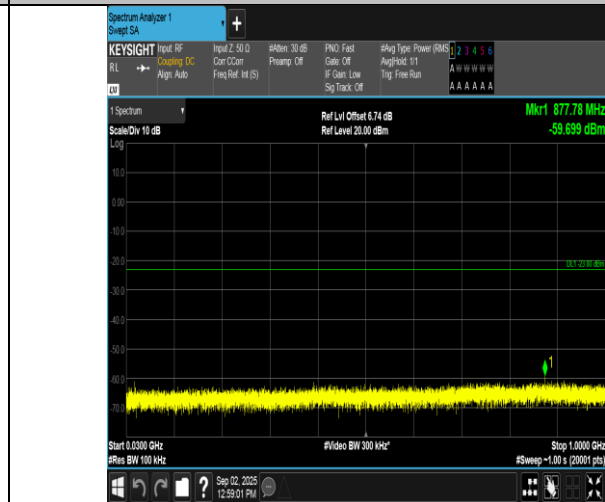
Band2-3MHz-16QAM-19185-15RB#0-30~1000-PASS
