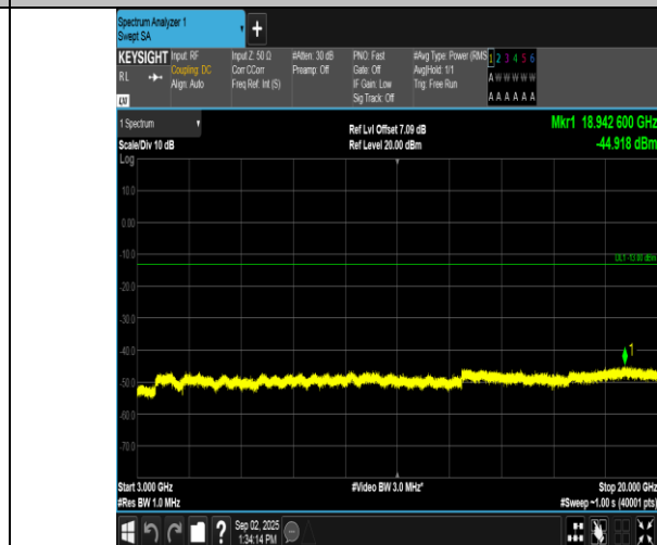
Band2-5MHz-16QAM-18625-25RB#0-3000~20000-PASS
