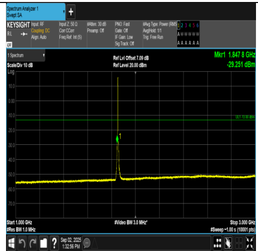
Band2-5MHz-QPSK-18625-25RB#0-1000~3000-PASS
