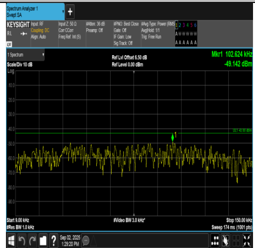
Band2-5MHz-16QAM-18625-1RB#0-0.009~0.15-PASS
