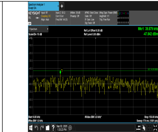
Band2-5MHz-16QAM-18625-25RB#0-0.009~0.15-PASS
