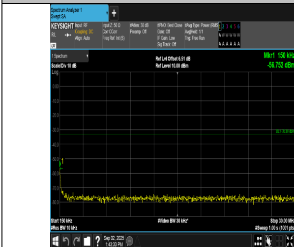
Band2-5MHz-16QAM-19175-1RB#0-0.15~30-PASS
