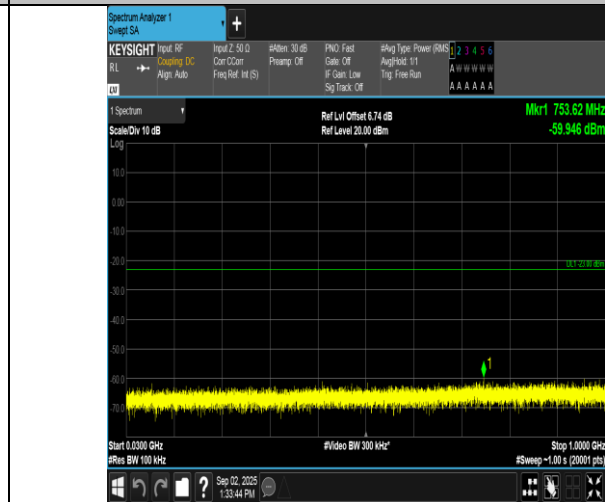
Band2-5MHz-16QAM-18625-25RB#0-30~1000-PASS
