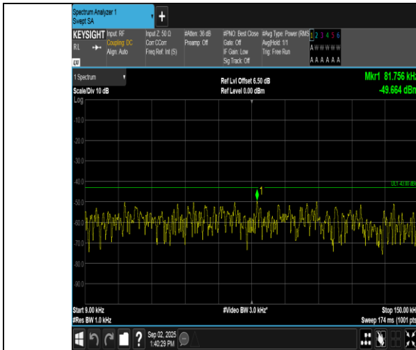
Band2-5MHz-QPSK-19175-1RB#0-0.009~0.15-PASS
