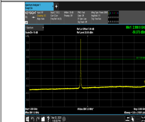
Band2-5MHz-16QAM-18900-25RB#0-1000~3000-PASS
