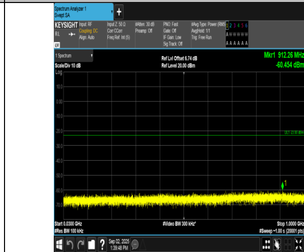
Band2-5MHz-16QAM-18900-25RB#0-30~1000-PASS
