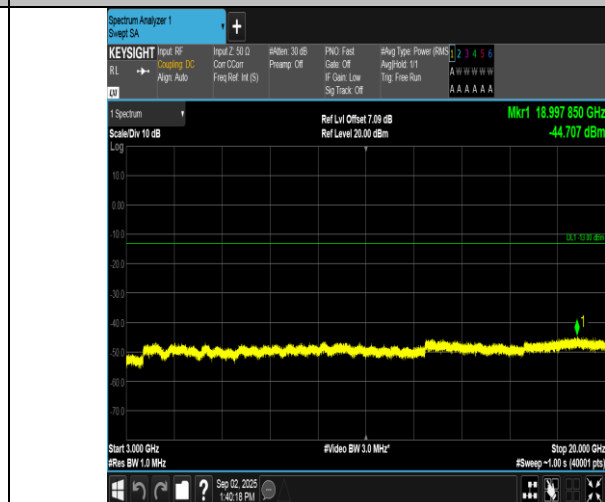
Band2-5MHz-16QAM-18900-25RB#0-3000~20000-PASS
