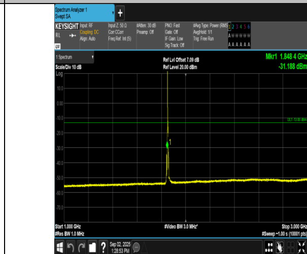
Band2-5MHz-QPSK-18625-1RB#0-1000~3000-PASS
