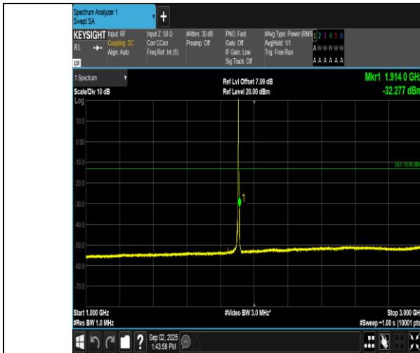
Band2-5MHz-16QAM-19175-1RB#0-1000~3000-PASS
