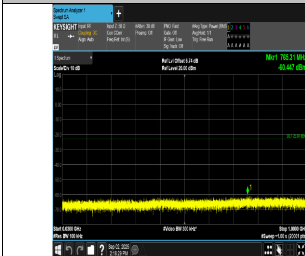
Band2-10MHz-16QAM-18650-1RB#49-30~1000-PASS
