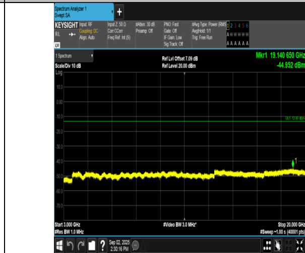
Band2-10MHz-QPSK-19150-1RB#49-3000~20000-PASS
