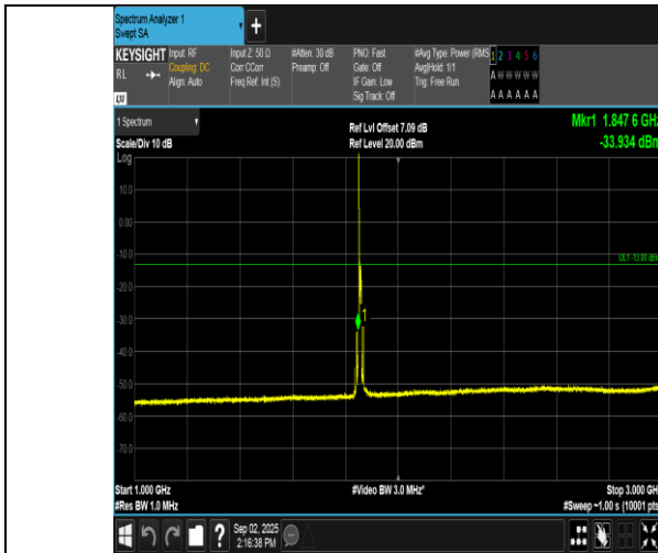
Band2-10MHz-16QAM-18650-1RB#0-1000~3000-PASS
