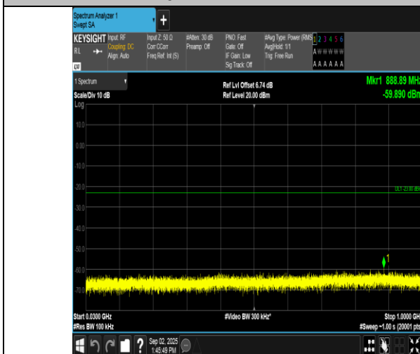
Band2-5MHz-16QAM-19175-1RB#24-30~1000-PASS
