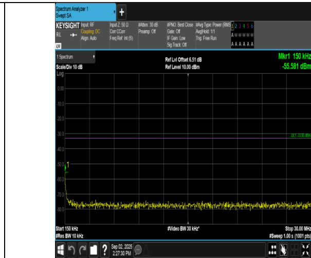
Band2-10MHz-QPSK-19150-1RB#0-0.15~30-PASS
