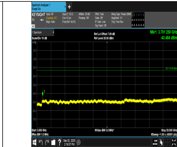
Band2-10MHz-16QAM-18650-1RB#0-3000~20000-PASS
