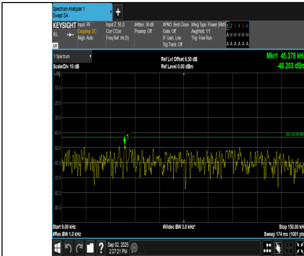
Band2-10MHz-QPSK-19150-1RB#0-0.009~0.15-PASS
