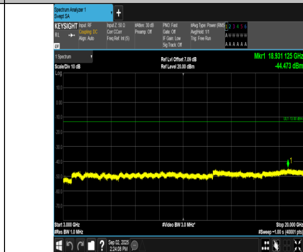
Band2-10MHz-QPSK-18900-1RB#49-3000~20000-PASS
