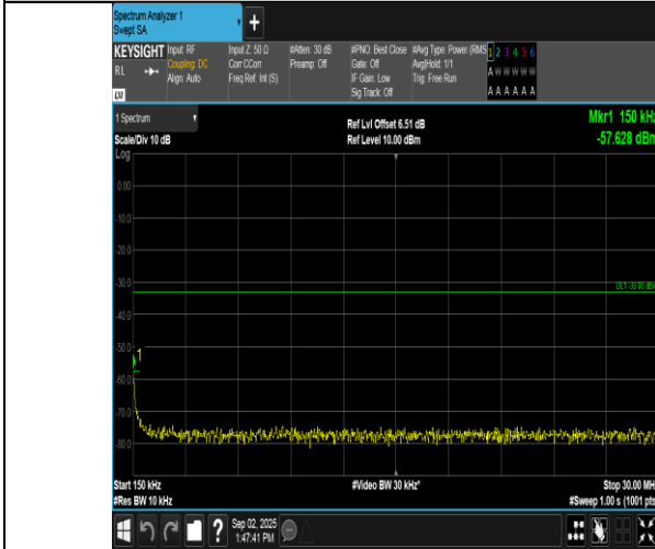
Band2-5MHz-16QAM-19175-25RB#0-0.15~30-PASS
