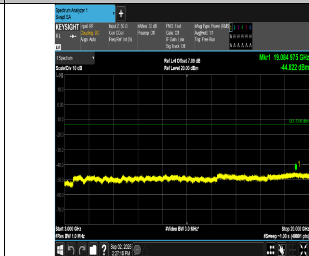
Band2-10MHz-16QAM-18900-50RB#0-3000~20000-PASS
