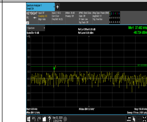
Band2-10MHz-QPSK-19150-1RB#49-0.009~0.15-PASS
