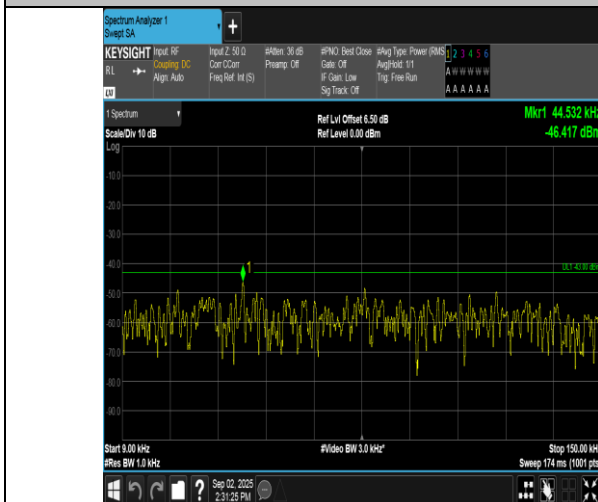
Band2-10MHz-QPSK-19150-50RB#0-0.009~0.15-PASS
