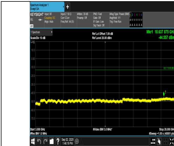
Band2-5MHz-16QAM-19175-1RB#24-3000~20000-PASS
