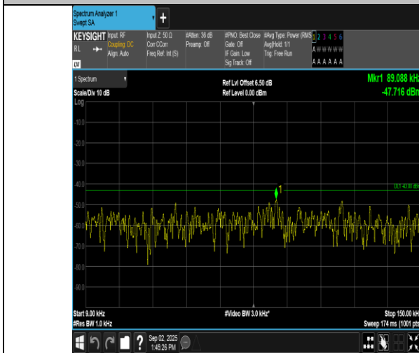
Band2-5MHz-16QAM-19175-1RB#24-0.009~0.15-PASS
