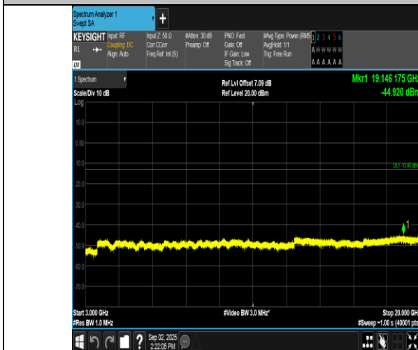
Band2-10MHz-QPSK-18900-1RB#0-3000~20000-PASS
