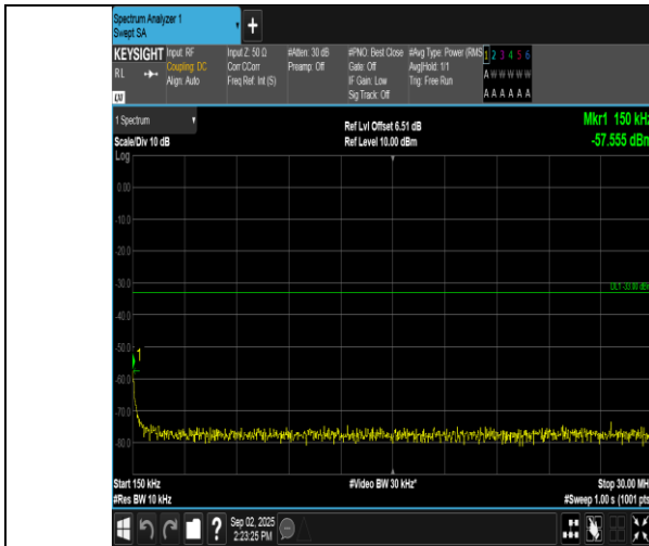
Band2-10MHz-QPSK-18900-1RB#49-0.15~30-PASS
