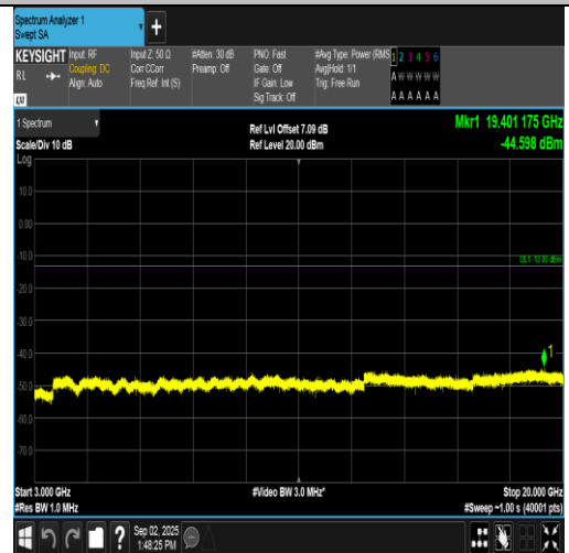
Band2-5MHz-16QAM-19175-25RB#0-3000~20000-PASS
