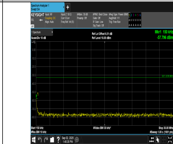
Band2-5MHz-16QAM-19175-1RB#24-0.15~30-PASS
