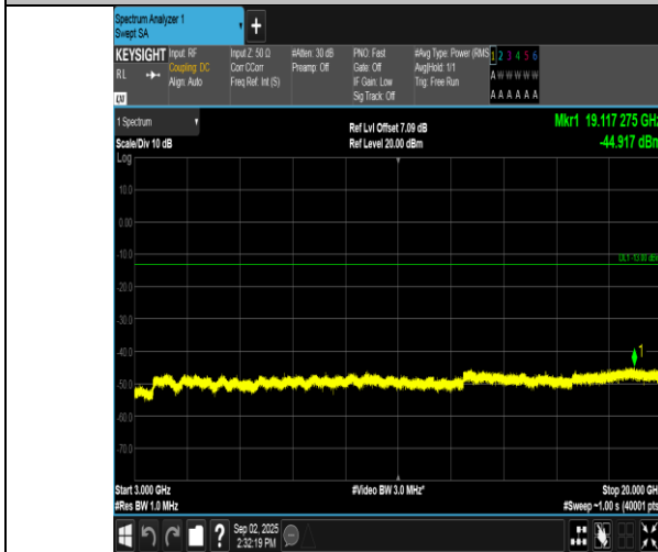
Band2-10MHz-QPSK-19150-50RB#0-3000~20000-PASS
