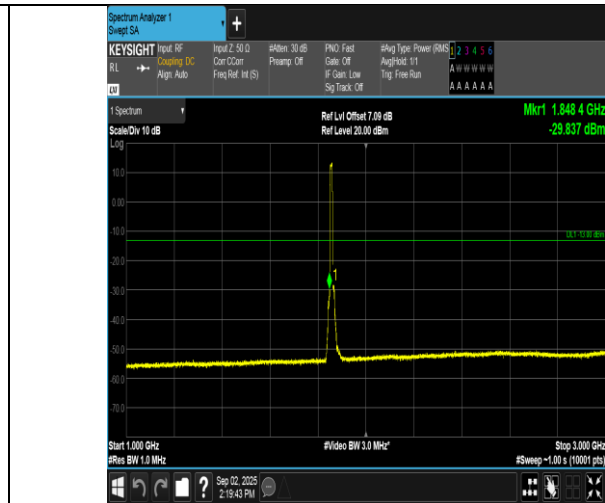
Band2-10MHz-QPSK-18650-50RB#0-1000~3000-PASS
