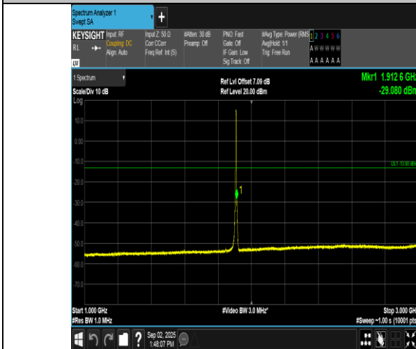
Band2-5MHz-16QAM-19175-25RB#0-1000~3000-PASS
