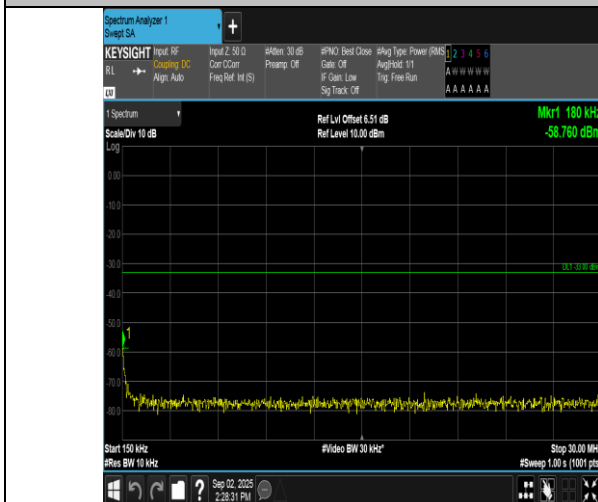
Band2-10MHz-16QAM-19150-1RB#0-0.15~30-PASS
