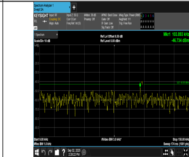
Band2-10MHz-16QAM-19150-1RB#0-0.009~0.15-PASS
