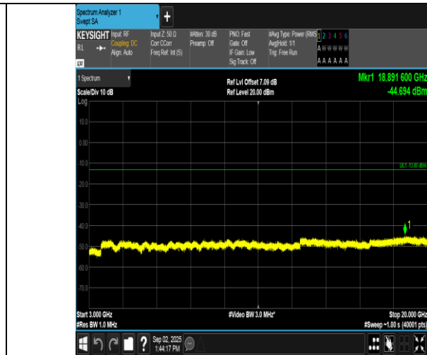
Band2-5MHz-16QAM-19175-1RB#0-3000~20000-PASS
