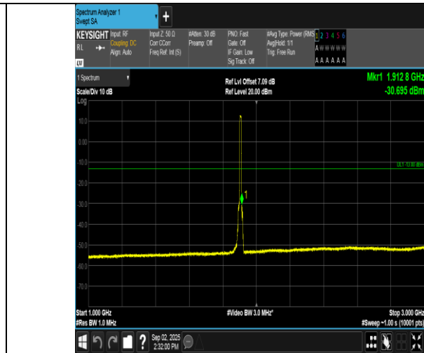
Band2-10MHz-QPSK-19150-50RB#0-1000~3000-PASS
