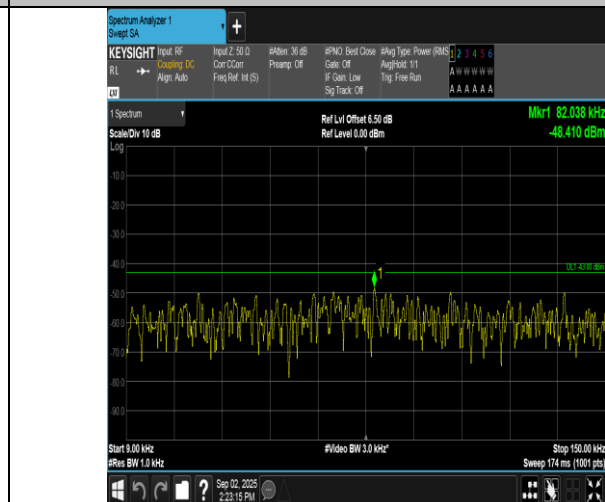
Band2-10MHz-QPSK-18900-1RB#49-0.009~0.15-PASS
