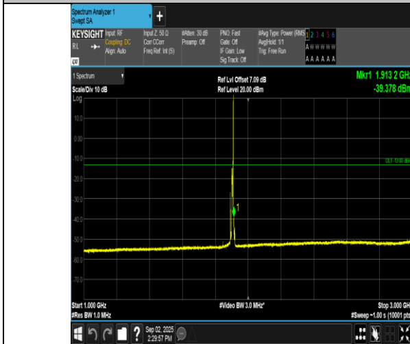
Band2-10MHz-QPSK-19150-1RB#49-1000~3000-PASS
