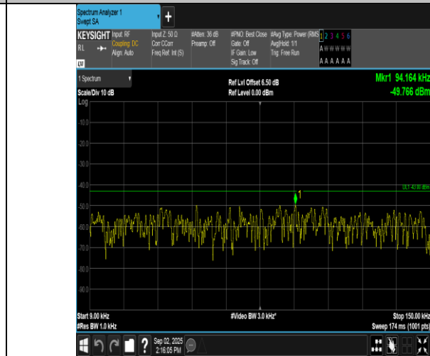
Band2-10MHz-16QAM-18650-1RB#0-0.009~0.15-PASS
