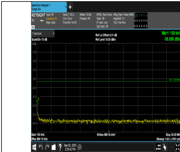
Band2-10MHz-QPSK-19150-1RB#49-0.15~30-PASS
