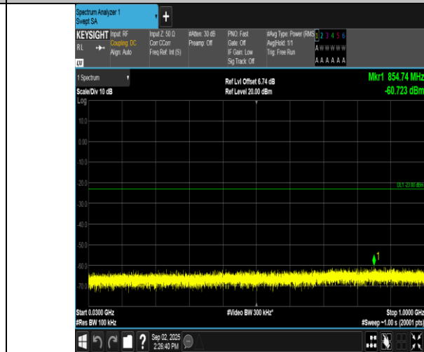
Band2-10MHz-16QAM-18900-50RB#0-30~1000-PASS
