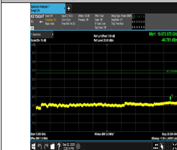
Band2-10MHz-QPSK-19150-1RB#0-3000~20000-PASS
