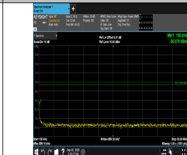
Band2-10MHz-QPSK-18900-50RB#0-0.15~30-PASS
