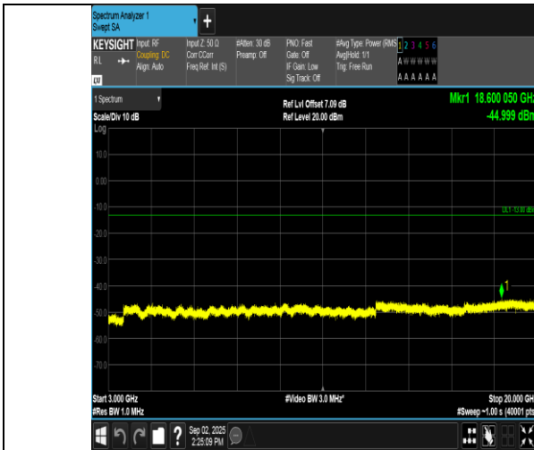
Band2-10MHz-16QAM-18900-1RB#49-3000~20000-PASS
