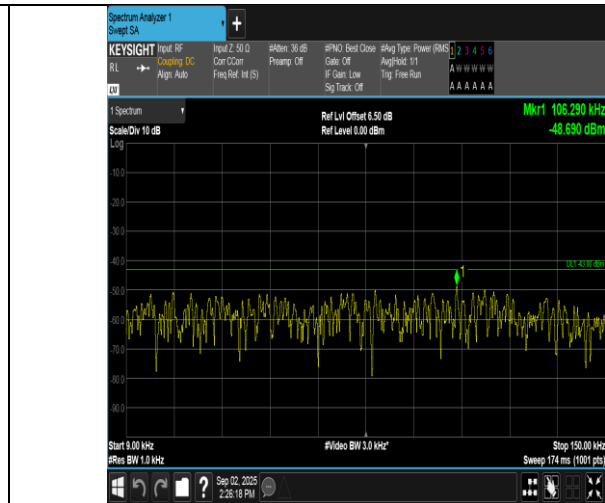
Band2-10MHz-16QAM-18900-50RB#0-0.009~0.15-PASS
