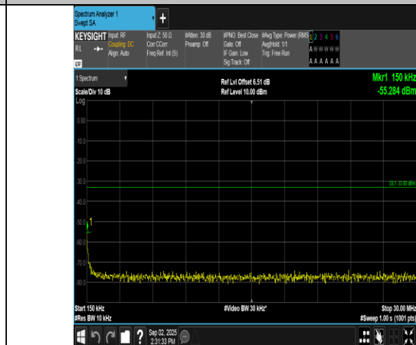
Band2-10MHz-QPSK-19150-50RB#0-0.15~30-PASS
