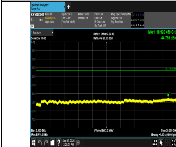
Band2-10MHz-QPSK-18650-50RB#0-3000~20000-PASS
