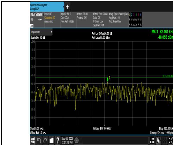
Band2-10MHz-QPSK-18900-1RB#0-0.009~0.15-PASS
