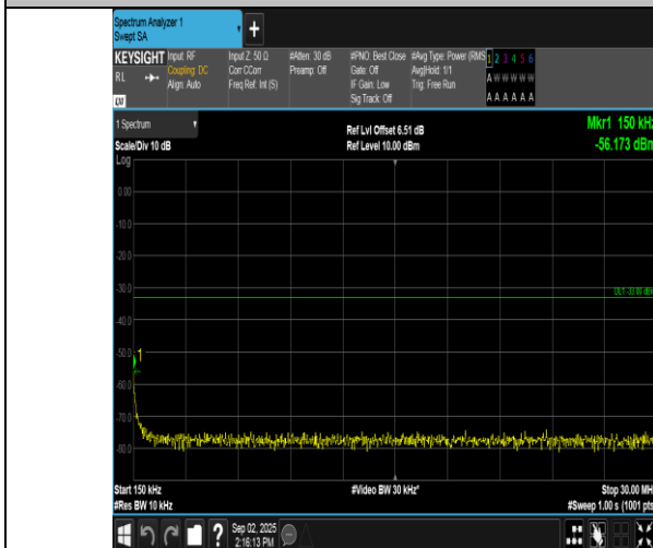
Band2-10MHz-16QAM-18650-1RB#0-0.15~30-PASS
