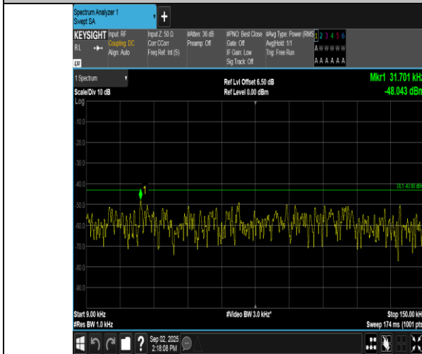
Band2-10MHz-16QAM-18650-1RB#49-0.009~0.15-PASS
