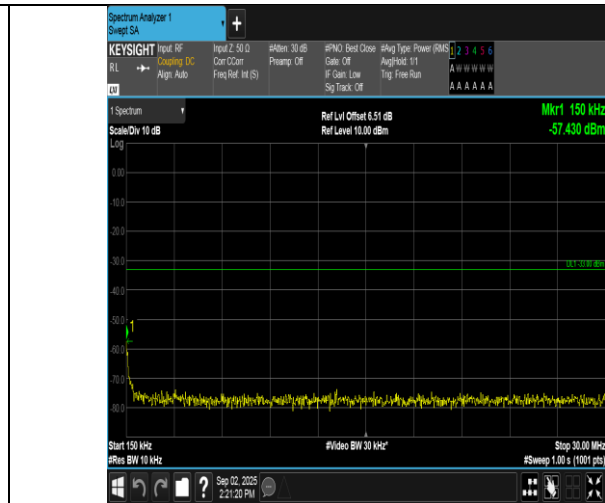
Band2-10MHz-QPSK-18900-1RB#0-0.15~30-PASS
