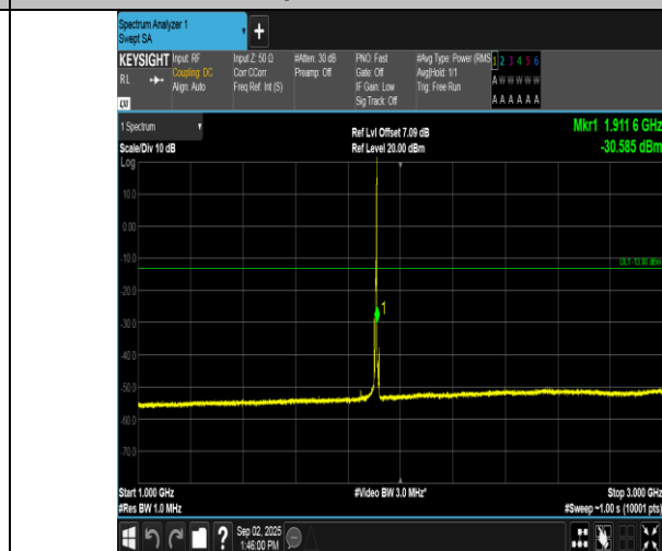
Band2-5MHz-16QAM-19175-1RB#24-1000~3000-PASS
