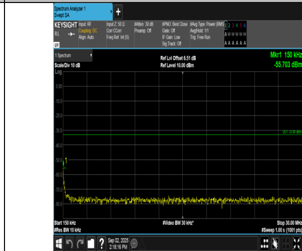
Band2-10MHz-16QAM-18650-1RB#49-0.15~30-PASS
