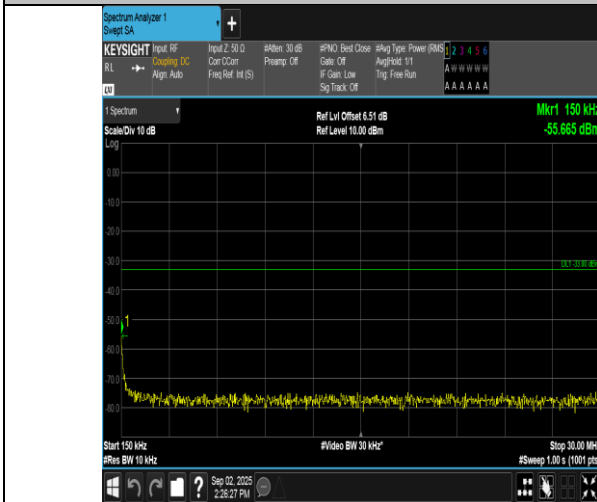
Band2-10MHz-16QAM-18900-50RB#0-0.15~30-PASS
