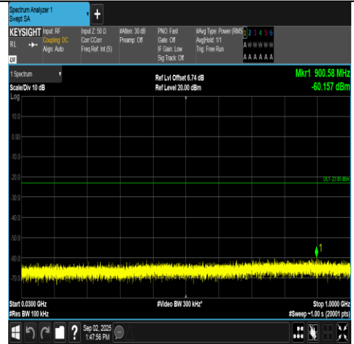
Band2-5MHz-16QAM-19175-25RB#0-30~1000-PASS
