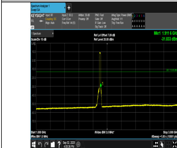
Band2-20MHz-16QAM-19100-100RB#0-1000~3000-PASS
