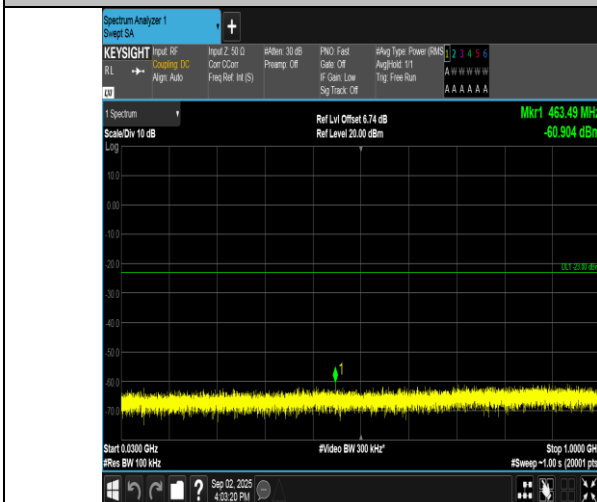
Band2-20MHz-16QAM-19100-1RB#99-30~1000-PASS
