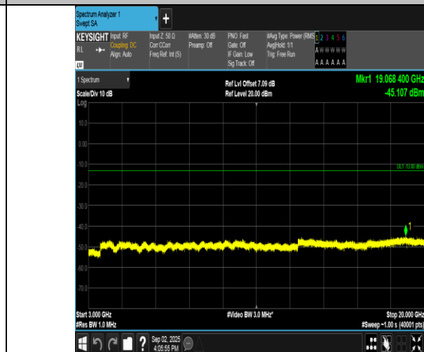
Band2-20MHz-16QAM-19100-100RB#0-3000~20000-PASS
