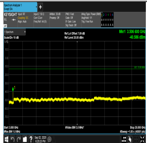
Band4-5MHz-16QAM-20375-25RB#0-3000~20000-PASS
