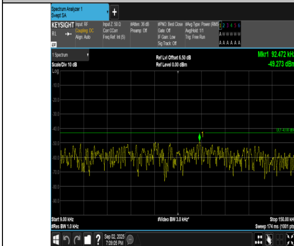
Band4-10MHz-QPSK-20350-50RB#0-0.009~0.15-PASS
