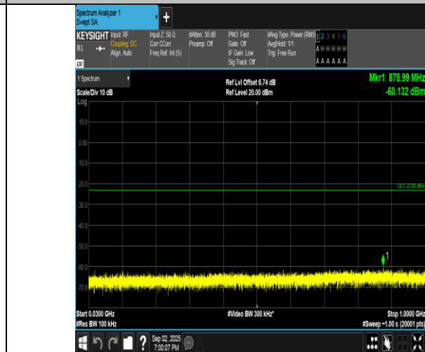
Band4-10MHz-16QAM-20175-1RB#0-30~1000-PASS
