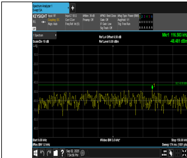
Band4-10MHz-QPSK-20350-1RB#0-0.009~0.15-PASS
