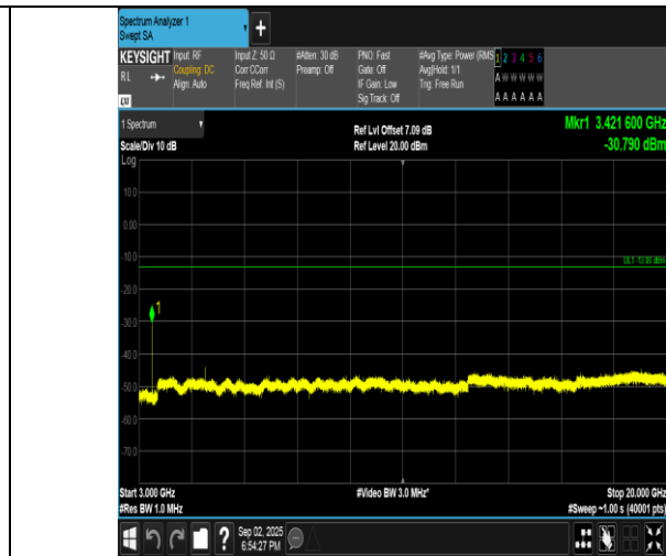
Band4-10MHz-16QAM-20000-1RB#0-3000~20000-PASS
