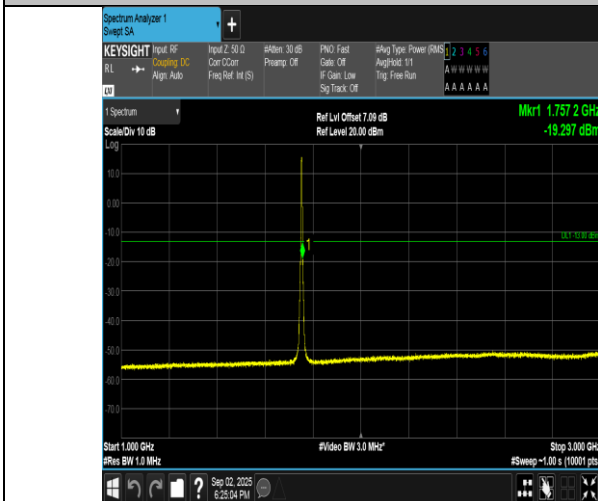
Band4-5MHz-16QAM-20375-25RB#0-1000~3000-PASS
