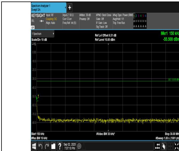
Band4-10MHz-QPSK-20350-1RB#49-0.15~30-PASS
