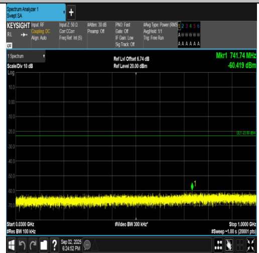
Band4-5MHz-16QAM-20375-25RB#0-30~1000-PASS
