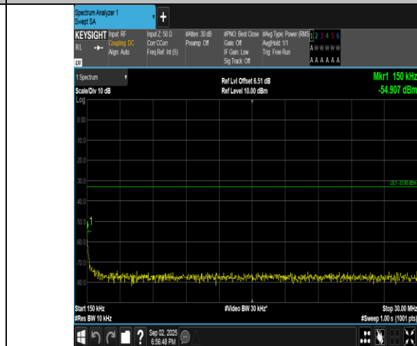
Band4-10MHz-QPSK-20000-50RB#0-0.15~30-PASS
