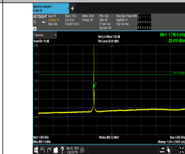
Band4-5MHz-16QAM-20375-1RB#24-1000~3000-PASS
