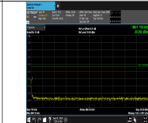
Band4-10MHz-QPSK-20350-50RB#0-0.15~30-PASS
