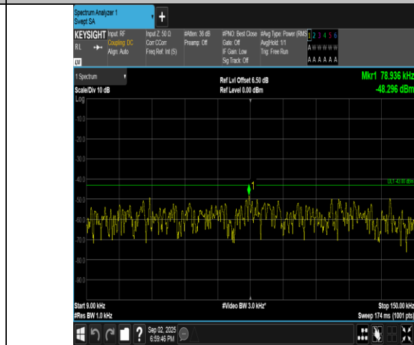
Band4-10MHz-16QAM-20175-1RB#0-0.009~0.15-PASS
