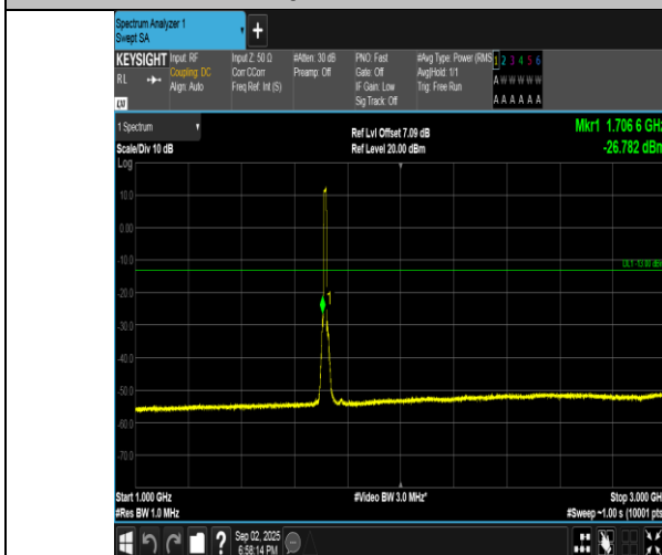
Band4-10MHz-16QAM-20000-50RB#0-1000~3000-PASS
