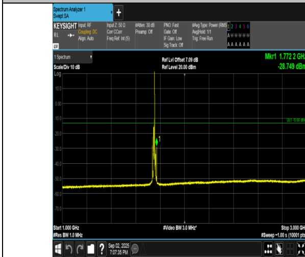
Band4-10MHz-QPSK-20350-1RB#49-1000~3000-PASS
