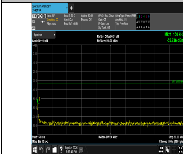
Band4-10MHz-16QAM-20000-50RB#0-0.15~30-PASS
