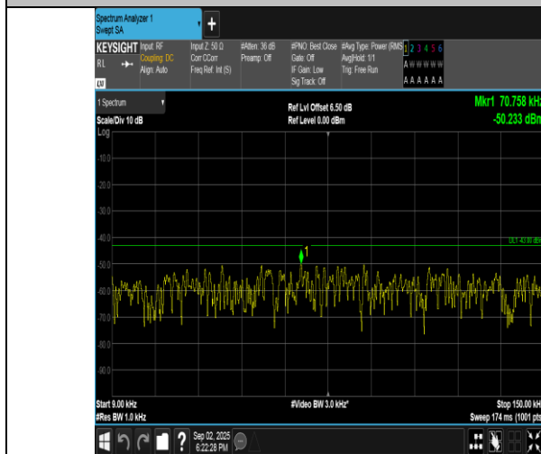
Band4-5MHz-16QAM-20375-1RB#24-0.009~0.15-PASS
