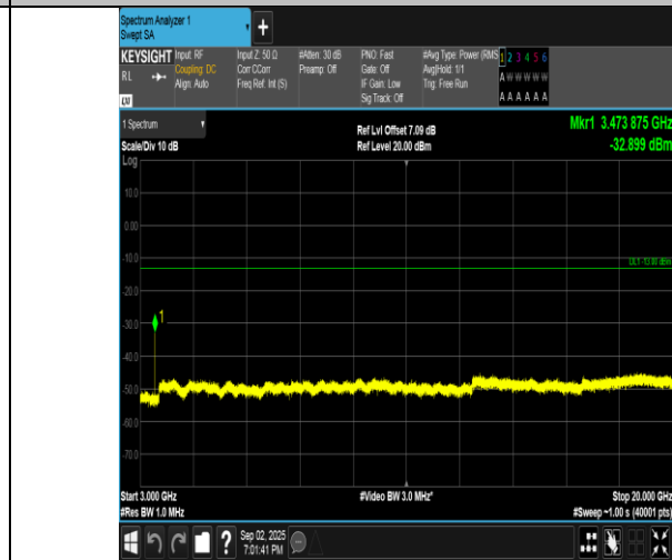
Band4-10MHz-QPSK-20175-1RB#49-3000~20000-PASS
