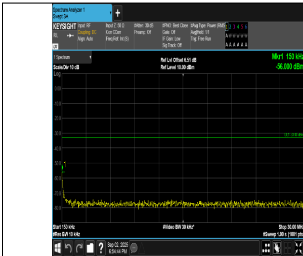
Band4-10MHz-QPSK-20000-1RB#49-0.15~30-PASS
