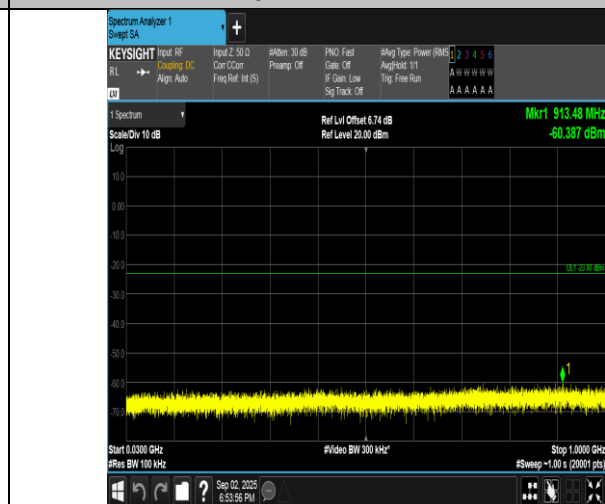
Band4-10MHz-16QAM-20000-1RB#0-30~1000-PASS
