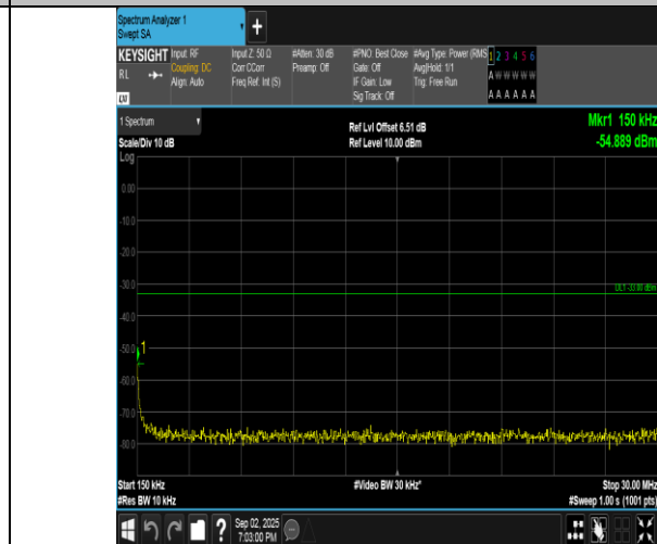
Band4-10MHz-QPSK-20175-50RB#0-0.15~30-PASS
