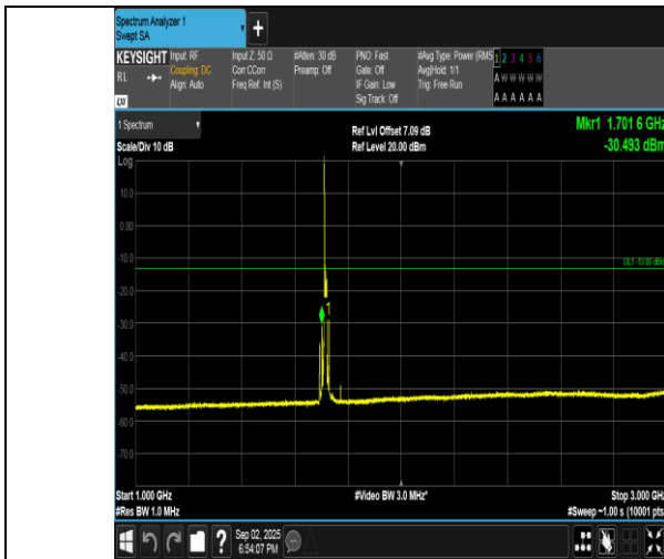
Band4-10MHz-16QAM-20000-1RB#0-1000~3000-PASS
