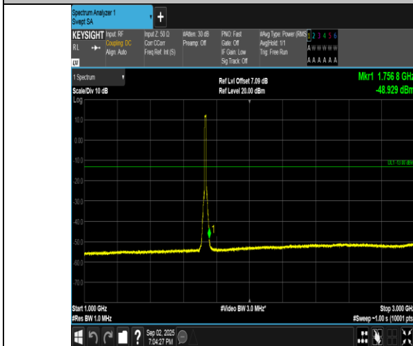
Band4-10MHz-16QAM-20175-50RB#0-1000~3000-PASS
