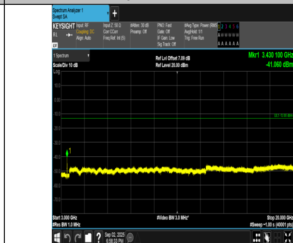
Band4-10MHz-16QAM-20000-50RB#0-3000~20000-PASS
