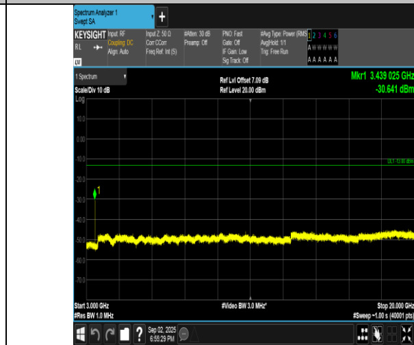
Band4-10MHz-QPSK-20000-1RB#49-3000~20000-PASS
