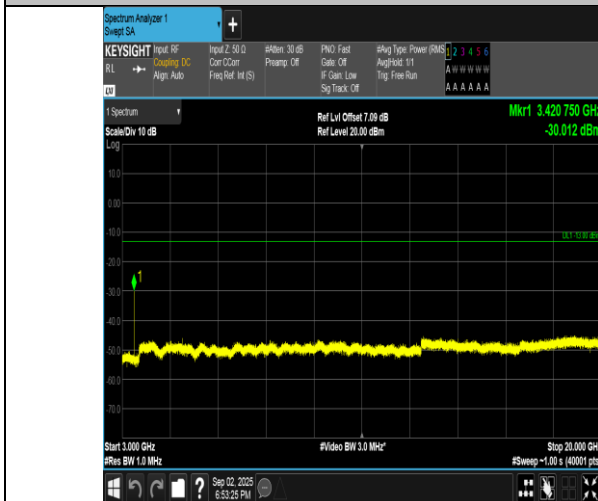
Band4-10MHz-QPSK-20000-1RB#0-3000~20000-PASS
