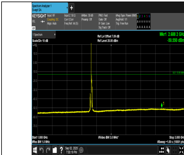
Band4-10MHz-16QAM-20175-1RB#0-1000~3000-PASS
