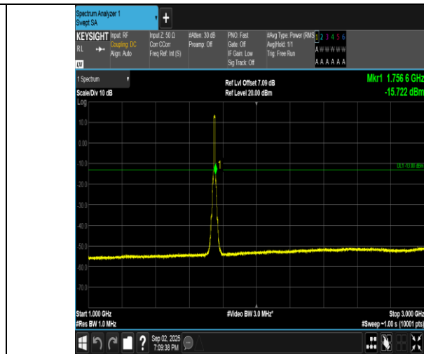
Band4-10MHz-QPSK-20350-50RB#0-1000~3000-PASS
