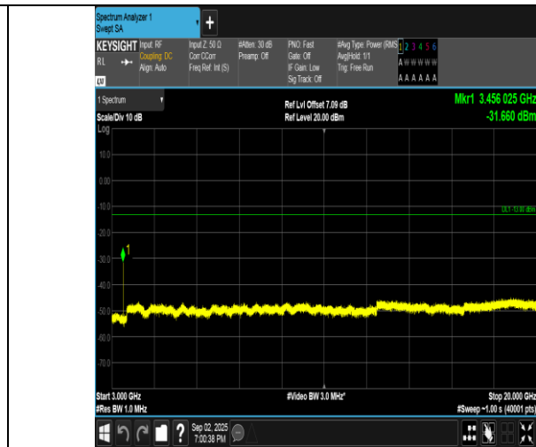
Band4-10MHz-16QAM-20175-1RB#0-3000~20000-PASS
