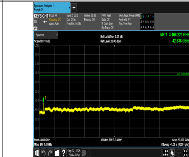
Band4-10MHz-16QAM-20175-50RB#0-3000~20000-PASS
