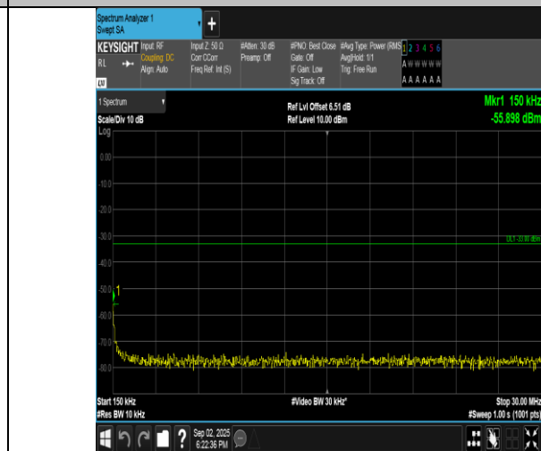
Band4-5MHz-16QAM-20375-1RB#24-0.15~30-PASS
