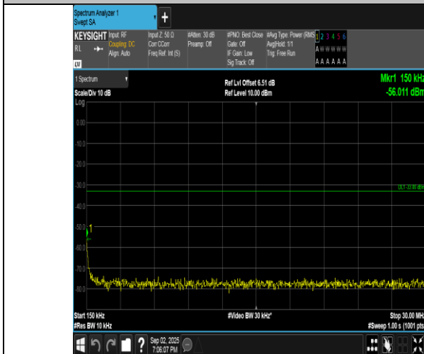
Band4-10MHz-16QAM-20350-1RB#0-0.15~30-PASS
