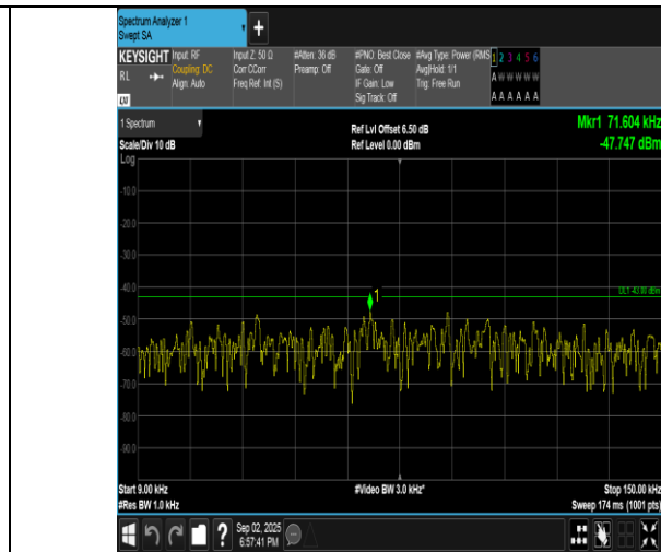
Band4-10MHz-16QAM-20000-50RB#0-0.009~0.15-PASS
