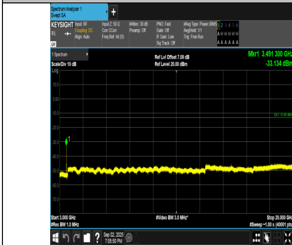
Band4-10MHz-QPSK-20350-1RB#0-3000~20000-PASS
