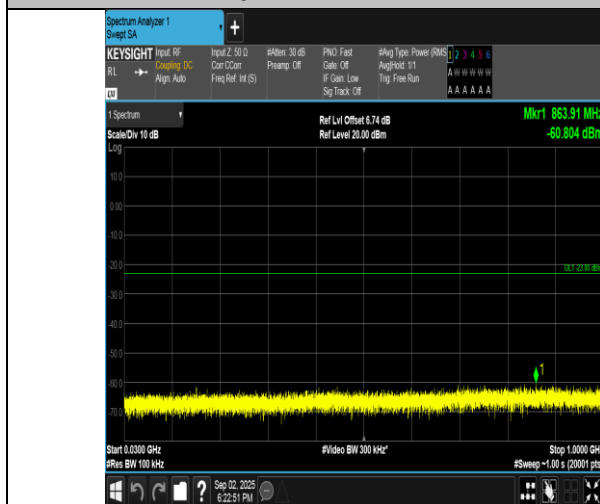
Band4-5MHz-16QAM-20375-1RB#24-30~1000-PASS
