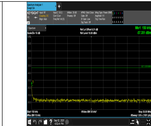
Band4-10MHz-QPSK-20000-1RB#0-0.15~30-PASS
