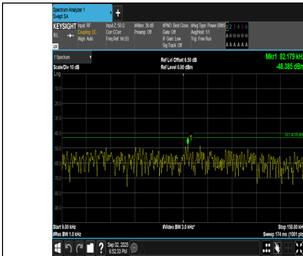
Band4-10MHz-QPSK-20000-1RB#0-0.009~0.15-PASS
