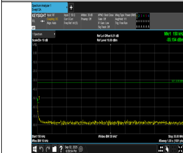
Band4-10MHz-16QAM-20175-1RB#0-0.15~30-PASS
