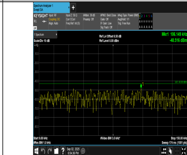
Band4-10MHz-QPSK-20000-1RB#49-0.009~0.15-PASS
