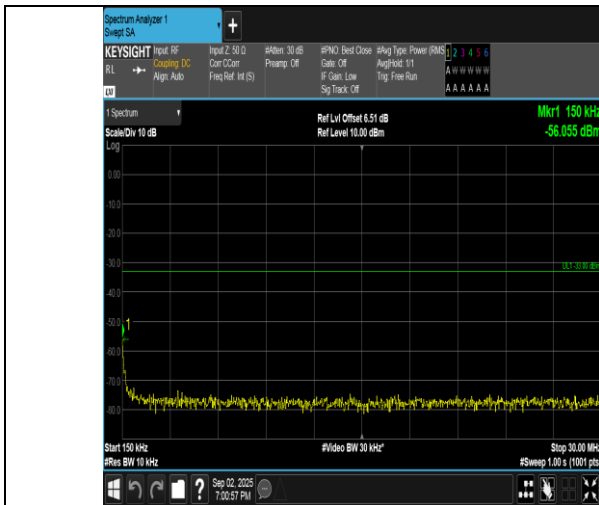
Band4-10MHz-QPSK-20175-1RB#49-0.15~30-PASS
