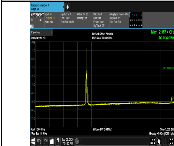
Band4-10MHz-QPSK-20175-1RB#49-1000~3000-PASS
