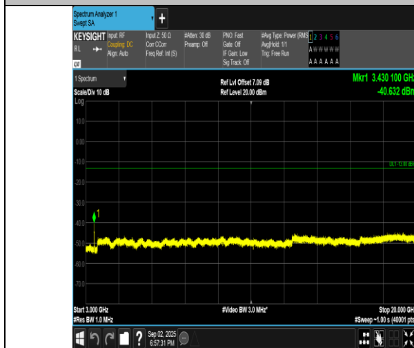
Band4-10MHz-QPSK-20000-50RB#0-3000~20000-PASS
