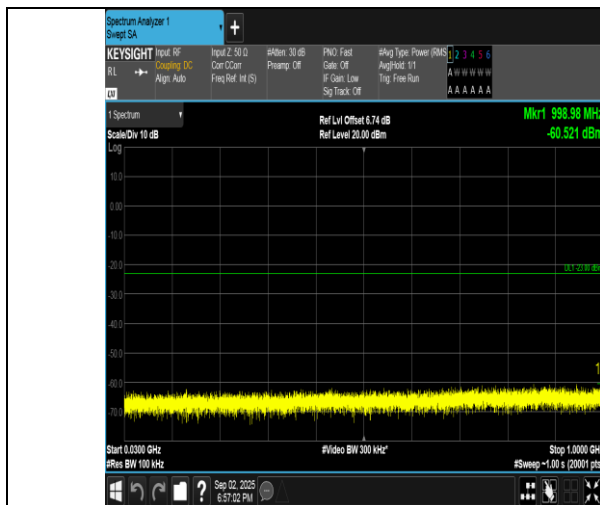
Band4-10MHz-QPSK-20000-50RB#0-30~1000-PASS
