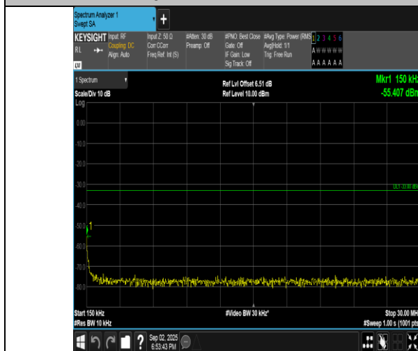
Band4-10MHz-16QAM-20000-1RB#0-0.15~30-PASS
