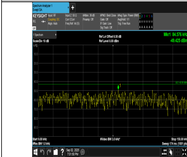
Band4-10MHz-16QAM-20175-1RB#49-0.009~0.15-PASS
