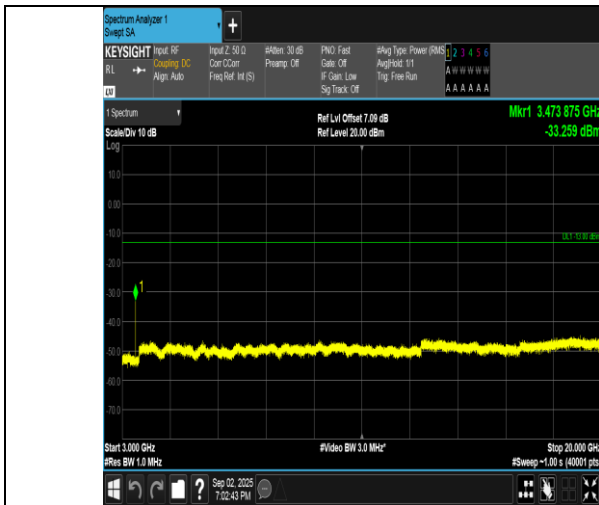
Band4-10MHz-16QAM-20175-1RB#49-3000~20000-PASS
