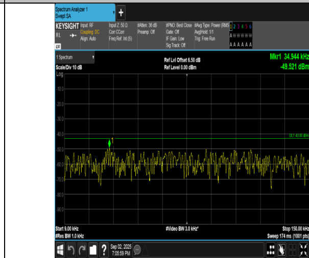
Band4-10MHz-16QAM-20350-1RB#0-0.009~0.15-PASS
