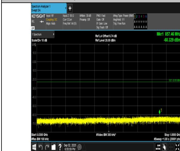
Band4-10MHz-16QAM-20000-1RB#49-30~1000-PASS
