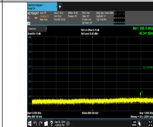
Band4-10MHz-16QAM-20000-50RB#0-30~1000-PASS
