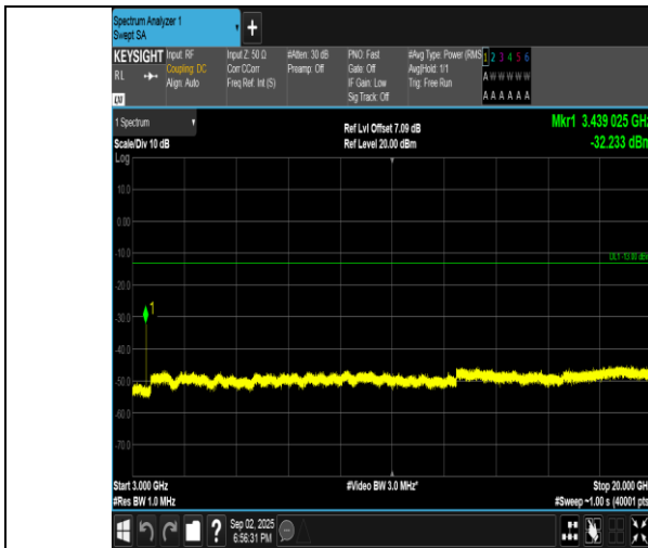
Band4-10MHz-16QAM-20000-1RB#49-3000~20000-PASS
