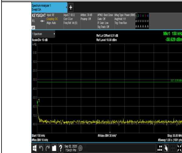
Band4-10MHz-16QAM-20175-50RB#0-0.15~30-PASS
