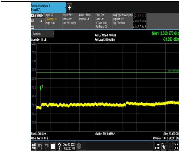
Band4-5MHz-16QAM-20375-1RB#24-3000~20000-PASS
