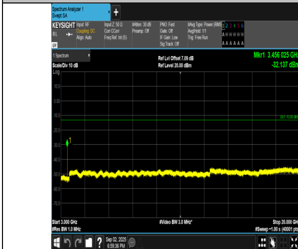
Band4-10MHz-QPSK-20175-1RB#0-3000~20000-PASS
