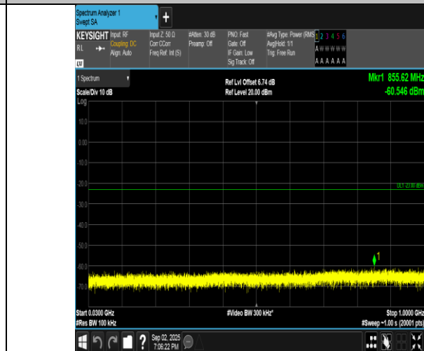
Band4-10MHz-16QAM-20350-1RB#0-30~1000-PASS
