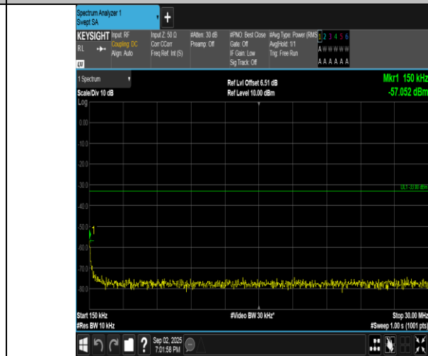
Band4-10MHz-16QAM-20175-1RB#49-0.15~30-PASS
