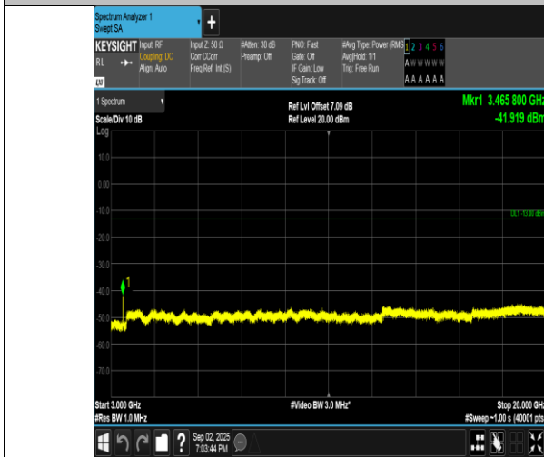
Band4-10MHz-QPSK-20175-50RB#0-3000~20000-PASS
