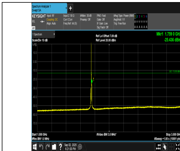
Band4-5MHz-16QAM-20375-1RB#0-1000~3000-PASS
