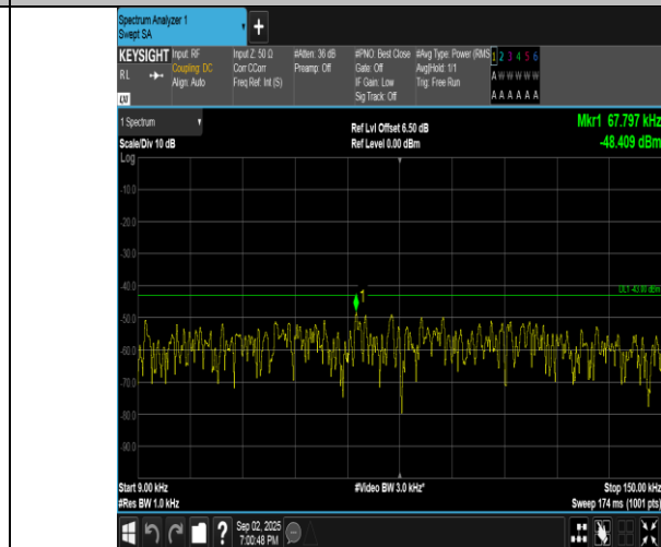
Band4-10MHz-QPSK-20175-1RB#49-0.009~0.15-PASS
