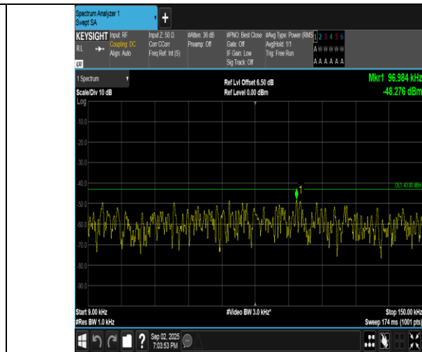
Band4-10MHz-16QAM-20175-50RB#0-0.009~0.15-PASS
