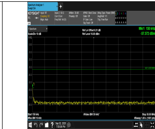
Band4-10MHz-QPSK-20350-1RB#0-0.15~30-PASS
