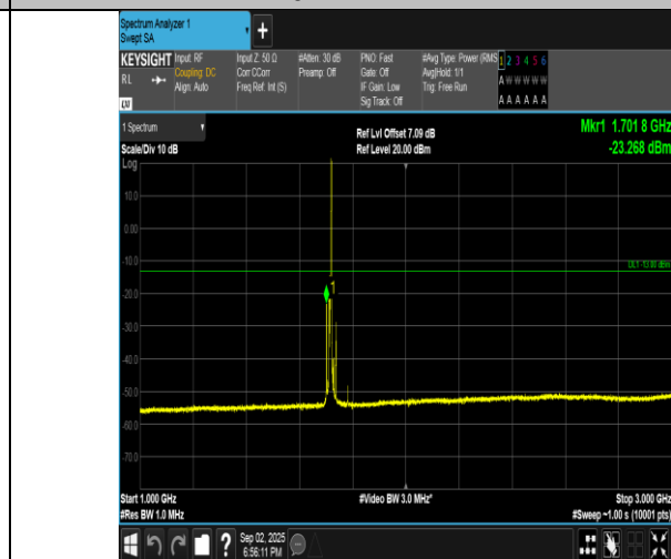
Band4-10MHz-16QAM-20000-1RB#49-1000~3000-PASS
