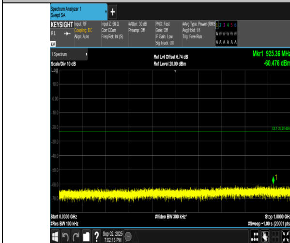
Band4-10MHz-16QAM-20175-1RB#49-30~1000-PASS
