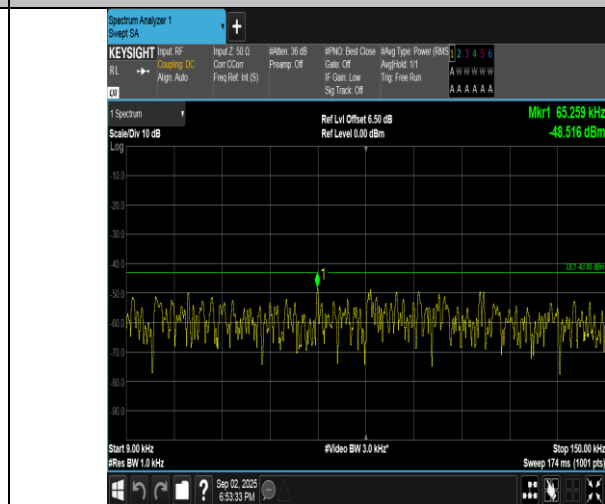
Band4-10MHz-16QAM-20000-1RB#0-0.009~0.15-PASS
