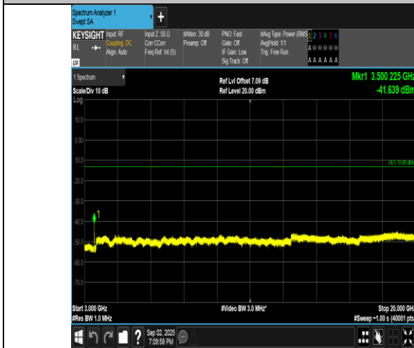
Band4-10MHz-QPSK-20350-50RB#0-3000~20000-PASS
