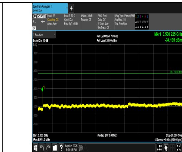
Band4-5MHz-16QAM-20375-1RB#0-3000~20000-PASS
