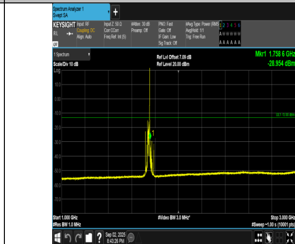
Band4-20MHz-16QAM-20300-1RB#99-1000~3000-PASS
