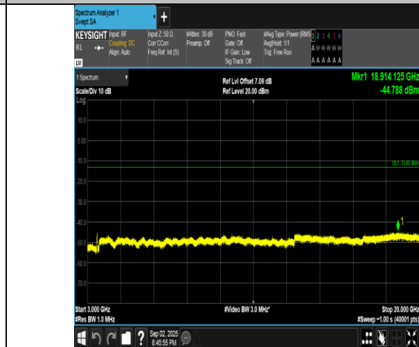
Band4-20MHz-16QAM-20300-100RB#0-3000~20000-PASS
