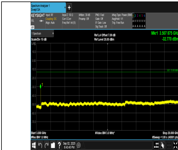
Band4-20MHz-16QAM-20300-1RB#99-3000~20000-PASS
