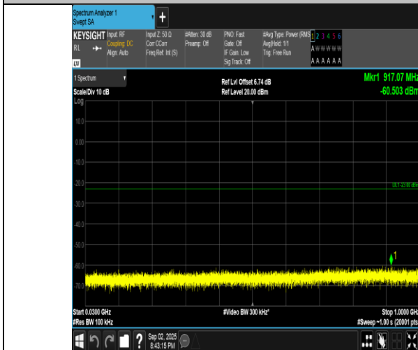
Band4-20MHz-16QAM-20300-1RB#99-30~1000-PASS
