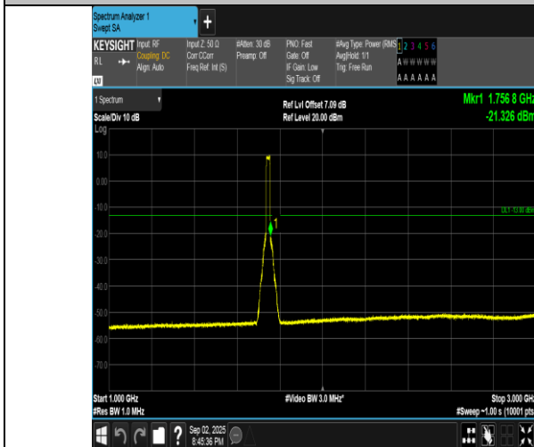
Band4-20MHz-16QAM-20300-100RB#0-1000~3000-PASS
