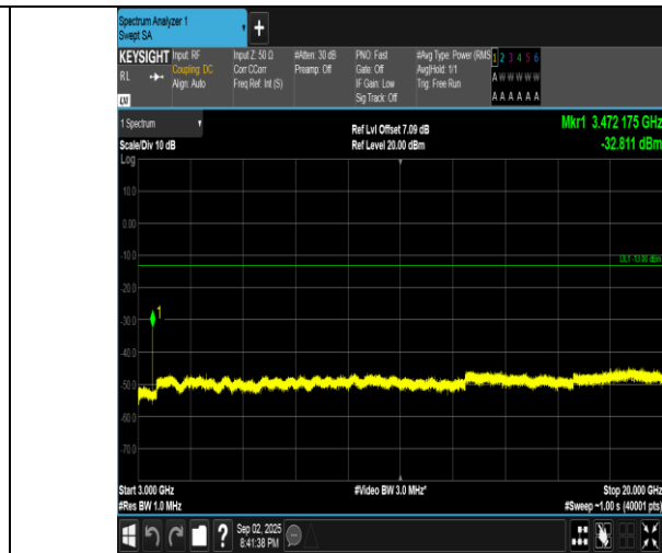
Band4-20MHz-16QAM-20300-1RB#0-3000~20000-PASS
