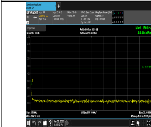
Band4-20MHz-16QAM-20300-100RB#0-0.15~30-PASS
