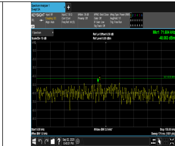
Band4-20MHz-16QAM-20300-100RB#0-0.009~0.15-PASS
