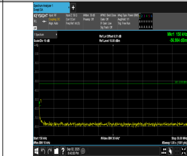
Band4-20MHz-16QAM-20300-1RB#99-0.15~30-PASS
