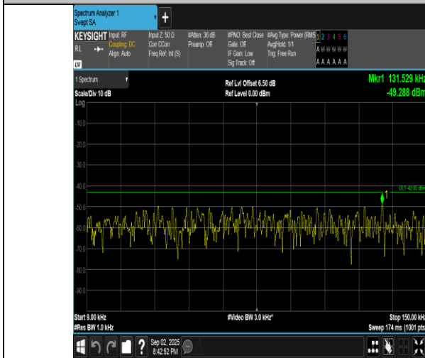
Band4-20MHz-16QAM-20300-1RB#99-0.009~0.15-PASS
