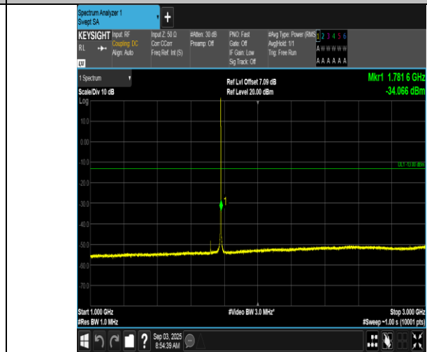
Band66-1.4MHz-QPSK-132665-1RB#0-1000~3000-PASS
