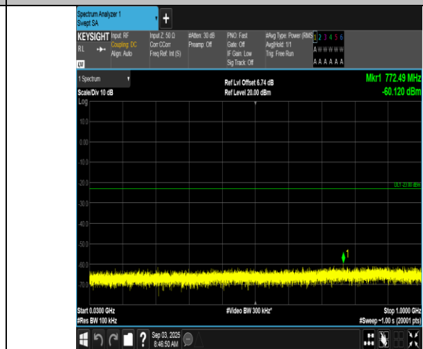
Band66-1.4MHz-16QAM-131979-6RB#0-30~1000-PASS
