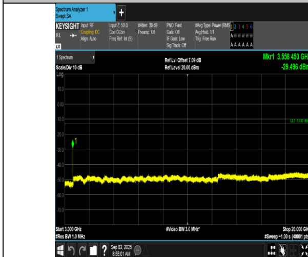
Band66-1.4MHz-QPSK-132665-1RB#0-3000~20000-PASS
