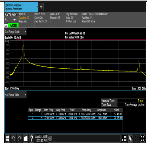
Band66-20MHz-16QAM-132072-1RB#0-PASS
