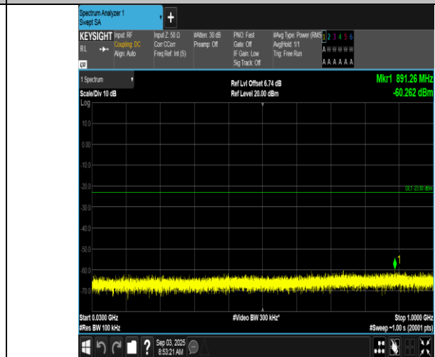
Band66-1.4MHz-16QAM-132322-6RB#0-30~1000-PASS
