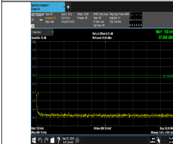
Band66-1.4MHz-16QAM-131979-1RB#0-0.15~30-PASS
