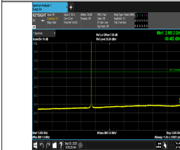
Band66-1.4MHz-QPSK-132322-1RB#5-1000~3000-PASS
