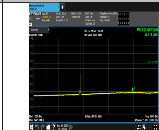
Band66-1.4MHz-16QAM-132322-1RB#5-1000~3000-PASS
