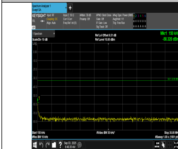
Band66-1.4MHz-16QAM-131979-6RB#0-0.15~30-PASS
