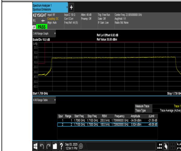
Band66-20MHz-QPSK-132072-100RB#0-PASS
