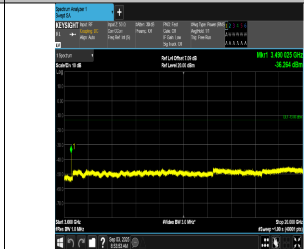
Band66-1.4MHz-16QAM-132322-6RB#0-3000~20000-PASS
