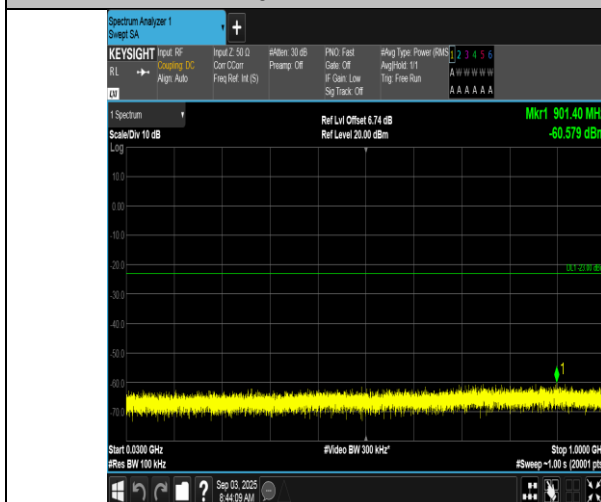
Band66-1.4MHz-16QAM-131979-1RB#5-30~1000-PASS
