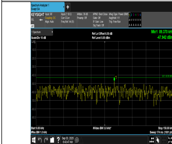
Band66-1.4MHz-16QAM-131979-1RB#5-0.009~0.15-PASS
