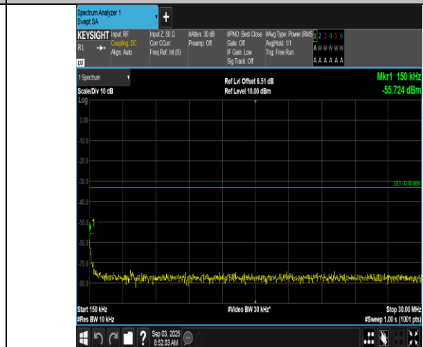
Band66-1.4MHz-QPSK-132322-6RB#0-0.15~30-PASS
