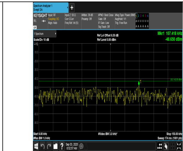
Band66-1.4MHz-16QAM-132322-6RB#0-0.009~0.15-PASS
