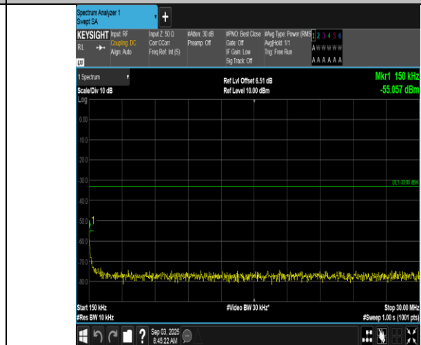
Band66-1.4MHz-QPSK-131979-6RB#0-0.15~30-PASS
