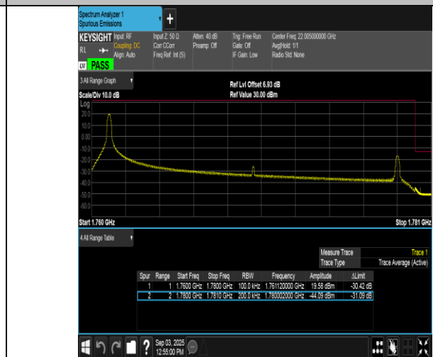
Band66-20MHz-16QAM-132572-1RB#0-PASS
