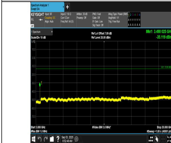
Band66-1.4MHz-QPSK-132322-6RB#0-3000~20000-PASS
