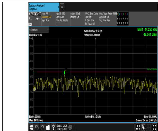
Band66-1.4MHz-16QAM-131979-6RB#0-0.009~0.15-PASS
