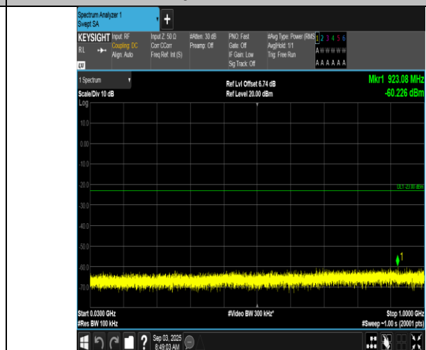
Band66-1.4MHz-16QAM-132322-1RB#0-30~1000-PASS
