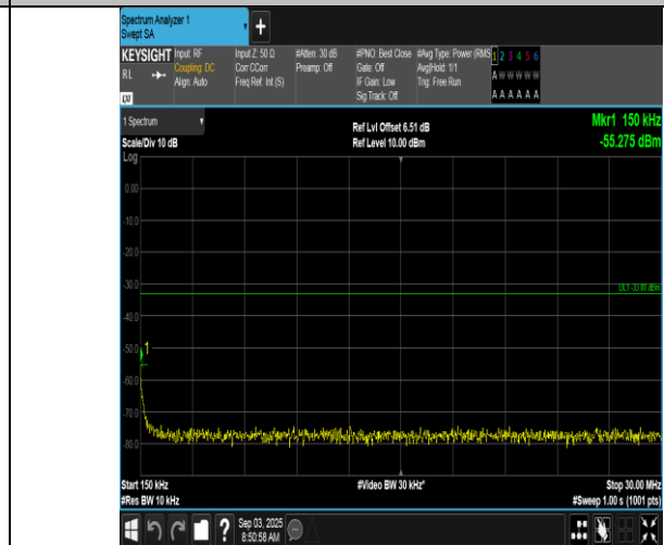
Band66-1.4MHz-16QAM-132322-1RB#5-0.15~30-PASS
