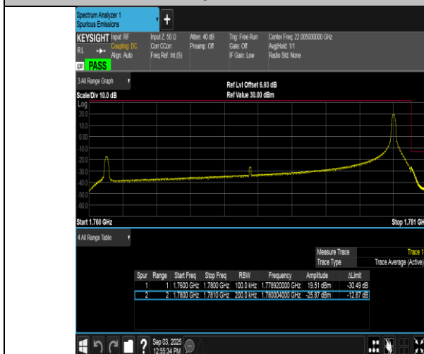
Band66-20MHz-16QAM-132572-1RB#99-PASS
