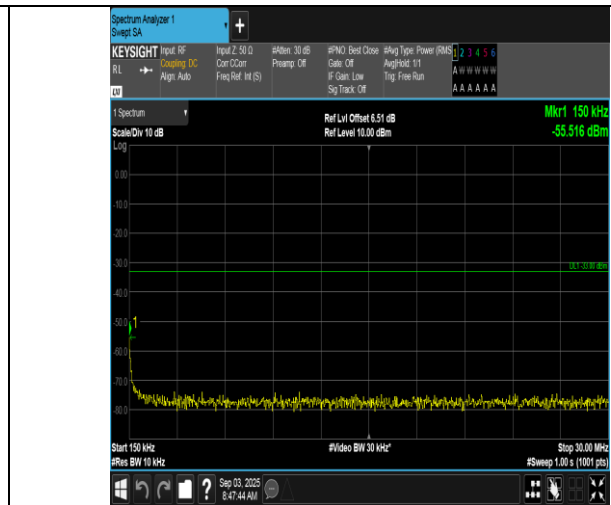
Band66-1.4MHz-QPSK-132322-1RB#0-0.15~30-PASS
