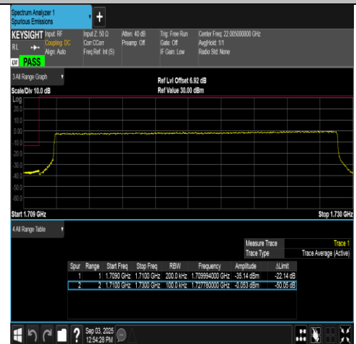
Band66-20MHz-16QAM-132072-100RB#0-PASS
