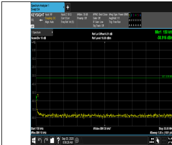
Band66-1.4MHz-QPSK-132665-1RB#5-0.15~30-PASS
