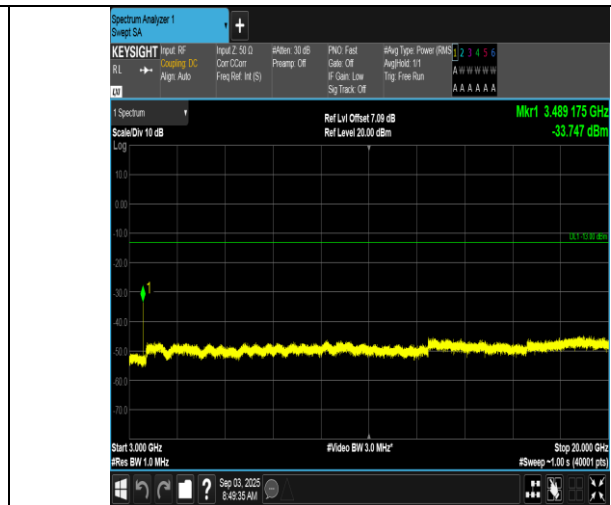
Band66-1.4MHz-16QAM-132322-1RB#0-3000~20000-PASS
