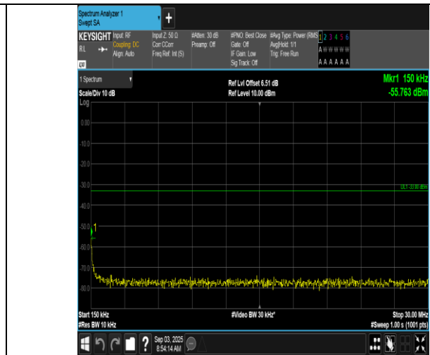
Band66-1.4MHz-QPSK-132665-1RB#0-0.15~30-PASS
