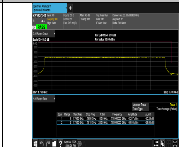
Band66-20MHz-16QAM-132572-100RB#0-PASS
