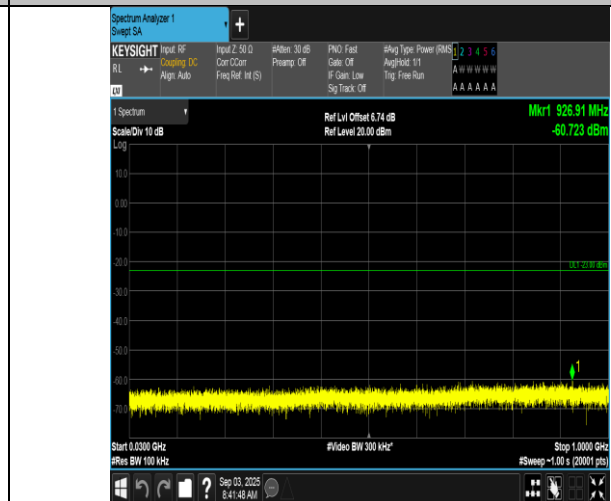
Band66-1.4MHz-16QAM-131979-1RB#0-30~1000-PASS
