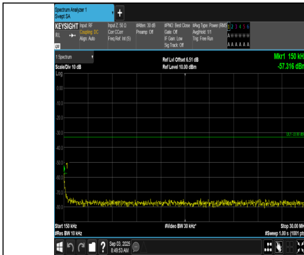
Band66-1.4MHz-QPSK-132322-1RB#5-0.15~30-PASS
