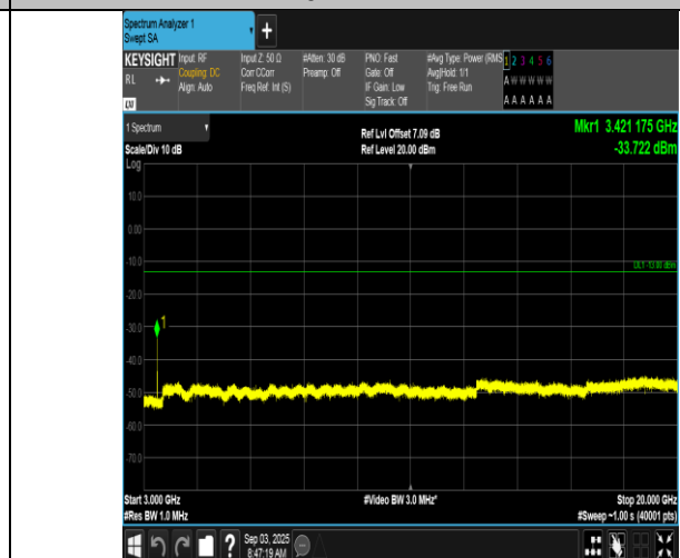
Band66-1.4MHz-16QAM-131979-6RB#0-3000~20000-PASS
