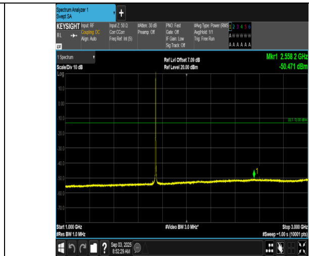
Band66-1.4MHz-QPSK-132322-6RB#0-1000~3000-PASS
