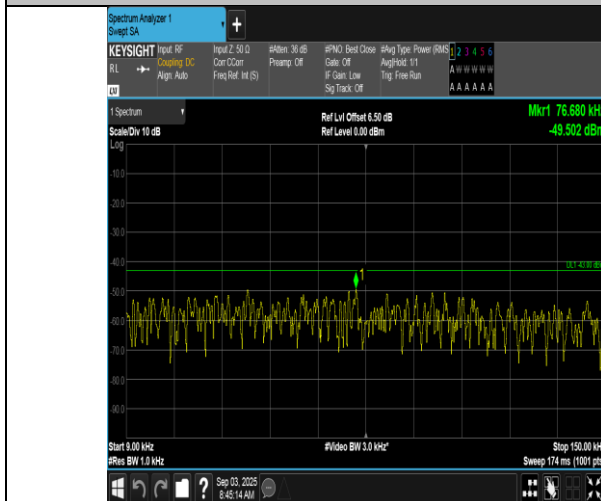
Band66-1.4MHz-QPSK-131979-6RB#0-0.009~0.15-PASS
