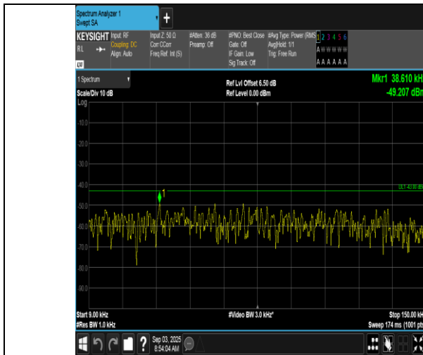
Band66-1.4MHz-QPSK-132665-1RB#0-0.009~0.15-PASS
