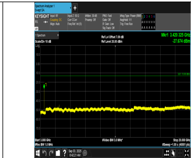
Band66-1.4MHz-16QAM-131979-1RB#0-3000~20000-PASS
