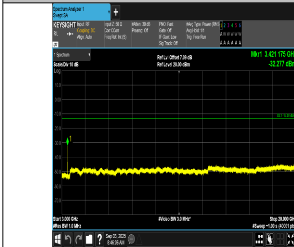
Band66-1.4MHz-QPSK-131979-6RB#0-3000~20000-PASS
