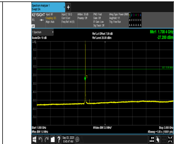
Band66-1.4MHz-QPSK-131979-6RB#0-1000~3000-PASS
