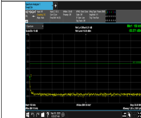
Band66-1.4MHz-16QAM-132322-6RB#0-0.15~30-PASS
