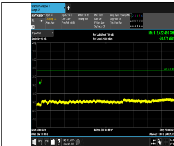
Band66-1.4MHz-16QAM-131979-1RB#5-3000~20000-PASS
