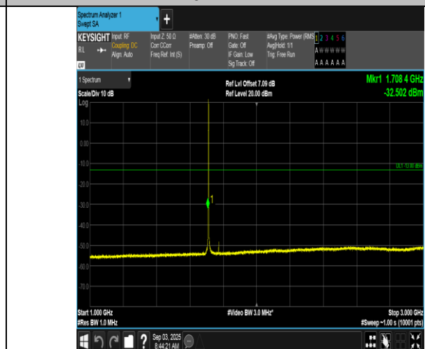
Band66-1.4MHz-16QAM-131979-1RB#5-1000~3000-PASS
