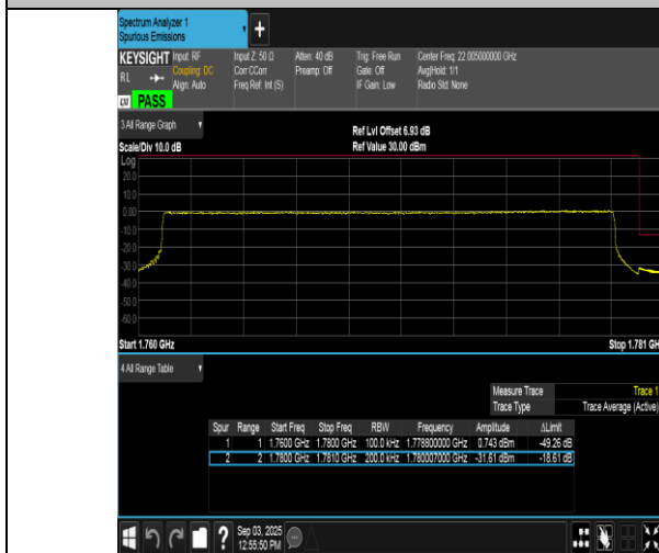
Band66-20MHz-QPSK-132572-100RB#0-PASS
