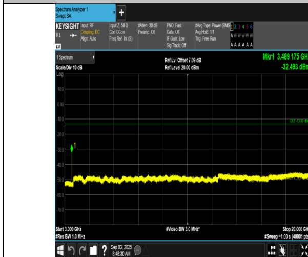
Band66-1.4MHz-QPSK-132322-1RB#0-3000~20000-PASS
