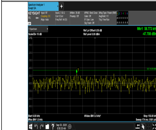
Band66-1.4MHz-QPSK-132665-6RB#0-0.009~0.15-PASS
