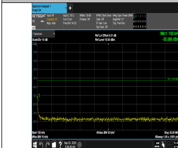
Band66-1.4MHz-16QAM-132322-1RB#0-0.15~30-PASS
