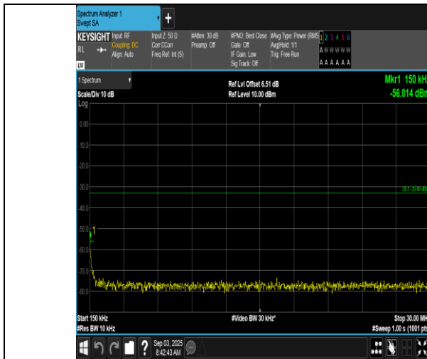
Band66-1.4MHz-QPSK-131979-1RB#5-0.15~30-PASS
