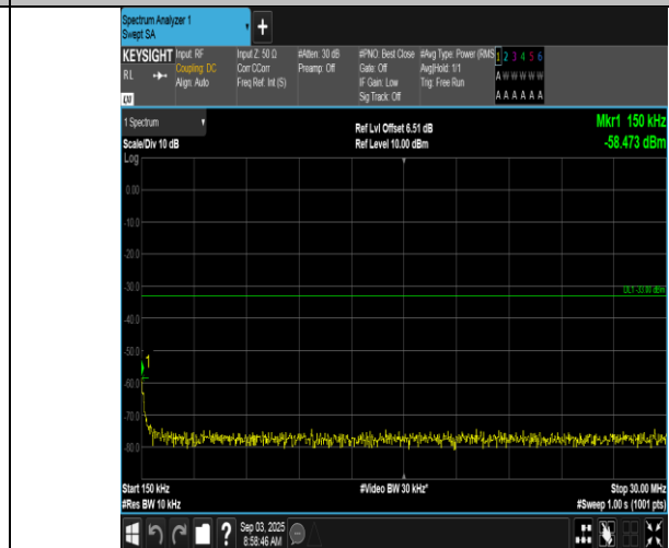
Band66-1.4MHz-QPSK-132665-6RB#0-0.15~30-PASS
