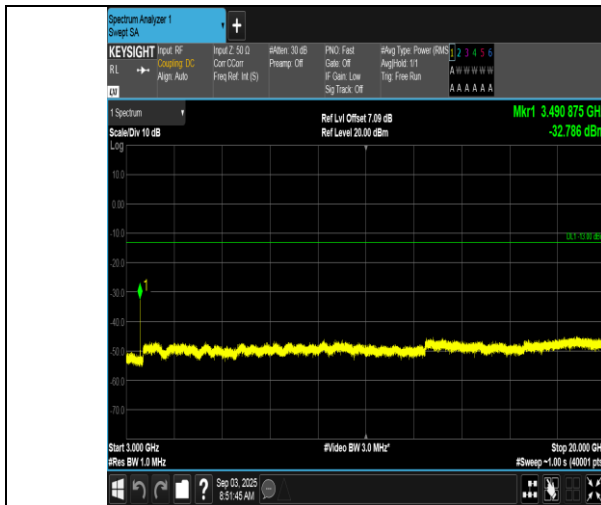
Band66-1.4MHz-16QAM-132322-1RB#5-3000~20000-PASS
