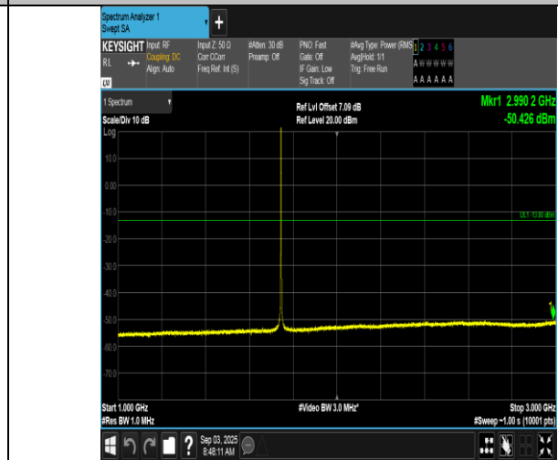
Band66-1.4MHz-QPSK-132322-1RB#0-1000~3000-PASS
