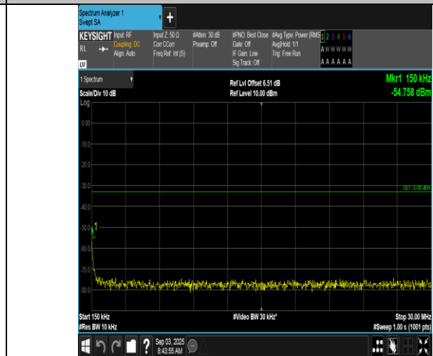
Band66-1.4MHz-16QAM-131979-1RB#5-0.15~30-PASS
