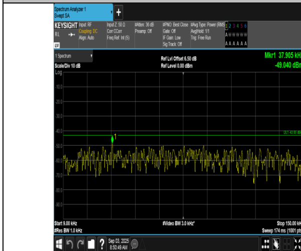
Band66-1.4MHz-16QAM-132322-1RB#5-0.009~0.15-PASS
