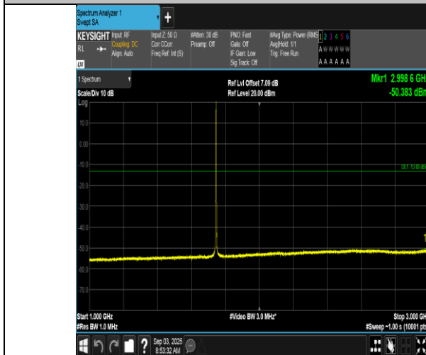
Band66-1.4MHz-16QAM-132322-6RB#0-1000~3000-PASS
