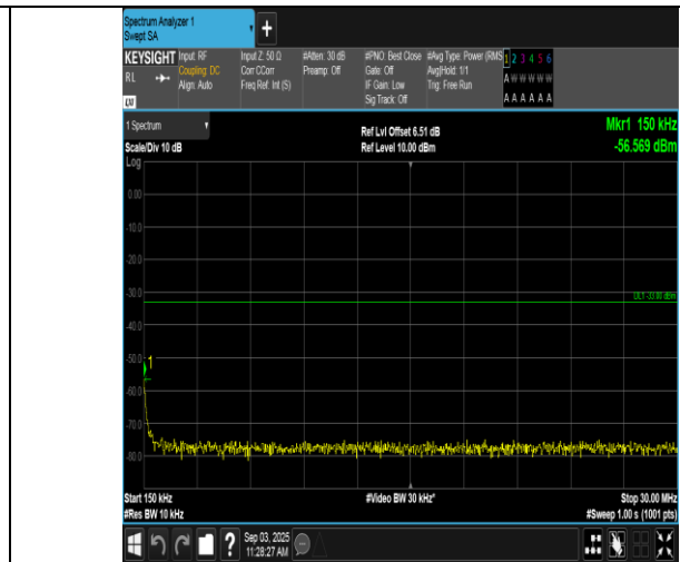
Band66-10MHz-QPSK-132622-1RB#0-0.15~30-PASS
