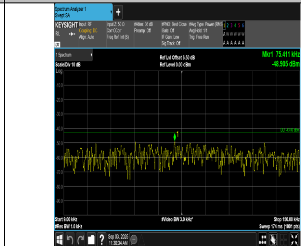
Band66-10MHz-QPSK-132622-1RB#49-0.009~0.15-PASS
