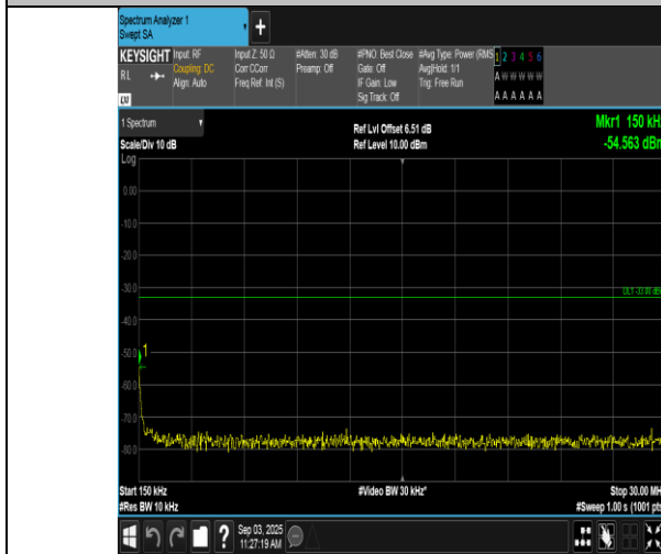
Band66-10MHz-16QAM-132322-50RB#0-0.15~30-PASS
