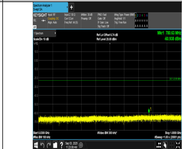
Band66-10MHz-16QAM-132322-1RB#0-30~1000-PASS
