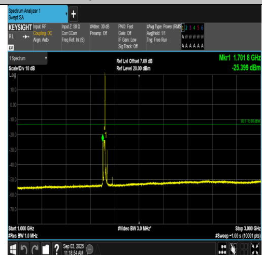
Band66-10MHz-16QAM-132022-1RB#49-1000~3000-PASS
