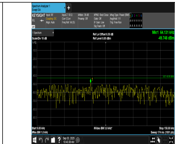
Band66-5MHz-16QAM-132647-25RB#0-0.009~0.15-PASS
