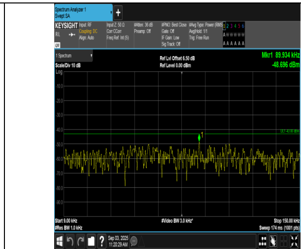
Band66-10MHz-16QAM-132022-50RB#0-0.009~0.15-PASS
