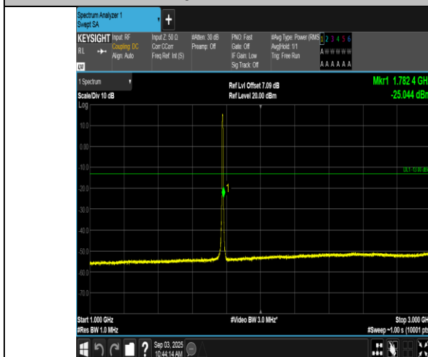
Band66-5MHz-16QAM-132647-25RB#0-1000~3000-PASS
