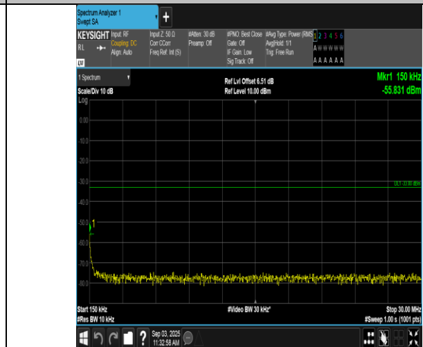
Band66-10MHz-QPSK-132622-50RB#0-0.15~30-PASS
