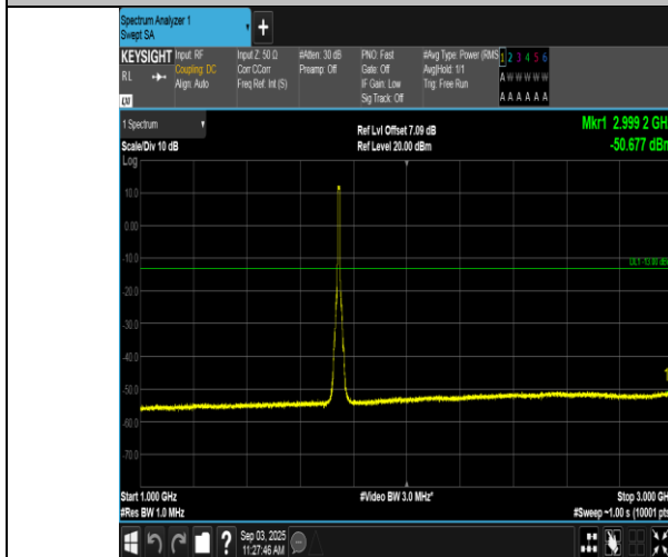
Band66-10MHz-16QAM-132322-50RB#0-1000~3000-PASS
