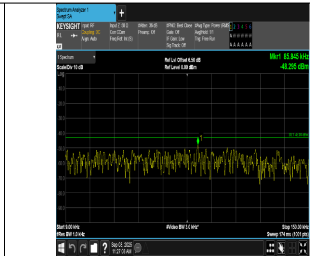
Band66-10MHz-16QAM-132322-50RB#0-0.009~0.15-PASS
