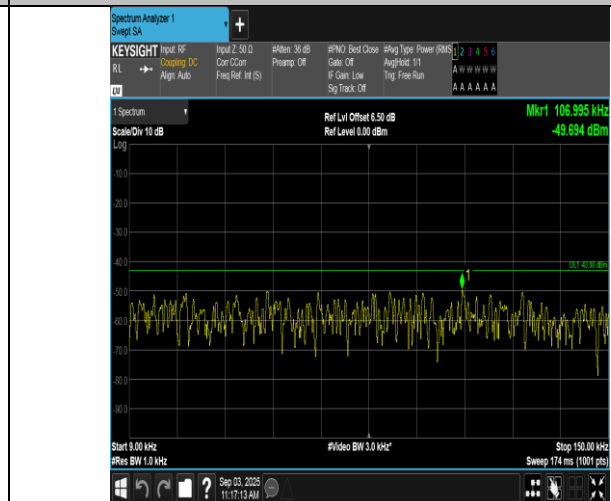
Band66-10MHz-QPSK-132022-1RB#49-0.009~0.15-PASS
