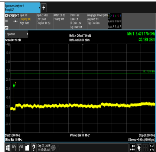
Band66-10MHz-16QAM-132022-1RB#0-3000~20000-PASS
