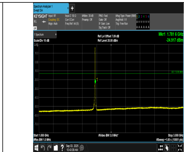
Band66-5MHz-QPSK-132647-25RB#0-1000~3000-PASS
