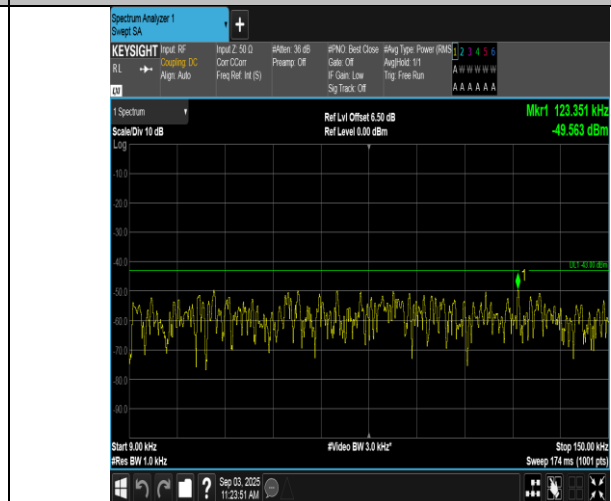
Band66-10MHz-QPSK-132322-1RB#49-0.009~0.15-PASS
