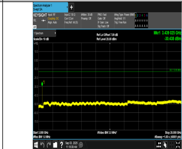
Band66-10MHz-QPSK-132022-1RB#49-3000~20000-PASS
