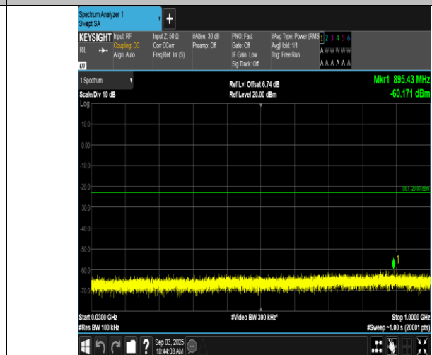
Band66-5MHz-16QAM-132647-25RB#0-30~1000-PASS
