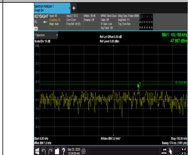
Band66-5MHz-16QAM-132647-1RB#0-0.009~0.15-PASS
