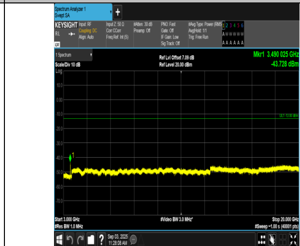
Band66-10MHz-16QAM-132322-50RB#0-3000~20000-PASS
