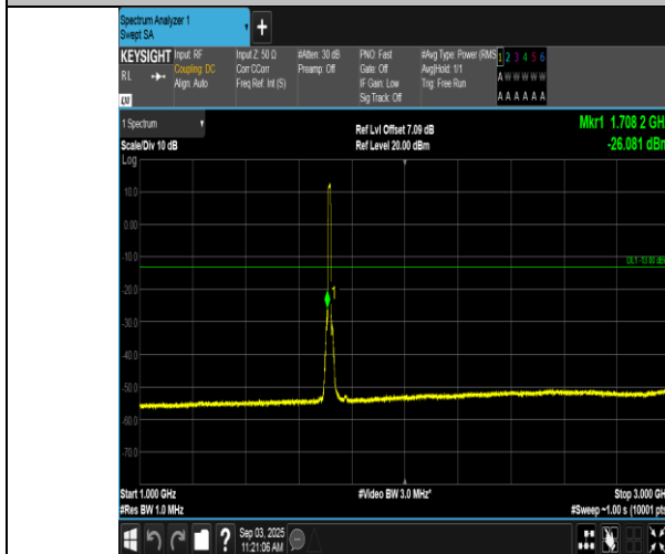
Band66-10MHz-16QAM-132022-50RB#0-1000~3000-PASS
