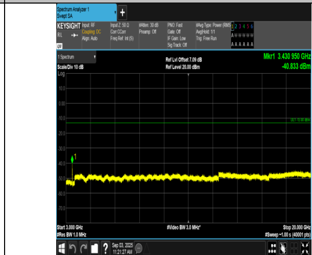
Band66-10MHz-16QAM-132022-50RB#0-3000~20000-PASS
