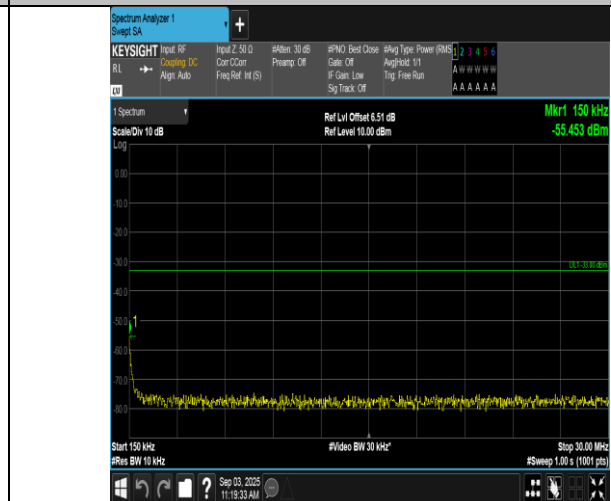
Band66-10MHz-QPSK-132022-50RB#0-0.15~30-PASS
