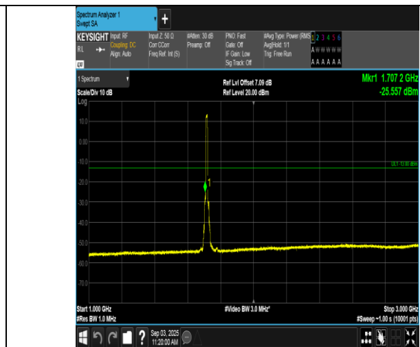
Band66-10MHz-QPSK-132022-50RB#0-1000~3000-PASS
