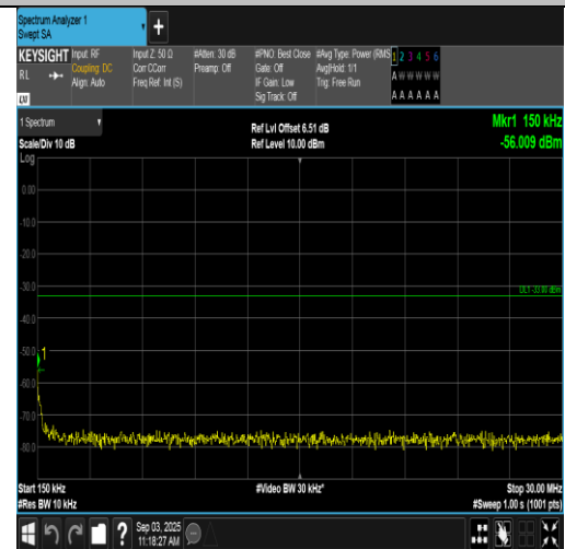
Band66-10MHz-16QAM-132022-1RB#49-0.15~30-PASS
