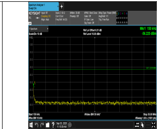
Band66-10MHz-QPSK-132022-1RB#0-0.15~30-PASS
