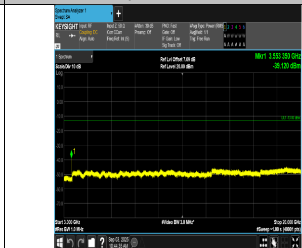
Band66-5MHz-16QAM-132647-25RB#0-3000~20000-PASS
