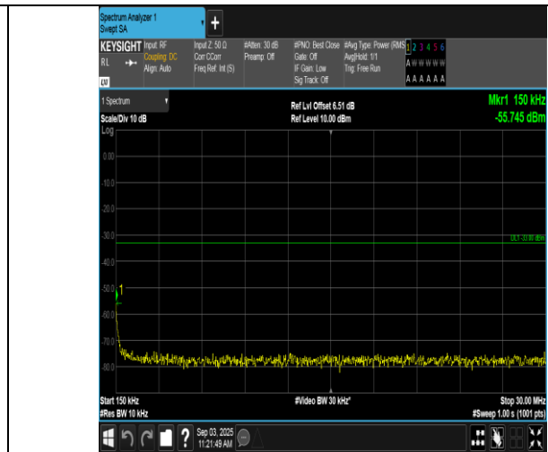
Band66-10MHz-QPSK-132322-1RB#0-0.15~30-PASS
