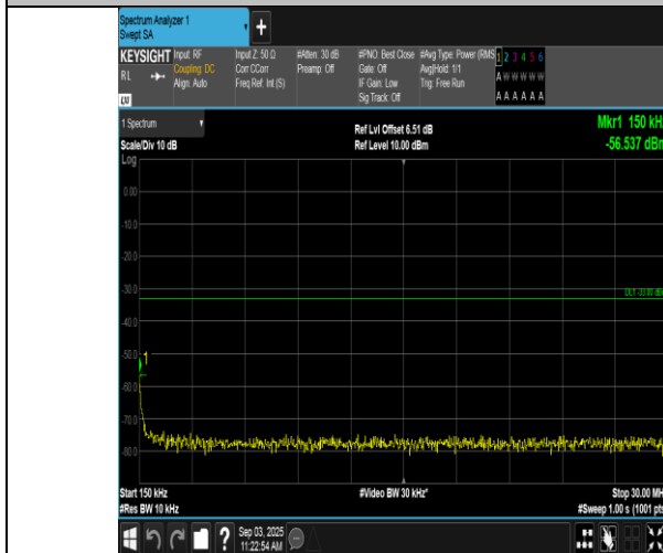
Band66-10MHz-16QAM-132322-1RB#0-0.15~30-PASS
