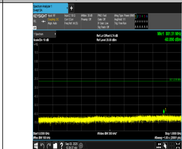
Band66-5MHz-16QAM-132647-1RB#0-30~1000-PASS
