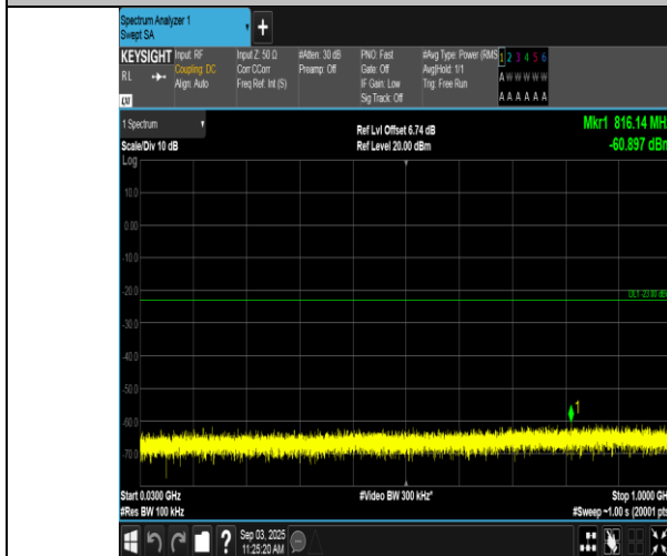
Band66-10MHz-16QAM-132322-1RB#49-30~1000-PASS
