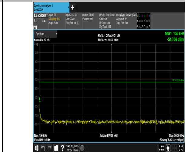
Band66-10MHz-QPSK-132322-50RB#0-0.15~30-PASS
