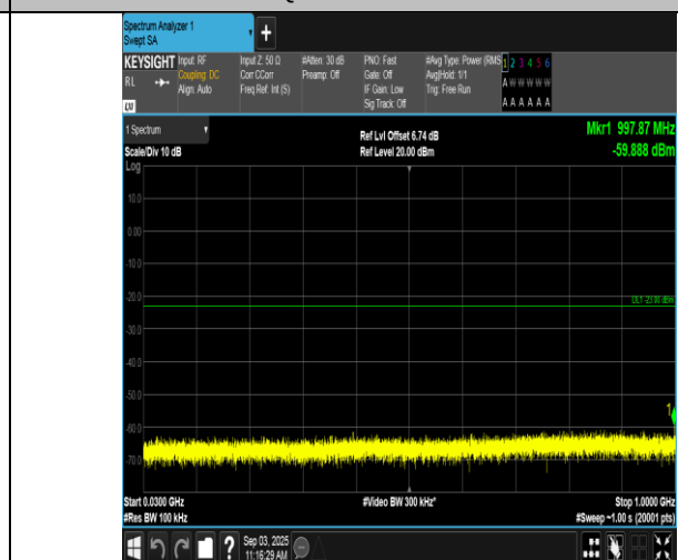
Band66-10MHz-16QAM-132022-1RB#0-30~1000-PASS
