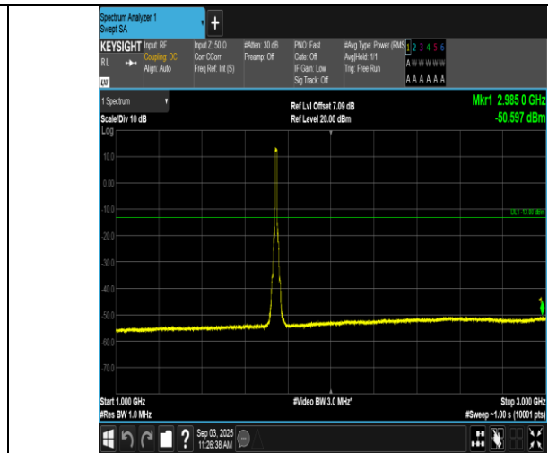
Band66-10MHz-QPSK-132322-50RB#0-1000~3000-PASS
