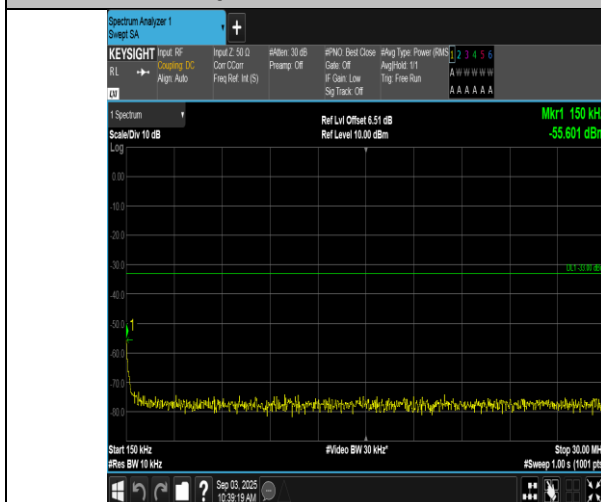
Band66-5MHz-16QAM-132647-1RB#0-0.15~30-PASS
