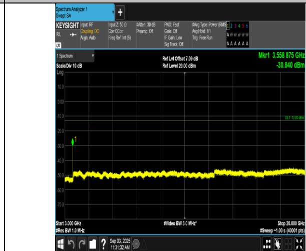
Band66-10MHz-QPSK-132622-1RB#49-3000~20000-PASS
