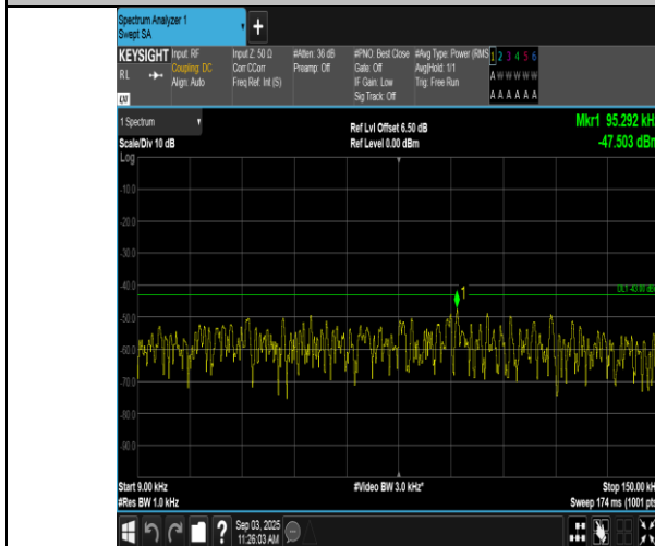
Band66-10MHz-QPSK-132322-50RB#0-0.009~0.15-PASS
