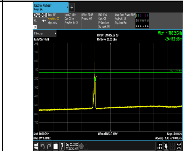
Band66-10MHz-QPSK-132622-1RB#0-1000~3000-PASS
