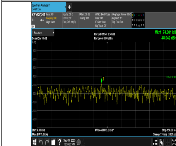
Band66-15MHz-QPSK-132597-75RB#0-0.009~0.15-PASS
