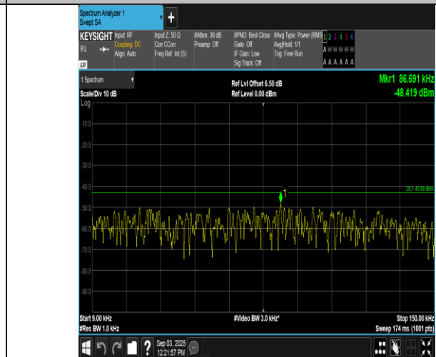
Band66-15MHz-QPSK-132597-1RB#74-0.009~0.15-PASS
