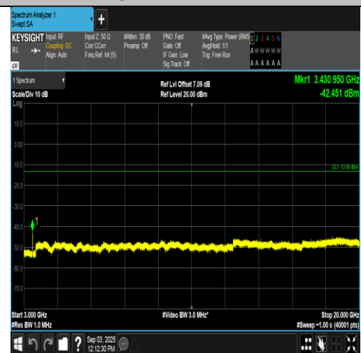
Band66-15MHz-16QAM-132047-75RB#0-3000~20000-PASS
