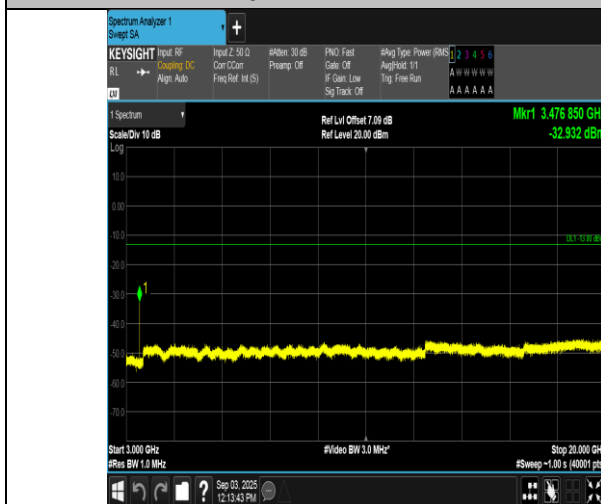
Band66-15MHz-QPSK-132322-1RB#0-3000~20000-PASS
