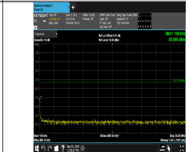
Band66-15MHz-16QAM-132047-1RB#74-0.15~30-PASS
