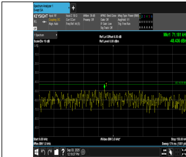
Band66-15MHz-QPSK-132597-1RB#0-0.009~0.15-PASS
