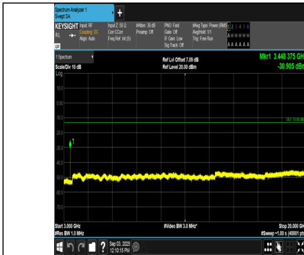
Band66-15MHz-16QAM-132047-1RB#74-3000~20000-PASS
