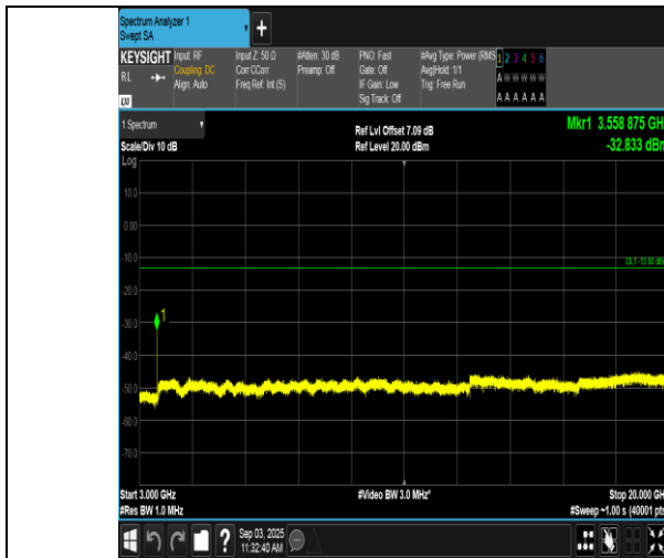
Band66-10MHz-16QAM-132622-1RB#49-3000~20000-PASS
