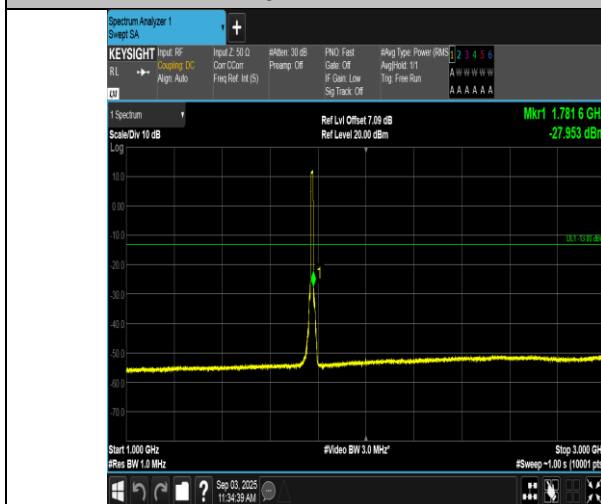
Band66-10MHz-16QAM-132622-50RB#0-1000~3000-PASS
