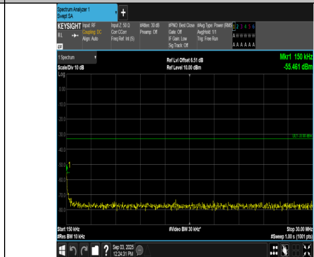
Band66-15MHz-QPSK-132597-75RB#0-0.15~30-PASS
