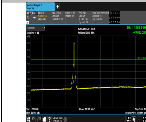
Band66-15MHz-16QAM-132322-75RB#0-1000~3000-PASS
