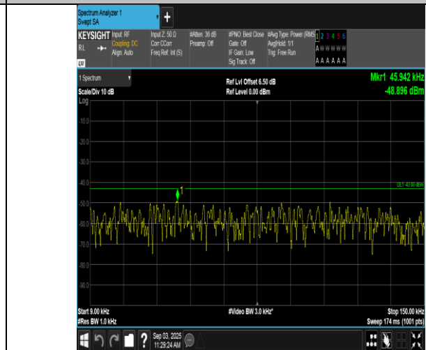
Band66-10MHz-16QAM-132622-1RB#0-0.009~0.15-PASS
