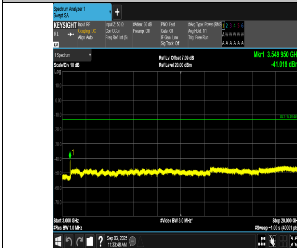
Band66-10MHz-QPSK-132622-50RB#0-3000~20000-PASS
