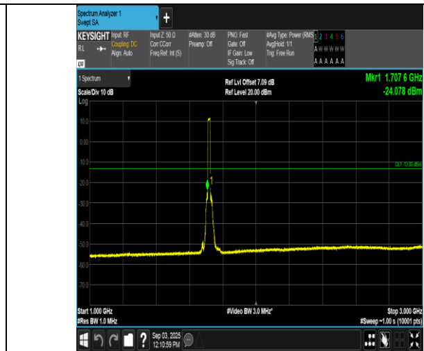
Band66-15MHz-QPSK-132047-75RB#0-1000~3000-PASS
