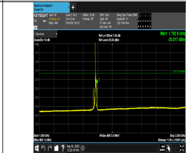
Band66-15MHz-QPSK-132597-1RB#0-1000~3000-PASS
