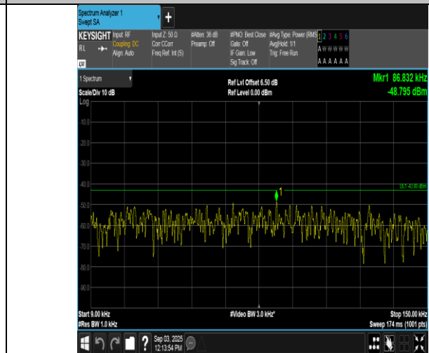
Band66-15MHz-16QAM-132322-1RB#0-0.009~0.15-PASS
