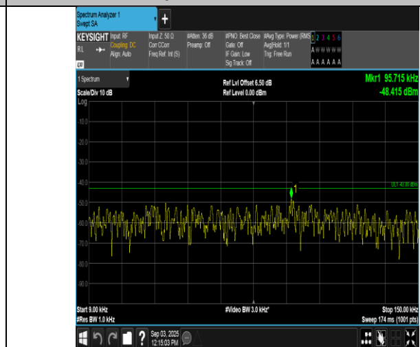
Band66-15MHz-QPSK-132322-1RB#74-0.009~0.15-PASS
