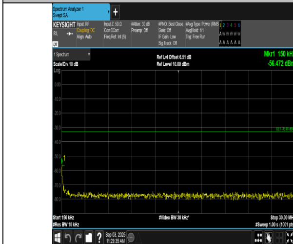
Band66-10MHz-16QAM-132622-1RB#0-0.15~30-PASS
