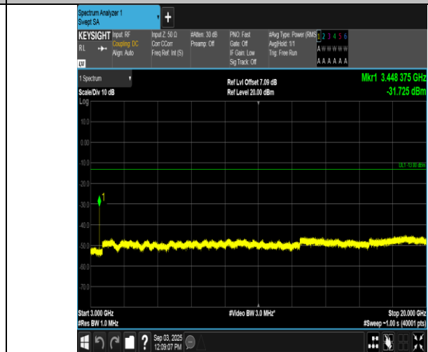
Band66-15MHz-QPSK-132047-1RB#74-3000~20000-PASS
