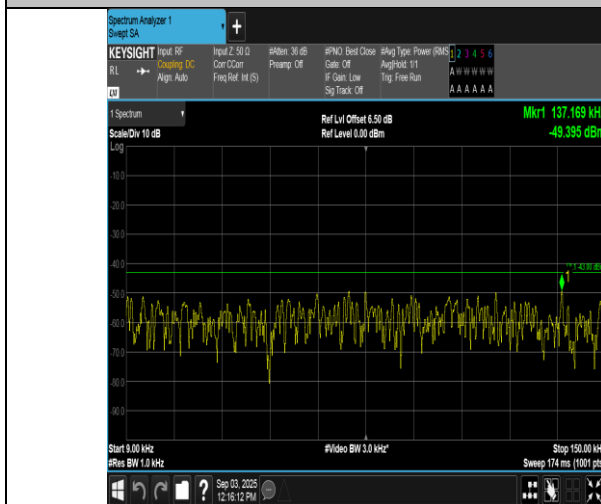
Band66-15MHz-16QAM-132322-1RB#74-0.009~0.15-PASS
