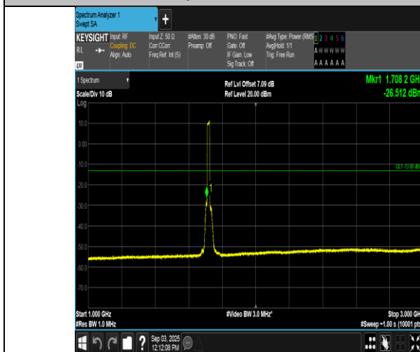
Band66-15MHz-16QAM-132047-75RB#0-1000~3000-PASS
