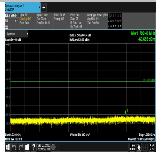
Band66-15MHz-16QAM-132047-75RB#0-30~1000-PASS
