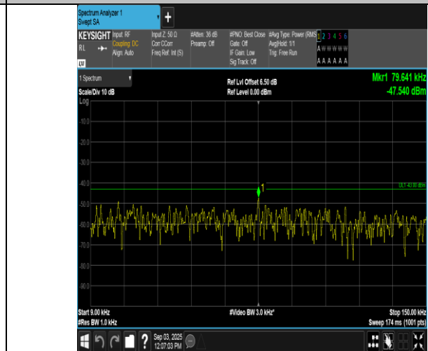
Band66-15MHz-16QAM-132047-1RB#0-0.009~0.15-PASS
