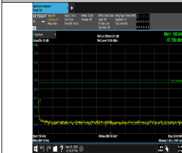
Band66-15MHz-16QAM-132322-75RB#0-0.15~30-PASS
