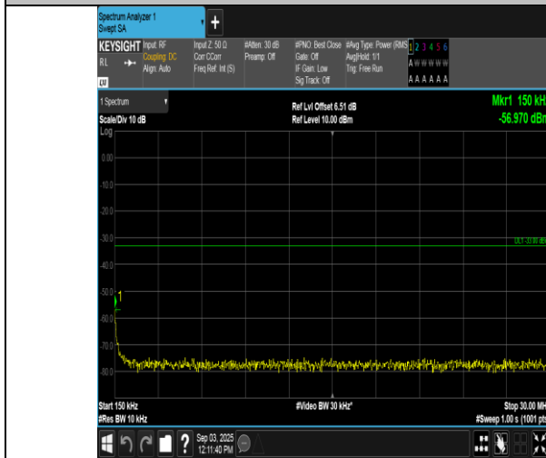
Band66-15MHz-16QAM-132047-75RB#0-0.15~30-PASS
