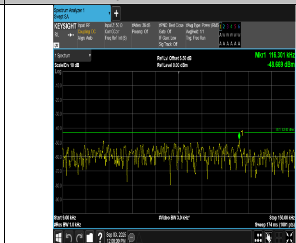
Band66-15MHz-QPSK-132047-1RB#74-0.009~0.15-PASS
