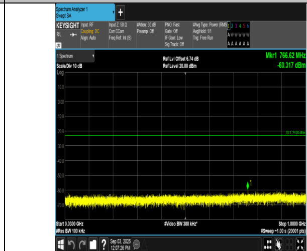
Band66-15MHz-16QAM-132047-1RB#0-30~1000-PASS
