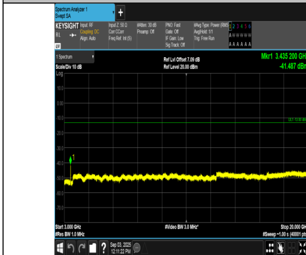
Band66-15MHz-QPSK-132047-75RB#0-3000~20000-PASS
