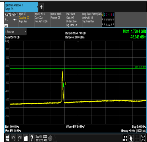
Band66-10MHz-16QAM-132622-1RB#49-1000~3000-PASS
