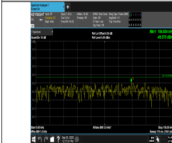
Band66-15MHz-QPSK-132322-75RB#0-0.009~0.15-PASS
