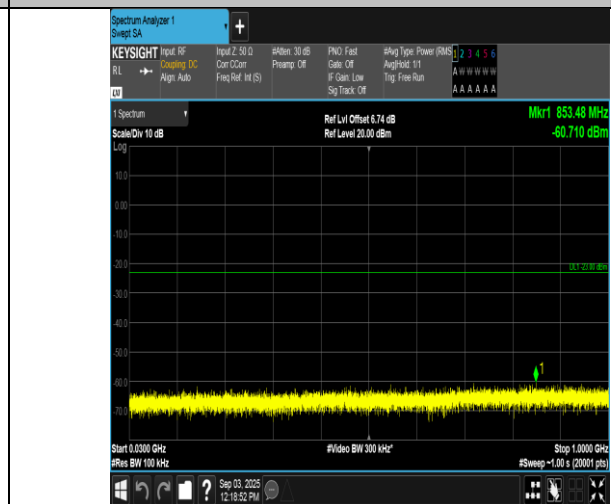
Band66-15MHz-16QAM-132322-75RB#0-30~1000-PASS
