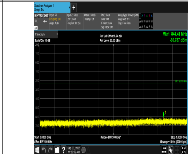
Band66-10MHz-16QAM-132622-1RB#0-30~1000-PASS
