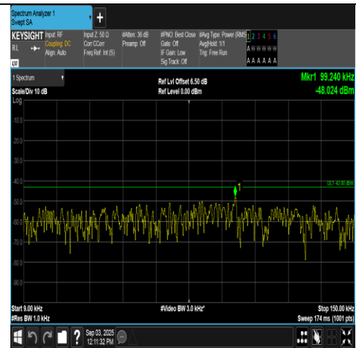
Band66-15MHz-16QAM-132047-75RB#0-0.009~0.15-PASS
