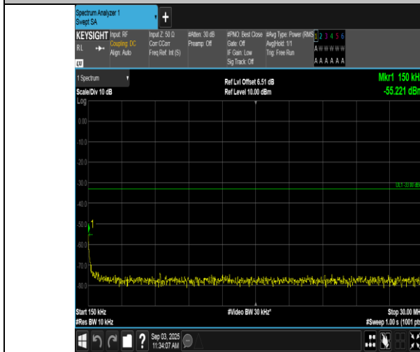
Band66-10MHz-16QAM-132622-50RB#0-0.15~30-PASS
