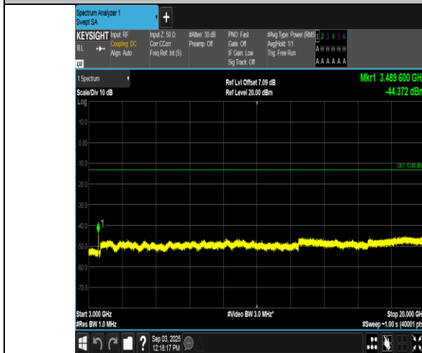
Band66-15MHz-QPSK-132322-75RB#0-3000~20000-PASS
