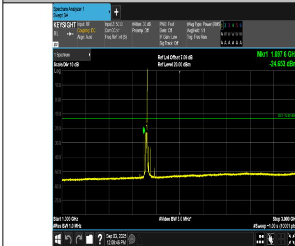
Band66-15MHz-QPSK-132047-1RB#74-1000~3000-PASS
