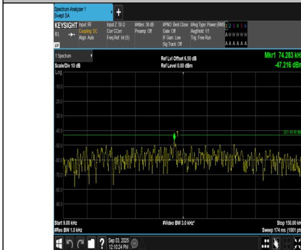
Band66-15MHz-QPSK-132047-75RB#0-0.009~0.15-PASS
