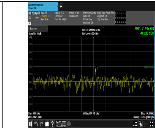
Band66-10MHz-16QAM-132622-50RB#0-0.009~0.15-PASS
