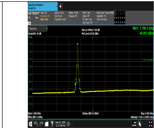
Band66-15MHz-QPSK-132322-75RB#0-1000~3000-PASS
