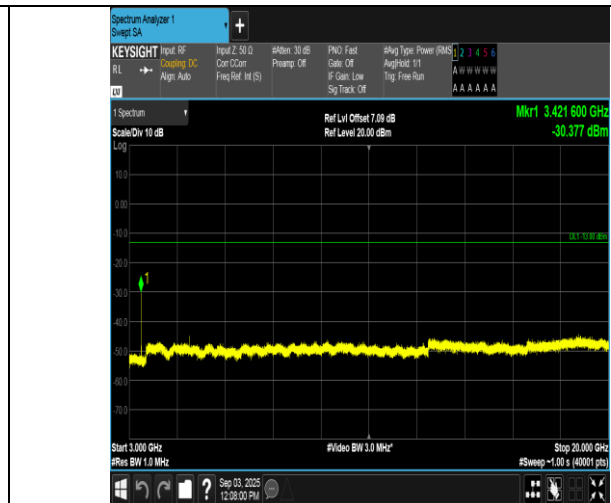
Band66-15MHz-16QAM-132047-1RB#0-3000~20000-PASS
