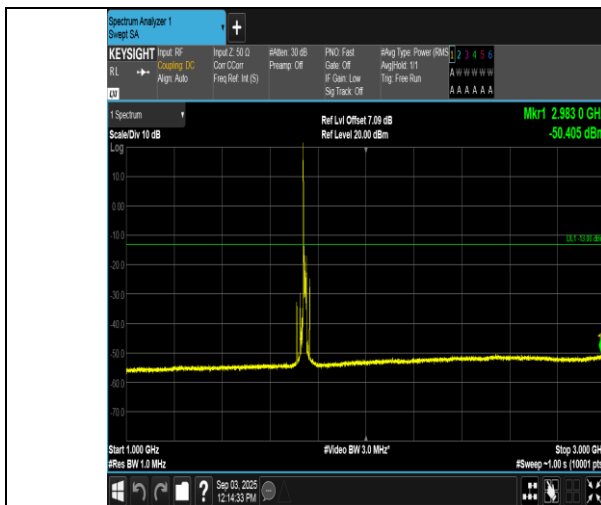
Band66-15MHz-16QAM-132322-1RB#0-1000~3000-PASS
