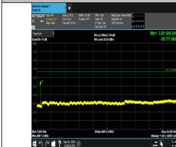
Band66-15MHz-QPSK-132047-1RB#0-3000~20000-PASS
