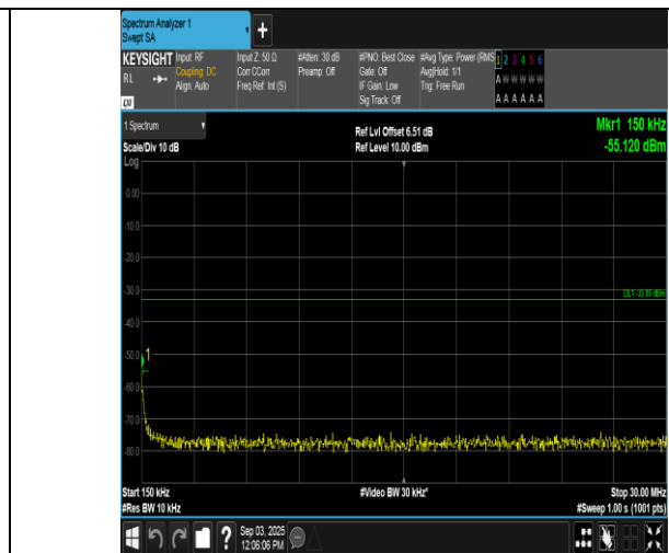
Band66-15MHz-QPSK-132047-1RB#0-0.15~30-PASS
