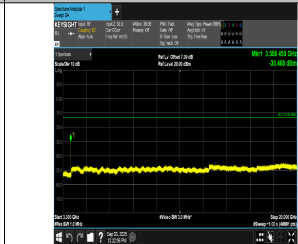
Band66-15MHz-QPSK-132597-1RB#74-3000~20000-PASS
