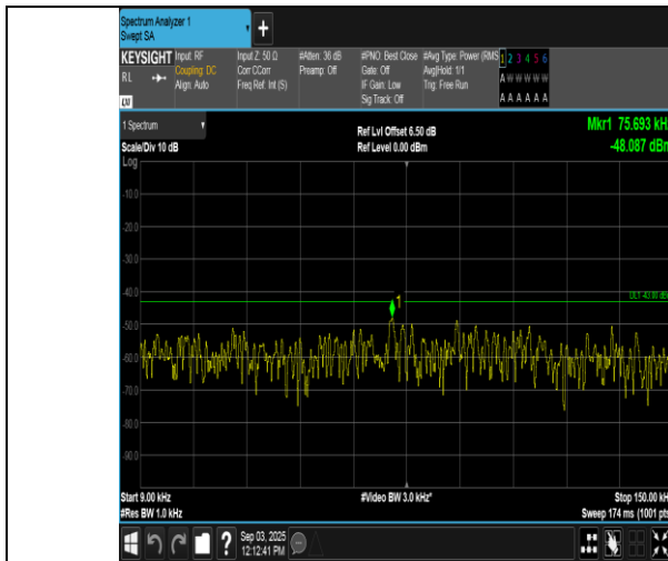
Band66-15MHz-QPSK-132322-1RB#0-0.009~0.15-PASS
