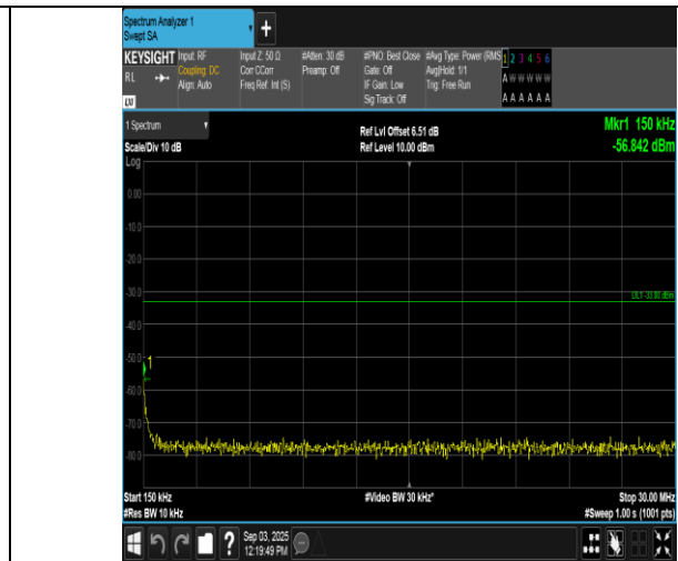
Band66-15MHz-QPSK-132597-1RB#0-0.15~30-PASS
