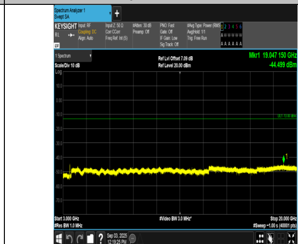
Band66-15MHz-16QAM-132322-75RB#0-3000~20000-PASS
