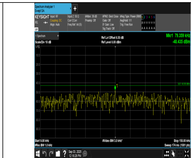
Band66-15MHz-16QAM-132322-75RB#0-0.009~0.15-PASS
