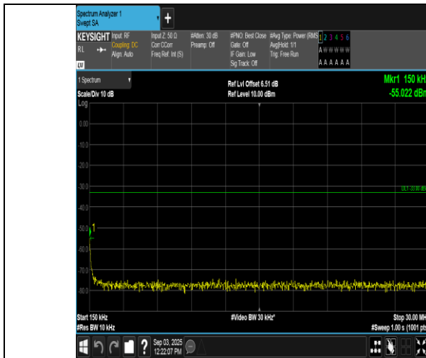
Band66-15MHz-QPSK-132597-1RB#74-0.15~30-PASS
