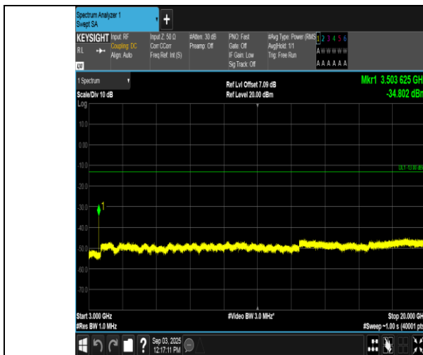
Band66-15MHz-16QAM-132322-1RB#74-3000~20000-PASS
