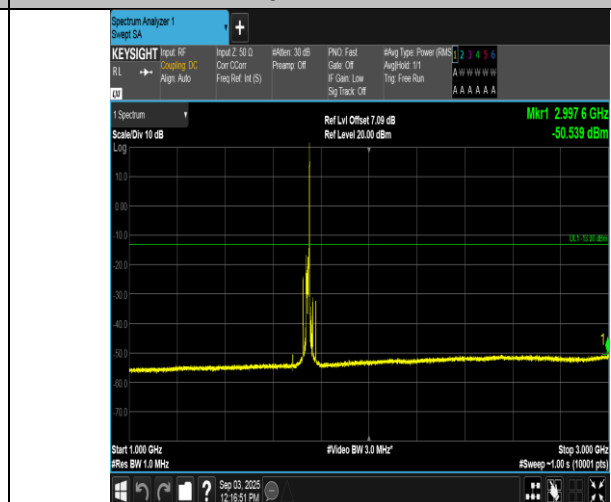
Band66-15MHz-16QAM-132322-1RB#74-1000~3000-PASS
