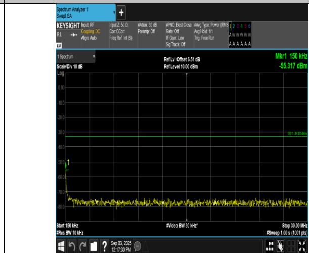
Band66-15MHz-QPSK-132322-75RB#0-0.15~30-PASS
