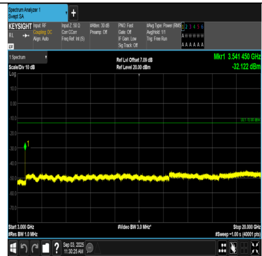
Band66-10MHz-16QAM-132622-1RB#0-3000~20000-PASS
