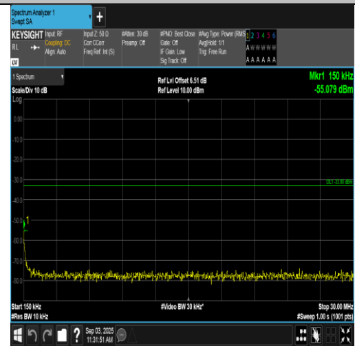
Band66-10MHz-16QAM-132622-1RB#49-0.15~30-PASS
