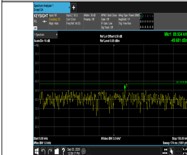
Band66-15MHz-16QAM-132047-1RB#74-0.009~0.15-PASS
