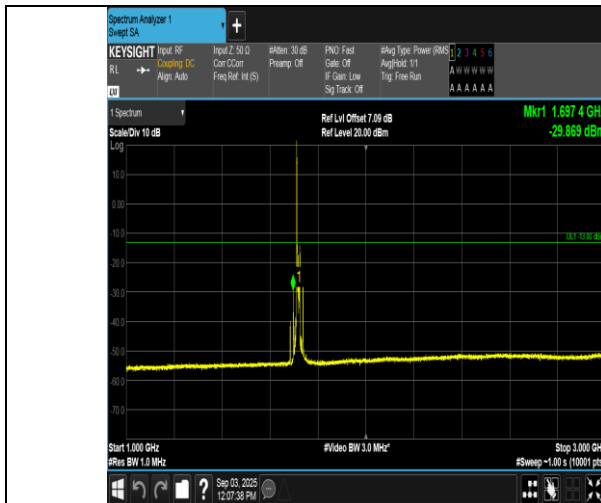
Band66-15MHz-16QAM-132047-1RB#0-1000~3000-PASS
