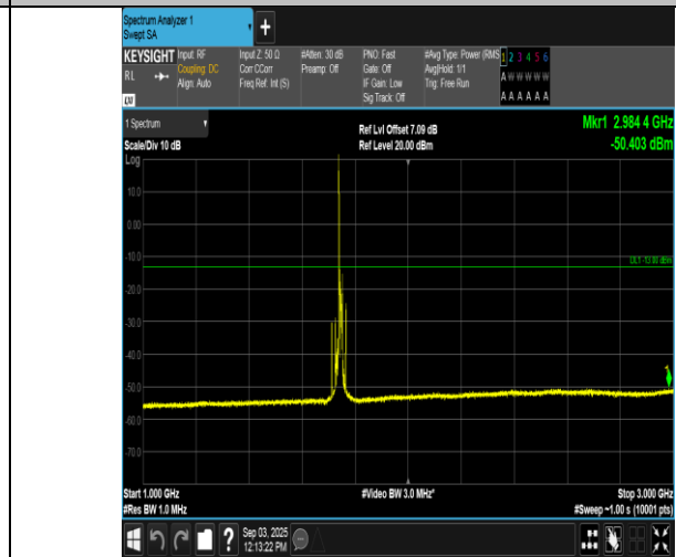
Band66-15MHz-QPSK-132322-1RB#0-1000~3000-PASS
