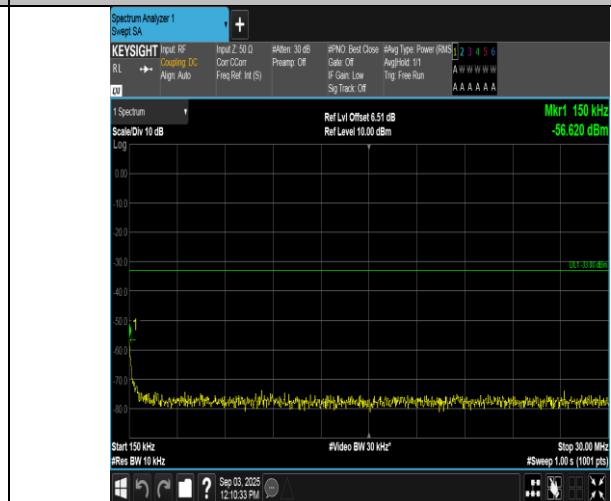
Band66-15MHz-QPSK-132047-75RB#0-0.15~30-PASS
