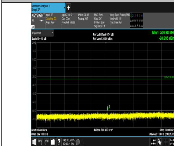
Band66-15MHz-QPSK-132047-1RB#0-30~1000-PASS
