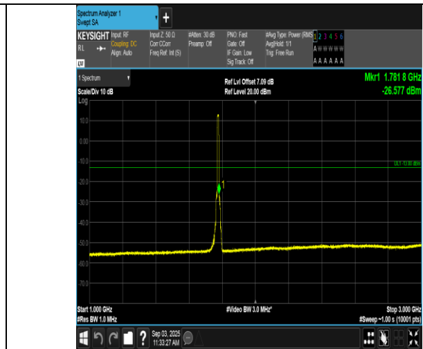
Band66-10MHz-QPSK-132622-50RB#0-1000~3000-PASS
