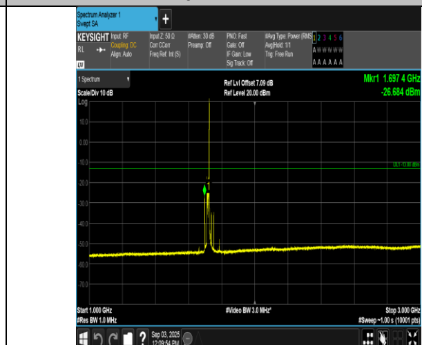
Band66-15MHz-16QAM-132047-1RB#74-1000~3000-PASS
