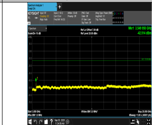
Band66-10MHz-16QAM-132622-50RB#0-3000~20000-PASS
