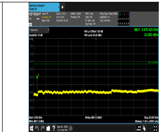
Band66-15MHz-16QAM-132322-1RB#0-3000~20000-PASS
