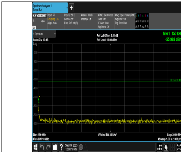
Band66-15MHz-QPSK-132047-1RB#74-0.15~30-PASS
