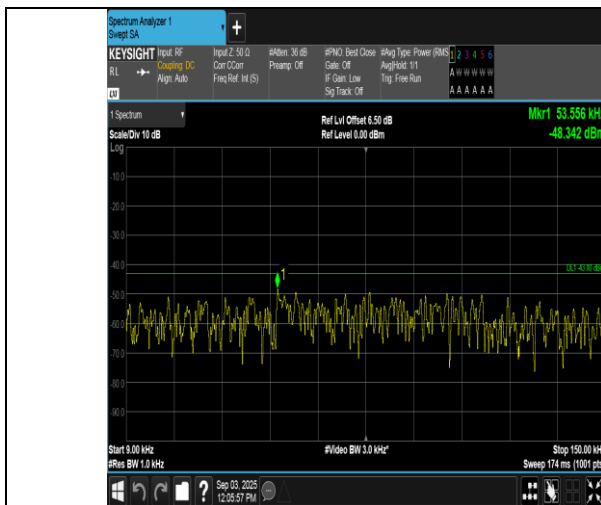
Band66-15MHz-QPSK-132047-1RB#0-0.009~0.15-PASS
