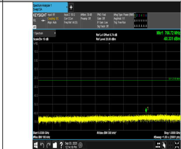
Band66-15MHz-16QAM-132322-1RB#0-30~1000-PASS
