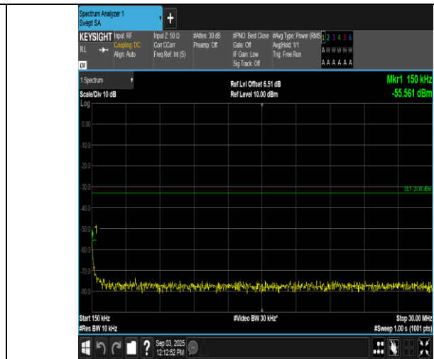
Band66-15MHz-QPSK-132322-1RB#0-0.15~30-PASS
