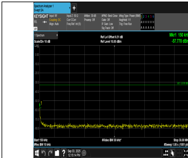
Band66-15MHz-QPSK-132322-1RB#74-0.15~30-PASS
