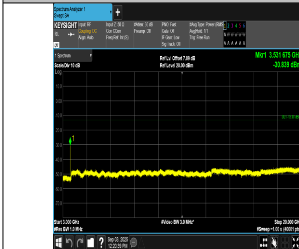
Band66-15MHz-QPSK-132597-1RB#0-3000~20000-PASS
