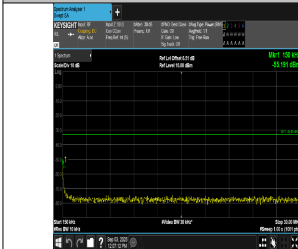
Band66-15MHz-16QAM-132047-1RB#0-0.15~30-PASS
