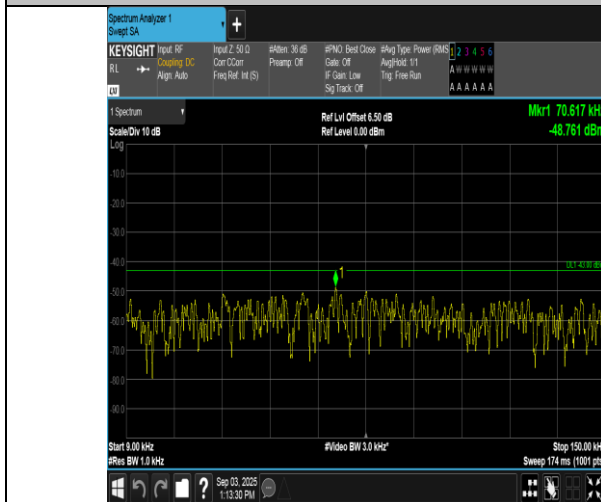
Band66-20MHz-16QAM-132572-1RB#99-0.009~0.15-PASS
