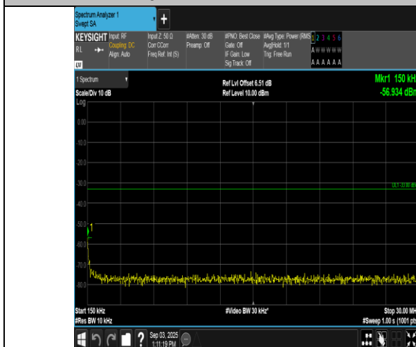
Band66-20MHz-16QAM-132572-1RB#0-0.15~30-PASS
