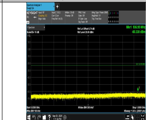
Band66-20MHz-16QAM-132572-1RB#0-30~1000-PASS
