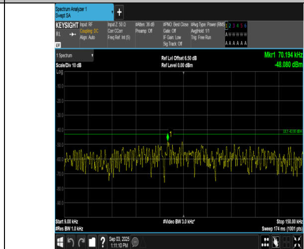
Band66-20MHz-16QAM-132572-1RB#0-0.009~0.15-PASS
