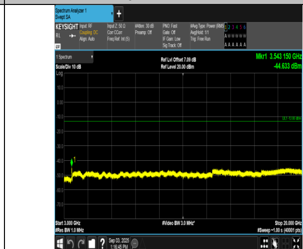
Band66-20MHz-16QAM-132572-100RB#0-3000~20000-PASS
