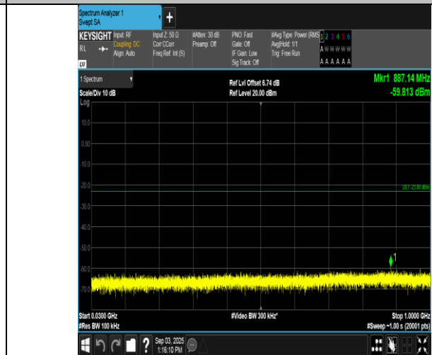
Band66-20MHz-16QAM-132572-100RB#0-30~1000-PASS
