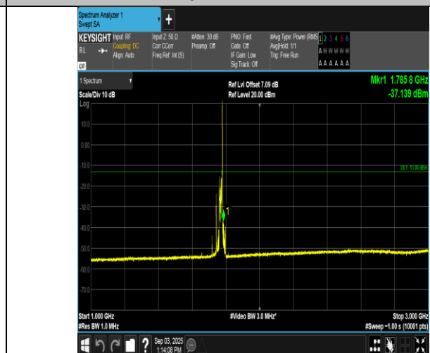
Band66-20MHz-16QAM-132572-1RB#99-1000~3000-PASS
