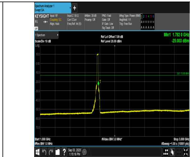
Band66-20MHz-QPSK-132572-100RB#0-1000~3000-PASS
