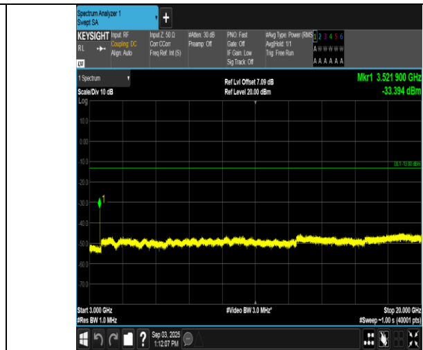
Band66-20MHz-16QAM-132572-1RB#0-3000~20000-PASS
