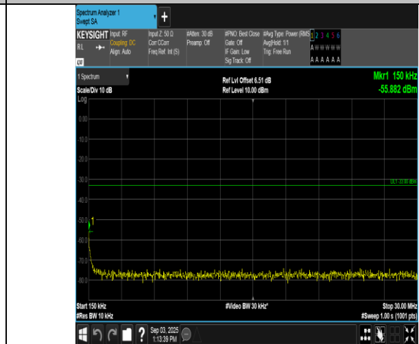
Band66-20MHz-16QAM-132572-1RB#99-0.15~30-PASS
