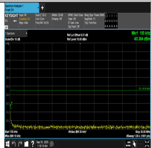
Band7-10MHz-16QAM-21100-1RB#49-0.15~30-PASS
