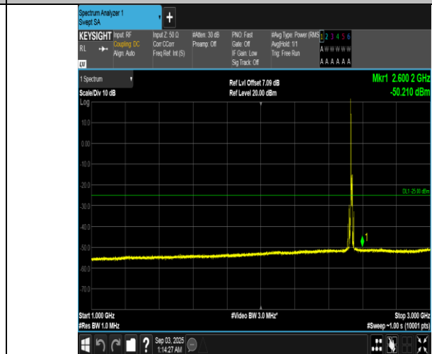
Band7-10MHz-QPSK-21100-1RB#0-1000~3000-PASS
