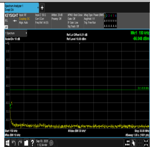
Band7-10MHz-16QAM-20800-50RB#0-0.15~30-PASS
