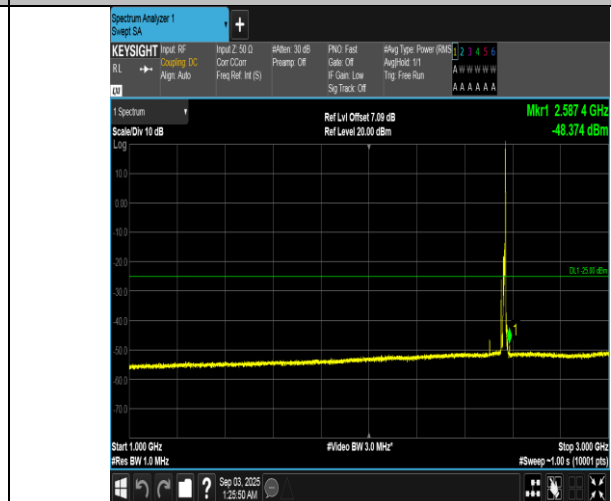
Band7-10MHz-QPSK-21400-1RB#49-1000~3000-PASS
