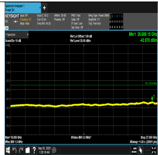
Band7-10MHz-QPSK-21400-50RB#0-18000~27000-PASS
