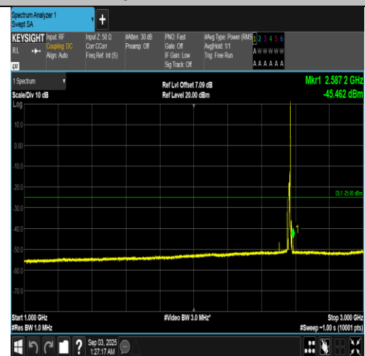
Band7-10MHz-16QAM-21400-1RB#49-1000~3000-PASS
