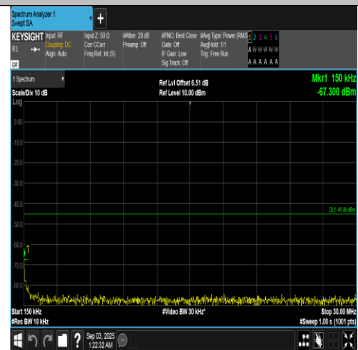
Band7-10MHz-QPSK-21400-1RB#0-0.15~30-PASS
