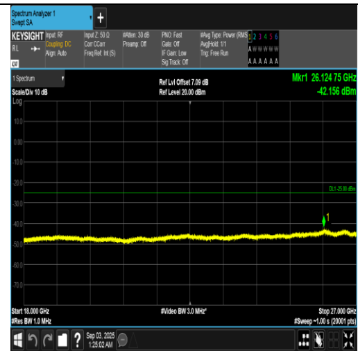
Band7-10MHz-16QAM-21400-1RB#0-18000~27000-PASS
