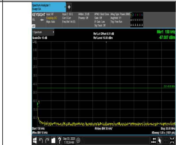
Band7-10MHz-16QAM-21100-1RB#0-0.15~30-PASS
