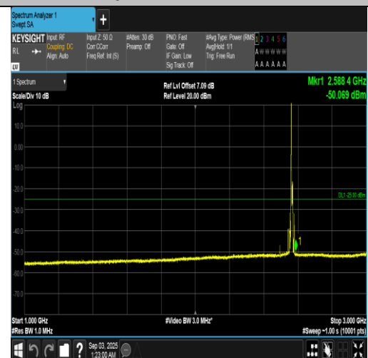
Band7-10MHz-QPSK-21400-1RB#0-1000~3000-PASS
