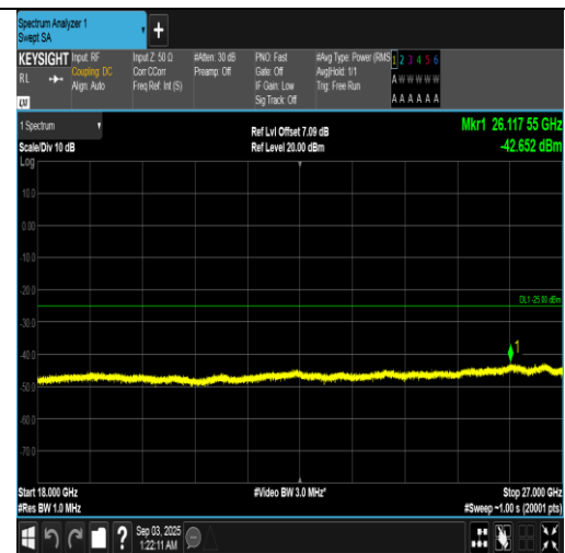
Band7-10MHz-16QAM-21100-50RB#0-18000~27000-PASS
