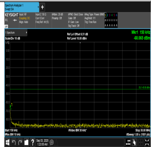
Band7-10MHz-16QAM-21400-1RB#0-0.15~30-PASS
