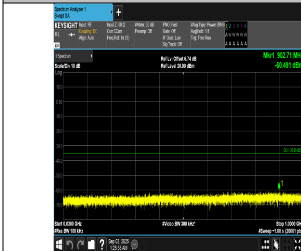
Band7-10MHz-QPSK-21400-1RB#49-30~1000-PASS
