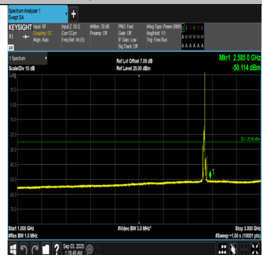
Band7-10MHz-16QAM-21100-1RB#49-1000~3000-PASS
