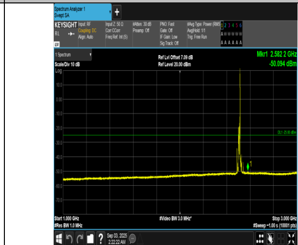
Band7-15MHz-QPSK-20825-1RB#74-1000~3000-PASS
