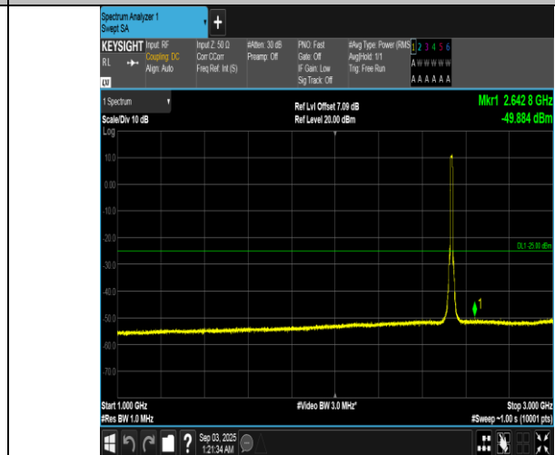
Band7-10MHz-16QAM-21100-50RB#0-1000~3000-PASS
