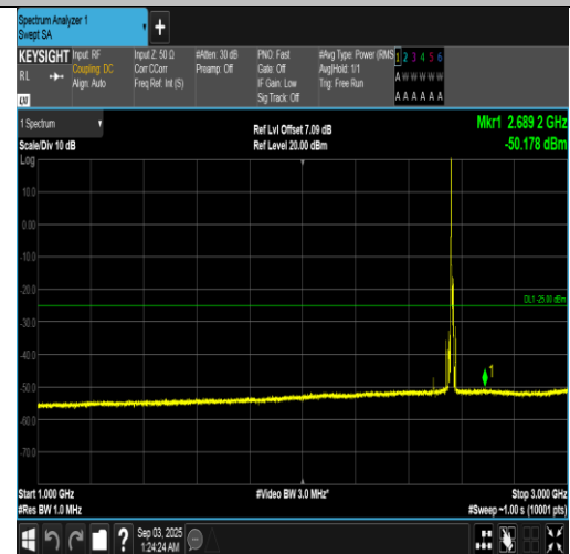
Band7-10MHz-16QAM-21400-1RB#0-1000~3000-PASS
