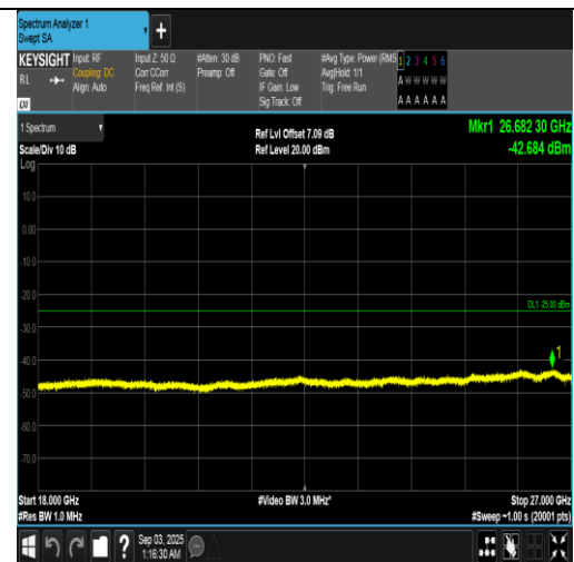
Band7-10MHz-16QAM-21100-1RB#0-18000~27000-PASS
