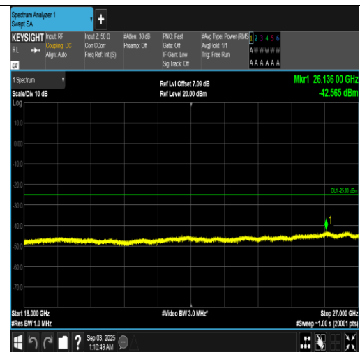
Band7-10MHz-16QAM-20800-1RB#49-18000~27000-PASS
