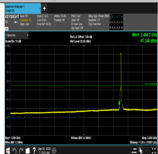
Band7-10MHz-16QAM-20800-50RB#0-1000~3000-PASS
