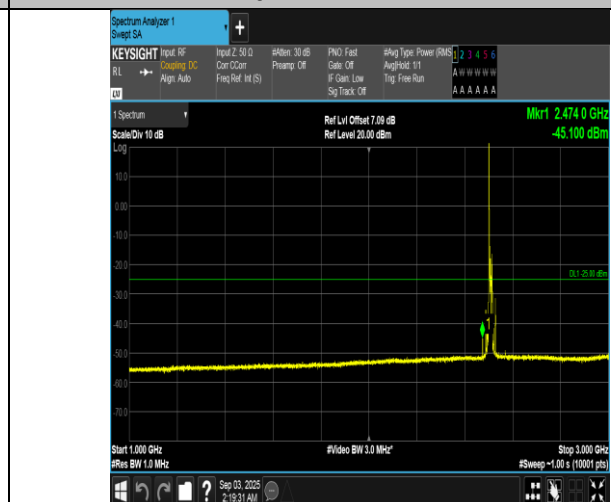
Band7-15MHz-QPSK-20825-1RB#0-1000~3000-PASS
