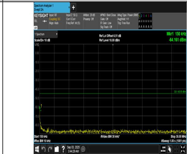
Band7-20MHz-QPSK-21100-1RB#99-0.15~30-PASS
