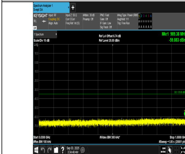
Band7-20MHz-16QAM-20850-1RB#0-30~1000-PASS
