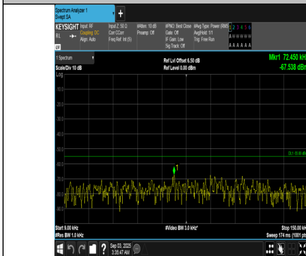
Band7-20MHz-QPSK-20850-1RB#99-0.009~0.15-PASS
