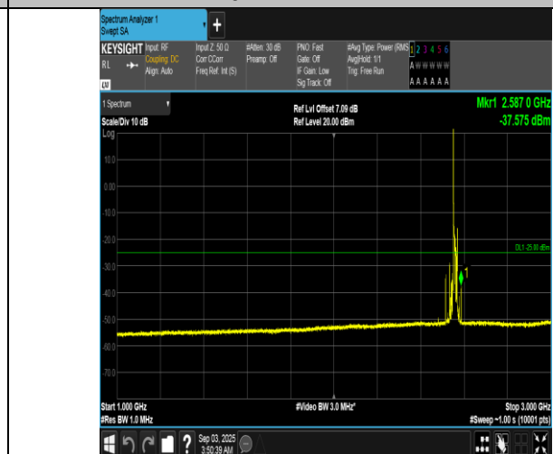
Band7-20MHz-QPSK-21350-1RB#0-1000~3000-PASS
