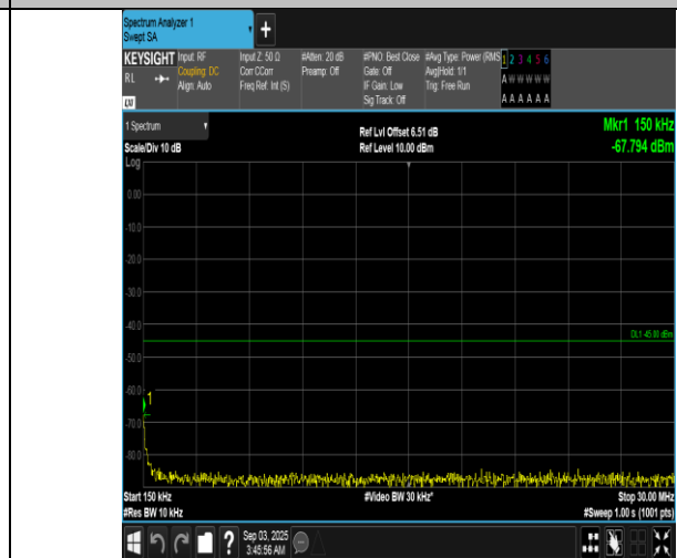
Band7-20MHz-16QAM-21100-1RB#99-0.15~30-PASS
