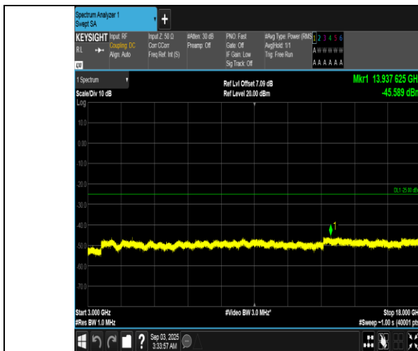
Band7-20MHz-QPSK-20850-1RB#0-3000~18000-PASS
