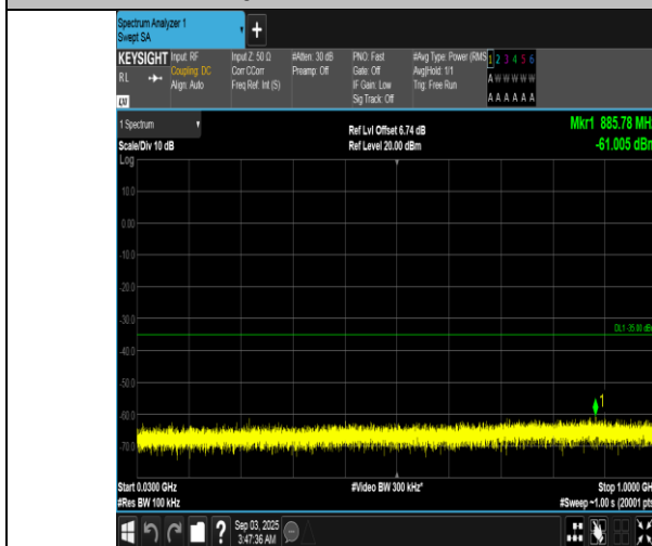
Band7-20MHz-QPSK-21100-100RB#0-30~1000-PASS
