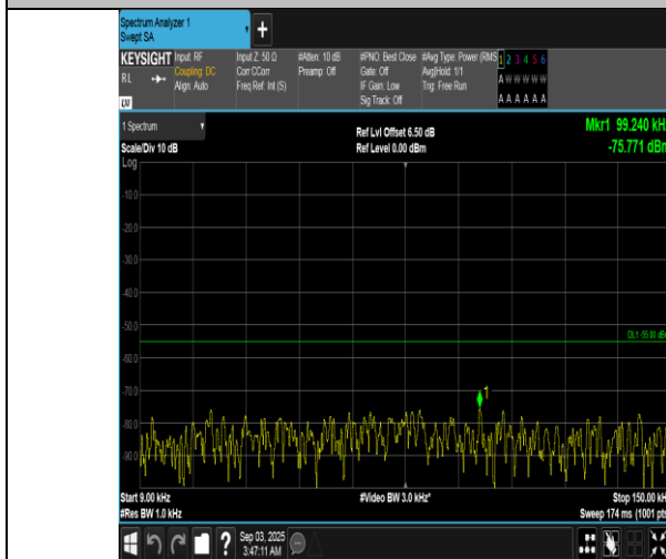
Band7-20MHz-QPSK-21100-100RB#0-0.009~0.15-PASS
