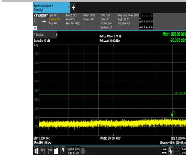
Band7-15MHz-16QAM-21375-75RB#0-30~1000-PASS
