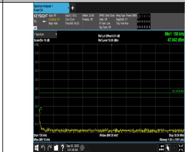
Band7-20MHz-QPSK-21100-1RB#0-0.15~30-PASS
