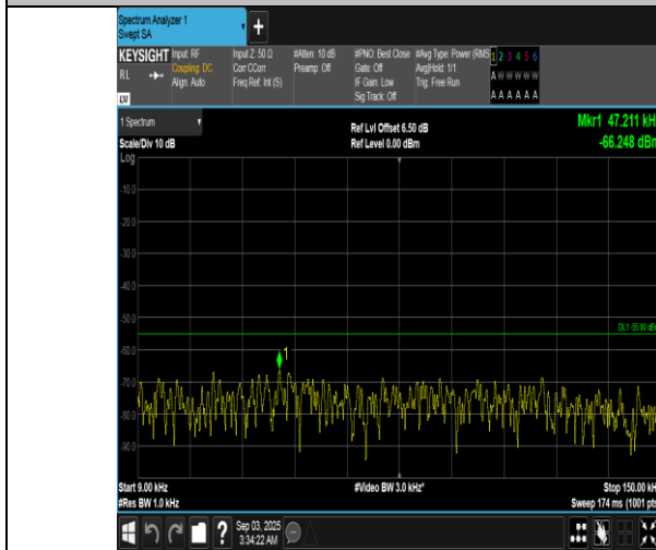
Band7-20MHz-16QAM-20850-1RB#0-0.009~0.15-PASS
