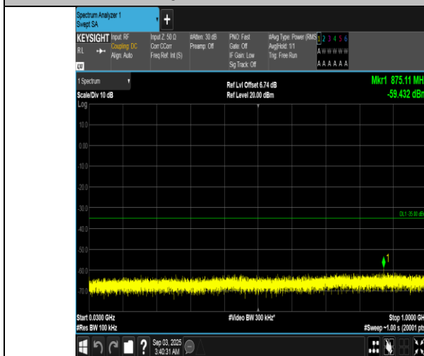
Band7-20MHz-16QAM-20850-100RB#0-30~1000-PASS
