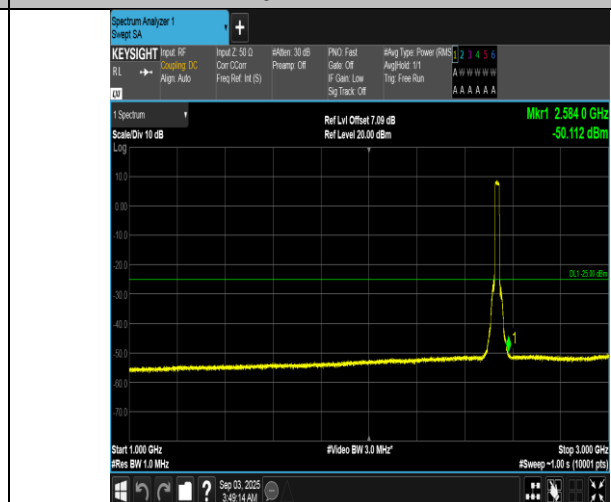
Band7-20MHz-16QAM-21100-100RB#0-1000~3000-PASS
