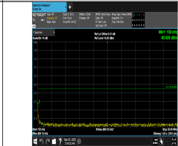
Band7-20MHz-16QAM-20850-1RB#0-0.15~30-PASS
