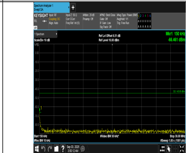
Band7-20MHz-QPSK-21350-1RB#0-0.15~30-PASS
