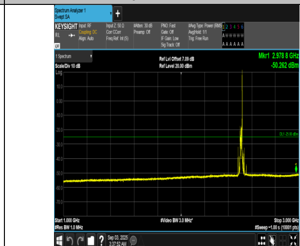
Band7-20MHz-16QAM-20850-1RB#99-1000~3000-PASS
