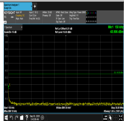
Band7-20MHz-16QAM-21100-1RB#0-0.15~30-PASS
