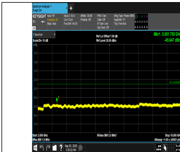
Band7-20MHz-16QAM-20850-1RB#0-3000~18000-PASS
