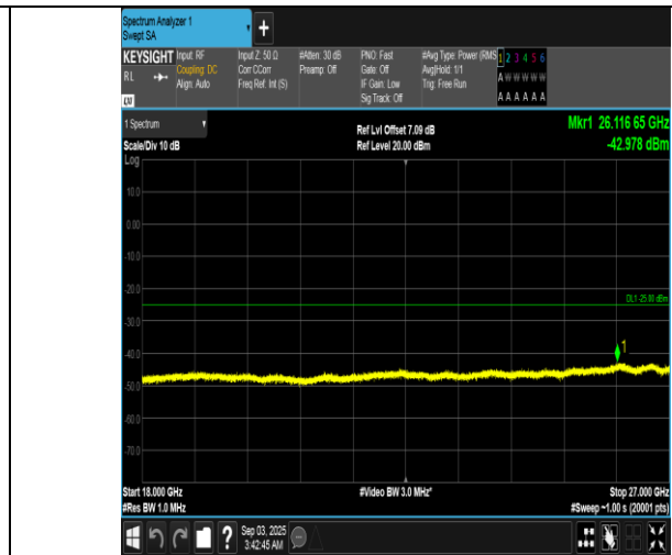
Band7-20MHz-QPSK-21100-1RB#0-18000~27000-PASS
