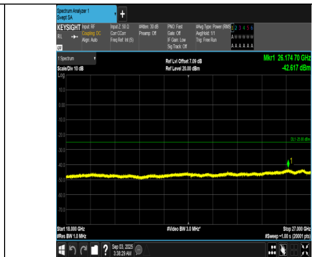
Band7-20MHz-16QAM-20850-1RB#99-18000~27000-PASS
