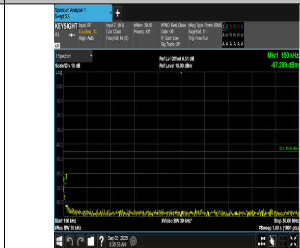
Band7-20MHz-QPSK-20850-1RB#99-0.15~30-PASS
