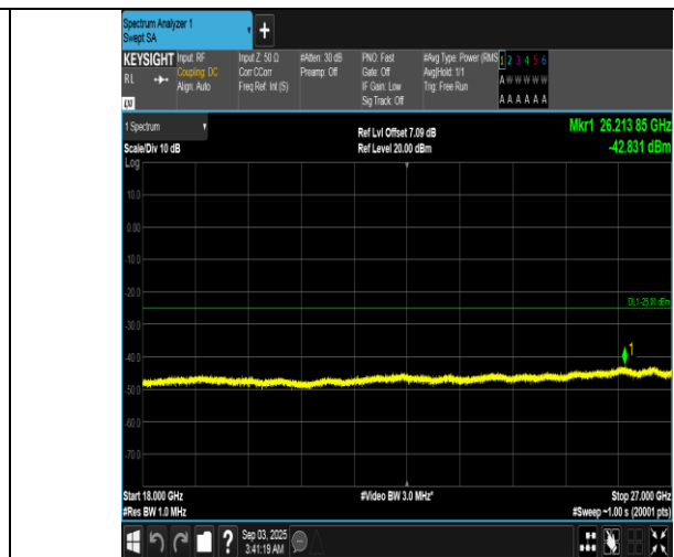
Band7-20MHz-16QAM-20850-100RB#0-18000~27000-PASS
