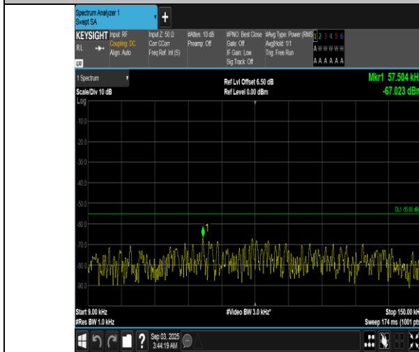
Band7-20MHz-QPSK-21100-1RB#99-0.009~0.15-PASS
