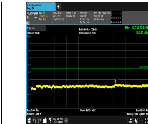
Band7-20MHz-16QAM-21100-1RB#0-3000~18000-PASS
