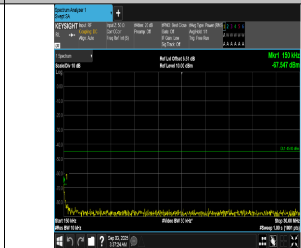
Band7-20MHz-16QAM-20850-1RB#99-0.15~30-PASS
