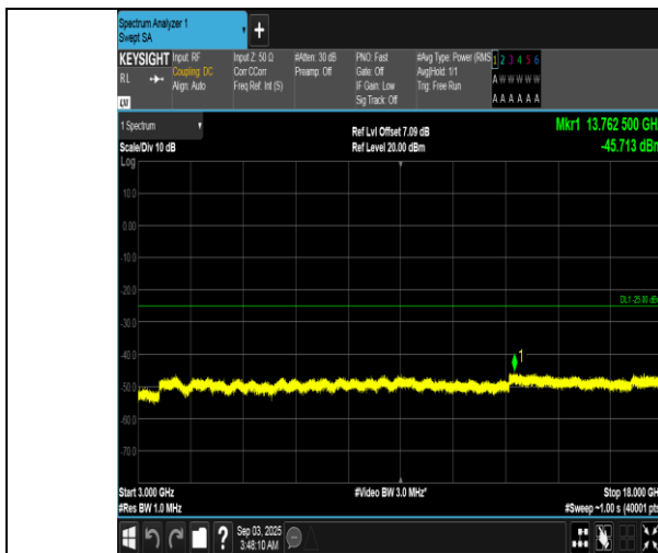
Band7-20MHz-QPSK-21100-100RB#0-3000~18000-PASS
