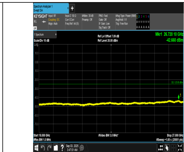
Band7-20MHz-16QAM-21100-1RB#99-18000~27000-PASS
