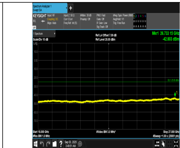
Band7-20MHz-16QAM-21100-100RB#0-18000~27000-PASS
