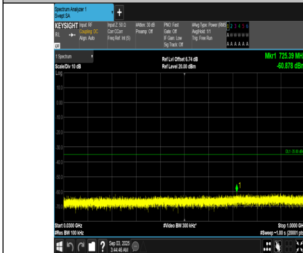
Band7-20MHz-QPSK-21100-1RB#99-30~1000-PASS
