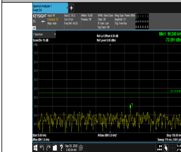
Band7-20MHz-16QAM-20850-100RB#0-0.009~0.15-PASS
