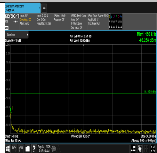
Band7-20MHz-QPSK-21100-100RB#0-0.15~30-PASS
