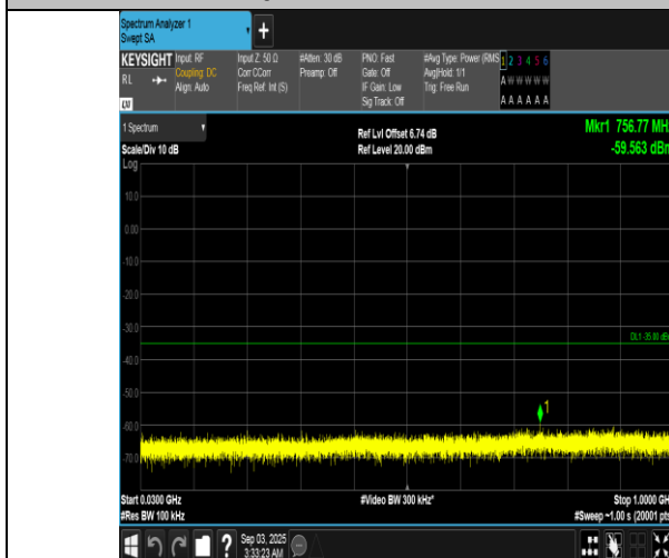
Band7-20MHz-QPSK-20850-1RB#0-30~1000-PASS
