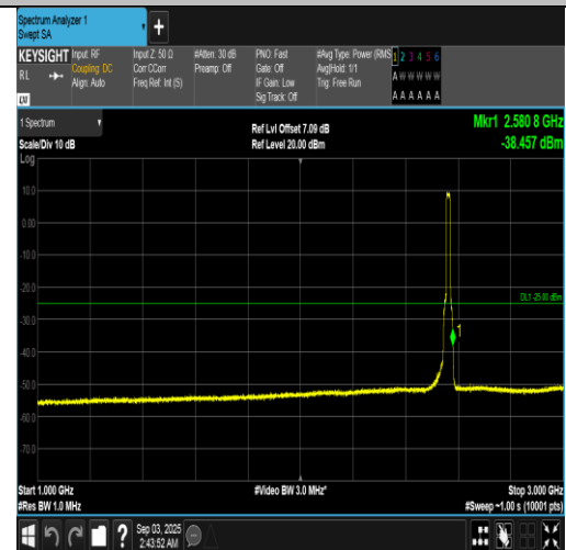
Band7-15MHz-16QAM-21375-75RB#0-1000~3000-PASS
