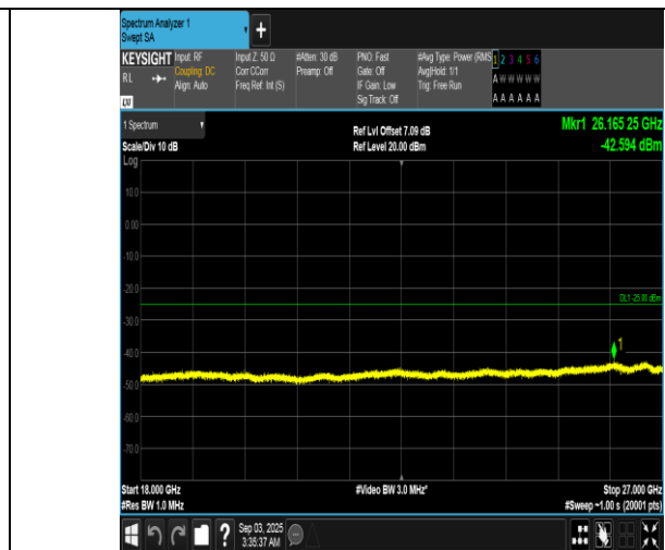
Band7-20MHz-16QAM-20850-1RB#0-18000~27000-PASS
