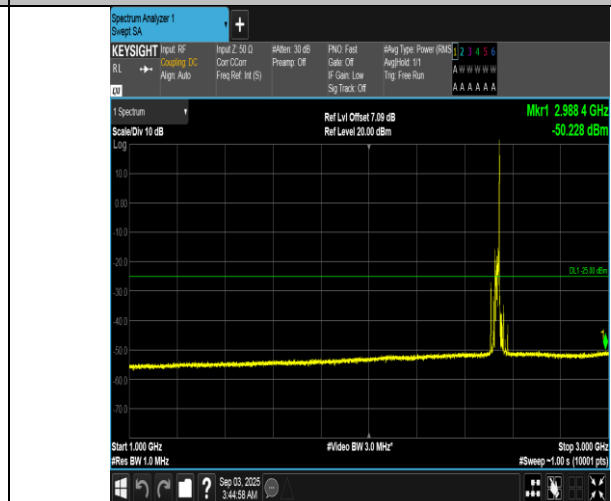
Band7-20MHz-QPSK-21100-1RB#99-1000~3000-PASS
