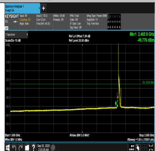
Band7-20MHz-QPSK-20850-1RB#0-1000~3000-PASS
