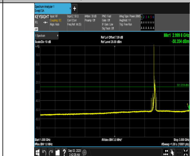
Band7-20MHz-QPSK-21100-1RB#0-1000~3000-PASS
