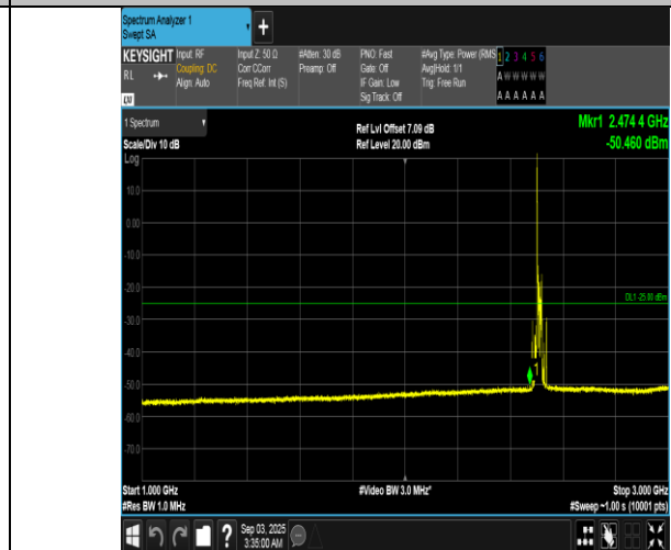
Band7-20MHz-16QAM-20850-1RB#0-1000~3000-PASS
