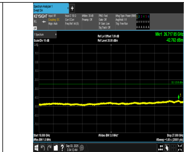
Band7-20MHz-QPSK-20850-1RB#0-18000~27000-PASS
