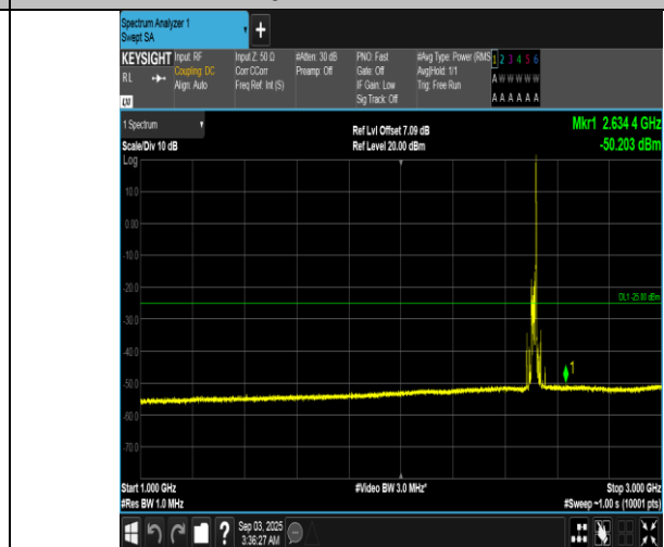
Band7-20MHz-QPSK-20850-1RB#99-1000~3000-PASS
