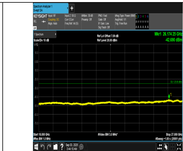
Band7-20MHz-16QAM-21100-1RB#0-18000~27000-PASS
