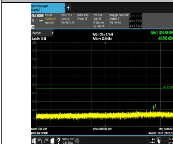
Band7-20MHz-QPSK-21100-1RB#0-30~1000-PASS
