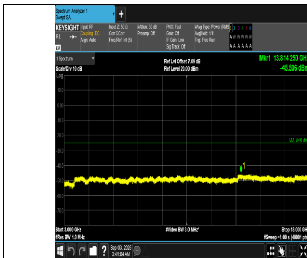
Band7-20MHz-16QAM-20850-100RB#0-3000~18000-PASS
