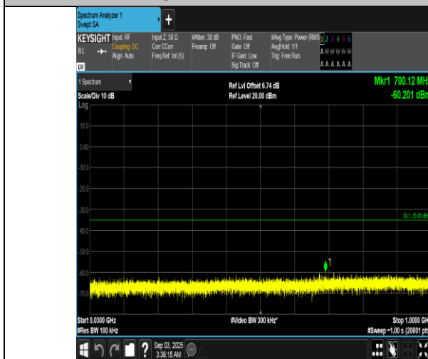
Band7-20MHz-QPSK-20850-1RB#99-30~1000-PASS
