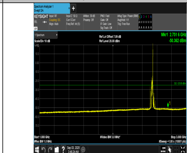
Band7-20MHz-16QAM-21100-1RB#99-1000~3000-PASS
