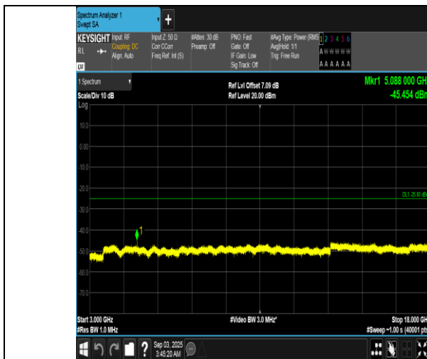
Band7-20MHz-QPSK-21100-1RB#99-3000~18000-PASS
