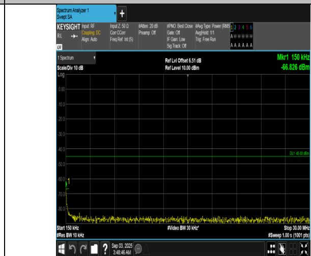
Band7-20MHz-16QAM-21100-100RB#0-0.15~30-PASS
