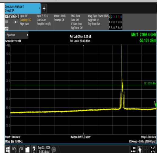
Band7-20MHz-16QAM-21100-1RB#0-1000~3000-PASS
