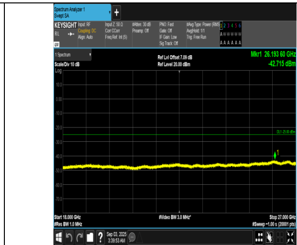
Band7-20MHz-QPSK-20850-100RB#0-18000~27000-PASS
