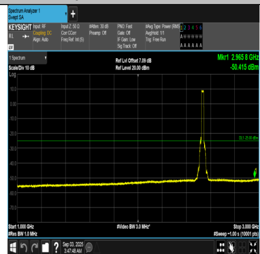
Band7-20MHz-QPSK-21100-100RB#0-1000~3000-PASS
