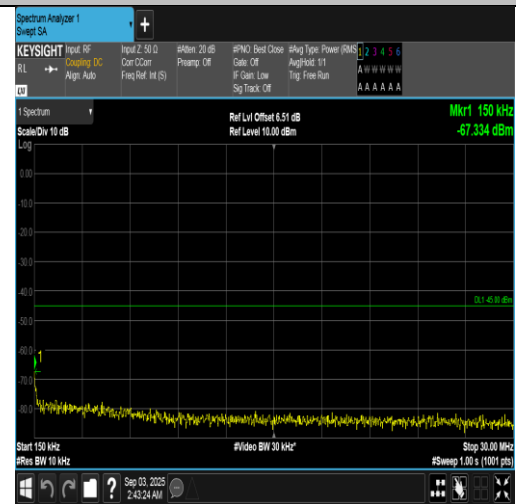
Band7-15MHz-16QAM-21375-75RB#0-0.15~30-PASS
