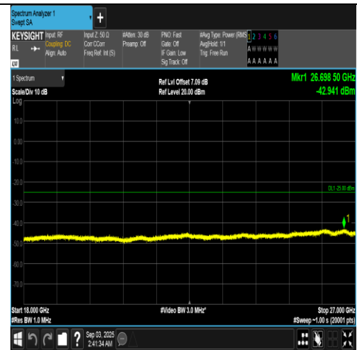
Band7-15MHz-16QAM-21375-1RB#74-18000~27000-PASS
