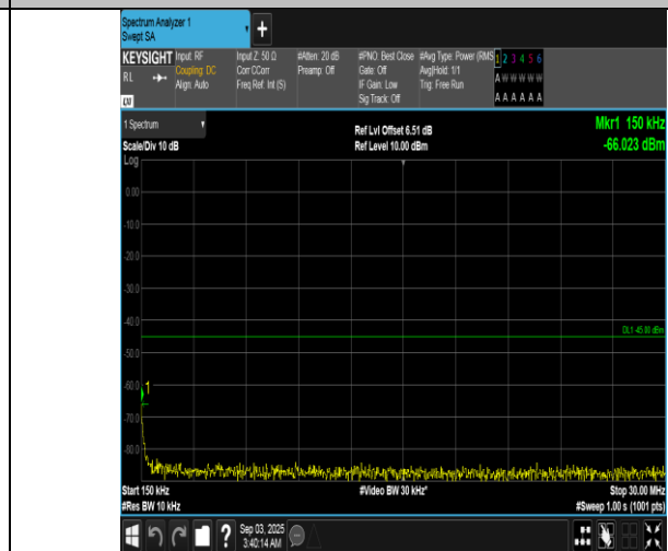
Band7-20MHz-16QAM-20850-100RB#0-0.15~30-PASS
