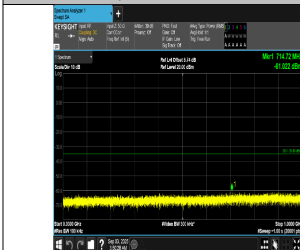
Band7-20MHz-QPSK-21350-1RB#0-30~1000-PASS
