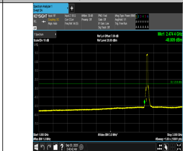
Band7-20MHz-16QAM-20850-100RB#0-1000~3000-PASS
