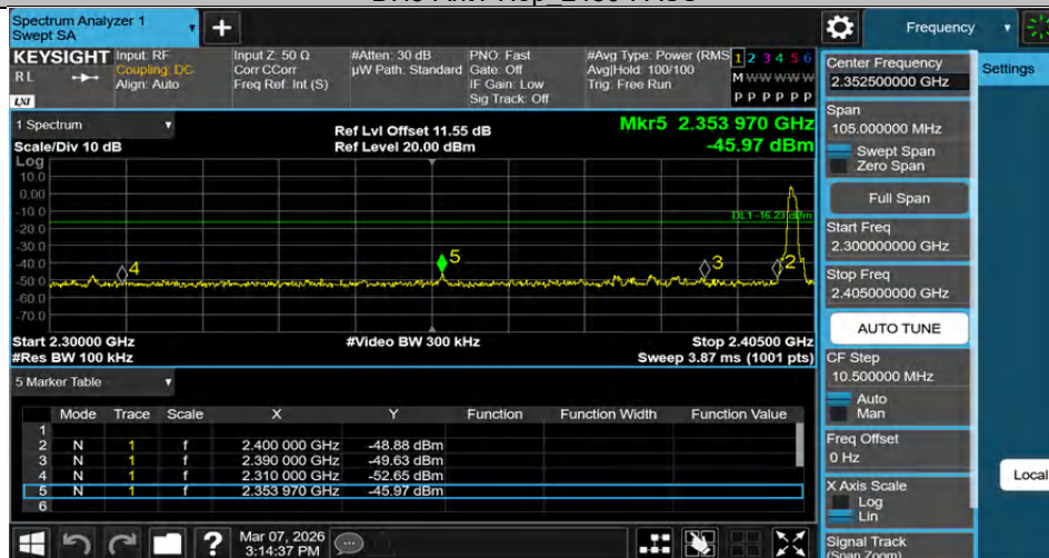
2DH5-Ant1-2402-PASS
