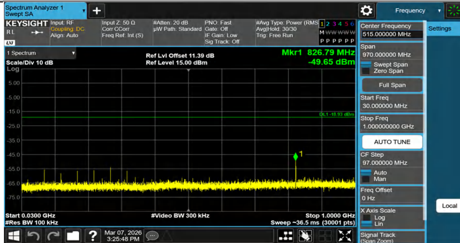
3DH5-Ant1-2480-30~1000-PASS
