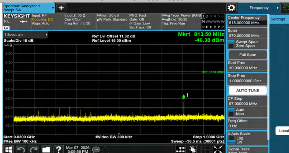
DH5-Ant1-2441-30~1000-PASS
