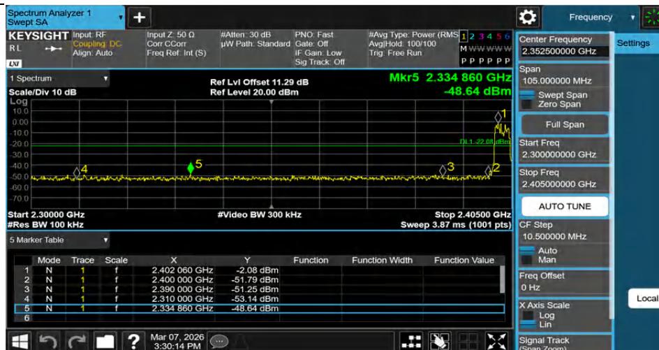
2DH5-Ant1-Hop_2402-PASS
