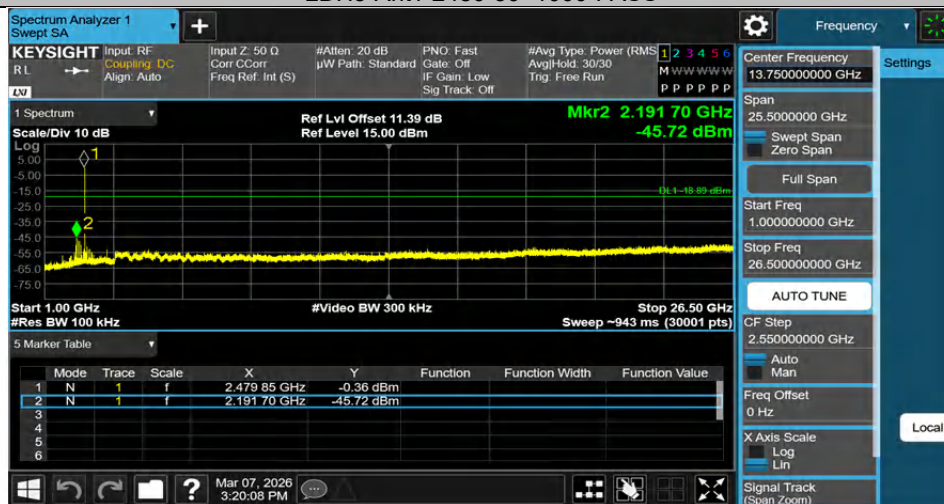
2DH5-Ant1-2480-1000~26500-PASS
