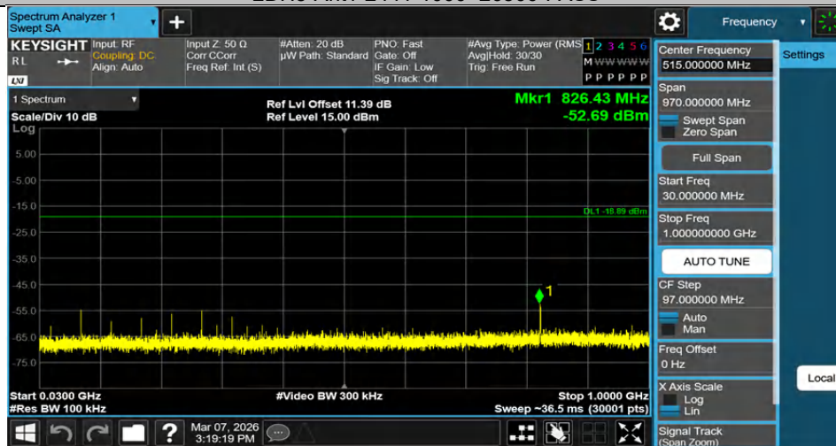
2DH5-Ant1-2480-30~1000-PASS
