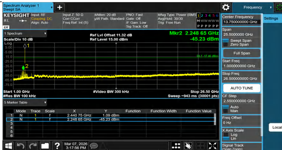
2DH5-Ant1-2441-1000~26500-PASS
