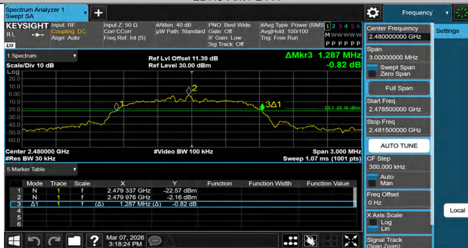
2DH5-Ant1-2480
