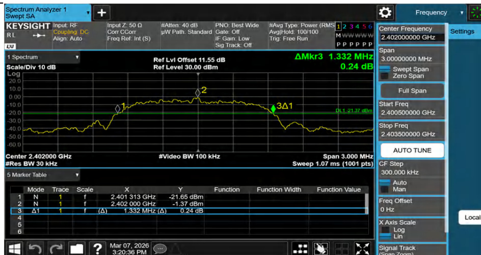
3DH5-Ant1-2402
