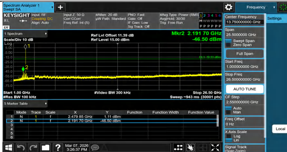
3DH5-Ant1-2480-1000~26500-PASS
