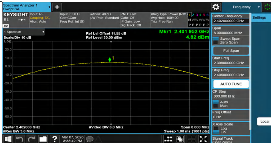
2DH5-Ant1-2402-PASS
