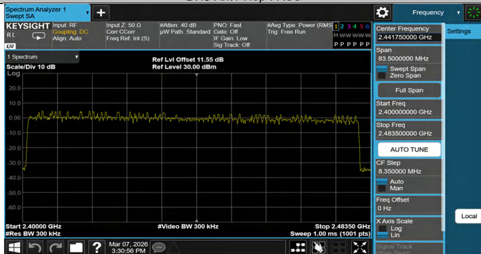
2DH5-Ant1-Hop-PASS
