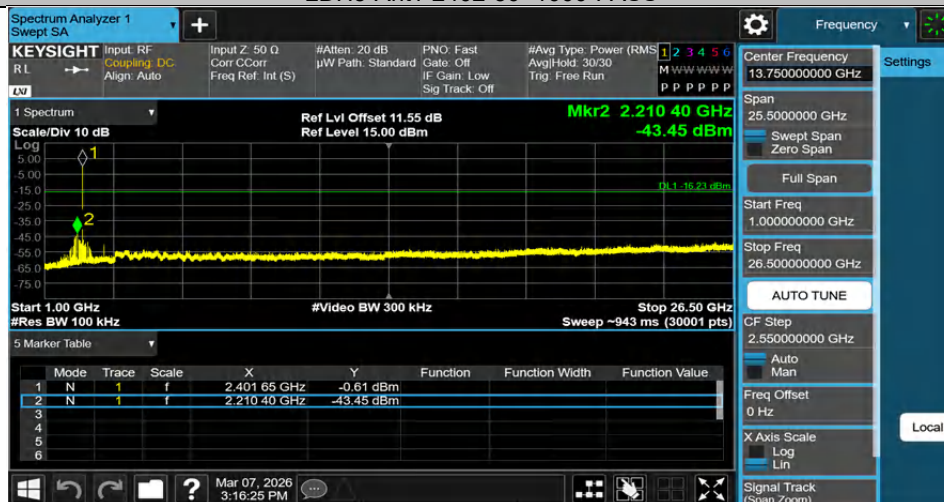
2DH5-Ant1-2402-1000~26500-PASS
