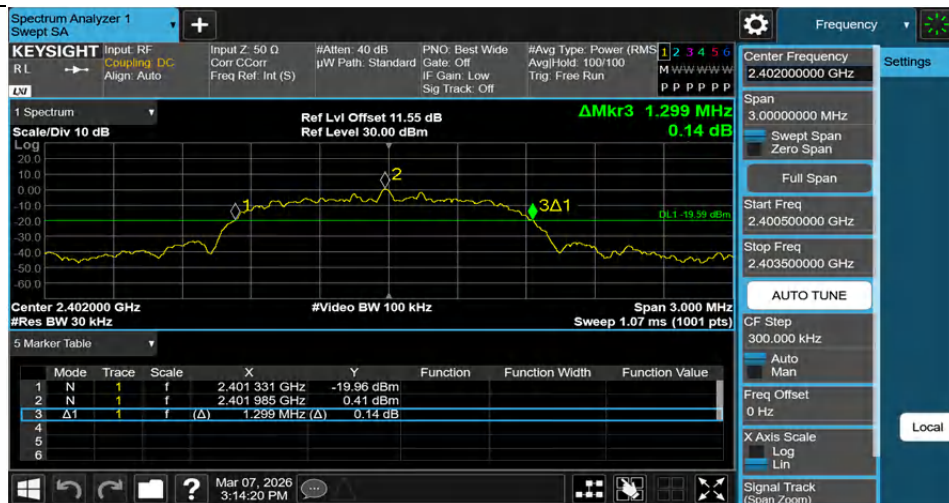
2DH5-Ant1-2402
