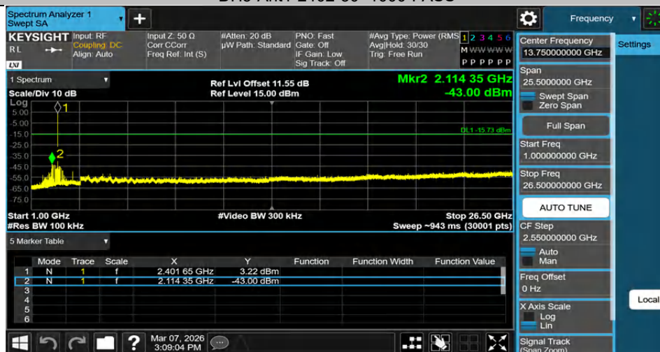
DH5-Ant1-2402-1000~26500-PASS
