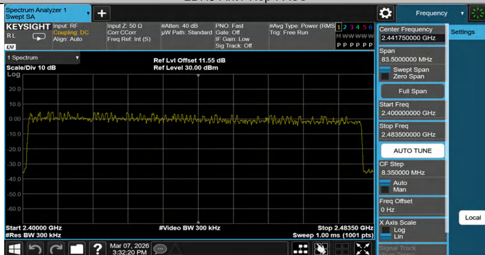
3DH5-Ant1-Hop-PASS
