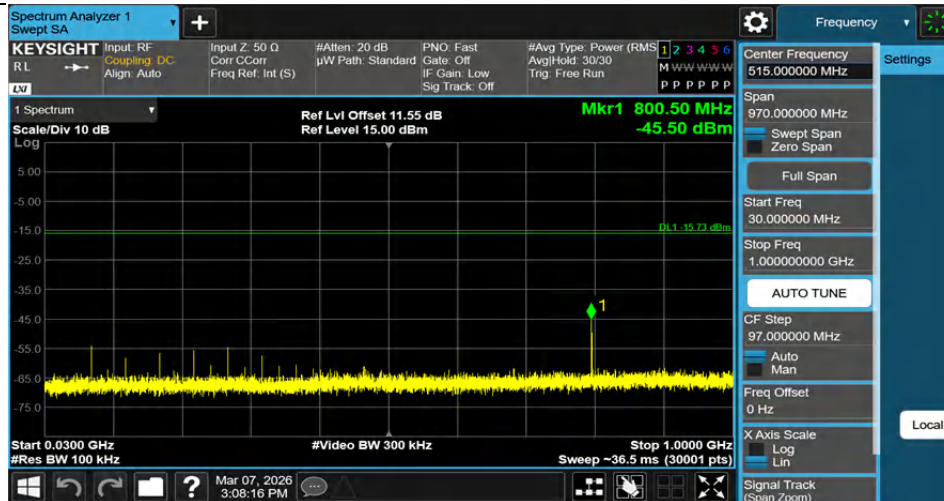
DH5-Ant1-2402-30~1000-PASS
