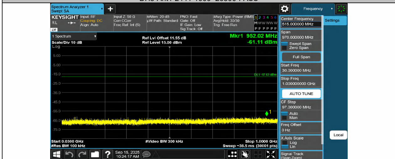
DH5-Ant1-2480-30~1000-PASS
