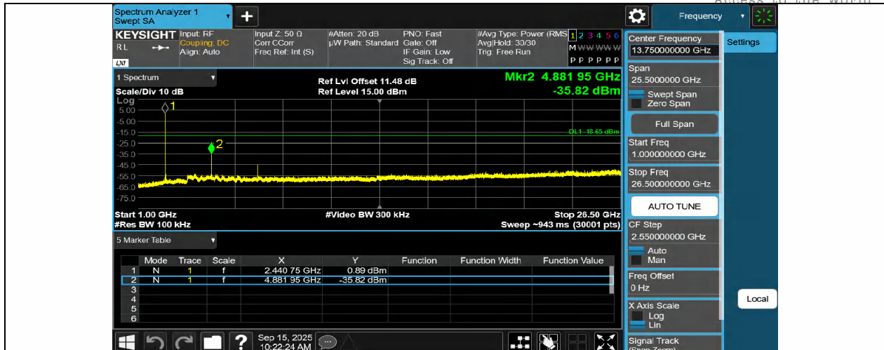
DH5-Ant1-2441-1000~26500-PASS
