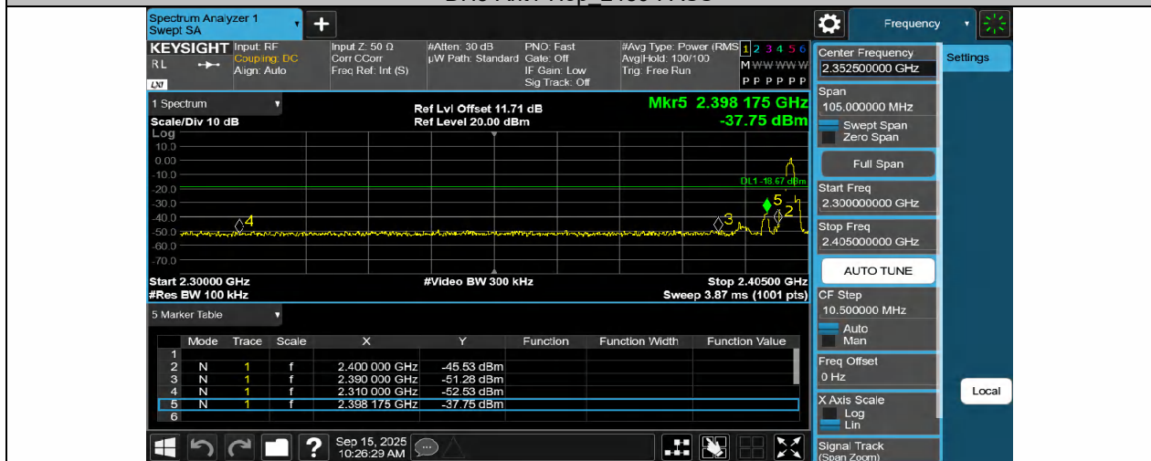
2DH5-Ant1-2402-PASS
