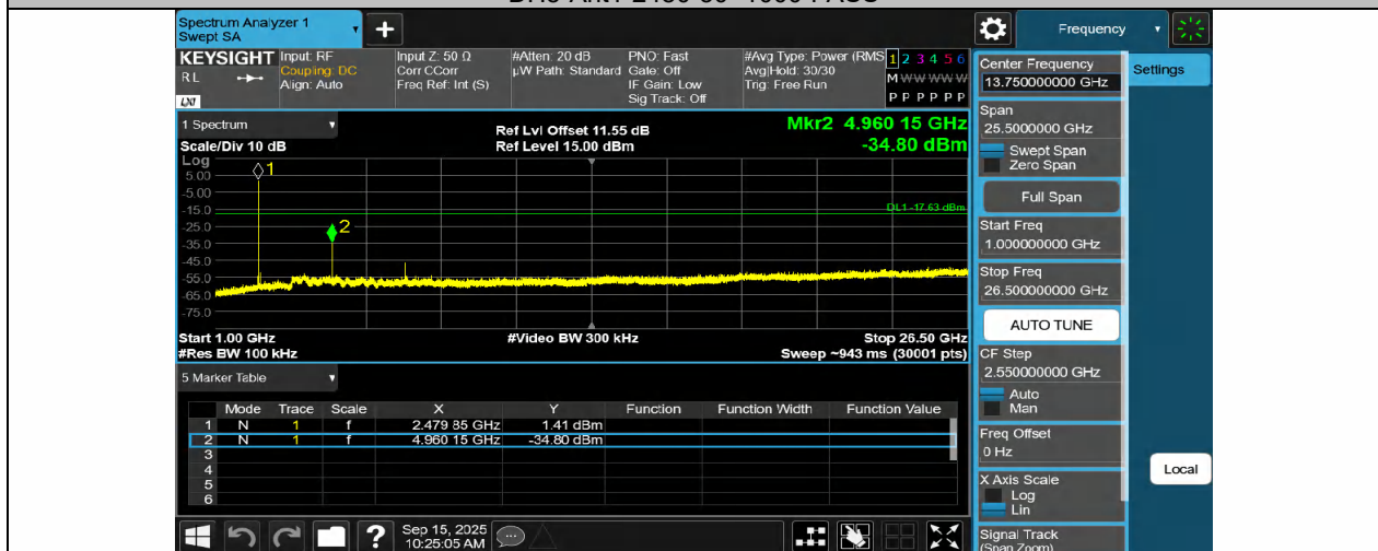
DH5-Ant1-2480-1000~26500-PASS
