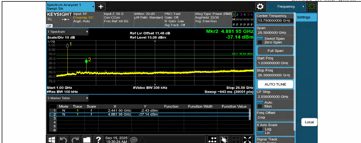
2DH5-Ant1-2441-1000~26500-PASS
