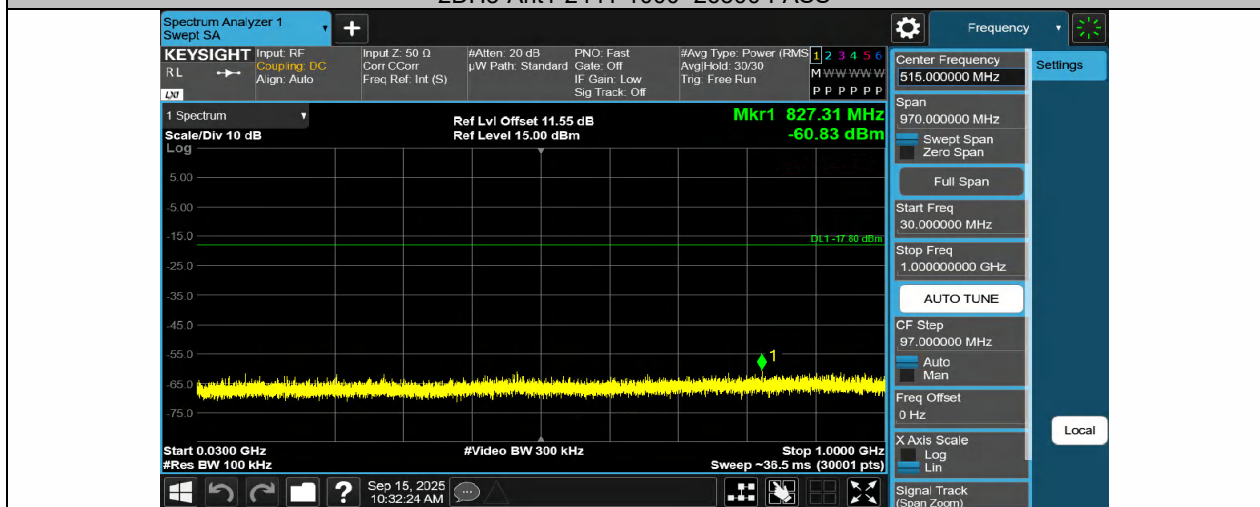
2DH5-Ant1-2480-30~1000-PASS
