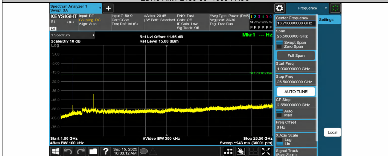
2DH5-Ant1-2480-1000~26500-PASS
