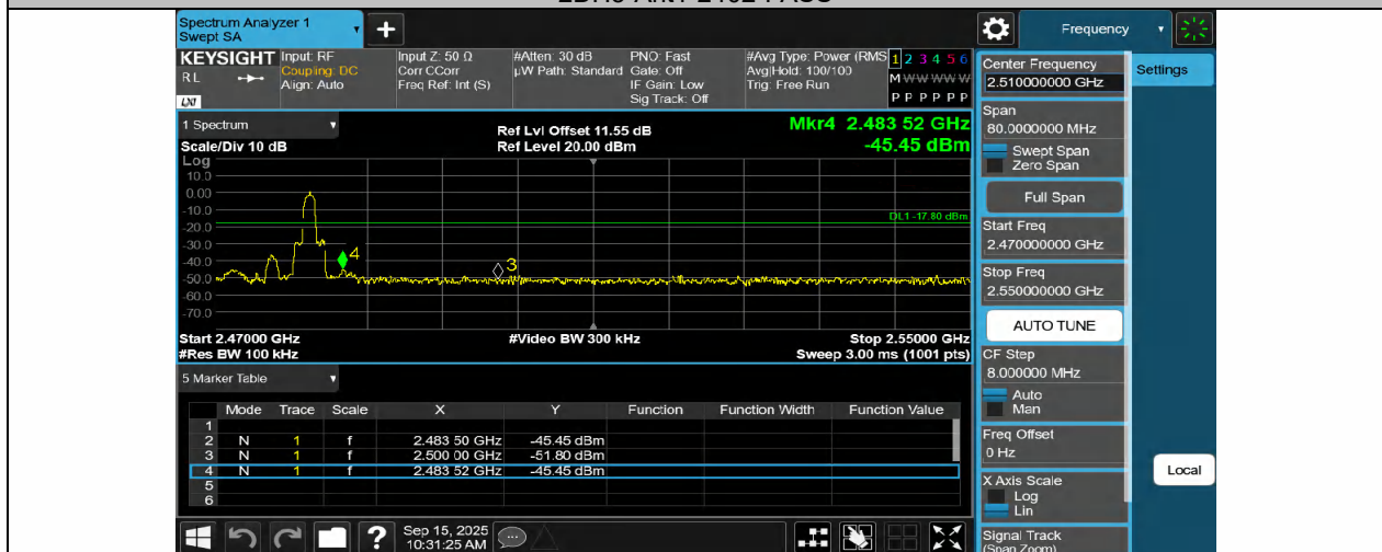
2DH5-Ant1-2480-PASS
