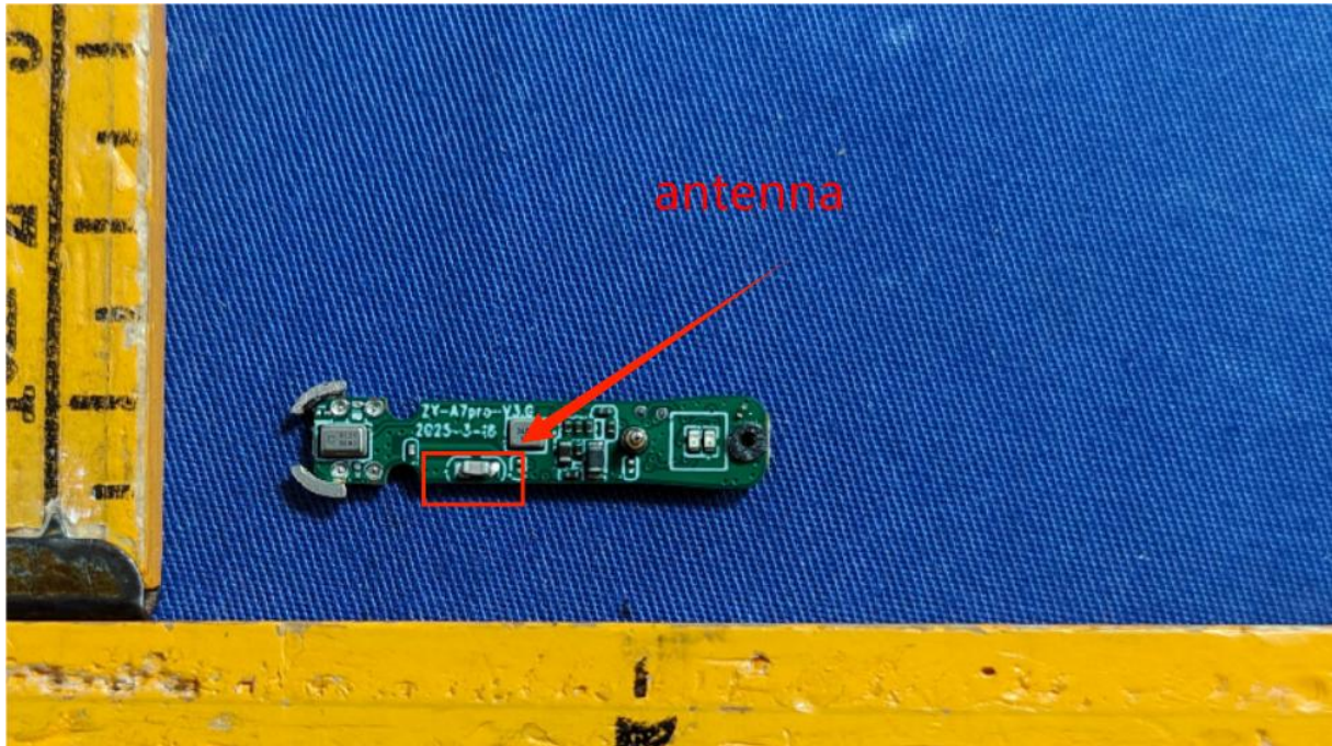
Right earphone PCB view
