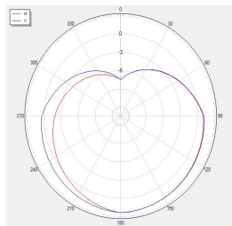
BLUETOOTH_Trp_H39 Polar
