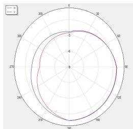
BLUETOOTH_Trp_H78 Polar
