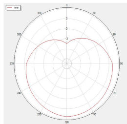
BLUETOOTH_Trp_H39 Total
