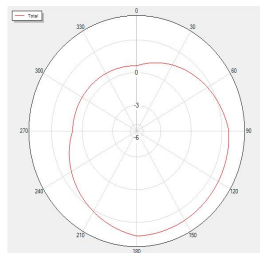
BLUETOOTH_Trp_H78 Total
