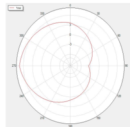
BLUETOOTH_Trp_V78 Total
