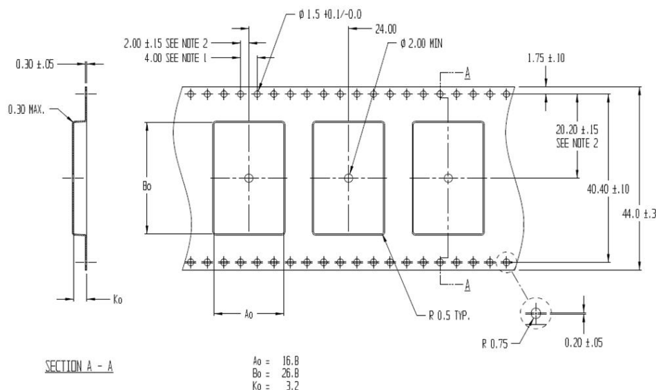
Figure 9: SARA-R4 series modules tape
