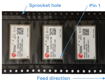
Figure 8: Orientation of SARA-R4 series modules on tape
