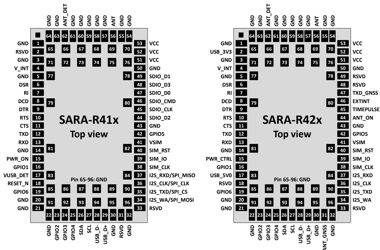
Figure 6: SARA-R4 series pin assignment (top view)
