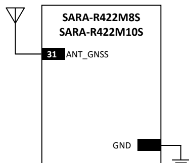
Figure 42: Minimum circuit with GNSS passive antenna
