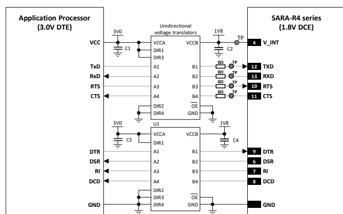
Figure 55: UART interface application circuit with complete V.24 link in DTE/DCE serial communication (3.0 V DTE)
