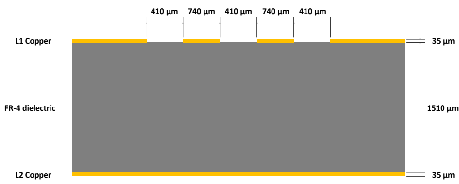
Figure 67: Example of USB line design, with Z_0 = 90\ \Omega and Z_{CM} = 30\ \Omega , for the described 2-layer board layout
