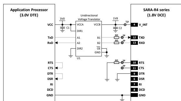
Figure 63: UART application circuit with a partial V.24 link (3-wire) in DTE/DCE serial communication (3.0 V DTE)
