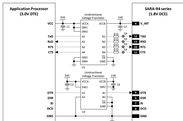
Figure 57: UART application circuit with partial V.24 link (6-wire) in DTE/DCE serial communication (3.0 V DTE)
