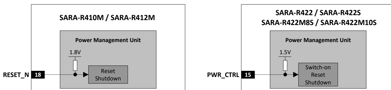
Figure 19: RESET_N and PWR_CTRL input pins description
