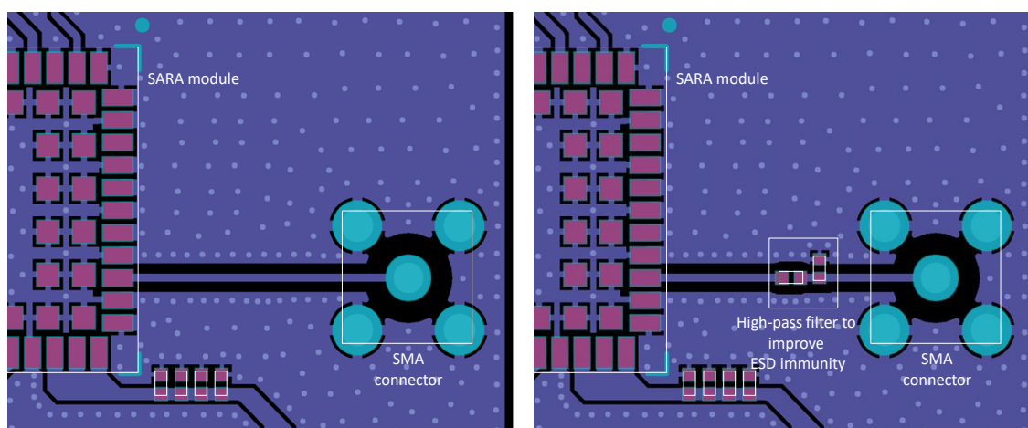
Figure 40: Example of circuit and layout for ANT RF circuits on the application board
