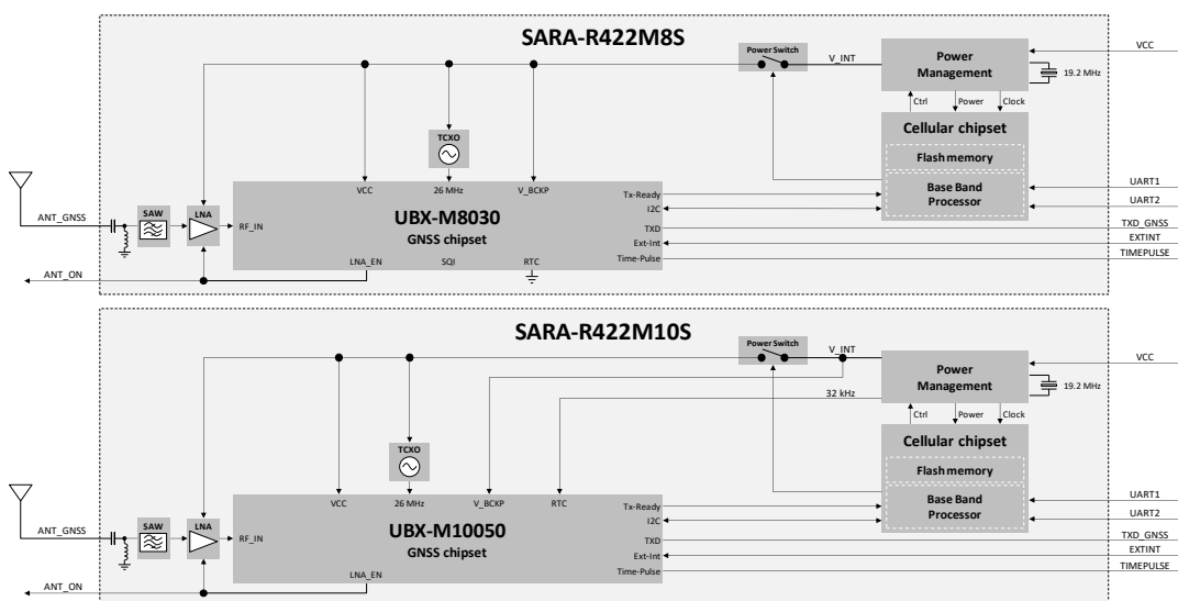
Figure 6: SARA-R422M8S and SARA-R422M10S modules GNSS section block diagram
