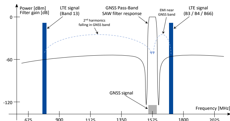
Figure 45: EMI due to Tx in LTE B3, B4, B66 low channels (1710 MHz) adjacent to GNSS frequency range (1561 to 1610 MHz), or due to Tx in LTE B13 high channels (787 MHz) with harmonics falling into the GNSS frequency range
