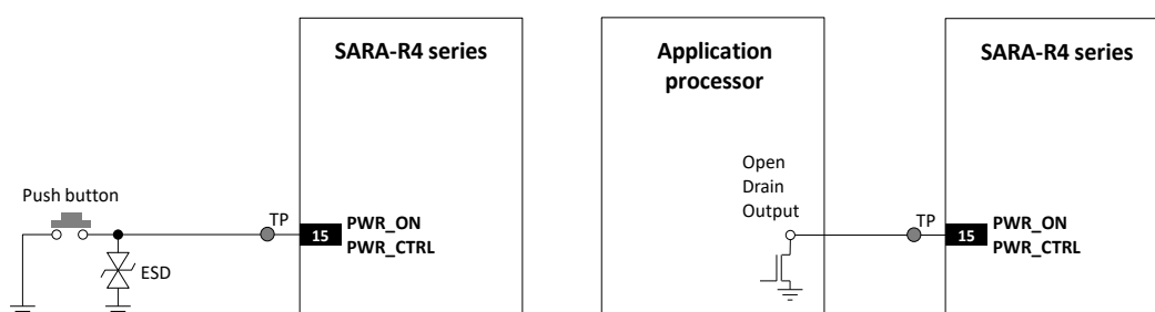
Figure 35: PWR_ON / PWR_CTRL circuits using a push button and an open drain output of an external processor
