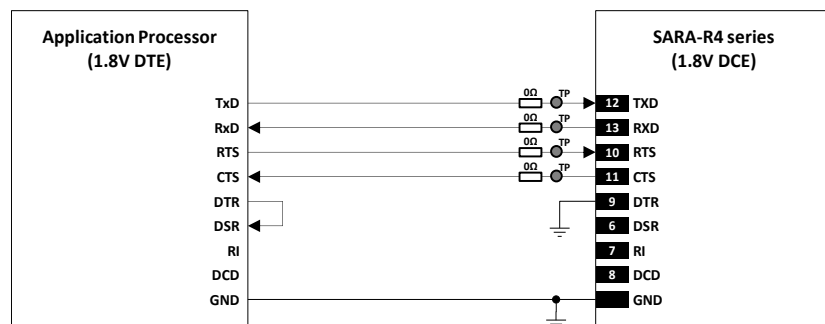
Figure 58: UART circuit with partial V.24 link (5-wire) in the DTE/DCE serial communication (1.8V DTE)
