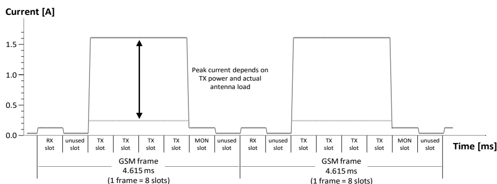
Figure 12: VCC current consumption profile versus time during a GPRS multi-slot class 12 call (4 TX slots, 1 RX slot)
