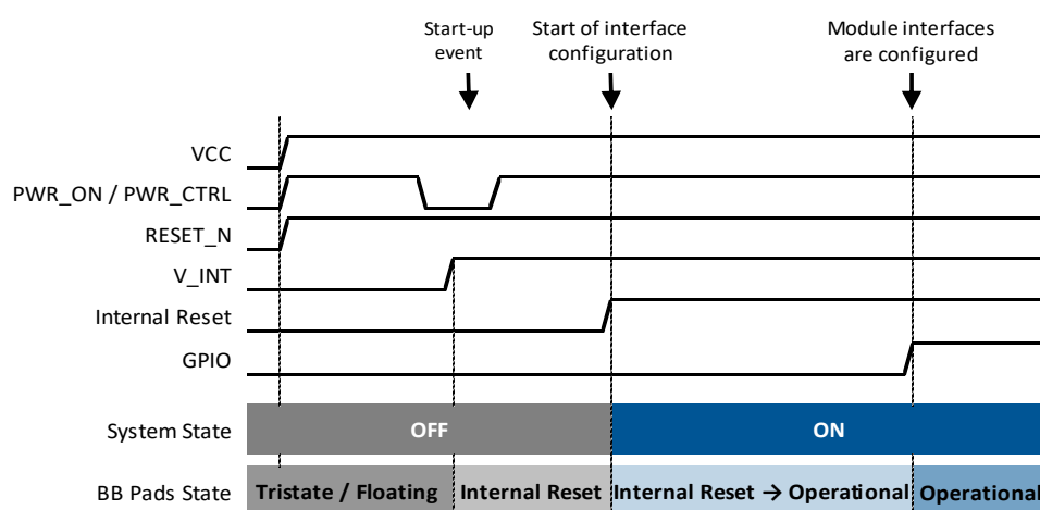
Figure 16: SARA-R4 series switch-on sequence description
