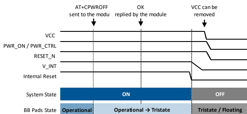
Figure 17: SARA-R4 series modules switch-off sequence by means of AT+CPWROFF command
