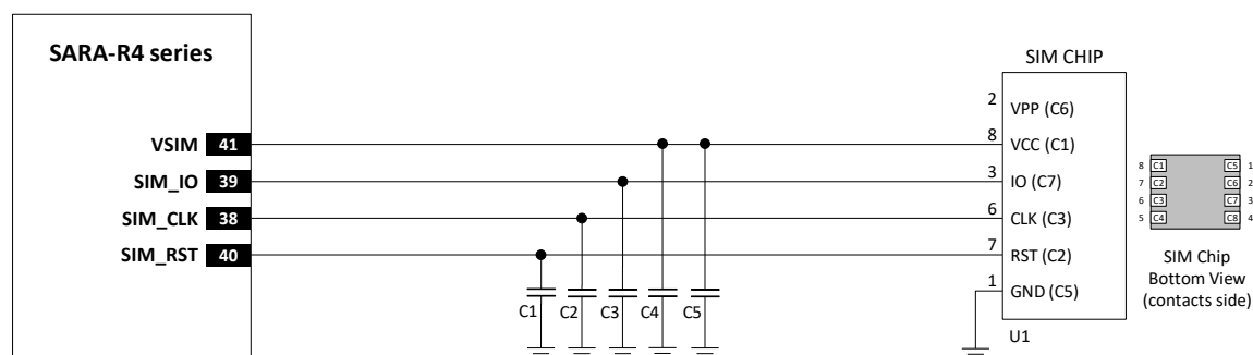
Figure 52: Application circuit to connect a single Surface-Mounted SIM chip, with SIM detection not implemented
