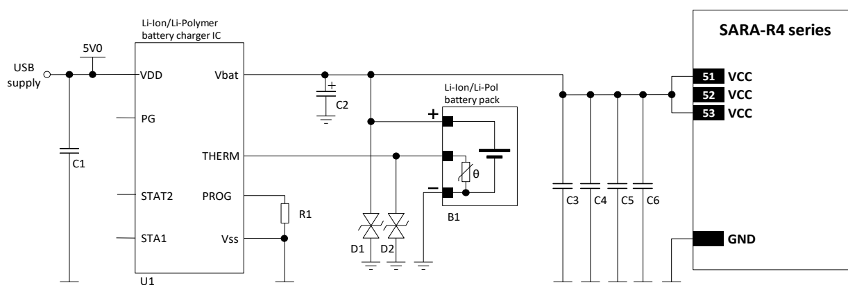
Figure 28: Li-Ion (or Li-Polymer) battery charging application circuit
