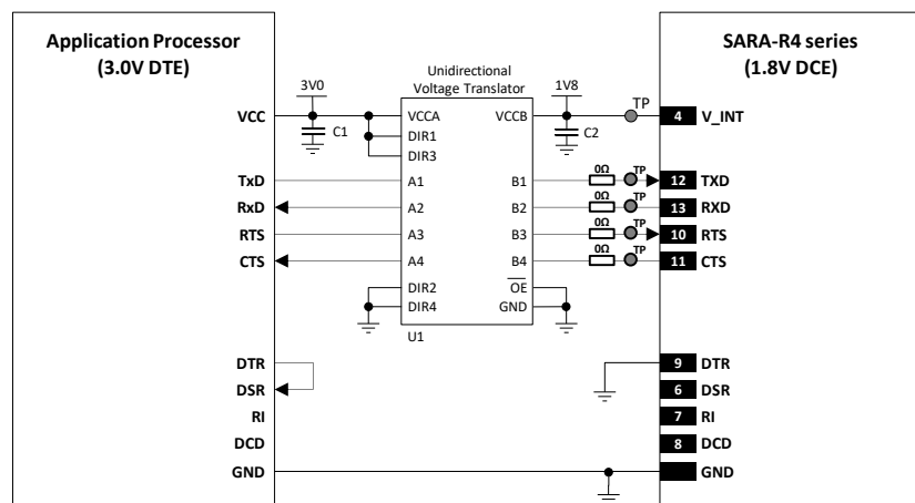
Figure 59: UART circuit with a partial V.24 link (5-wire) in DTE/DCE serial communication (3.0 V DTE)
