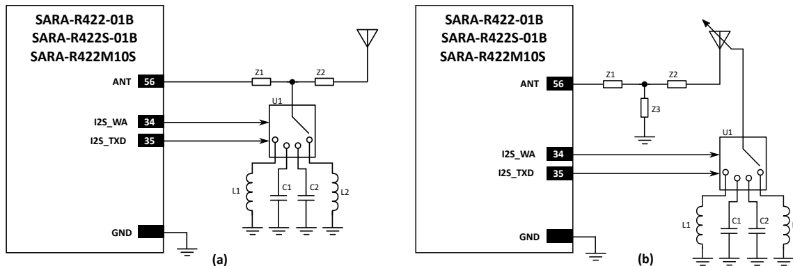
Figure 50: Examples of schematics for cellular antenna dynamic impedance tuning (a) and aperture tuning (b).
