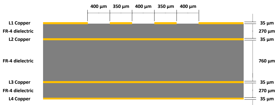
Figure 66: Example of USB line design, with Z_0 = 90\ \Omega and Z_{CM} = 30\ \Omega , for the described 4-layer board layout
