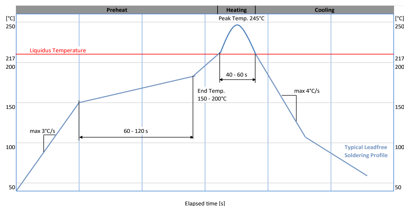
Figure 74: Recommended soldering profile
