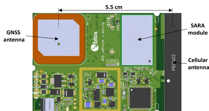
Figure 47: PCB top rendering for the B36 blueprint with annotated distance between cellular and GNSS antennas
