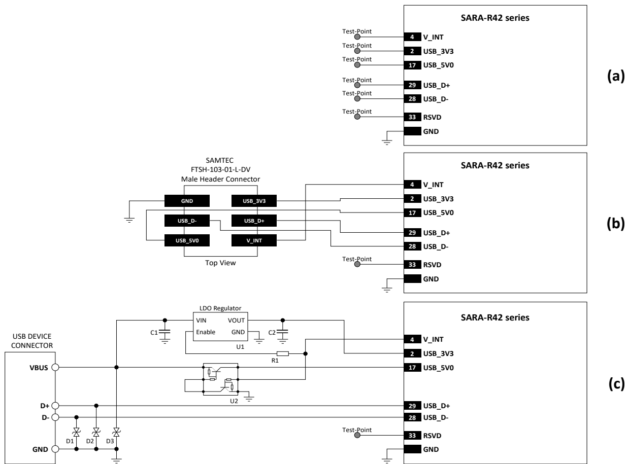
Figure 65: USB application circuits for SARA-R422, SARA-R422S, SARA-R422M8S and SARA-R422M10S modules
