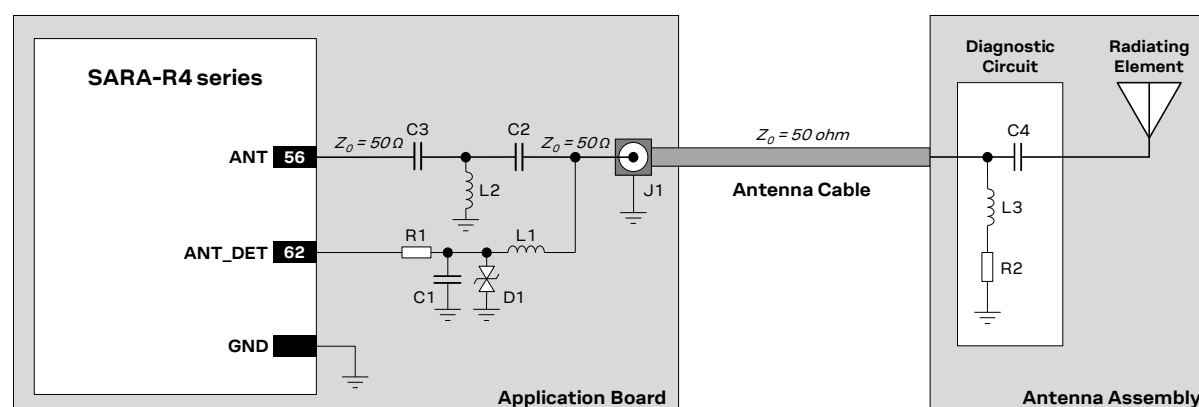
Figure 48: Schematic for antenna detection circuit on application PCB and diagnostic circuit on antenna assembly
