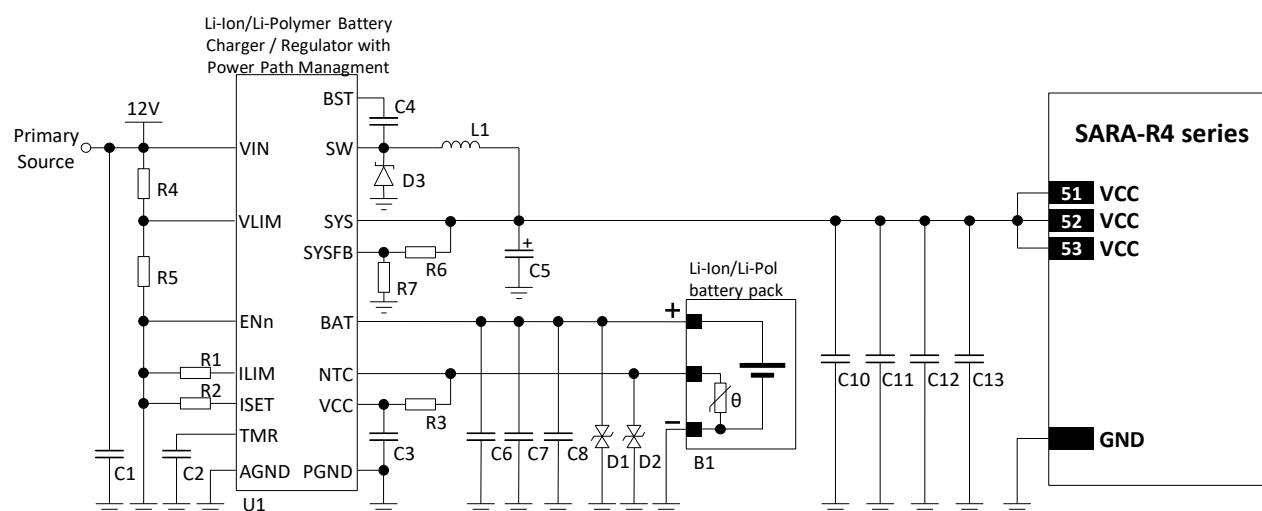
Figure 30: Li-Ion (or Li-Polymer) battery charging and power path management application circuit
