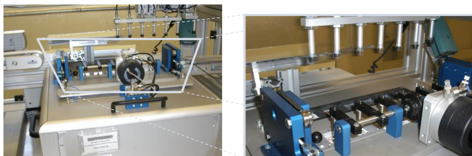
Figure 75: Automatic test equipment for module tests
