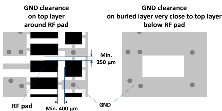
Figure 37: GND keep-out area on top layer around ANT / ANT_GNSS pad and on very close buried layer below pad
