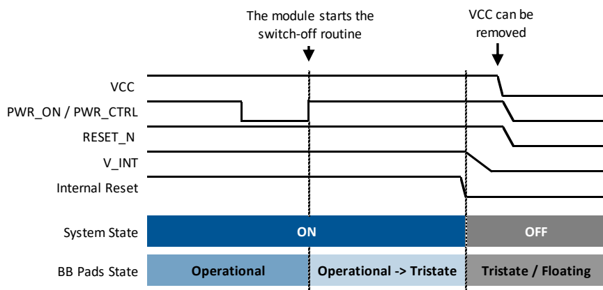
Figure 18: SARA-R4 series modules switch-off sequence by means of PWR_ON / PWR_CTRL pin
