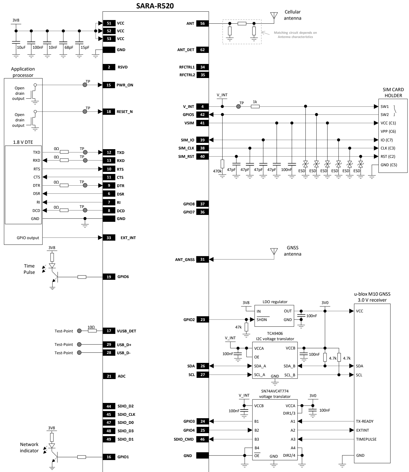
Figure 72: Example schematic diagram integrating a SARA-R520 module
