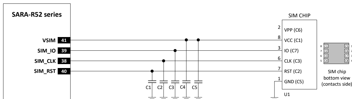
Figure 47: Application circuits for the connection to a single Surface-Mounted SIM chip
