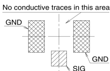
Figure 36: U.FL surface mounted connector mounting pattern layout
