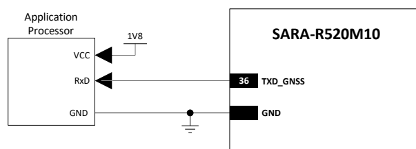
Figure 68: Application circuit for GNSS peripheral UART data output pin
