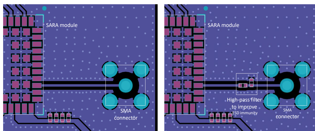
Figure 35: Example of circuit and layout for ANT RF circuits on the application board
