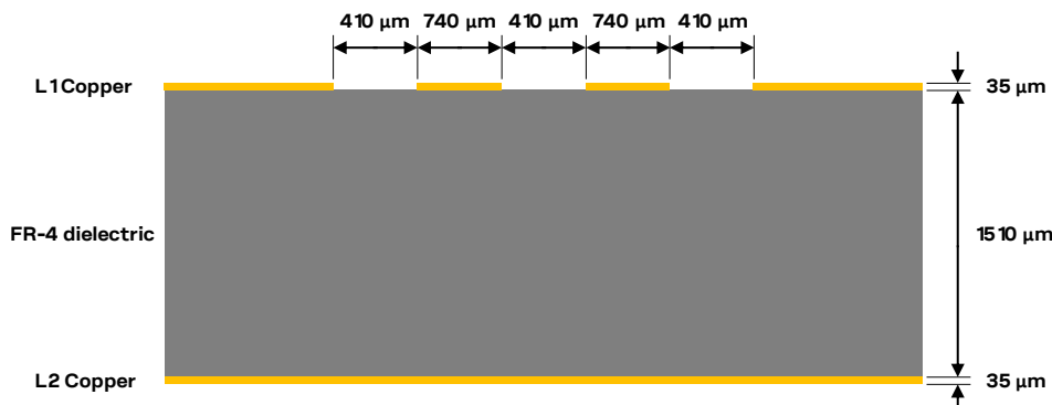
Figure 64: Example of USB line design, with Z_0 = 90 \Omega and Z_{CM} = 30 \Omega , for the described 2-layer PCB layout
