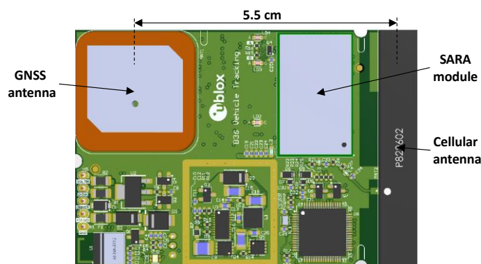
Figure 42: PCB top rendering for the B36 blueprint with annotated distance between cellular and GNSS antennas
