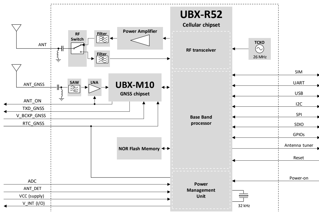
Figure 2: SARA-R520M10 module simplified block diagram
