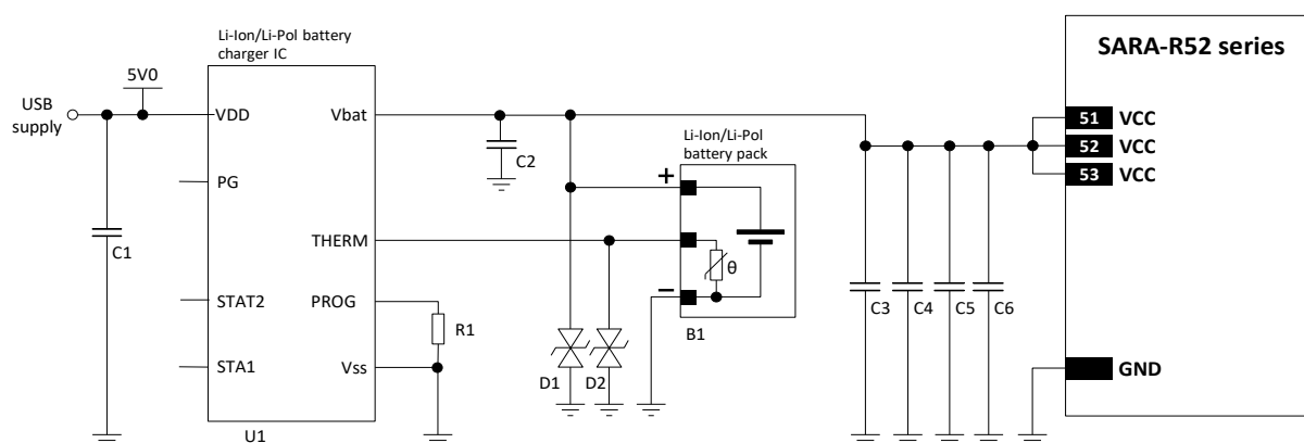
Figure 23: Li-Ion (or Li-Pol) battery charging application circuit
