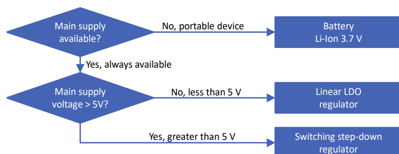
Figure 20: VCC supply concept selection
