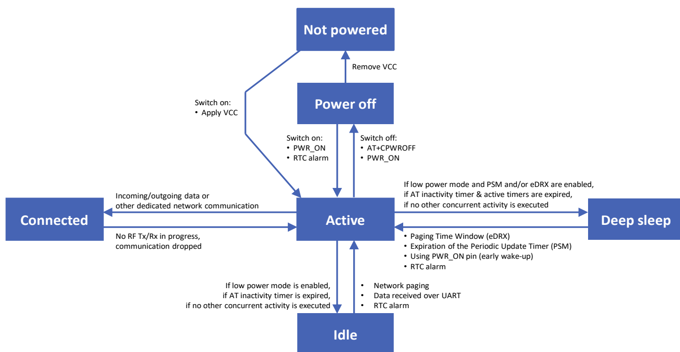
Figure 4: SARA-R52 series modules operating modes transitions
