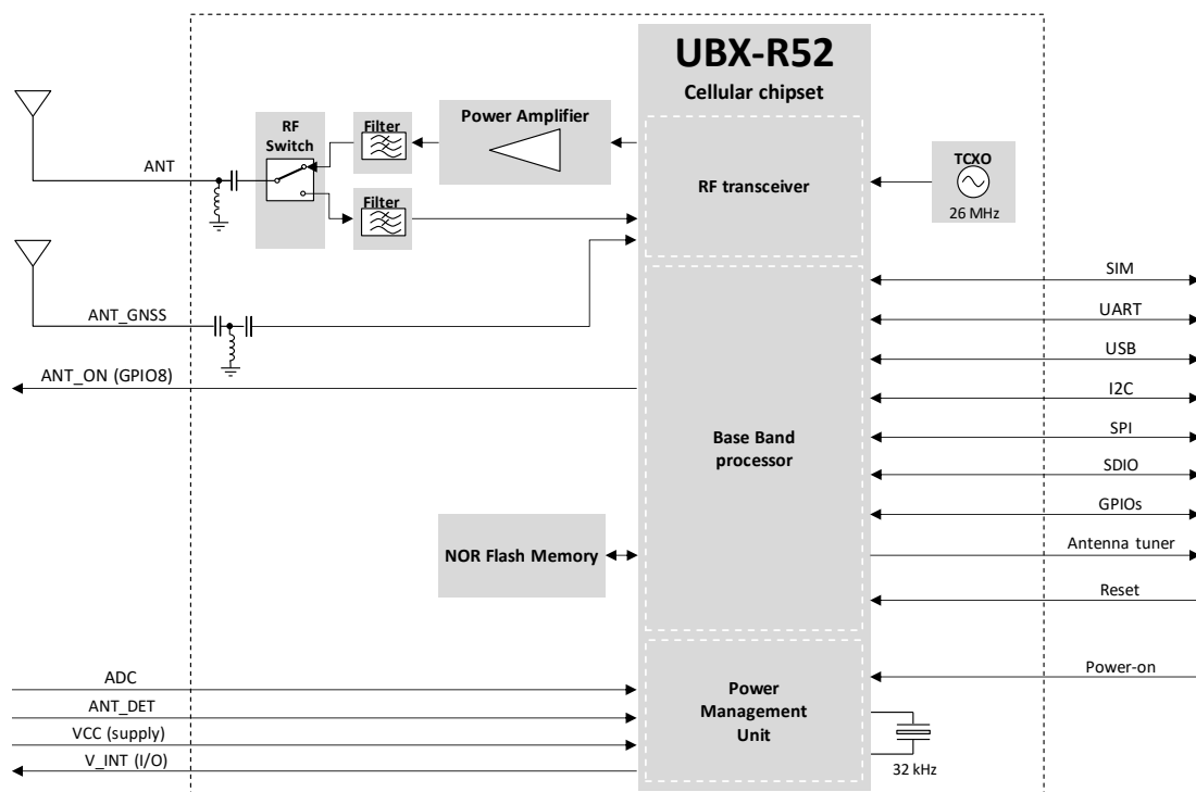
Figure 1: SARA-R520 module simplified block diagram
