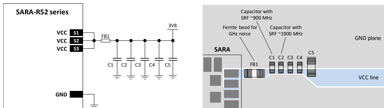
Figure 26: Suggested design to reduce ripple / noise on VCC, particularly suitable when using an integrated antenna
