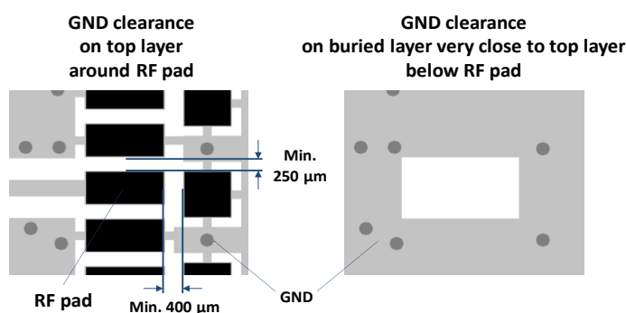
Figure 32: GND keep-out area on top layer around ANT / ANT_GNSS pad and on very close buried layer below pad
