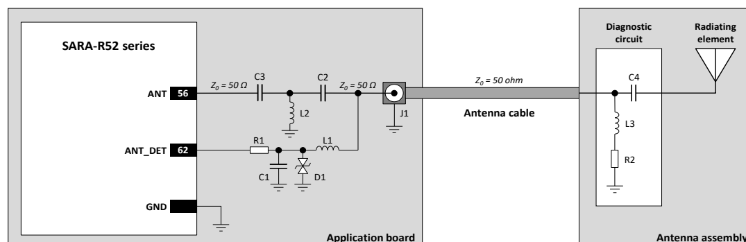
Figure 43: Schematic for antenna detection circuit on application PCB and diagnostic circuit on antenna assembly
