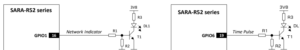
Figure 67: Application circuit for network indication provided over GPIO1 and/or time pulse provided over GPIO6
