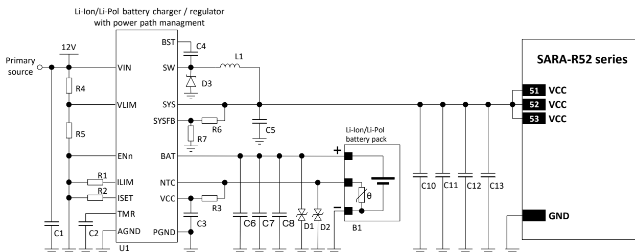
Figure 25: Li-Ion (or Li-Pol) battery charging and power path management application circuit
