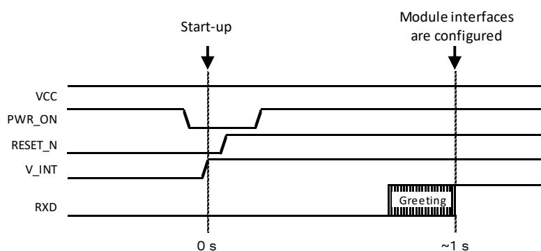
Figure 12: SARA-R52 series switch-on / early wake-up sequence description from power-off / deep-sleep mode
