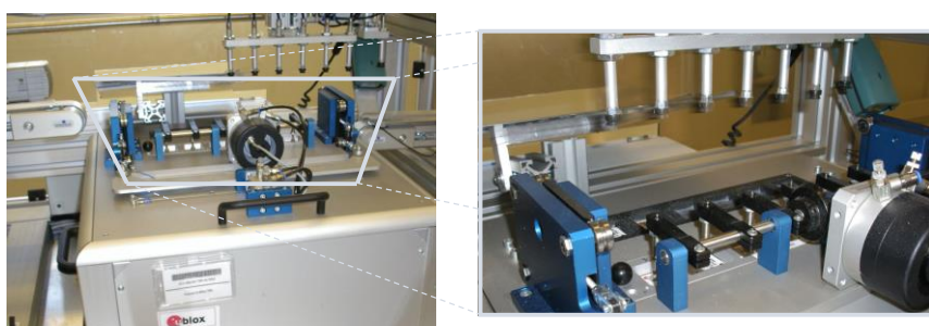
Figure 75: Automatic test equipment for module tests
