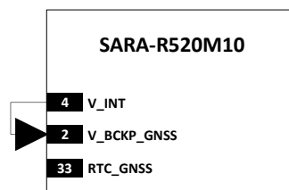
Figure 70: GNSS RTC application circuit with clock generated internally
