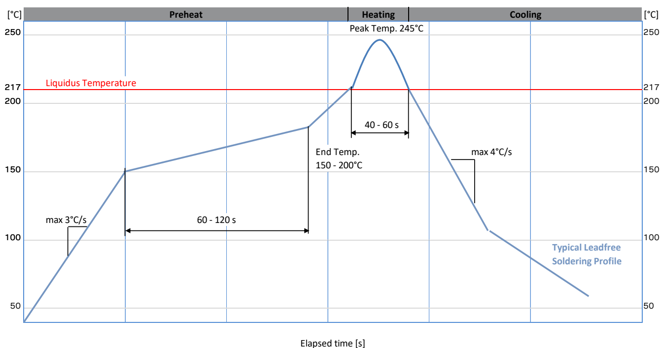
Figure 74: Recommended soldering profile
