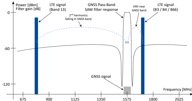
Figure 40: EMI due to Tx in LTE B3, B4, B66 low channels (1710 MHz) adjacent to GNSS frequency range (1561 to 1610 MHz), or due to Tx in LTE B13 high channels (787 MHz) with harmonics falling into the GNSS frequency range
