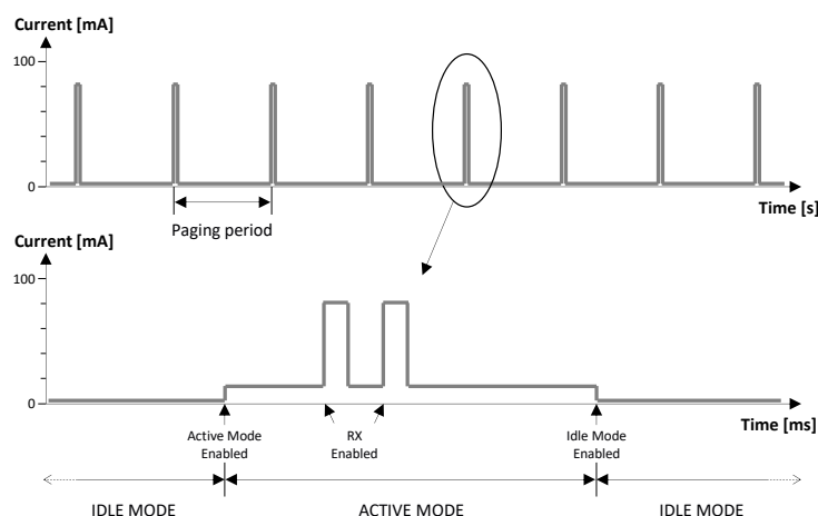
Figure 7: VCC current consumption profile with low power mode enabled
