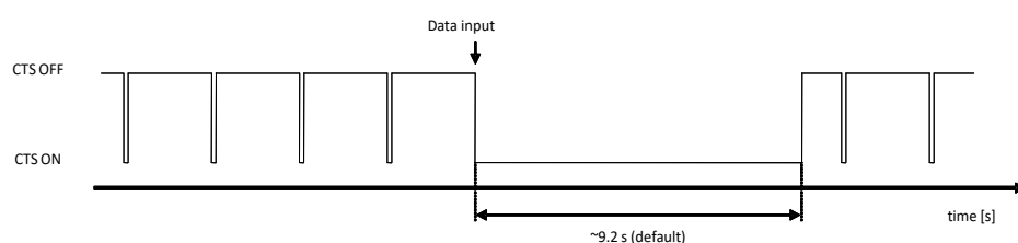
Figure 17: CTS behavior with power saving enabled (AT+UPSV=1) and HW flow control enabled:
