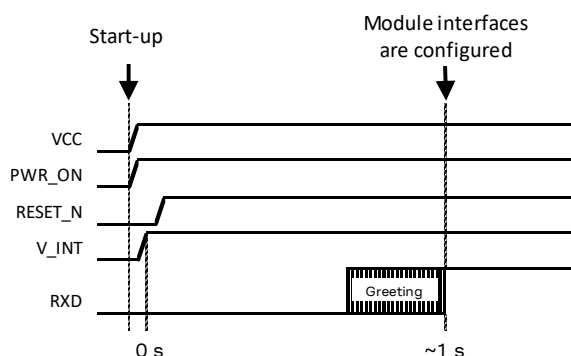
Figure 11: SARA-R52 series switch-on sequence description from not-powered mode
