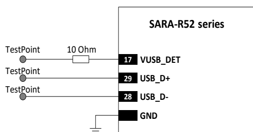
Figure 62: SARA-R52 series modules USB application circuit providing access for diagnostic purposes
