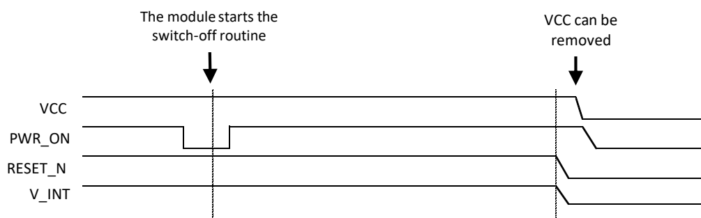
Figure 14: SARA-R52 series modules switch-off sequence by toggling the PWR_ON input pin
