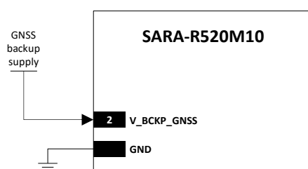
Figure 28: V_BCKP_GNSS application circuit using an independent power supply
