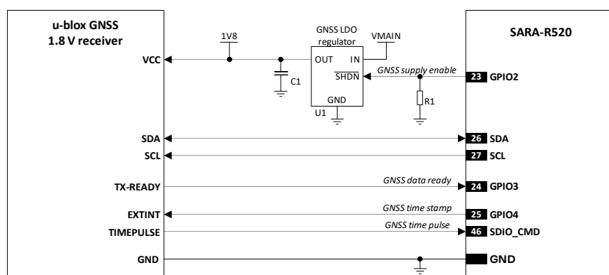
Figure 65: Application circuit for connecting SARA-R520 modules to a u-blox 1.8 V GNSS receiver
