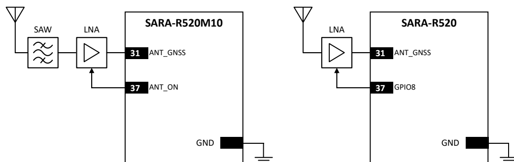
Figure 38: Example for best performance and better jamming immunity with GNSS passive antenna placed far away
