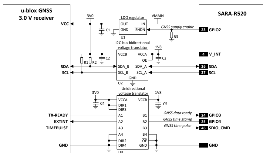
Figure 66: Application circuit for connecting SARA-R520 modules to a u-blox 3.0 V GNSS receiver
