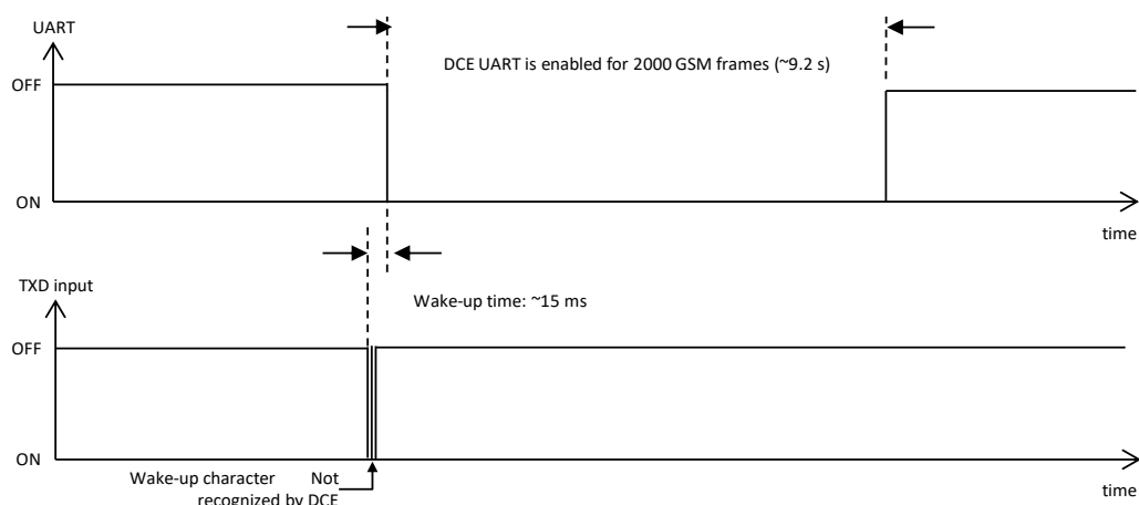
Figure 18: Wake-up via data reception without further communication
