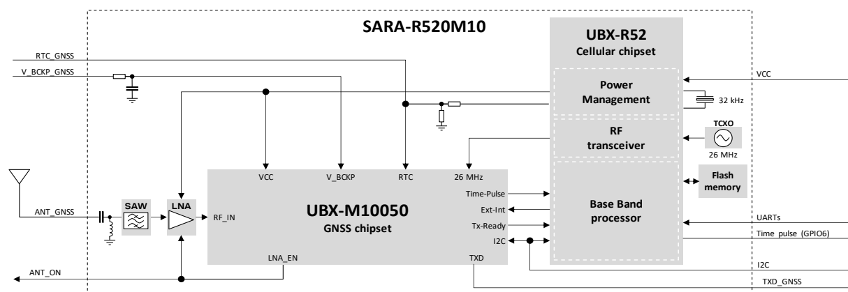
Figure 3: SARA-R520M10 modules GNSS section block diagram
