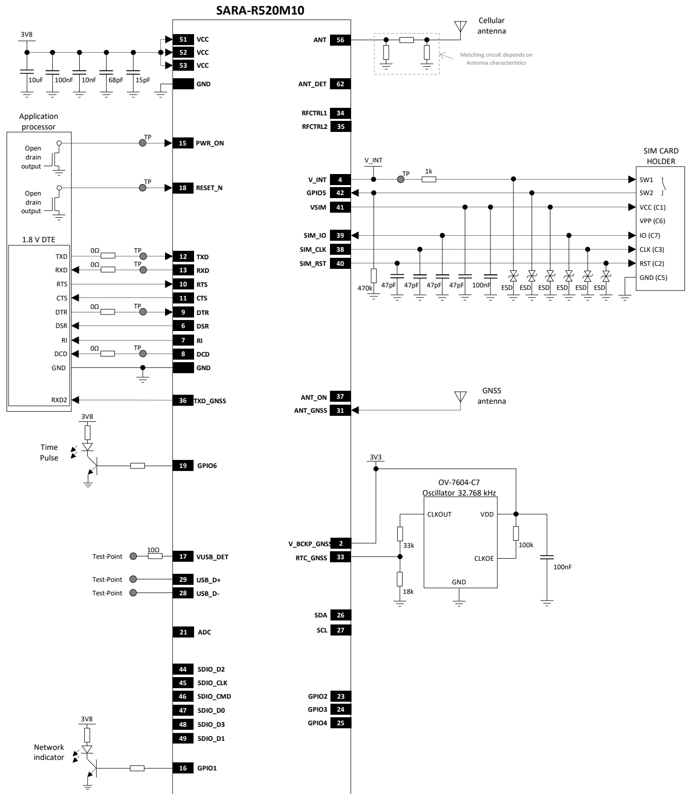
Figure 73: Example schematic diagram integrating a SARA-R520M10 module
