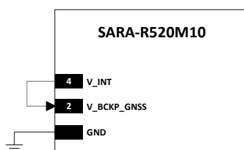
Figure 29: V_BCKP_GNSS application circuit shorting with V_INT supply
