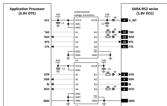
Figure 50: 1 UART interface application circuit with complete V.24 link in DTE/DCE serial communication (3.0 V DTE)
