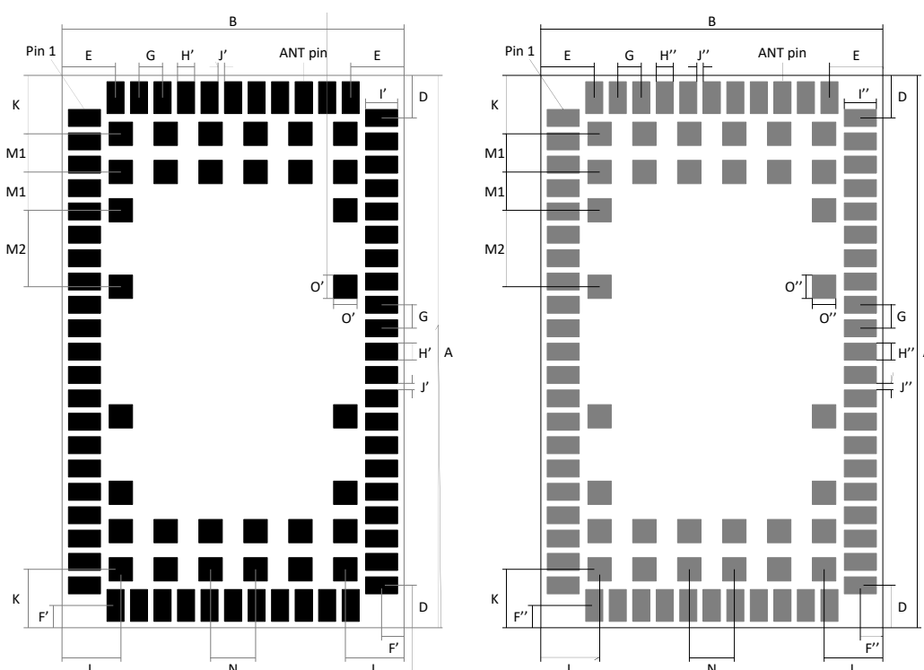
Figure 71: SARA-R52 series modules suggested footprint and paste mask (application board top view)
