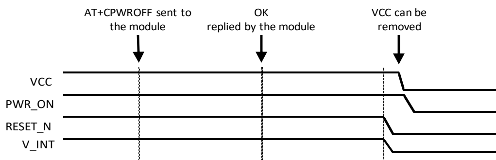
Figure 13: SARA-R52 series modules switch-off sequence by the +CPWROFF AT command
