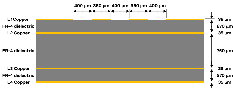
Figure 63: Example of USB line design, with Z_0 = 90 \Omega and Z_{CM} = 30 \Omega , for the described 4-layer PCB layout
