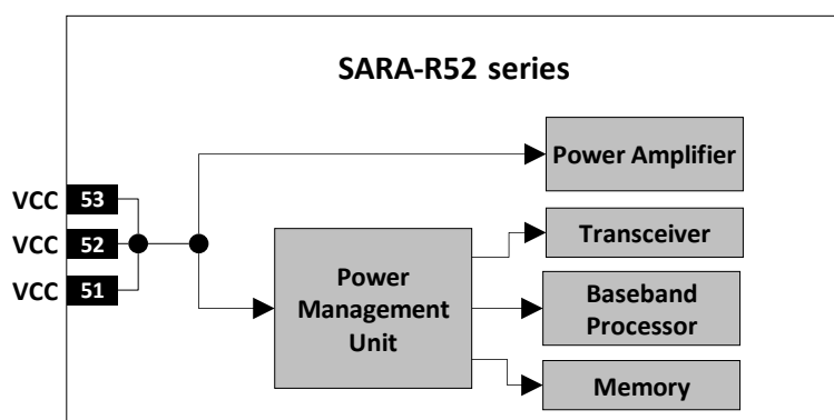
Figure 5: SARA-R52 series modules' internal VCC supply routing
