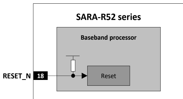
Figure 15: SARA-R52 series RESET_N input equivalent circuit description
