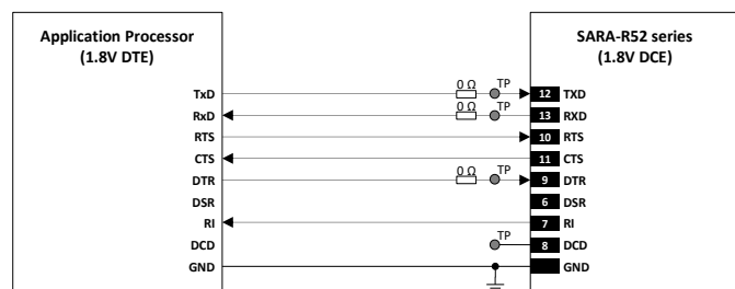
Figure 51: 1 UART interface application circuit with 7-wire link in DTE/DCE serial communication (1.8 V DTE)
