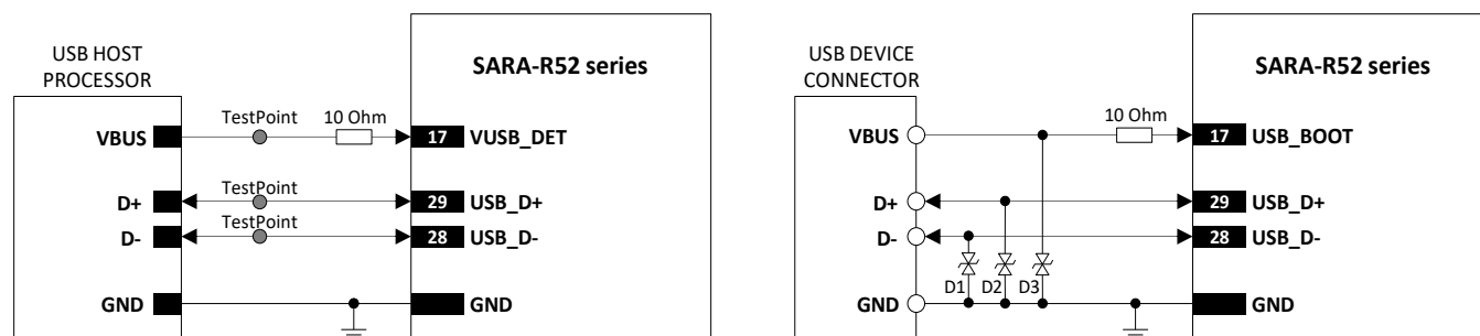
Figure 61: SARA-R52 series modules USB application circuit for AT and data communication
