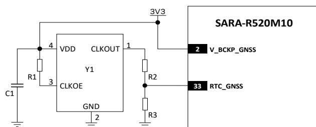
Figure 69: GNSS RTC application circuit with clock provided externally
