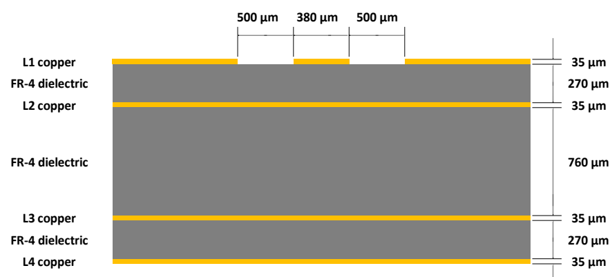
Figure 32: Example of 50 \Omega coplanar waveguide transmission line design for the described 4-layer board layup
