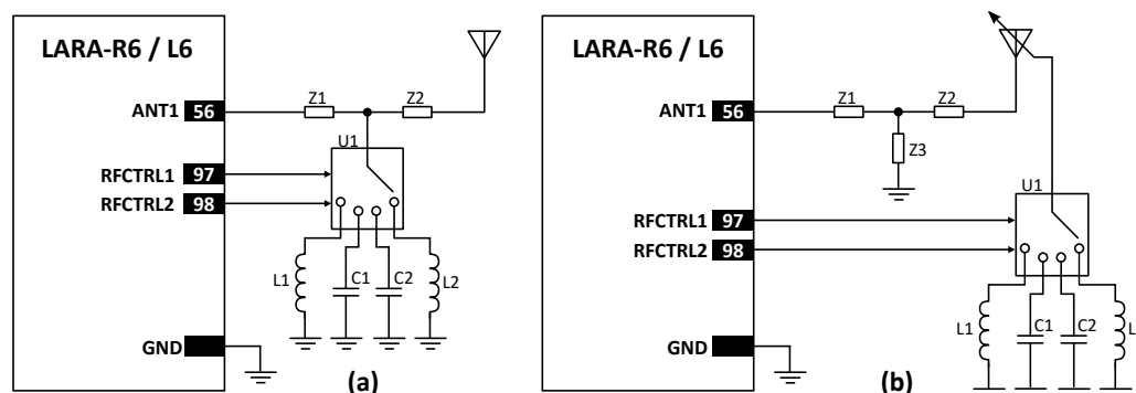
Figure 41: Examples of schematics for cellular antenna dynamic impedance tuning (a) and aperture tuning (b).
