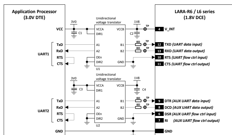
Figure 55: 2 UART application circuit without HW flow control in DTE/DCE serial communications (3.0 V DTE)
