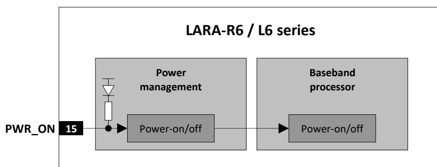
Figure 11: LARA-R6 / LARA-L6 series PWR_ON input description
