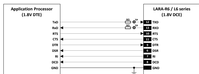
Figure 46: UART application circuit with complete V.24 link in DTE/DCE serial communication (1.8 V DTE)
