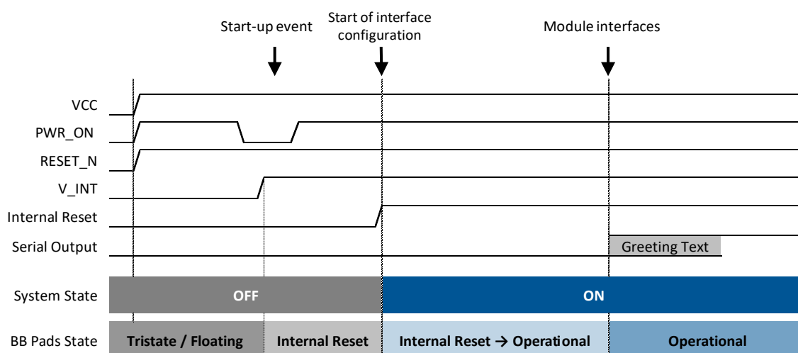
Figure 12: LARA-R6 / LARA-L6 series switch-on / wake-up sequence description
