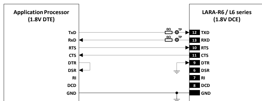
Figure 48: UART application circuit with partial V.24 link in the DTE/DCE serial communication (1.8 V DTE)
