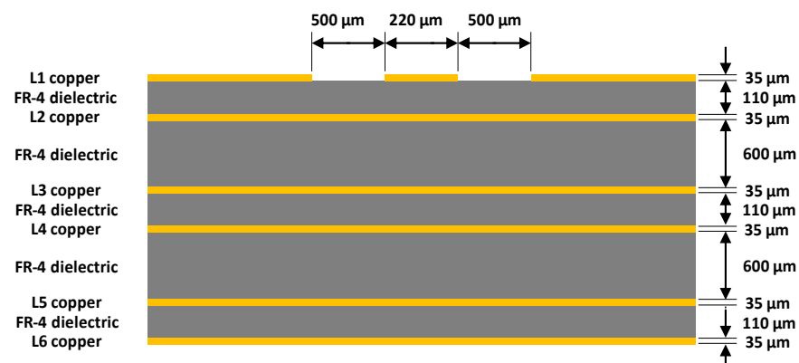
Figure 33: Example of 50 \Omega coplanar waveguide transmission line design for the described 6-layer board layup
