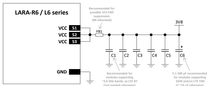
Figure 25: Suggested schematic for VCC bypass capacitors to reduce ripple / noise on supply voltage profile
