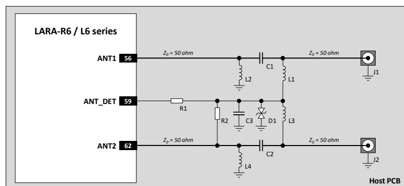
Figure 36: Antenna trace design implemented on the host PCB, with additional antenna detection circuit
