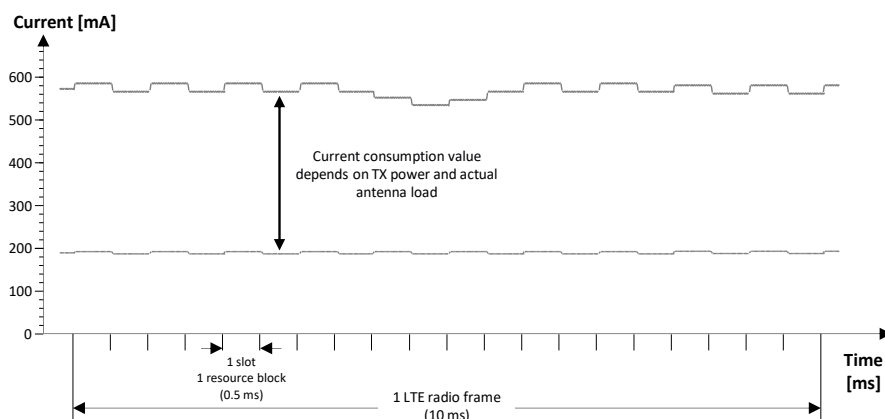
Figure 4: VCC current consumption profile versus time during LTE connection (TX and RX continuously enabled)
