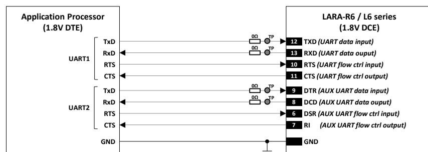
Figure 50: 2 UART application circuit with HW flow control in DTE/DCE serial communications (1.8 V DTE)
