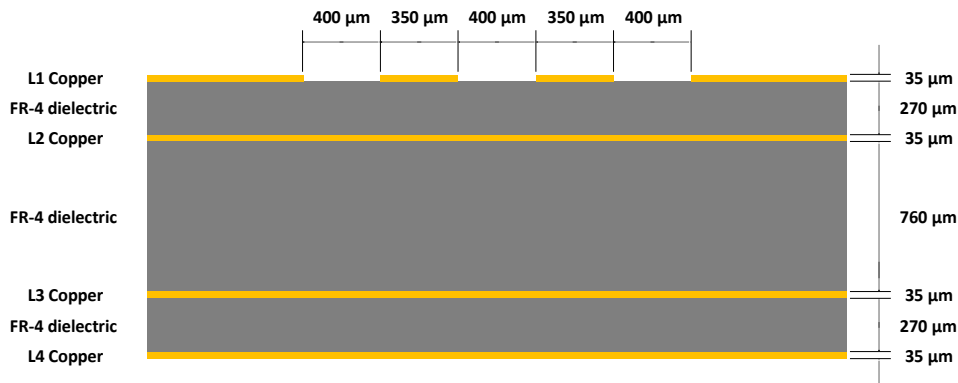
Figure 57: Example of USB line design, with Z_0 = 90\ \Omega and Z_{CM} = 30\ \Omega , for the described 4-layer board layout
