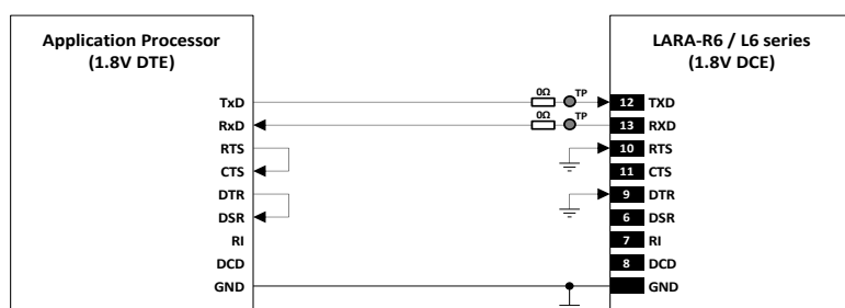
Figure 52: UART circuit with partial V.24 link (3-wire) in the DTE/DCE serial communication (1.8 V DTE)
