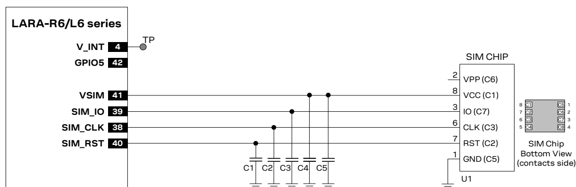
Figure 43: Circuit for the connection to a single solderable SIM chip, with SIM detection not implemented
