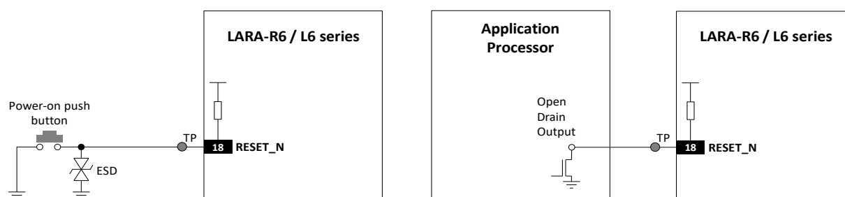
Figure 30: RESET_N application circuits using a push button and an open drain output of an external processor
