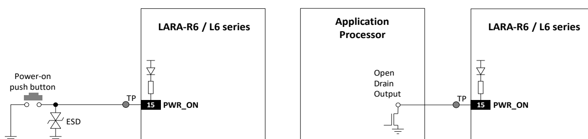
Figure 29: PWR_ON application circuits using a push button and an open drain output of an external processor
