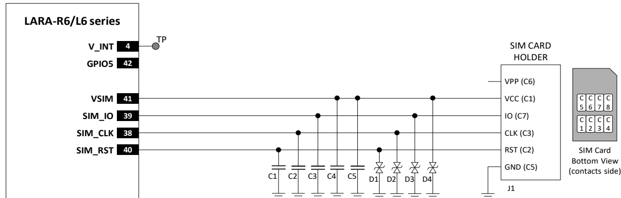
Figure 42: Circuit for the connection to a single removable SIM card, with SIM detection not implemented
