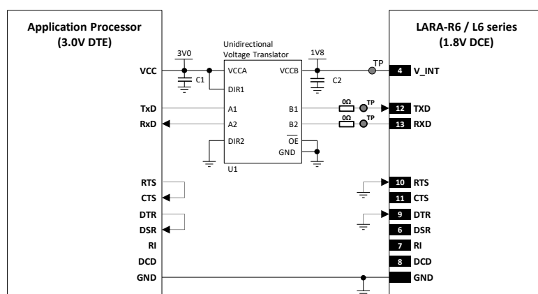
Figure 53: UART application circuit with partial V.24 link (3-wire) in DTE/DCE serial communication (3.0 V DTE)
