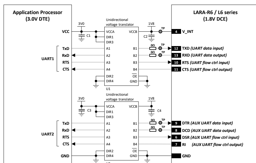
Figure 51: 2 UART application circuit with HW flow control in DTE/DCE serial communications (3.0 V DTE)
