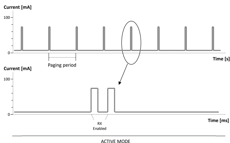
Figure 8: VCC current consumption profile with power saving disabled and module registered with the network
