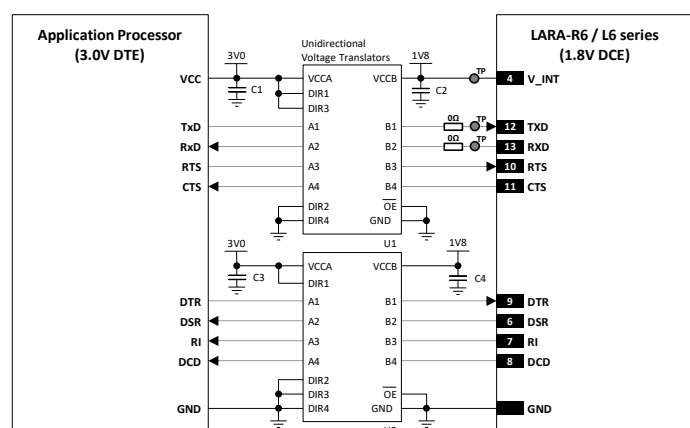
Figure 47: UART application circuit with complete V.24 link in DTE/DCE serial communication (3.0 V DTE)
