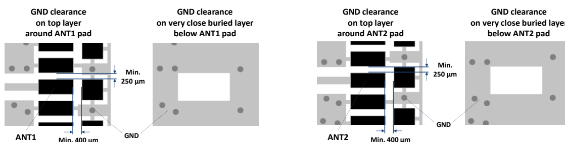
Figure 31: GND keep-out area on top layer around ANT1 / ANT2 pads and on very close buried layer below
