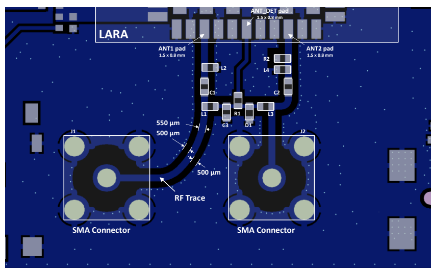
Figure 37: Top layer (L1) layout of the host PCB with the antenna RF trace design
