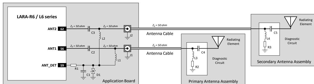
Figure 40: Suggested schematic for the antenna detection circuit and the diagnostic circuit
