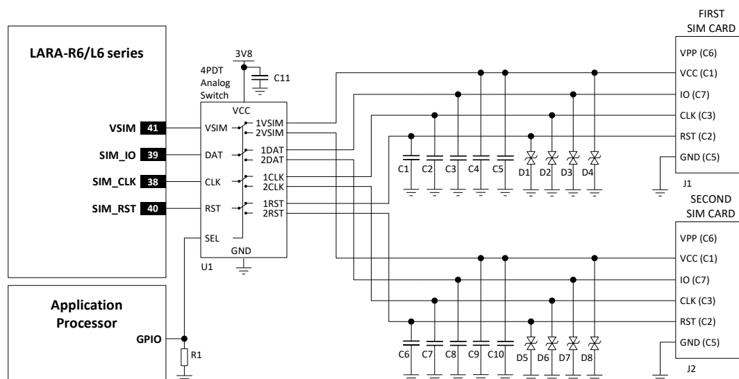
Figure 45: Circuit for the connection to two removable SIM cards, with SIM detection not implemented
