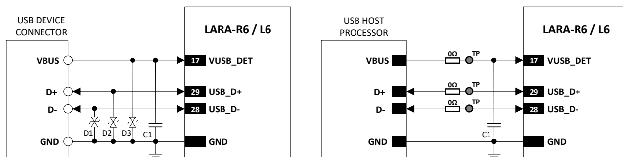
Figure 56: USB Interface application circuits
