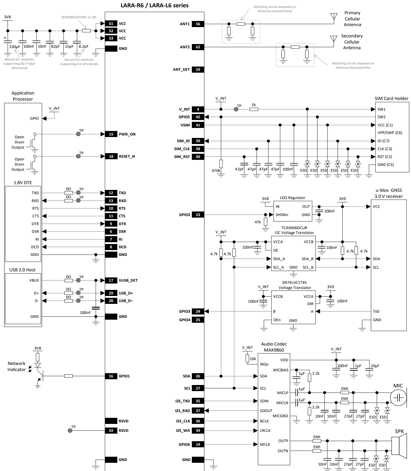
Figure 66: Example of schematic diagram to integrate a LARA-R6 / LARA-L6 module using almost all interfaces
