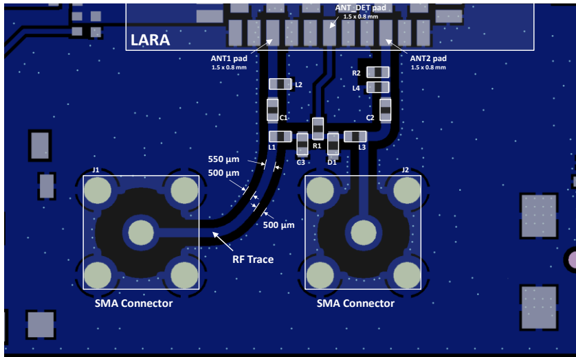
Figure 39: Buried metal layer (L2) layout of the u host PCB, below the antenna RF trace design
