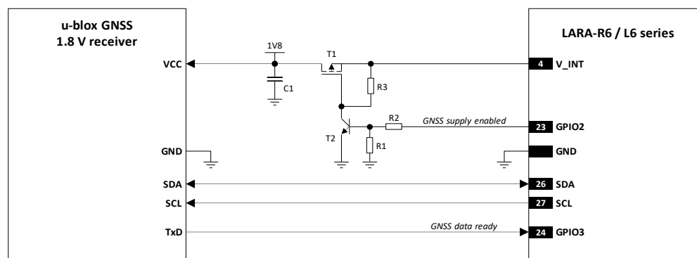
Figure 60: Application circuit for connecting the modules to u-blox 1.8 V GNSS receivers using V_INT as supply
