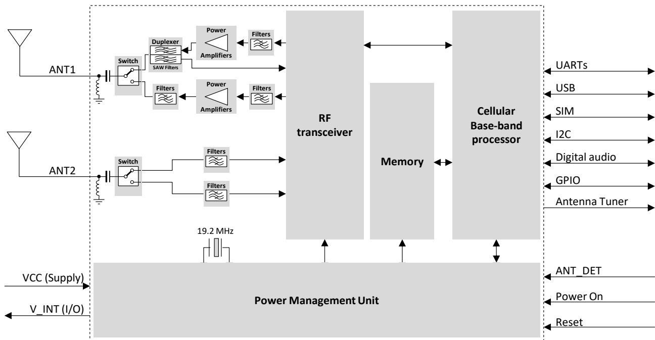
Figure 1: LARA-R6 / LARA-L6 series modules simplified block diagram
