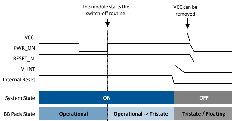
Figure 14: LARA-R6 / LARA-L6 series modules switch-off sequence by PWR_ON pin
