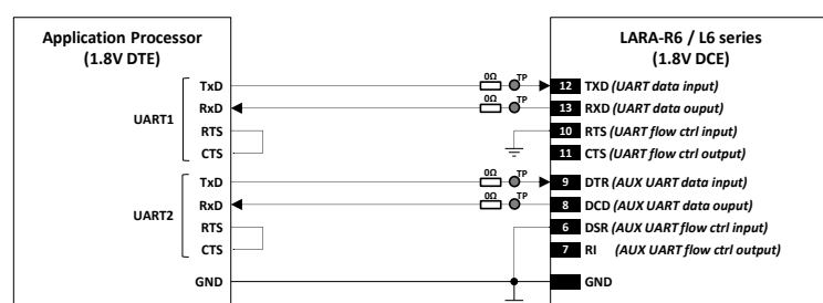
Figure 54: 2 UART application circuit without HW flow control in DTE/DCE serial communications (1.8 V DTE)
