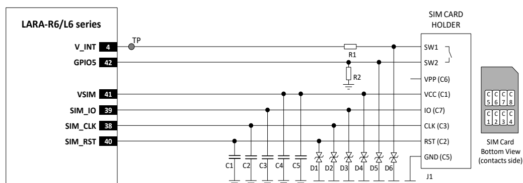
Figure 44: Circuit for the connection to a single removable SIM card, with SIM detection implemented
