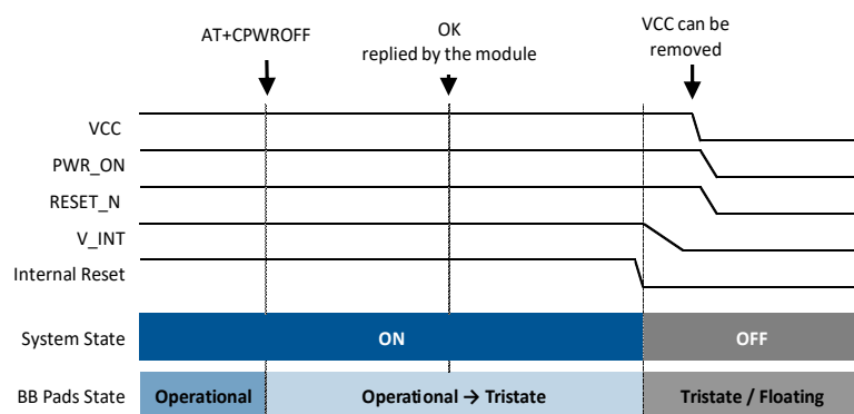
Figure 13: LARA-R6 / LARA-L6 series modules switch-off sequence by AT+CPWROFF command
