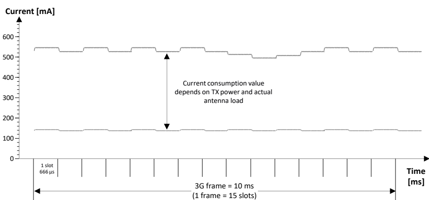
Figure 5: VCC current consumption profile versus time during a 3G connection (TX and RX continuously enabled)
