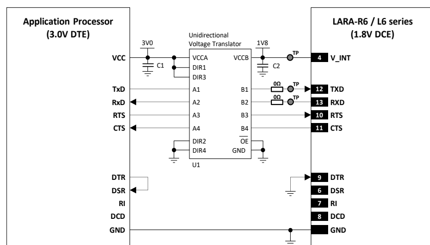
Figure 49: UART application circuit with partial V.24 link in DTE/DCE serial communication (3.0 V DTE)
