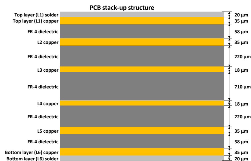
Figure 38: Stack-up structure of the host PCB
