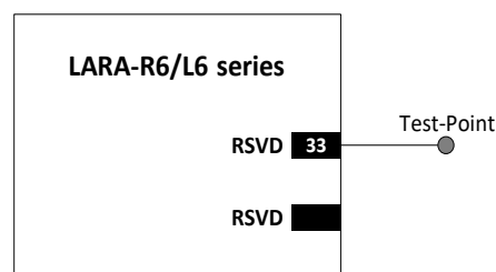
Figure 64: Application circuit for the reserved pins (RSVD)
