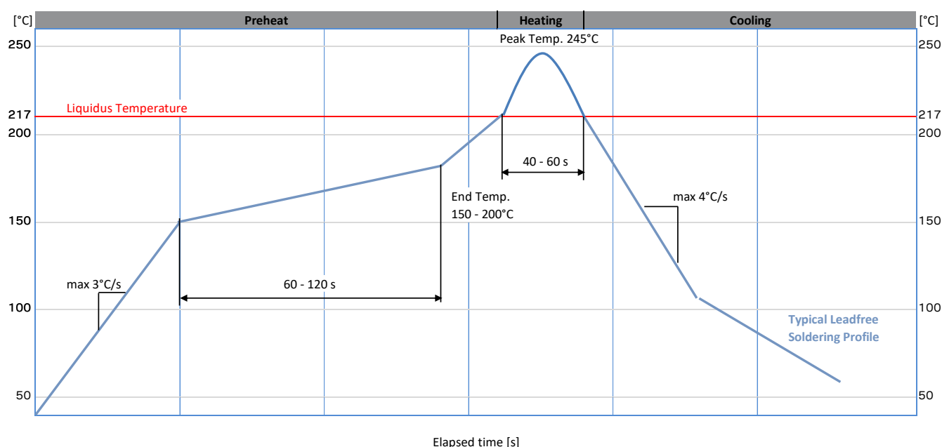
Figure 67: Recommended soldering profile
