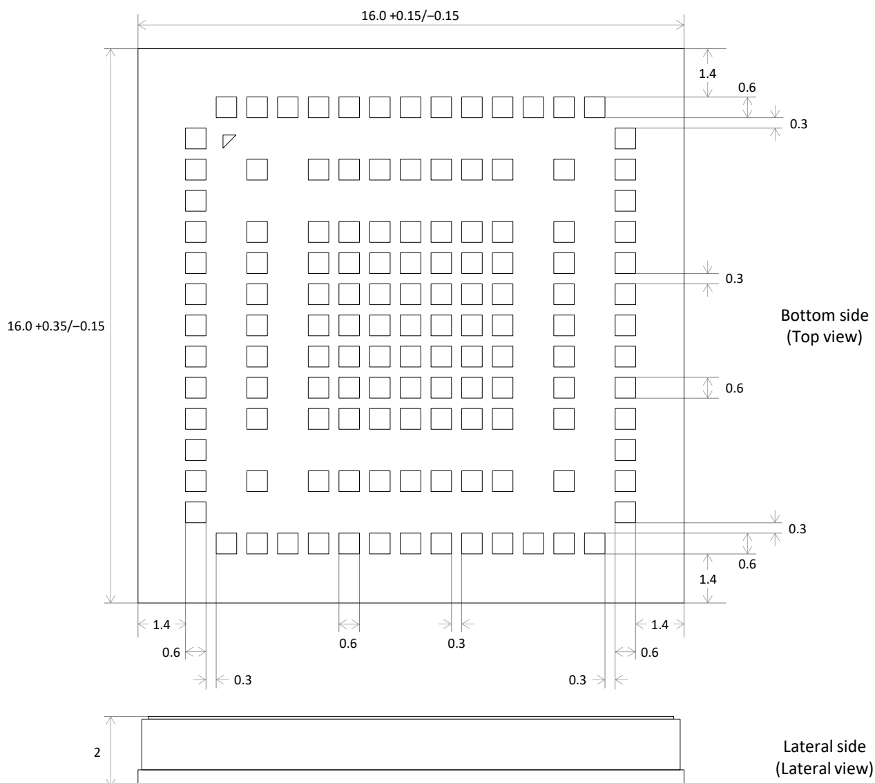
Figure 3: LEXI-R422 dimensions, typical values [mm]
