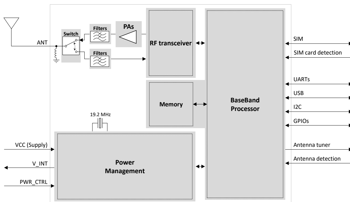
Figure 1: LEXI-R422 block diagram
