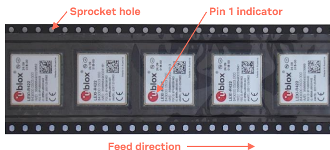
Figure 4: Orientation of LEXI-R422 modules on tape
