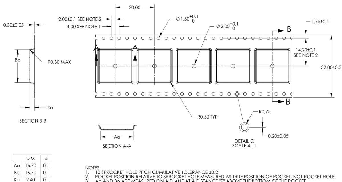
Figure 5: LEXI-R422 modules tape (all dimensions in millimeters)
