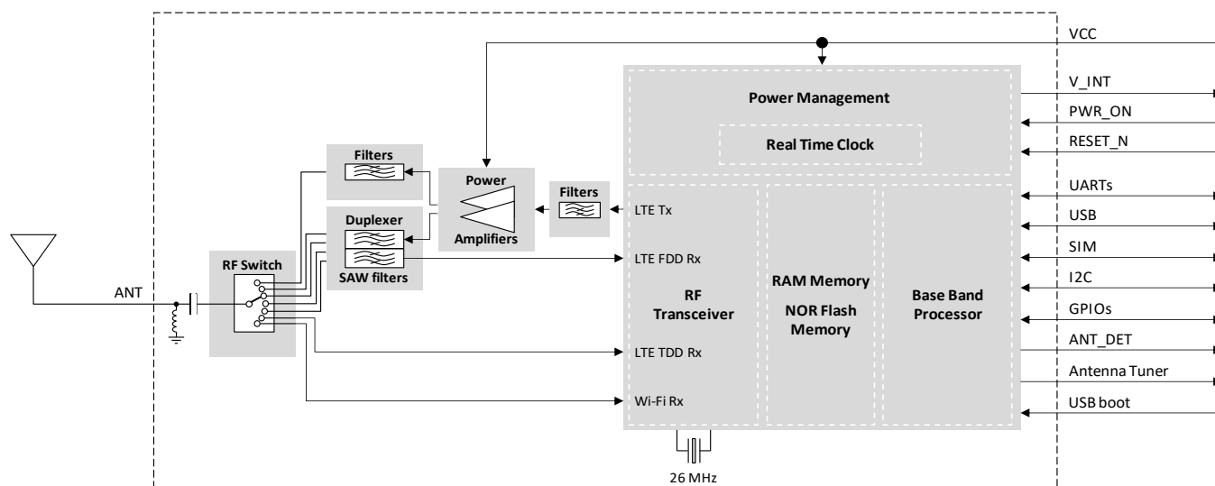
Figure 1: LEXI-R10 series modules' simplified block diagram
