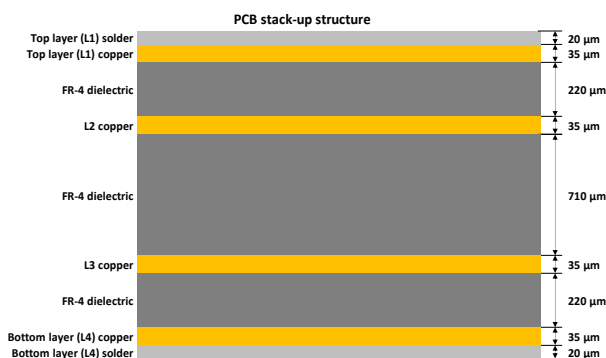
Figure 36: Stack-up structure of the host PCB for LEXI-R10001D / LEXI-R10011D modules
