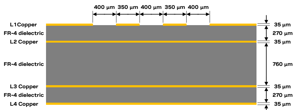
Figure 56: Example of USB line design, with Z_0 = 90 \Omega and Z_{CM} = 30 \Omega , for the described 4-layer PCB layup
