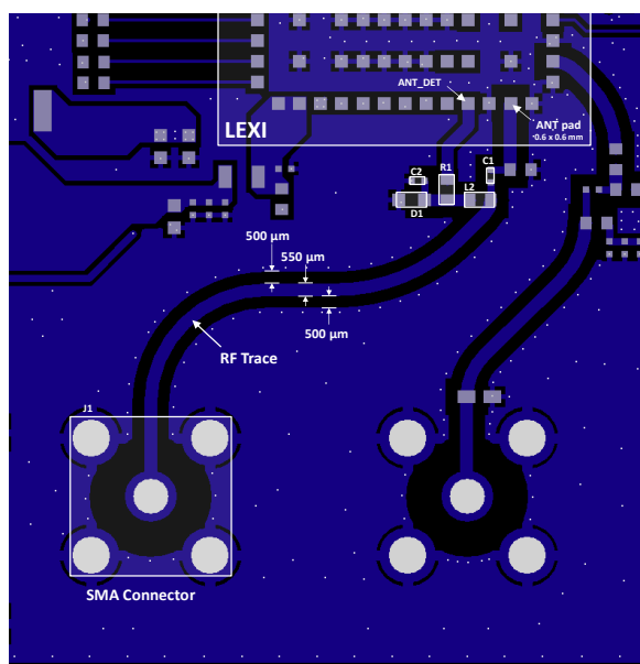
Figure 31: Top layer (L1) layout of the host PCB with the antenna RF trace design for LEXI-R10401D / LEXI-R10801D
