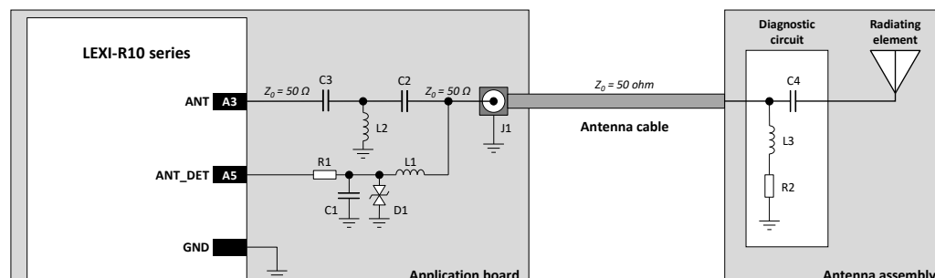
Figure 40: Schematic example for antenna detection circuit on host PCB and diagnostic circuit on antenna assembly
