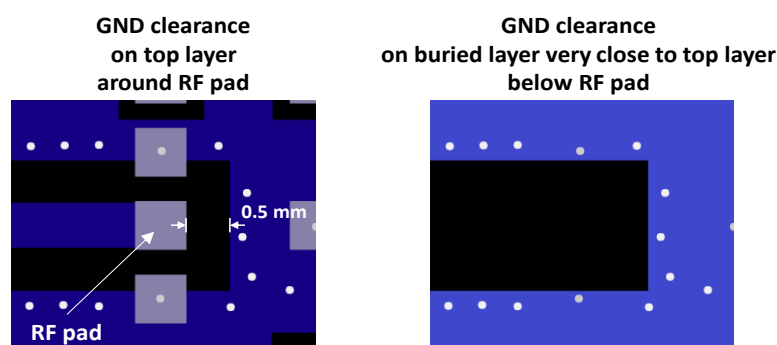
Figure 25: GND keep-out area on top layer around RF pad and on very close buried layer below RF pad (ANT)
