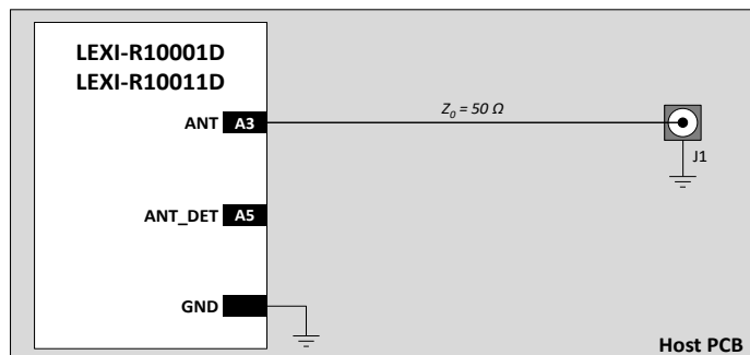
Figure 34: Antenna trace design implemented on the host PCB used for LEXI-R10001D / LEXI-R10011D modules
