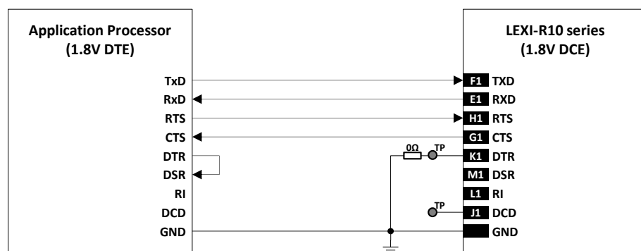
Figure 49: UART application circuit with partial V.24 link (5-wire) in the DTE/DCE serial communication (1.8V DTE)
