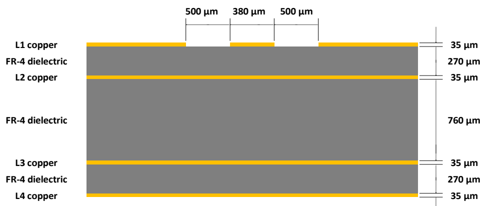
Figure 26: Example of 50 \Omega coplanar waveguide transmission line design for the described 4-layer board layup
