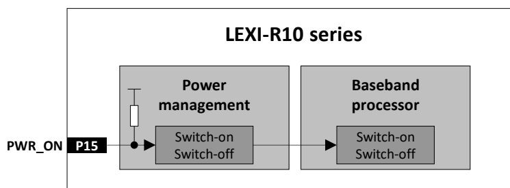
Figure 5: PWR_ON input pin description
