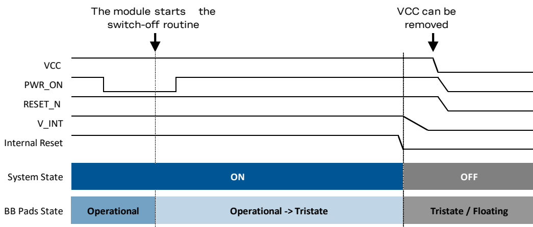
Figure 8: LEXI-R10 series modules switch-off sequence by PWR_ON pin
