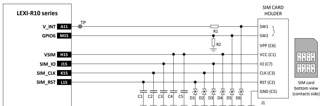
Figure 45: Circuit to connect a removable SIM card with SIM card detection implemented, keeping AT+UPSV=0
