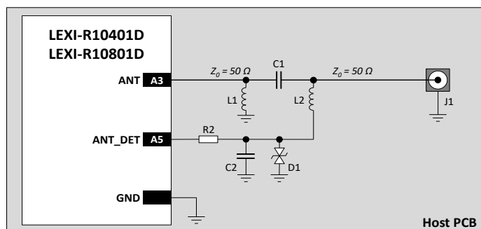
Figure 30: Antenna trace design implemented on the host PCB used for LEXI-R10401D and LEXI-R10801D modules
