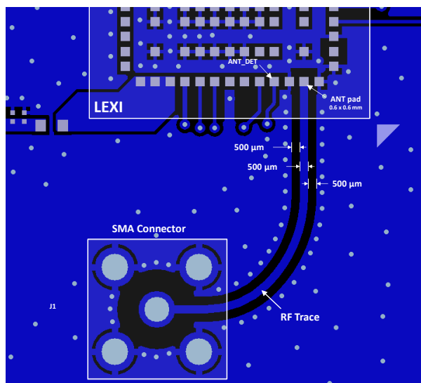
Figure 35: Top layer (L1) layout of the host PCB with the antenna RF trace design for LEXI-R10001D / LEXI-R10011D
