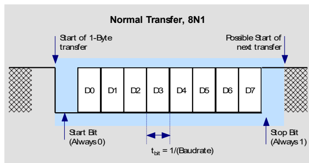
Figure 10: UART 8N1 frame format (8 data bits, no parity, 1 stop bit)
