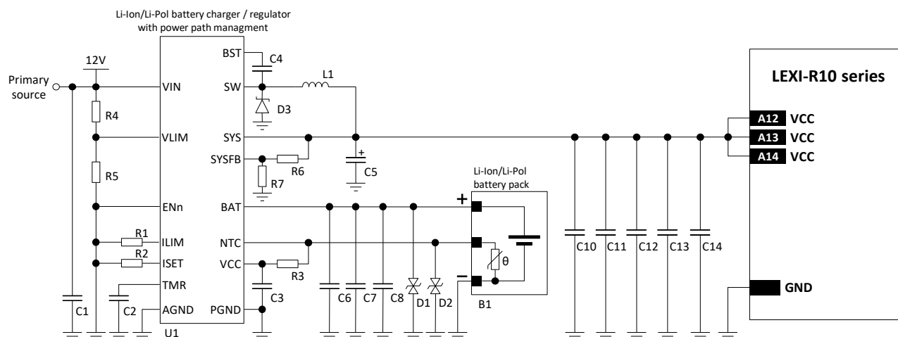
Figure 19: Li-Ion (or Li-Polymer) battery charging and power path management application circuit
