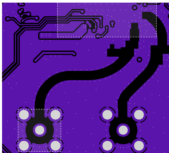
Figure 33: Buried layer (L2) of the host PCB for LEXI-R10401D / LEXI-R10801D, below the antenna RF trace design
