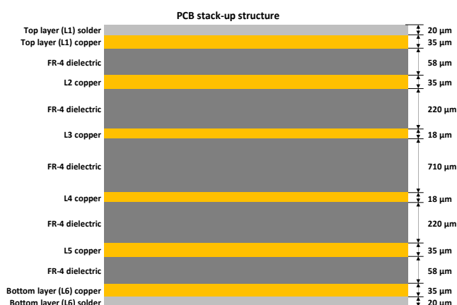
Figure 32: Stack-up structure of the host PCB for LEXI-R10401D / LEXI-R10801D modules
