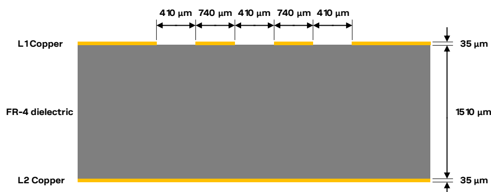
Figure 57: Example of USB line design, with Z_0 = 90 \Omega and Z_{CM} = 30 \Omega , for the described 2-layer PCB layup
