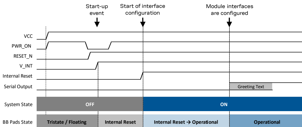
Figure 6: LEXI-R10 series switch-on sequence description
