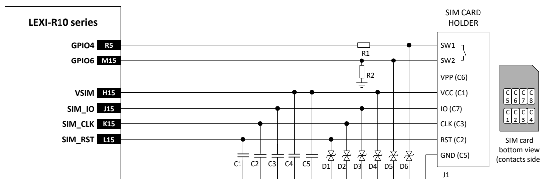
Figure 46: Circuit to connect a removable SIM card with SIM card detection implemented, using AT+UPSV≠0
