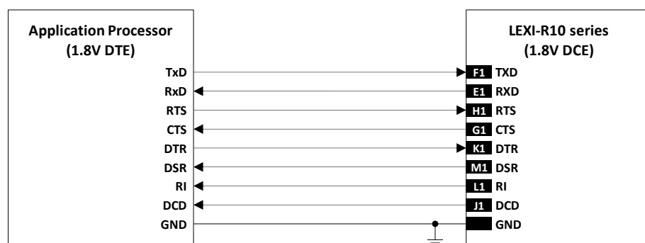
Figure 47: UART interface application circuit with complete V.24 link in DTE/DCE serial communication (1.8V DTE)
