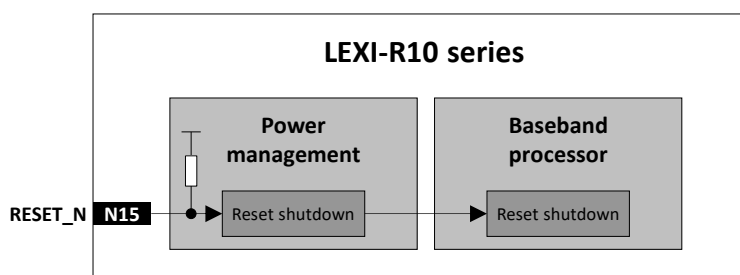
Figure 9: RESET_N input pin description
