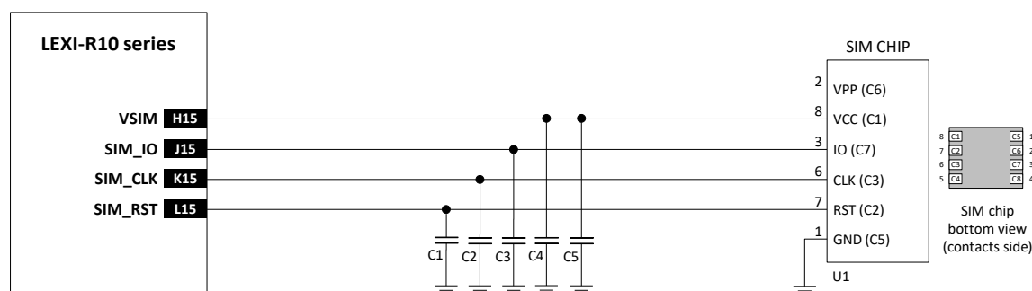
Figure 44: Application circuits for the connection to a Surface-Mounted SIM chip
