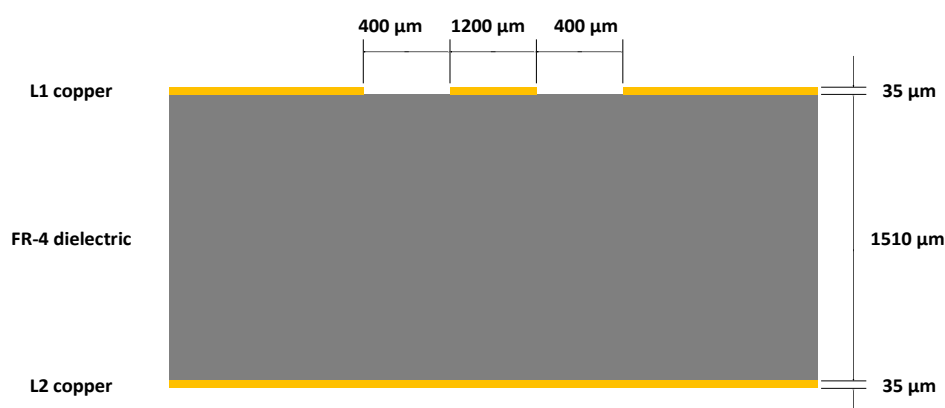
Figure 27: Example of 50 \Omega coplanar waveguide transmission line design for the described 2-layer board layup
