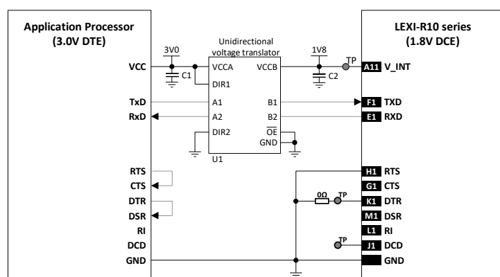
Figure 54: UART application circuit with a partial V.24 link (3-wire) in DTE/DCE serial communication (3.0 V DTE)
