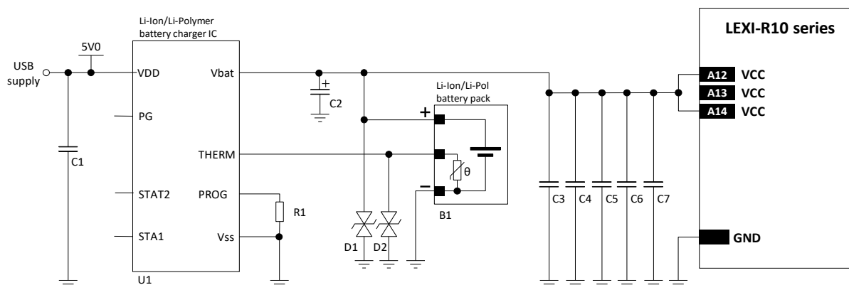
Figure 17: Li-Ion (or Li-Polymer) battery charging application circuit
