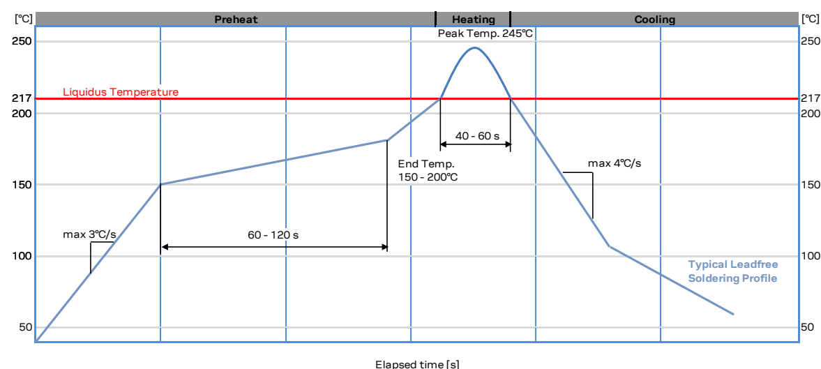
Figure 61: Recommended soldering profile
