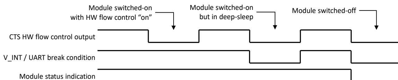
Figure 11: LEXI-R10 illustrative behavior of UART and “always-on” GPIO with power saving configurations enabled
