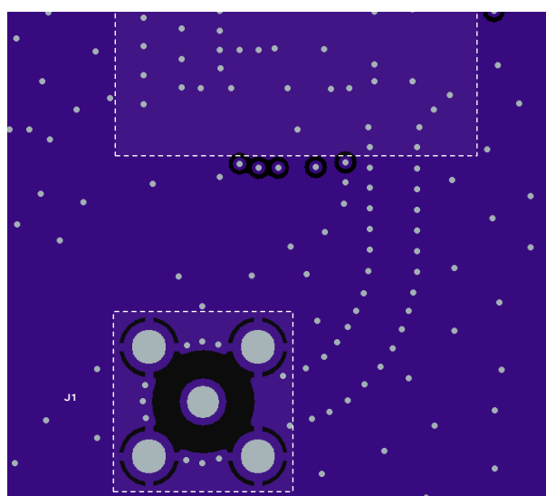
Figure 37: Buried layer (L2) of the host PCB for LEXI-R10001D / LEXI-R10011D, below the antenna RF trace design
