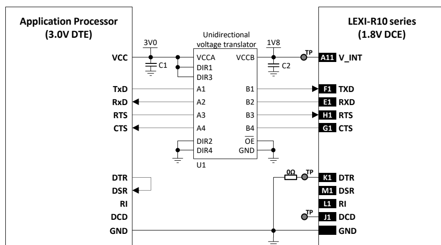
Figure 50: UART application circuit with a partial V.24 link (5-wire) in DTE/DCE serial communication (3.0 V DTE)
