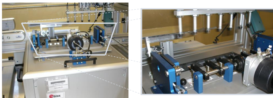
Figure 62: Automatic test equipment for module tests
