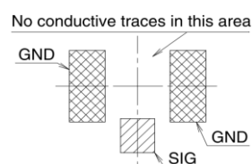
Figure 29: U.FL surface mounted connector mounting pattern layout
