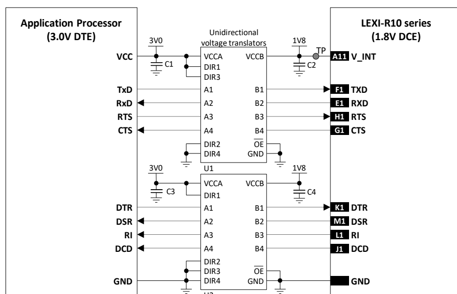
Figure 48: UART interface application circuit with complete V.24 link in DTE/DCE serial communication (3.0 V DTE)
