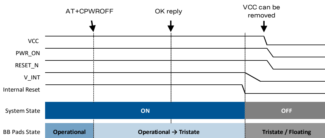
Figure 7: LEXI-R10 series modules switch-off sequence by AT+CPWROFF command
