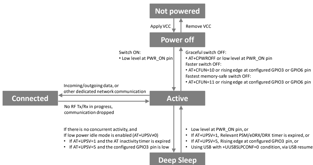
Figure 2: LEXI-R10 series modules operating modes transitions
