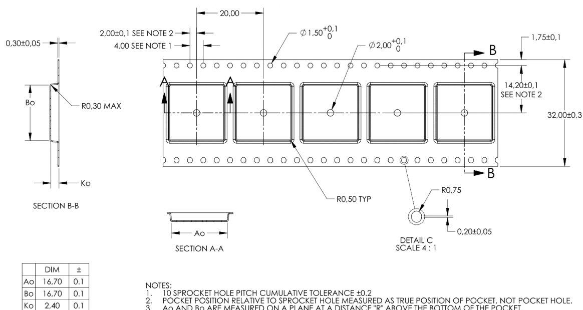
Figure 6: LEXI-R520 modules tape
