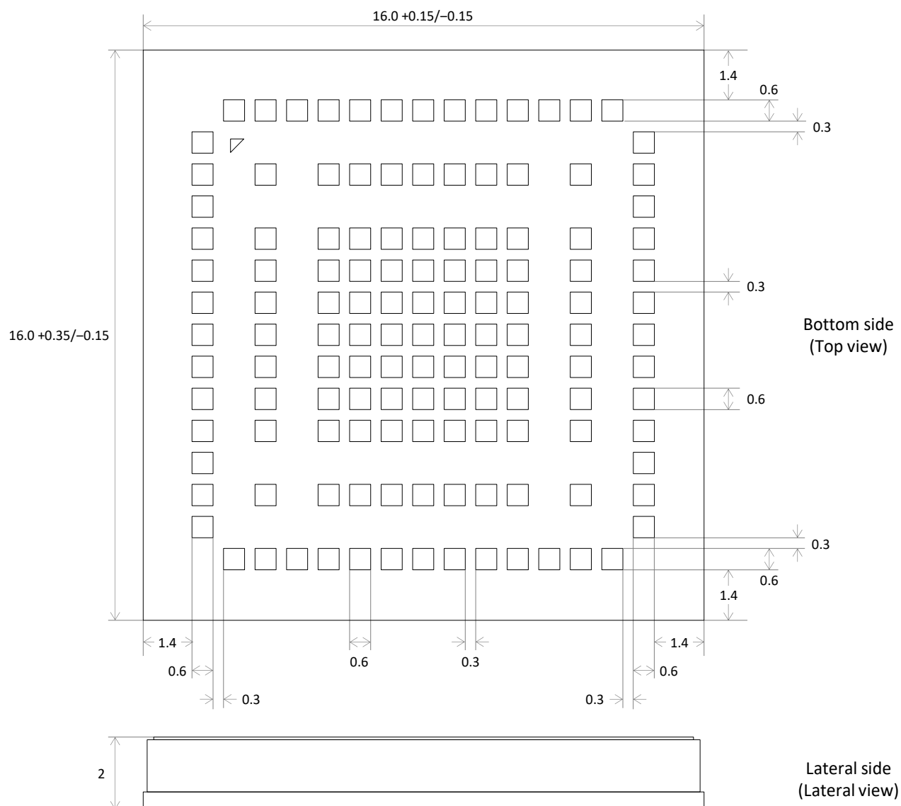
Figure 4: LEXI-R520 dimensions, typical values [mm]
