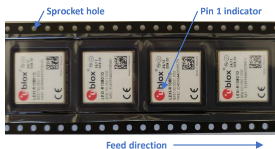
Figure 5: Orientation of modules on tape
