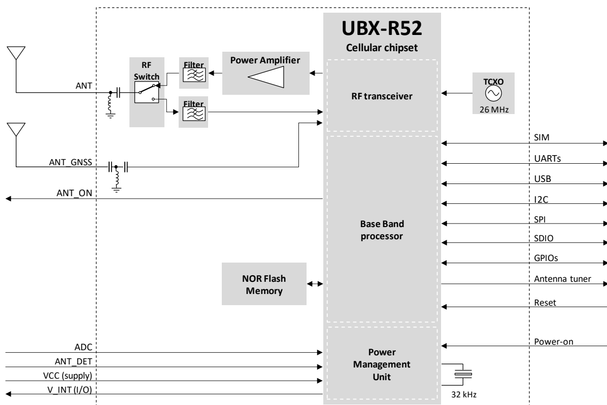
Figure 1: LEXI-R520 block diagram
