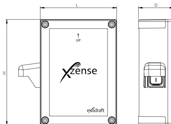
Power Unit
