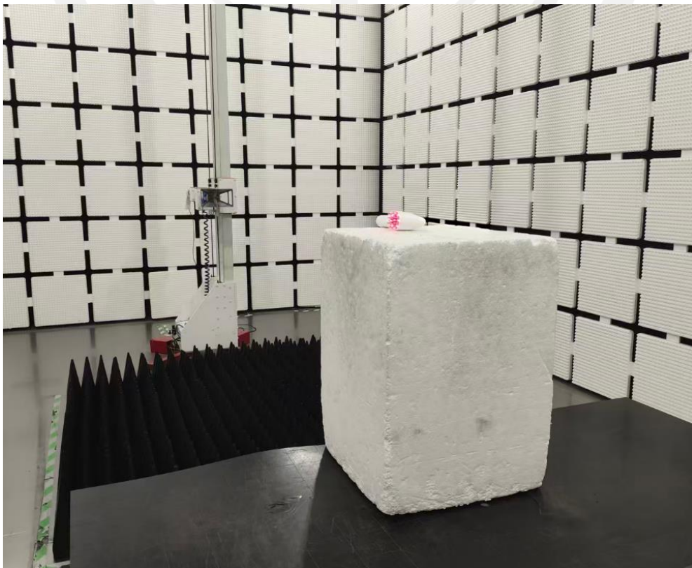
Spurious Radiation Emissions Test (> 1G)
