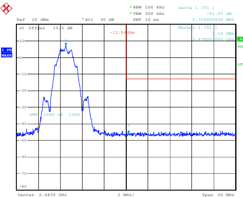
BLE_2M_High_Channel
