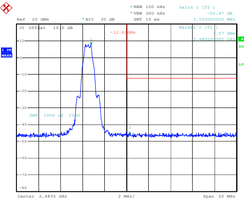
BLE_1M_High_Channel
