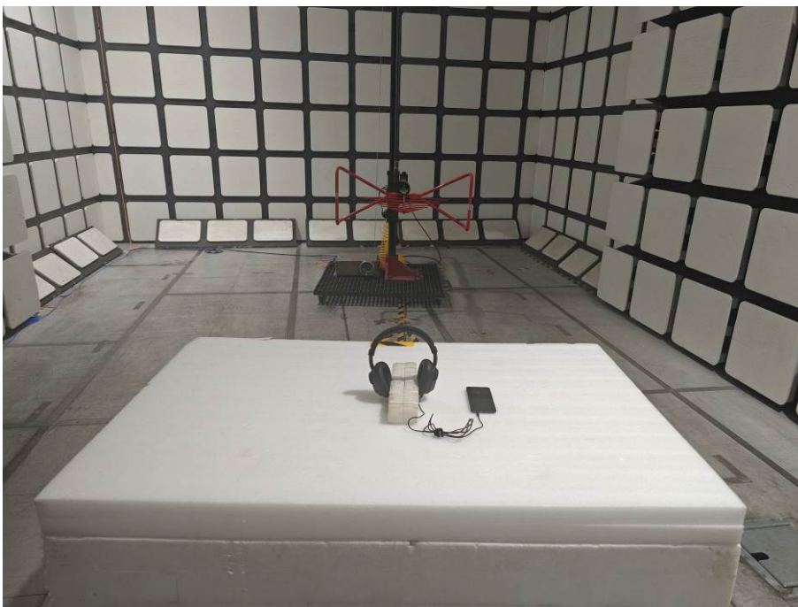
Radiated EmissionsView (Below 960MHz)
