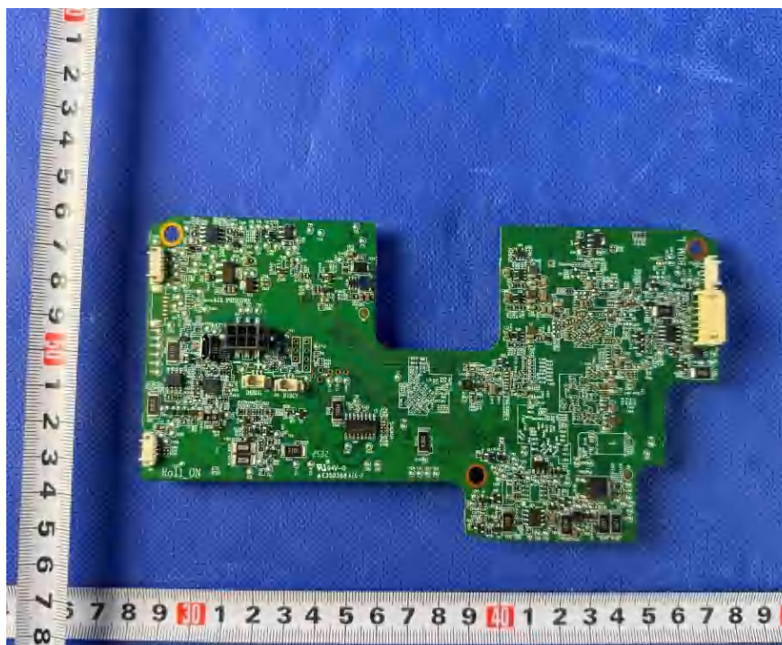
Figure 28. Main PCB
