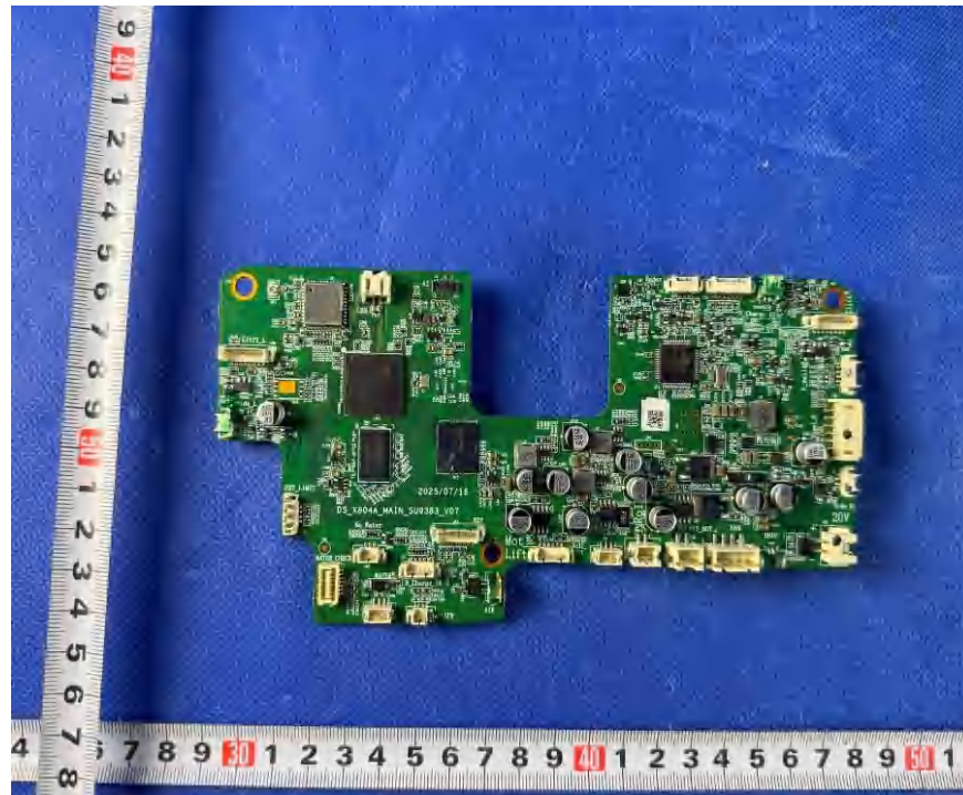
Figure 27. Main PCB
