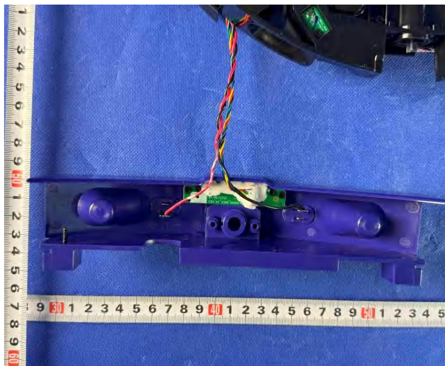
Figure 18. Internal view
