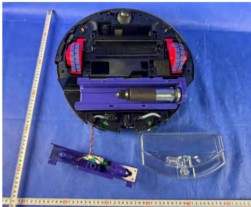
Figure 14. Internal view
