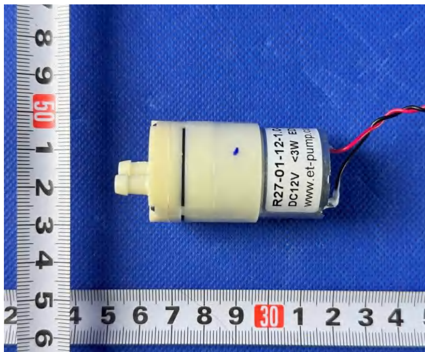
Figure 36. Vacuum pump
