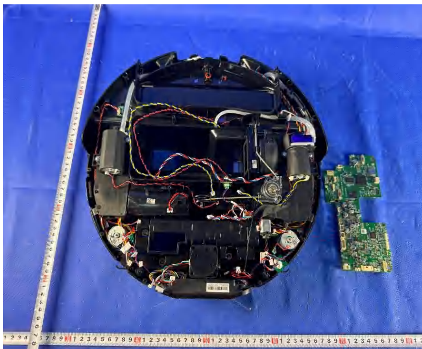
Figure 26. Internal view
