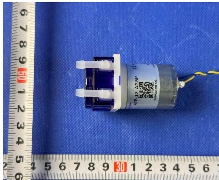
Figure 38. Peristaltic pump
