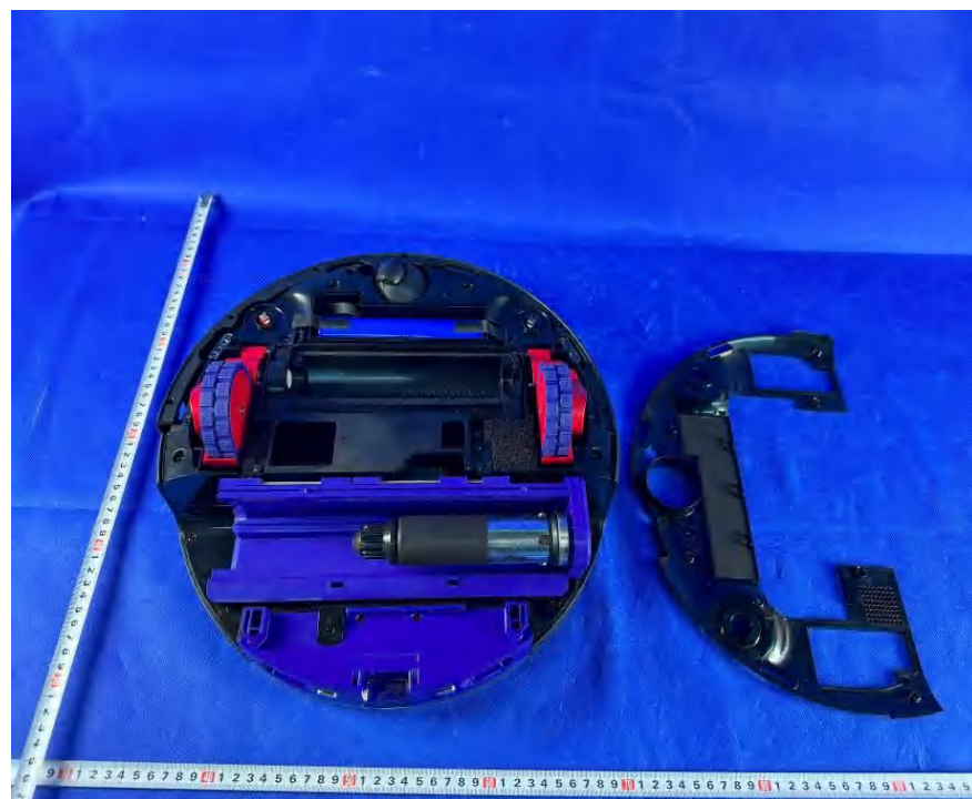
Figure 10. Internal view
