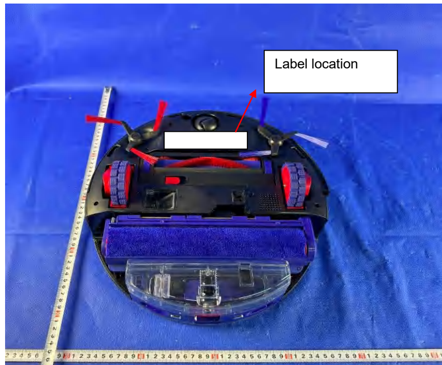
Figure 7. Internal view
