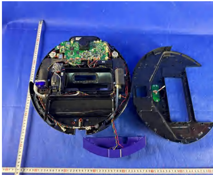
Figure 17. Internal view
