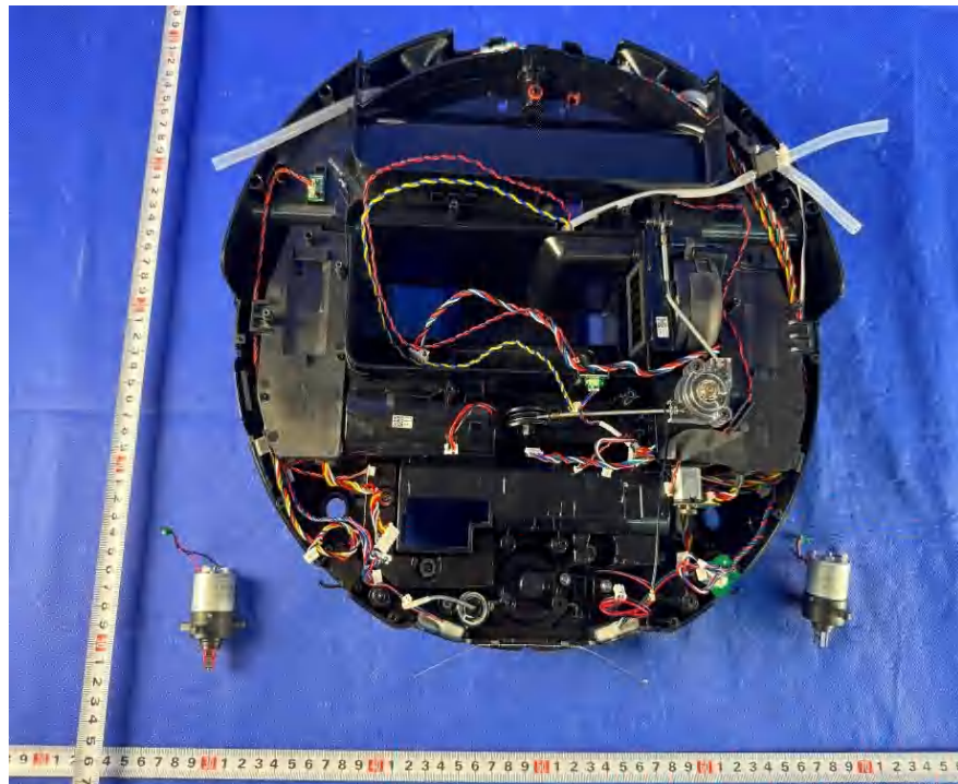
Figure 39. Internal view
