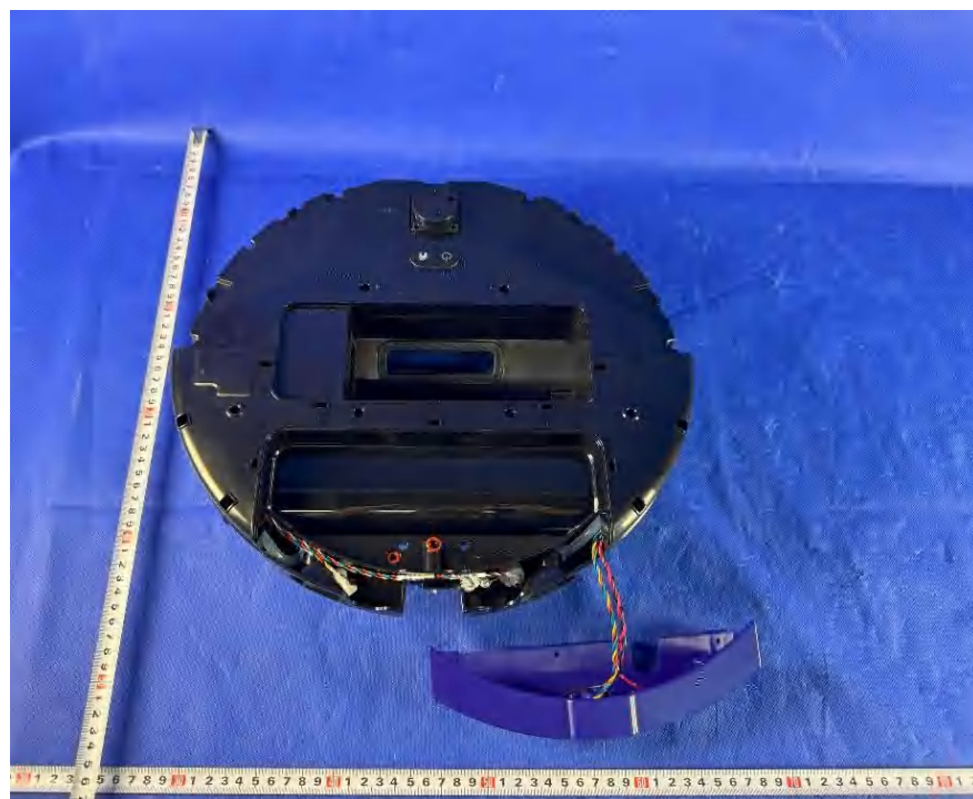
Figure 16. Internal view
