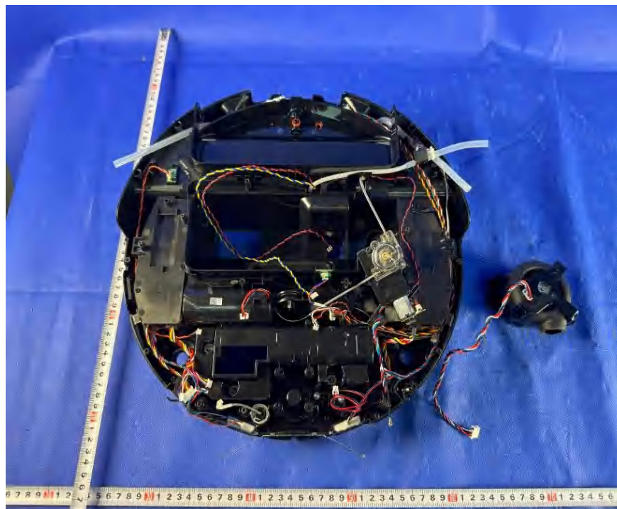
Figure 46. Internal view
