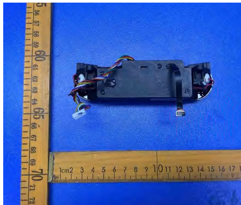
Figure 32. Laser module
