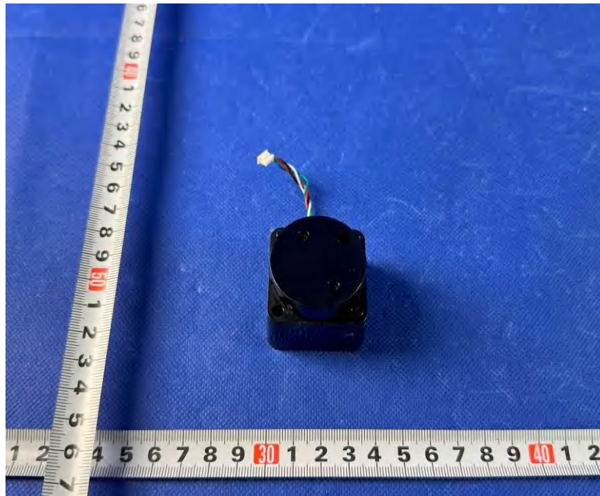
Figure 33. Lidar Motor
