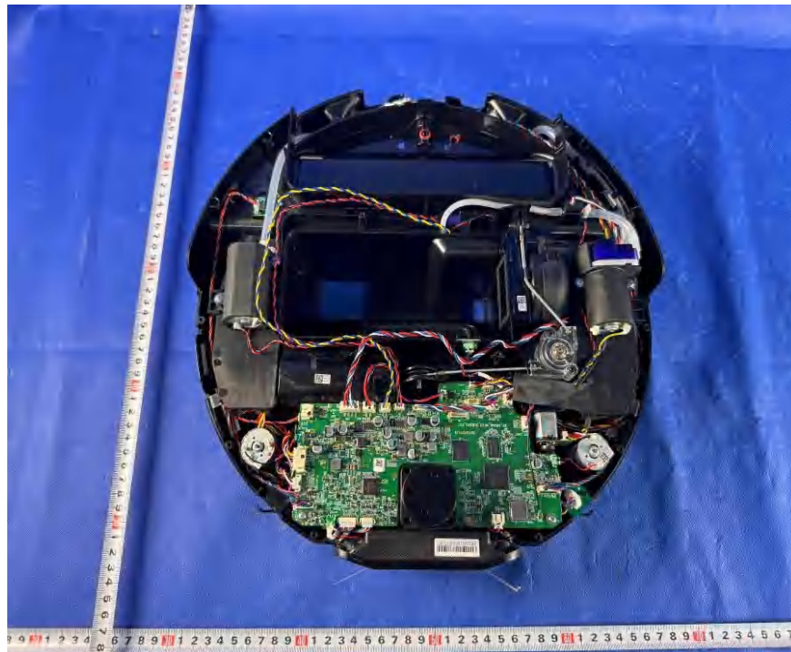
Figure 25. Internal view
