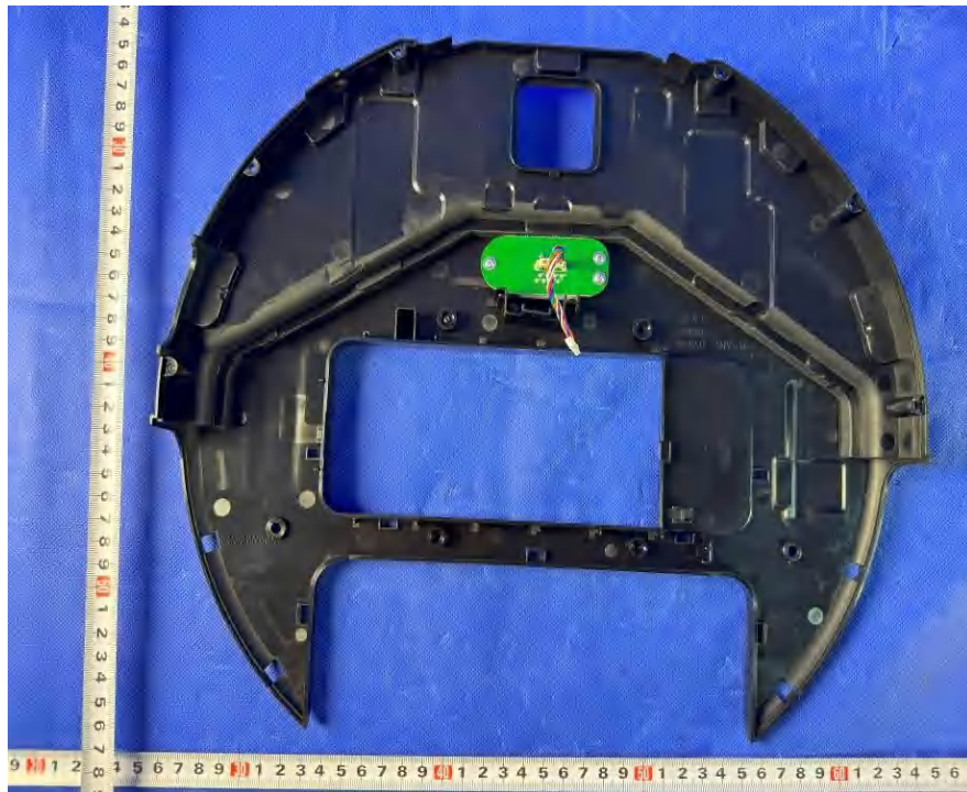
Figure 21. Internal view
