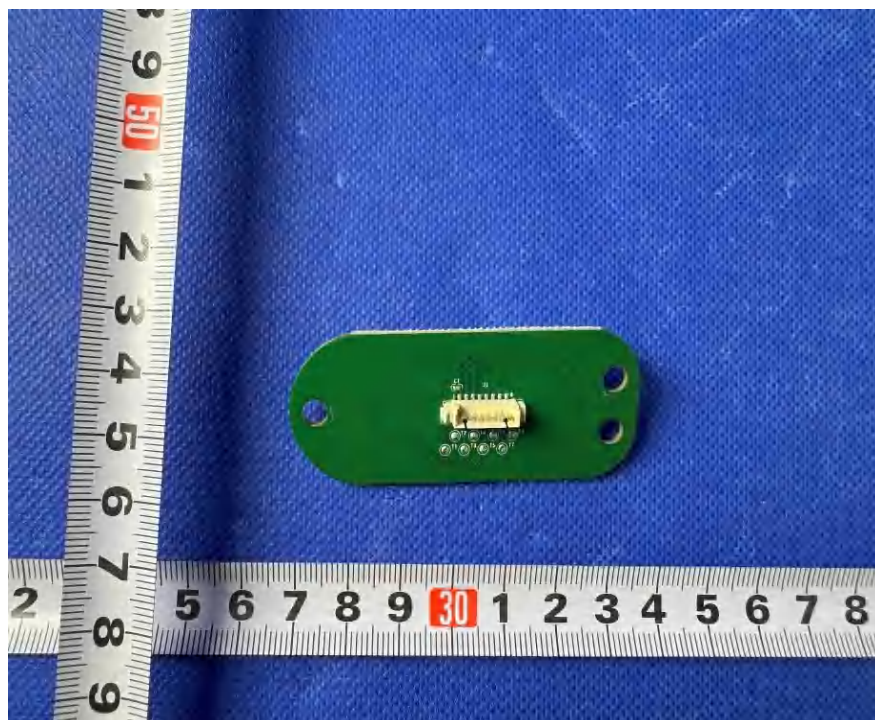
Figure 24. Control PCB
