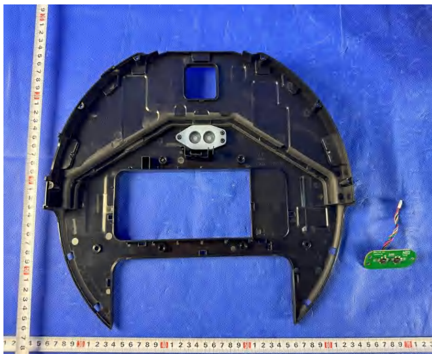
Figure 22. Internal view
