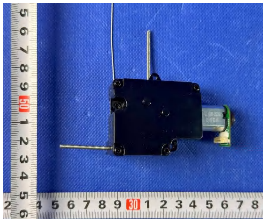
Figure 50. Roller lifting motor
