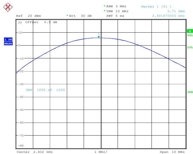
1Mbps_Lowest
